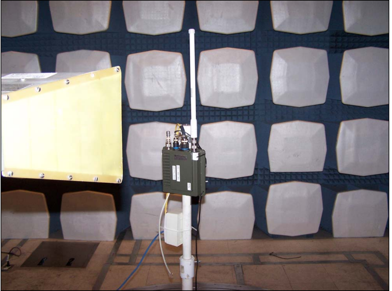
Photograph 8. Radiated Spurious Emission, Test Setup, M25 Radio
