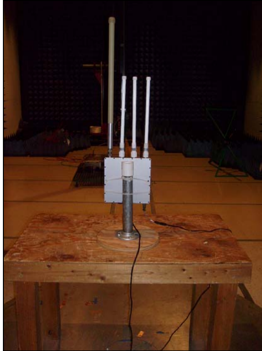
Photograph 4. Radiated Emission, Test Setup, Rear View
