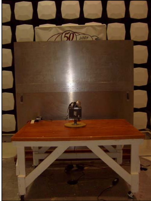
Photograph 6. Conducted Emissions, Test Setup, M25 Radio
