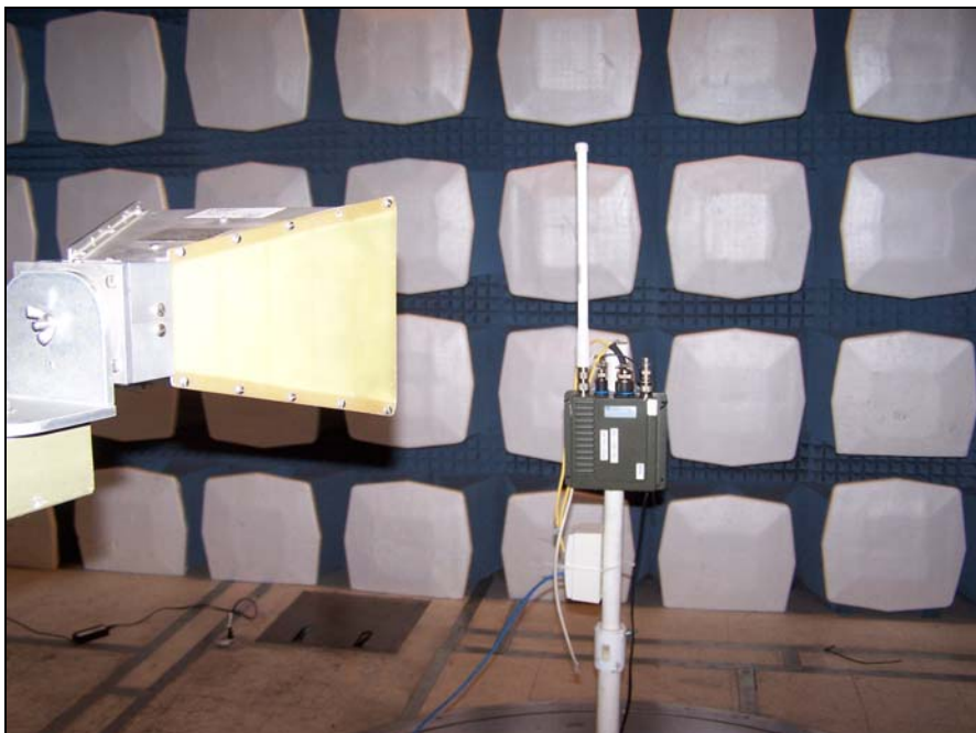
Photograph 11. Radiated Spurious Emission, Test Setup, M5 Radio
