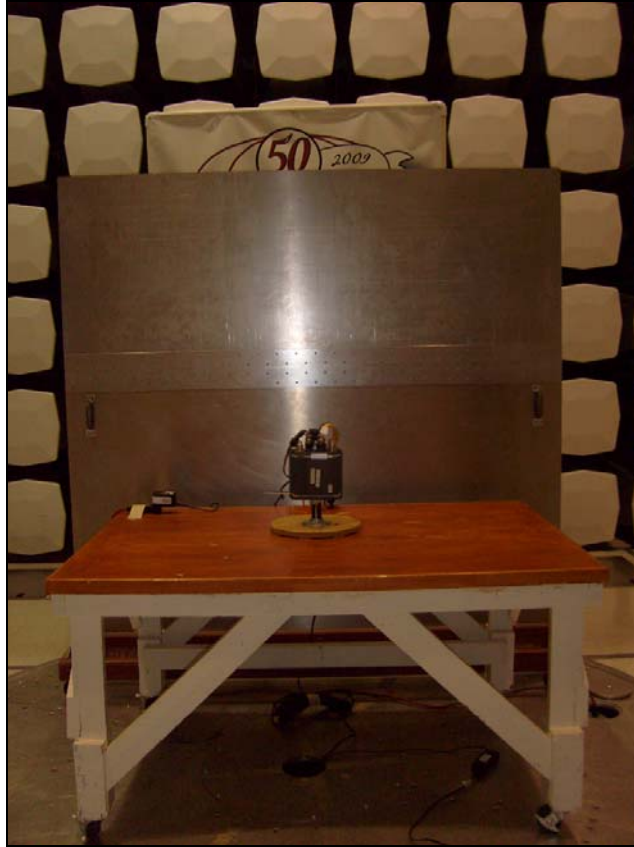
Photograph 9. Conducted Emissions, Test Setup, M5 Radio
