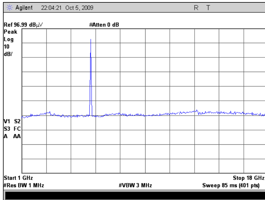
Plot 85. Radiated Spurious Emissions, Low Channel, 802.11a, 1 GHz – 18 GHz, M5 Radio
