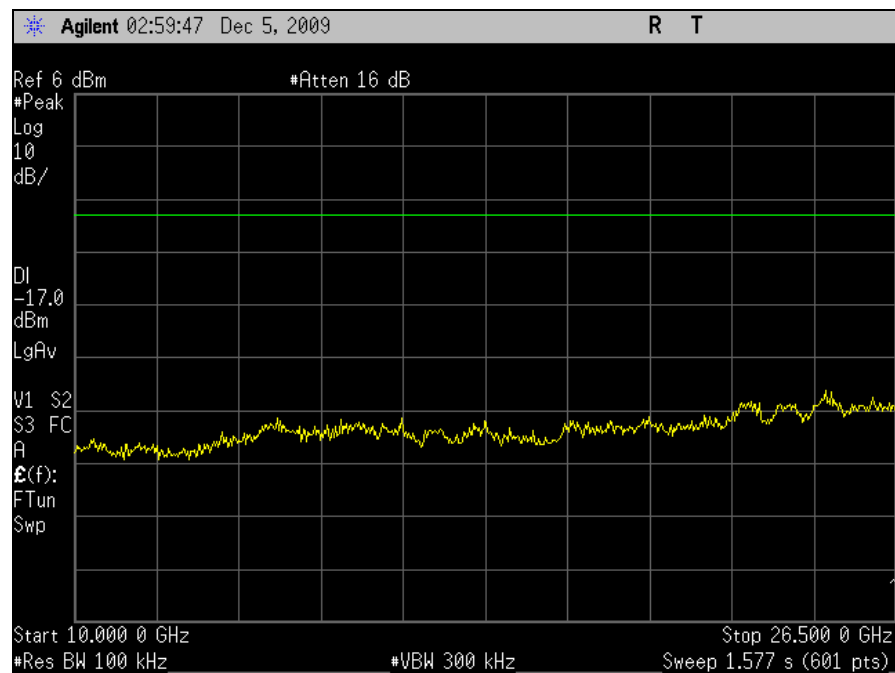
Plot 60. Conducted Emissions, Mid Channel, 10 GHz – 26.5 GHz, 802.11g, M25 Radio
