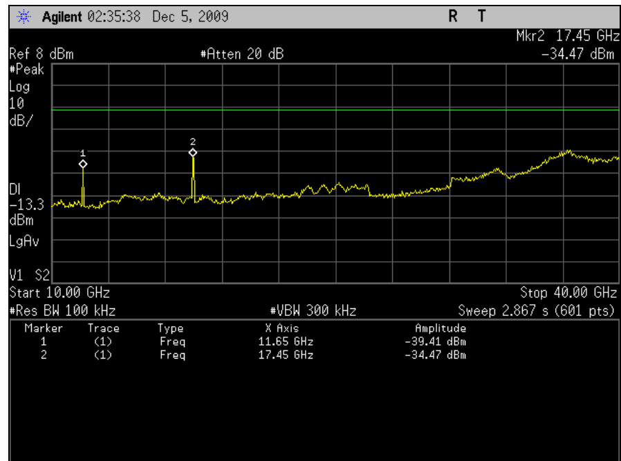
Plot 100. Conducted Emissions, High Channel, 10 GHz – 40 GHz, 802.11a, M5 Radio
