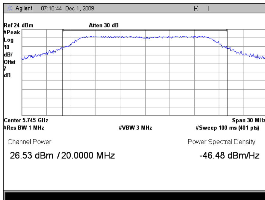
Plot 82. Peak Output Power, Low Channel (5745MHz), M5 Radio
