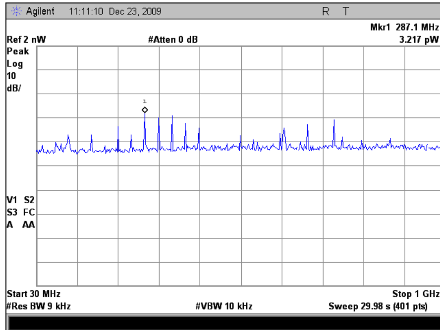
Plot 42. Receiver Spurious Emission, 30 MHz – 1 GHz, 802.11a, M25 Radio
