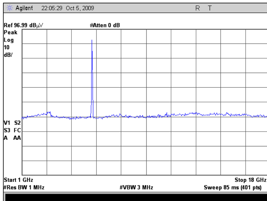
Plot 86. Radiated Spurious Emissions, Mid Channel, 802.11a, 1 GHz – 18 GHz, M5 Radio
