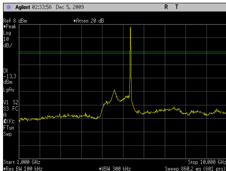
Plot 99. Conducted Emissions, High Channel, 1 GHz – 10 GHz, 802.11a, M5 Radio
