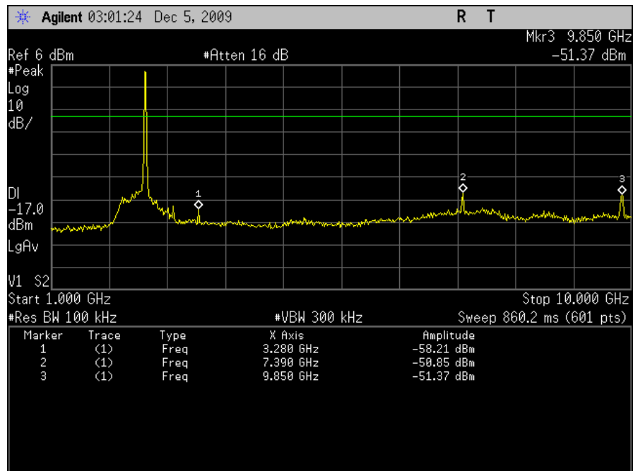
Plot 62. Conducted Emissions, High Channel, 1 GHz – 10 GHz, 802.11g, M25 Radio
