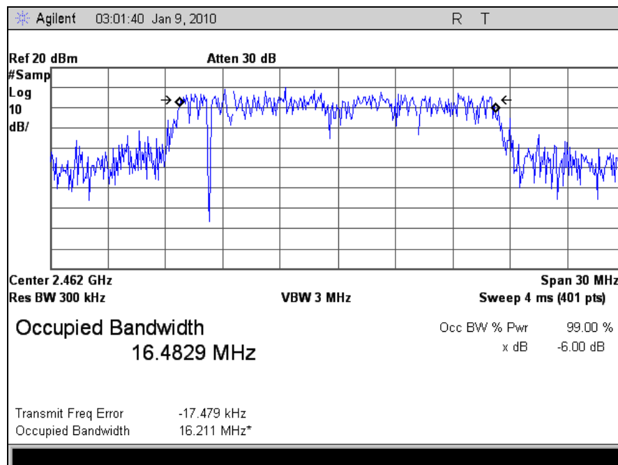
Plot 19. Occupied Bandwidth, High Channel (2462 MHz), 802.11g, 99% BW, M25 Radio
