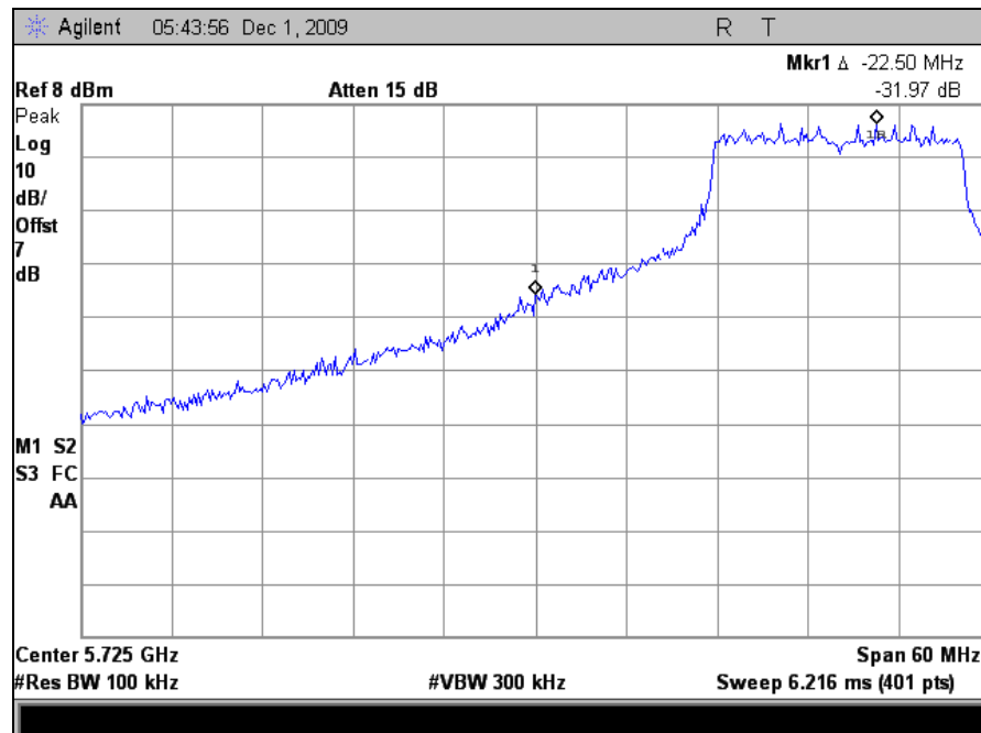
Plot 64. Conducted Band Edge, Low, 802.11a, M25 Radio
