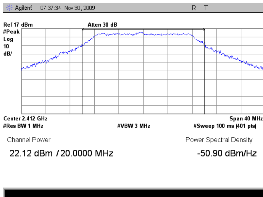
Plot 23. Peak Output Power, Low Channel (2412MHz), 802.11g, M25 Radio
