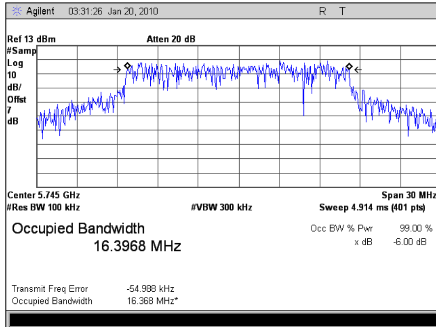
Plot 8. Occupied Bandwidth, Low Channel (5745MHz), 802.11a, 6dB BW, M25 Radio
