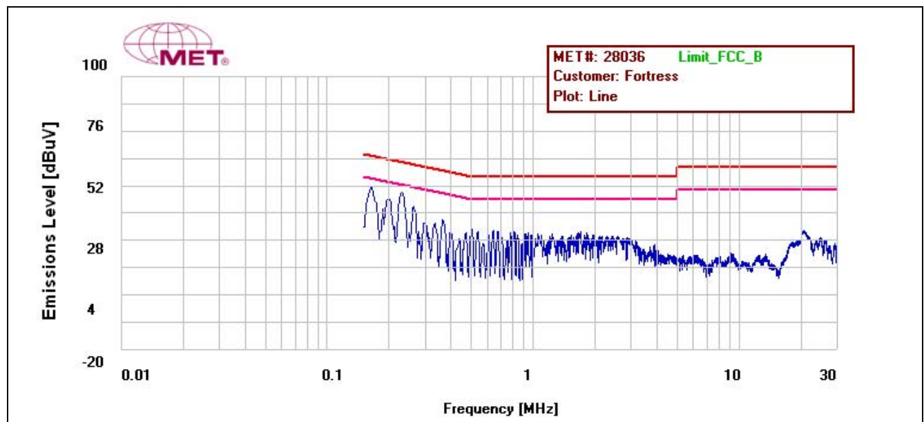
Plot 74. Conducted Emissions, Phase Line, M5 Radio
