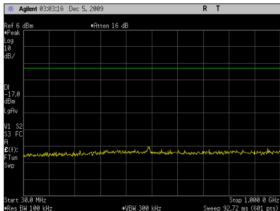
Plot 61. Conducted Emissions, High Channel, 30 MHz – 1 GHz, 802.11g, M25 Radio
