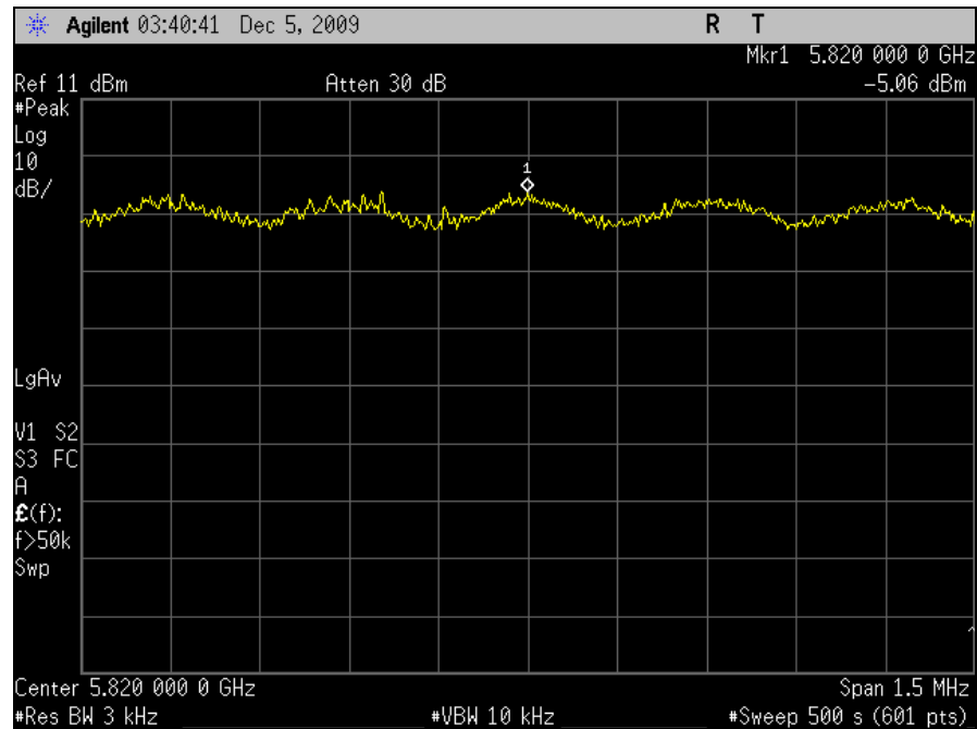
Plot 105. Peak Power Spectral Density, High Channel, M5 Radio
