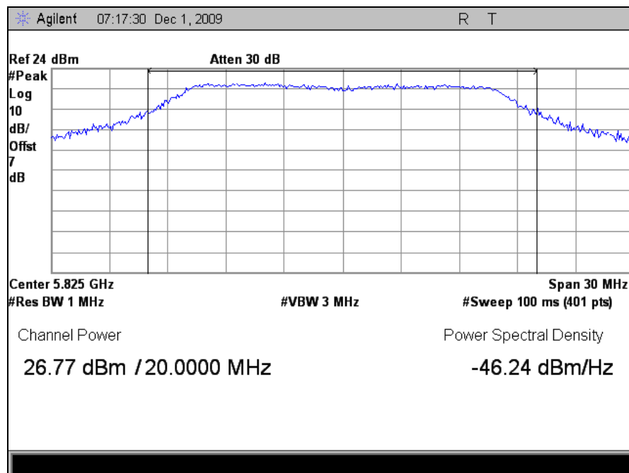
Plot 84. Peak Output Power, High Channel (5825MHz), M5 Radio
