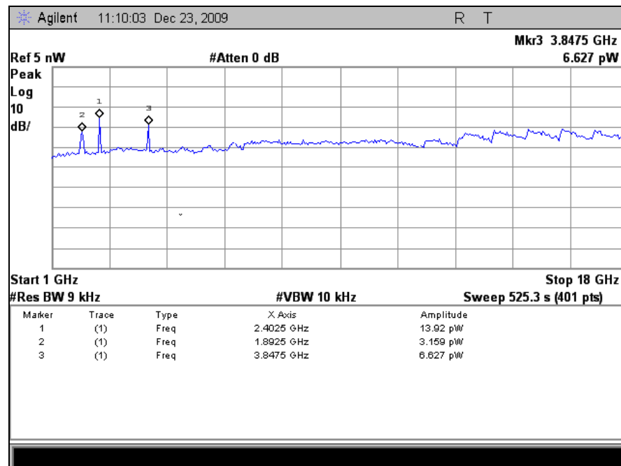
Plot 43. Receiver Spurious Emission, 1 GHz – 18 GHz, 802.11a, M25 Radio
