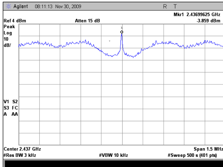
Plot 72. Peak Power Spectral Density, Mid Channel, 802.11g, M25 Radio
