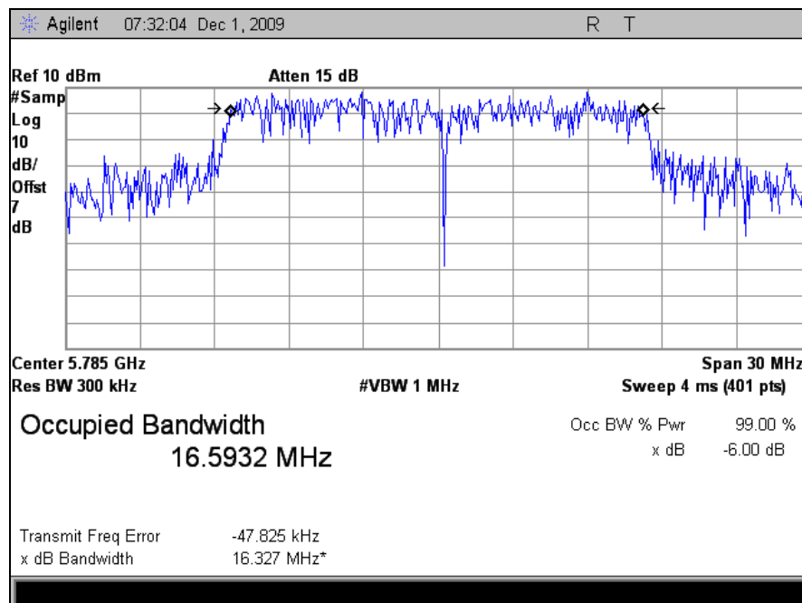
Plot 77. Occupied Bandwidth, Mid Channel (5785MHz), 99% BW, M5 Radio
