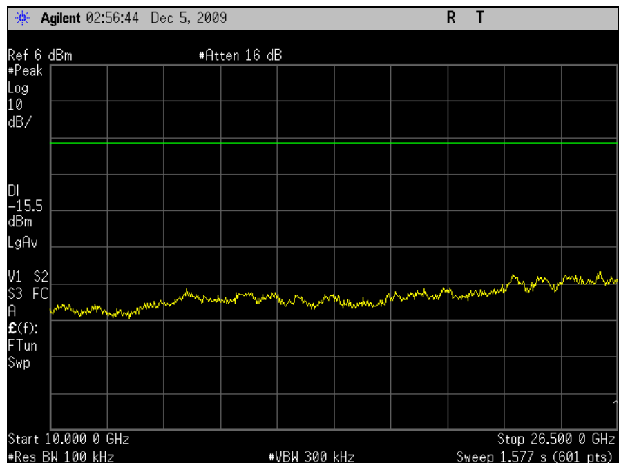
Plot 57. Conducted Emissions, Low Channel, 10 GHz – 26.5 GHz, 802.11g, M25 Radio
