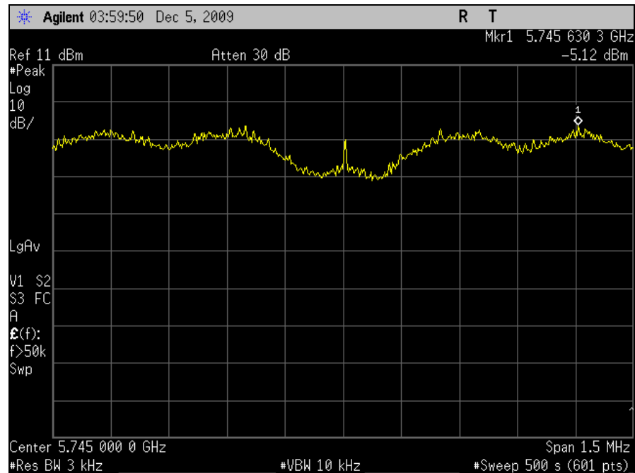
Plot 103. Peak Power Spectral Density, Low Channel, M5 Radio
