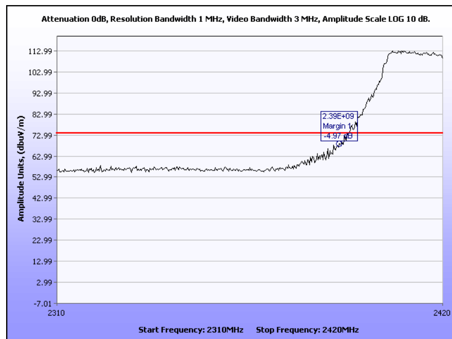
Plot 39. Lower Band Edge, Peak, 802.11g, M25 Radio
