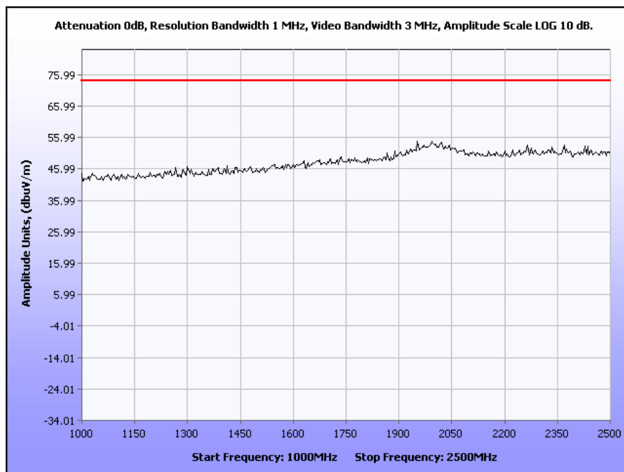
Plot 29. Radiated Spurious Emissions, Low Channel, 802.11g, 1 GHz – 2.5 GHz (Peak), M25 Radio
