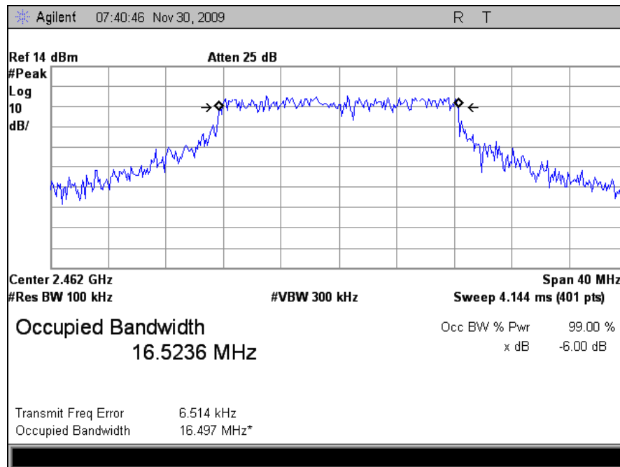
Plot 16. Occupied Bandwidth, High Channel (2462MHz), 802.11g, 6dB BW, M25 Radio
