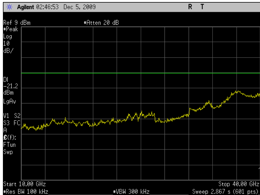
Plot 54. Conducted Emissions, High Channel, 10 GHz – 40 GHz, 802.11a, M25 Radio
