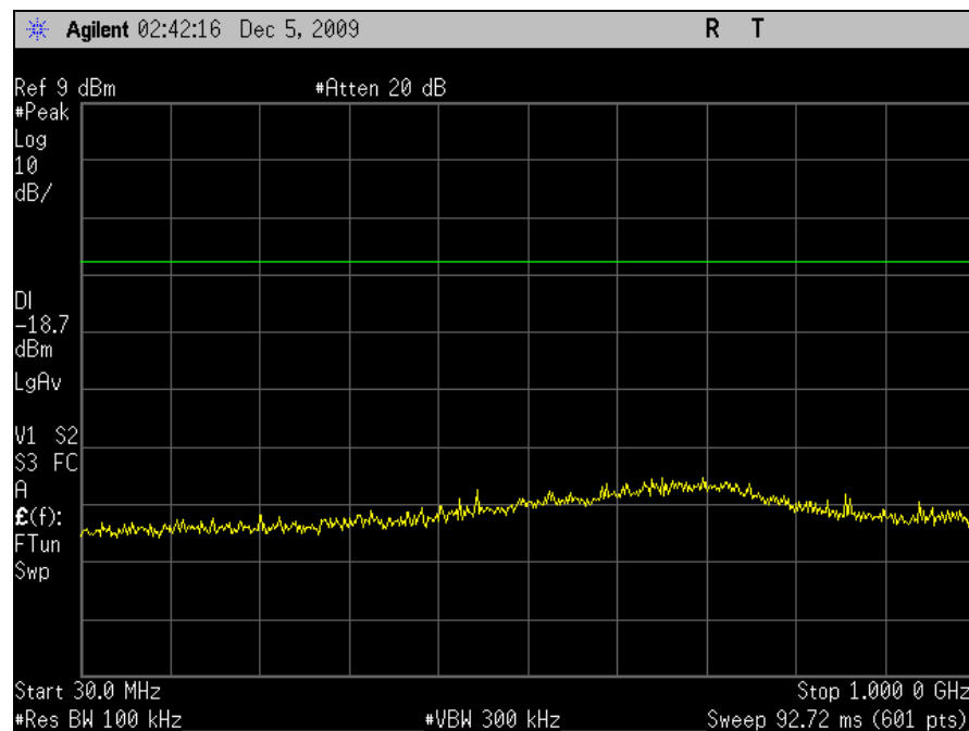
Plot 46. Conducted Emissions, Low Channel, 30 MHz – 1 GHz, 802.11a, M25 Radio
