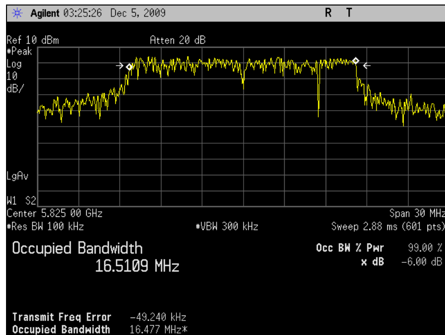
Plot 81. Occupied Bandwidth, High Channel (5825MHz), 6dB BW, M5 Radio
