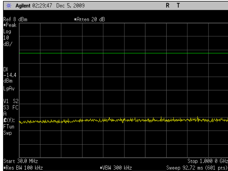
Plot 92. Conducted Emissions, Low Channel, 30 MHz – 1 GHz, 802.11a, M5 Radio
