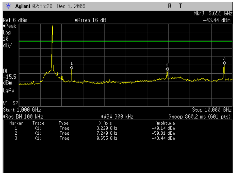
Plot 56. Conducted Emissions, Low Channel, 1 GHz – 10 GHz, 802.11g, M25 Radio
