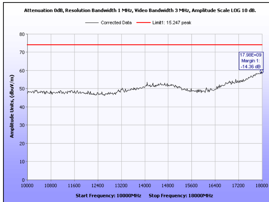
Plot 31. Radiated Spurious Emissions, Low Channel, 802.11g, 10 GHz – 18 GHz (Peak with Pre-Amp), M25 Radio
