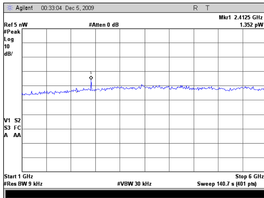
Plot 89. Receiver Spurious Emission, 1 GHz – 6 GHz, M5 Radio
