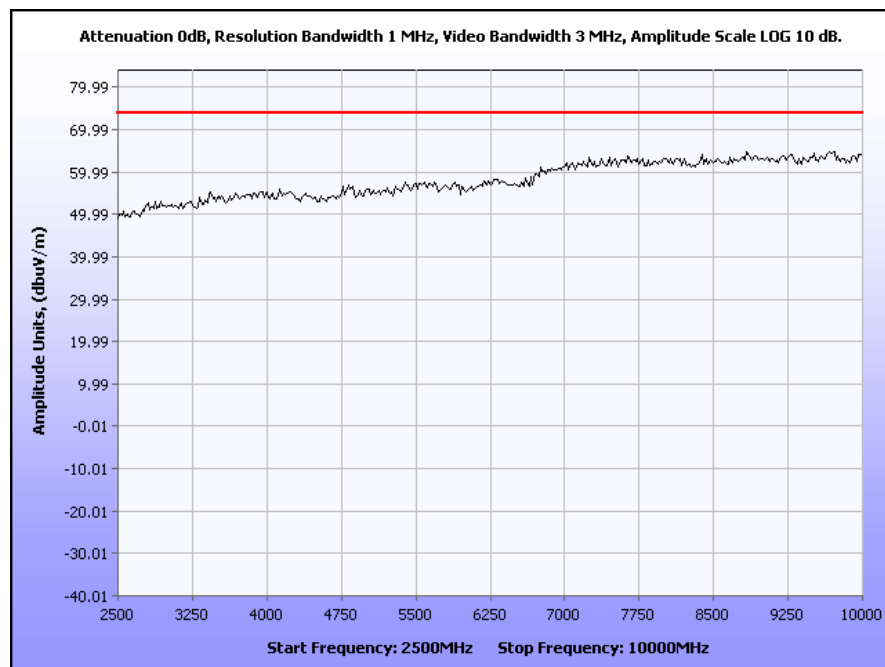
Plot 33. Radiated Spurious Emissions, Mid Channel, 802.11g, 2.5 GHz – 10 GHz (Peak), M25 Radio
