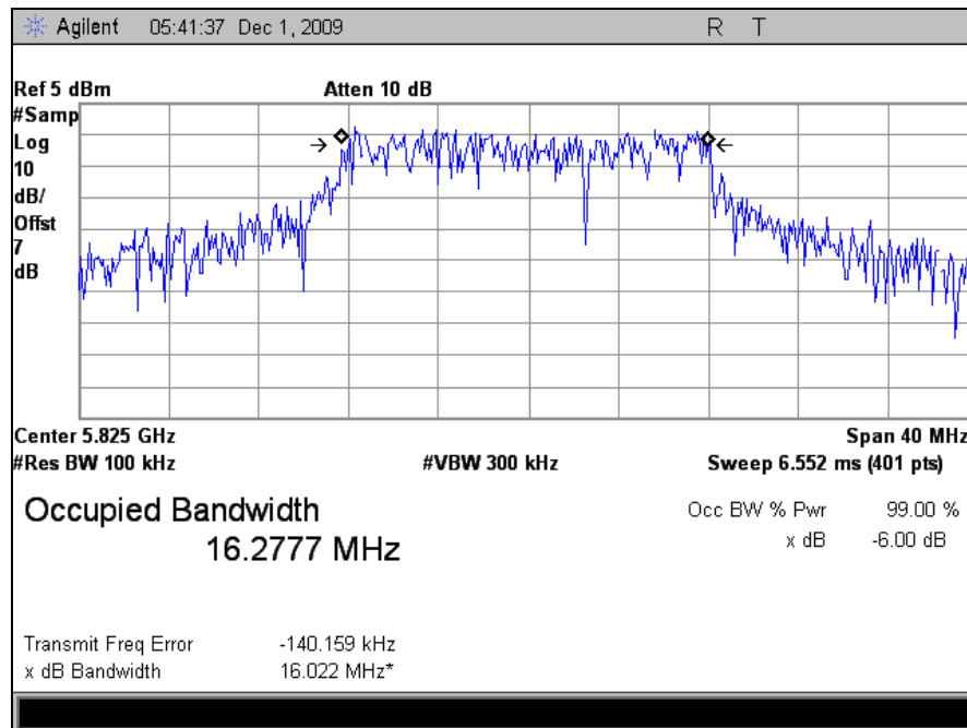
Plot 10. Occupied Bandwidth, High Channel (5825MHz), 802.11a, 6dB BW, M25 Radio
