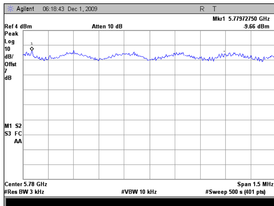
Plot 69. Peak Power Spectral Density, Mid Channel, 802.11a, M25 Radio
