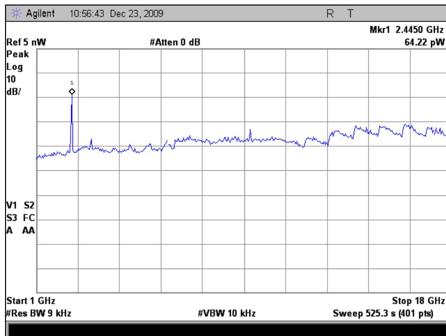
Plot 45. Receiver Spurious Emission, 1 GHz – 18 GHz, 802.11g, M25 Radio
