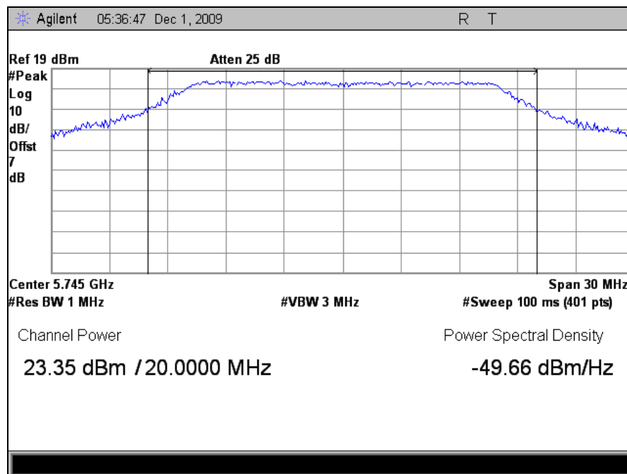
Plot 20. Peak Output Power, Low Channel (5745MHz), 802.11a, M25 Radio
