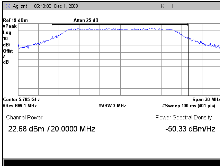
Plot 21. Peak Output Power, Mid Channel (5785MHz), 802.11a, M25 Radio
