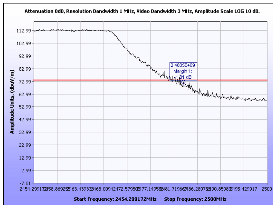
Plot 41. Upper Band Edge, Peak, 802.11g, M25 Radio
