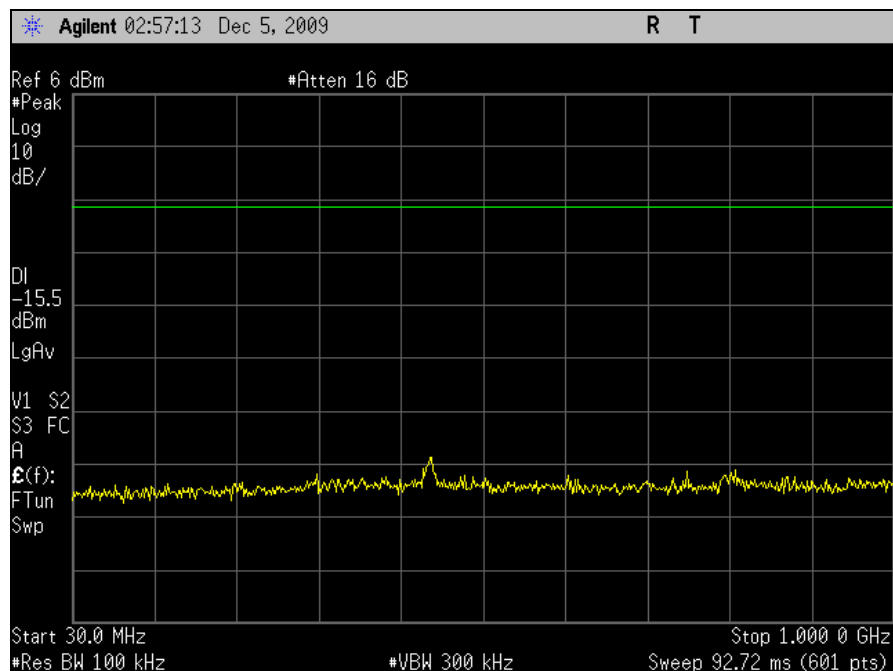
Plot 55. Conducted Emissions, Low Channel, 30 MHz – 1 GHz, 802.11g, M25 Radio
