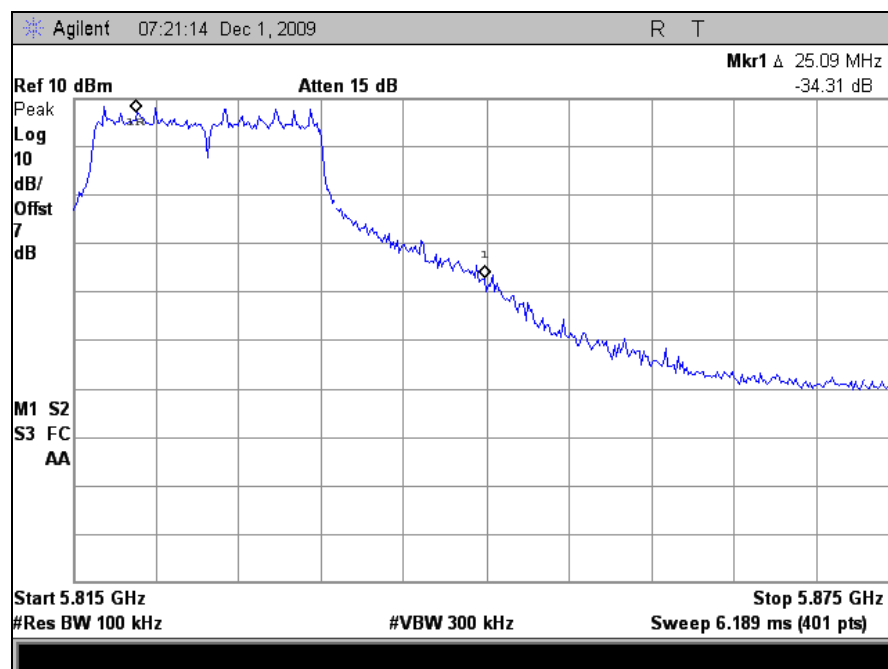
Plot 102. Conducted Band Edge, High, M5 Radio
