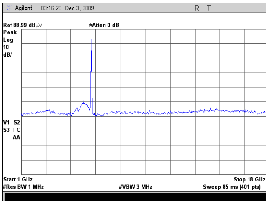
Plot 27. Radiated Spurious Emissions, Mid Channel, 802.11a, 1 GHz – 18 GHz, M25 Radio
