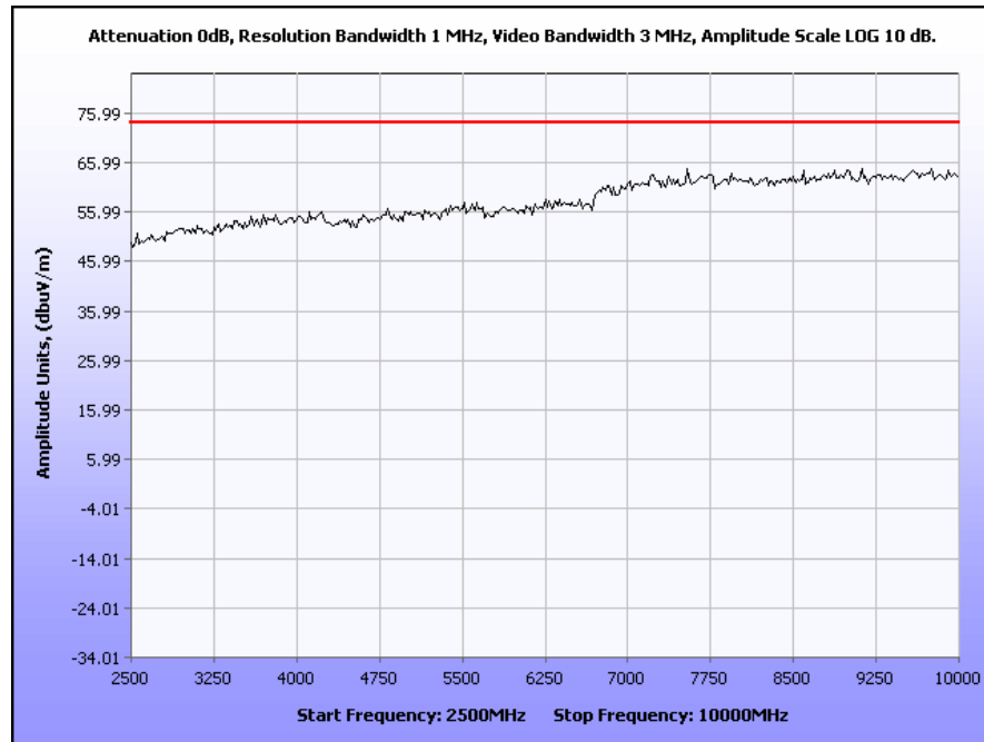
Plot 30. Radiated Spurious Emissions, Low Channel, 802.11g, 2.5 GHz – 10 GHz (Peak), M25 Radio
