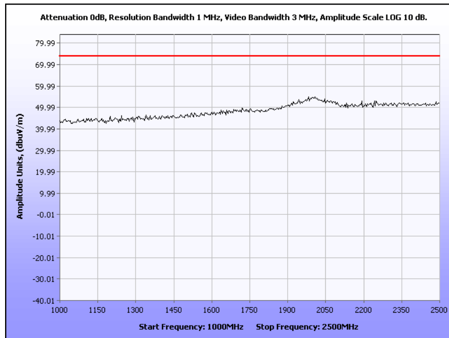
Plot 32. Radiated Spurious Emissions, Mid Channel, 802.11g, 1 GHz – 2.5 GHz (Peak), M25 Radio
