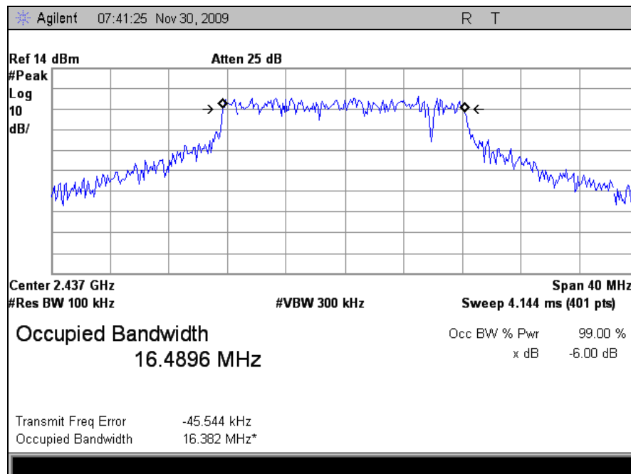
Plot 15. Occupied Bandwidth, Low Channel (2437MHz), 802.11g, 6dB BW, M25 Radio
