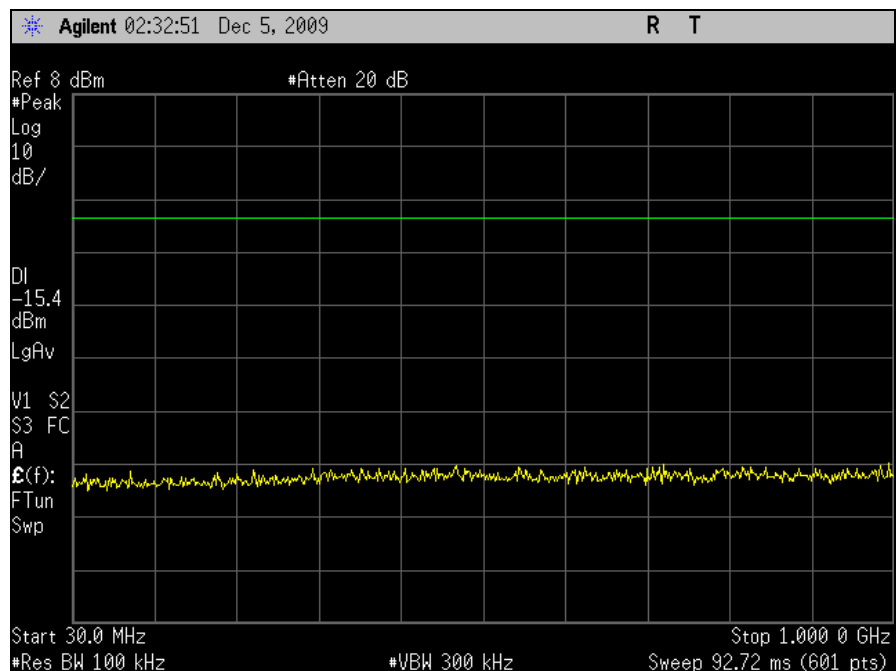
Plot 95. Conducted Emissions, Mid Channel, 30 MHz – 1 GHz, , 802.11a, M5 Radio
