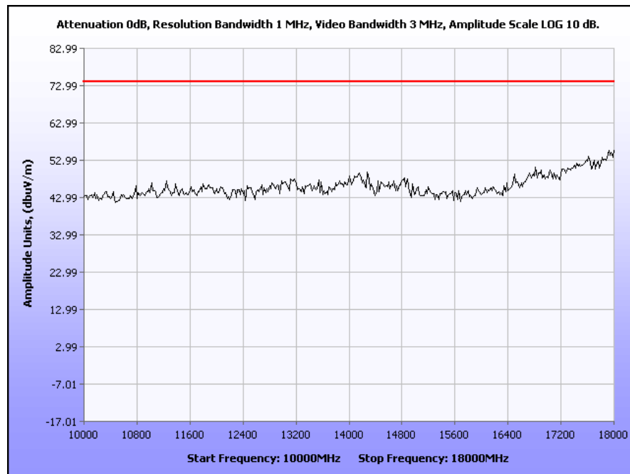
Plot 34. Radiated Spurious Emissions, Mid Channel, 802.11g, 10 GHz – 18 GHz (Peak with Pre-Amp), M25 Radio
