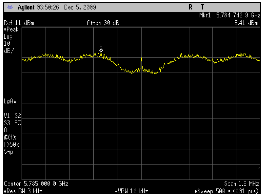
Plot 104. Peak Power Spectral Density, Mid Channel, M5 Radio
