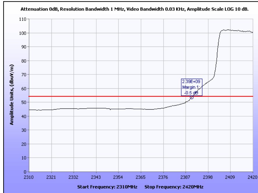
Plot 38. Lower Band Edge, Average, 802.11g, M25 Radio
