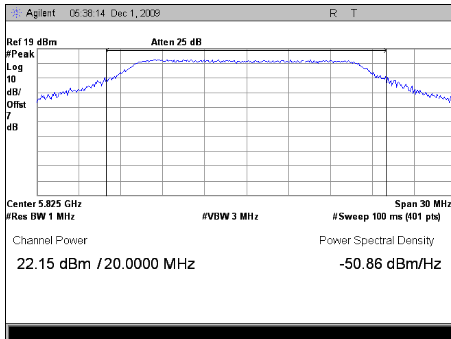
Plot 22. Peak Output Power, High Channel (5825MHz), 802.11a, M25 Radio
