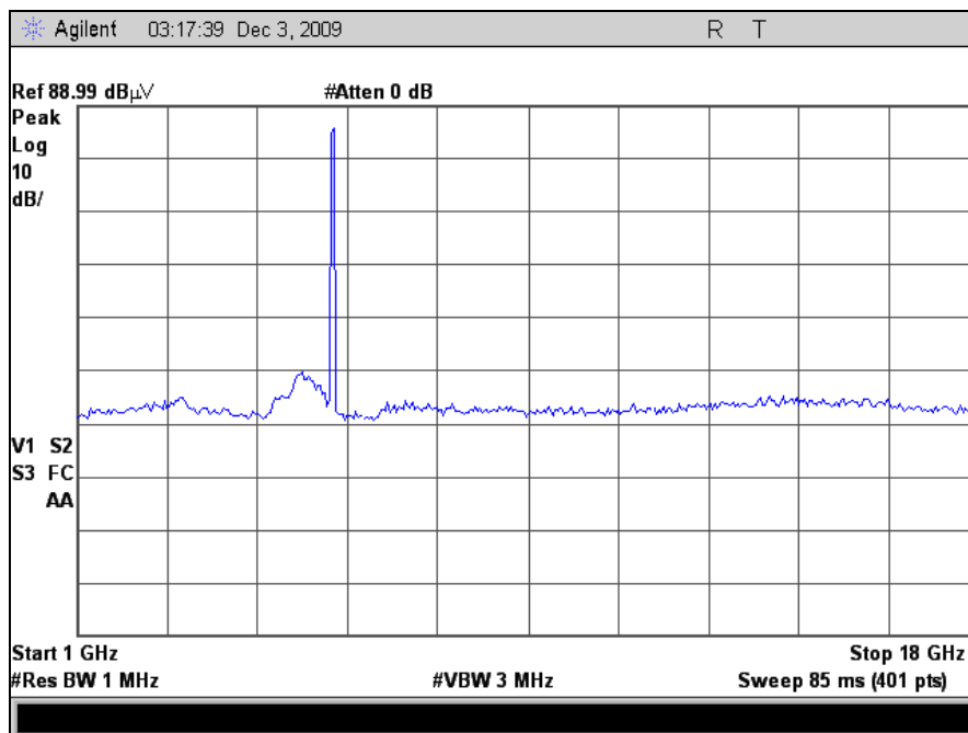
Plot 28. Radiated Spurious Emissions, High Channel, 802.11a, 1 GHz – 18 GHz, M25 Radio
