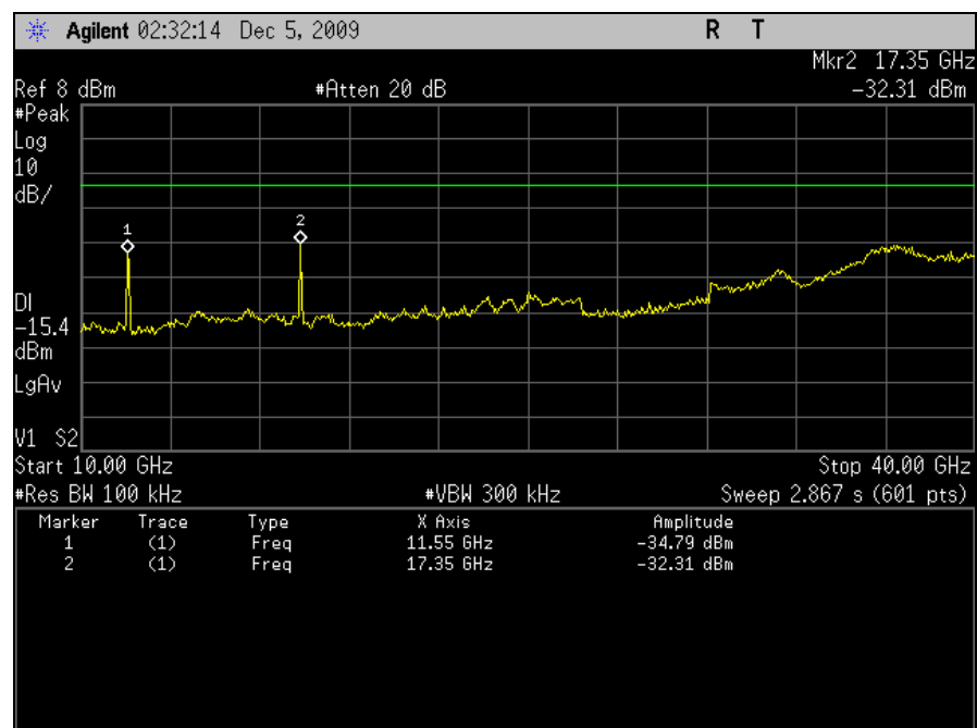
Plot 97. Conducted Emissions, Mid Channel, 10 GHz – 40 GHz, 802.11a, M5 Radio
