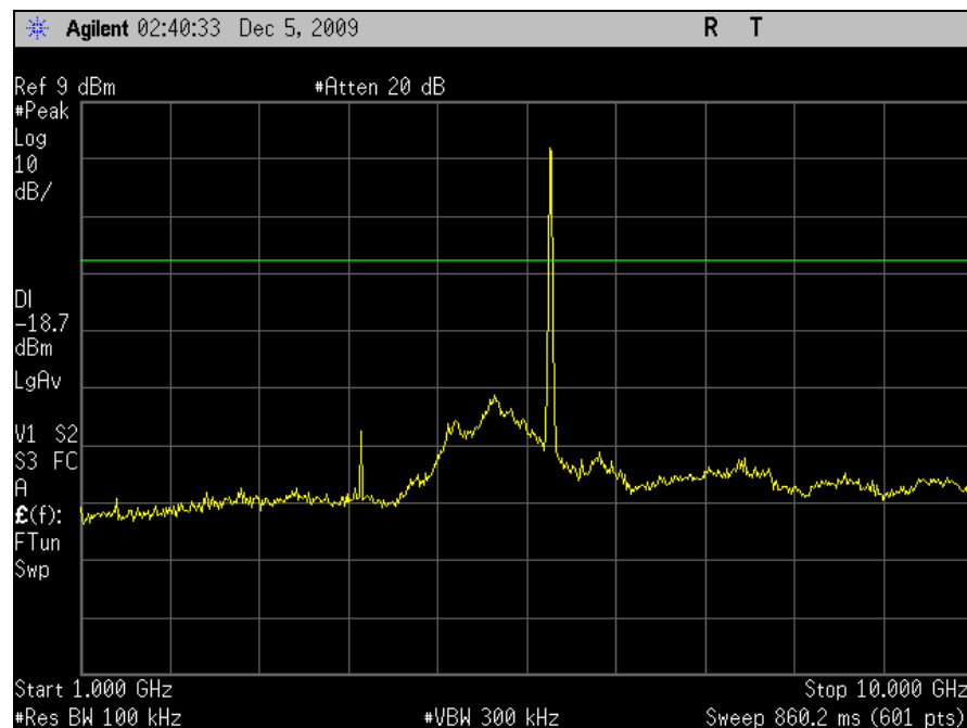
Plot 47. Conducted Emissions, Low Channel, 1 GHz – 10 GHz, 802.11a, M25 Radio
