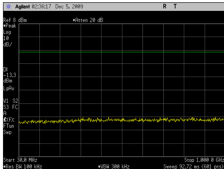
Plot 98. Conducted Emissions, High Channel, 30 MHz – 1 GHz, 802.11a, M5 Radio
