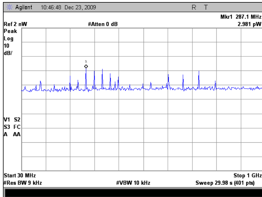
Plot 44. Receiver Spurious Emission, 30 MHz – 1 GHz, 802.11g, M25 Radio
