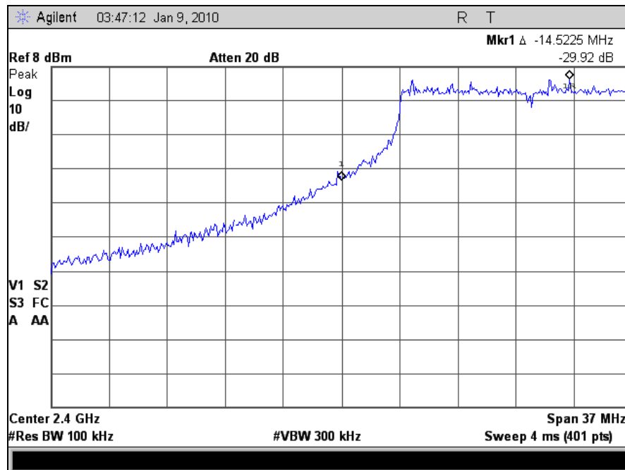
Plot 66. Conducted Band Edge, Low, 802.11g, M25 Radio
