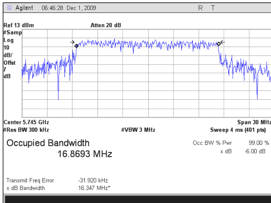
Plot 11. Occupied Bandwidth, Low Channel (5745MHz), 802.11a, 99% BW, M25 Radio
