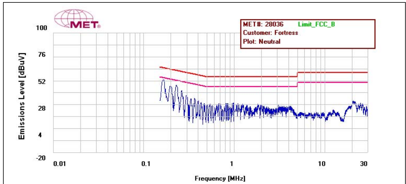
Plot 75. Conducted Emissions, Neutral Line, M5 Radio
