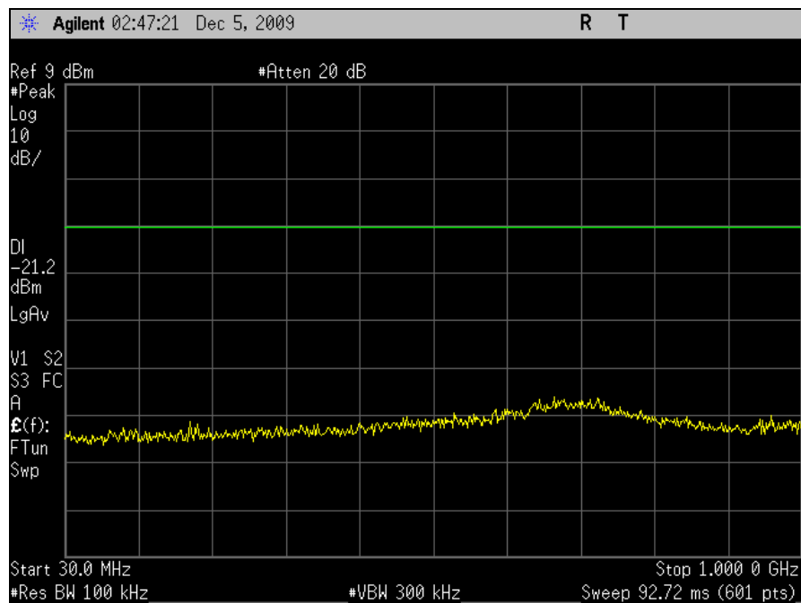
Plot 52. Conducted Emissions, High Channel, 30 MHz – 1 GHz, 802.11a, M25 Radio
