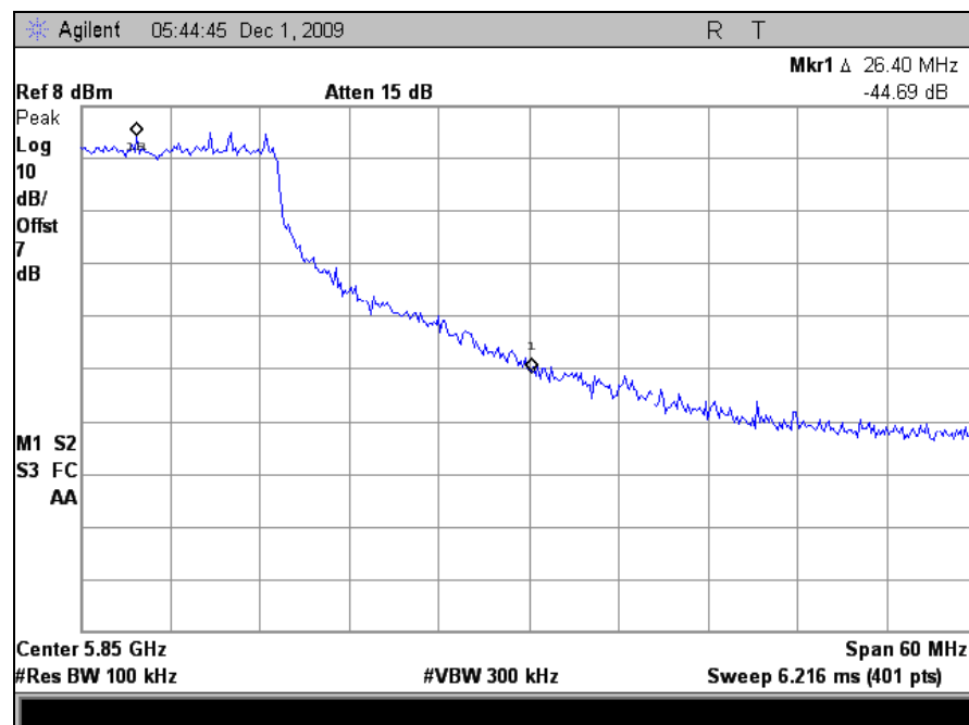
Plot 65. Conducted Band Edge, High, 802.11a, M25 Radio
