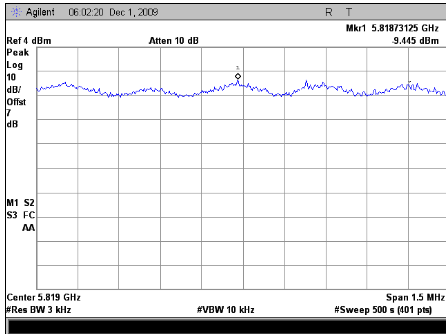
Plot 70. Peak Power Spectral Density, High Channel, 802.11a, M25 Radio
