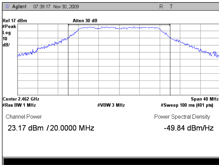
Plot 25. Peak Output Power, High Channel (2462MHz), 802.11g, M25 Radio
