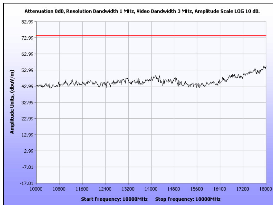
Plot 37. Radiated Spurious Emissions, High Channel, 802.11g, 10 GHz – 18 GHz (Peak with Pre-Amp), M25 Radio
