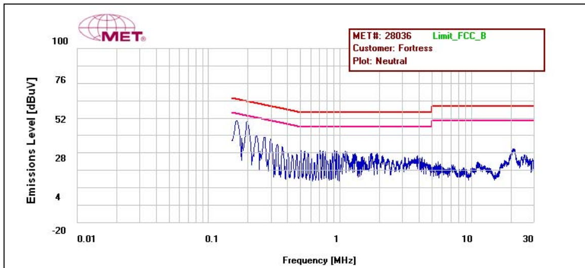
Plot 7. Conducted Emissions, Neutral Line, M25 Radio
