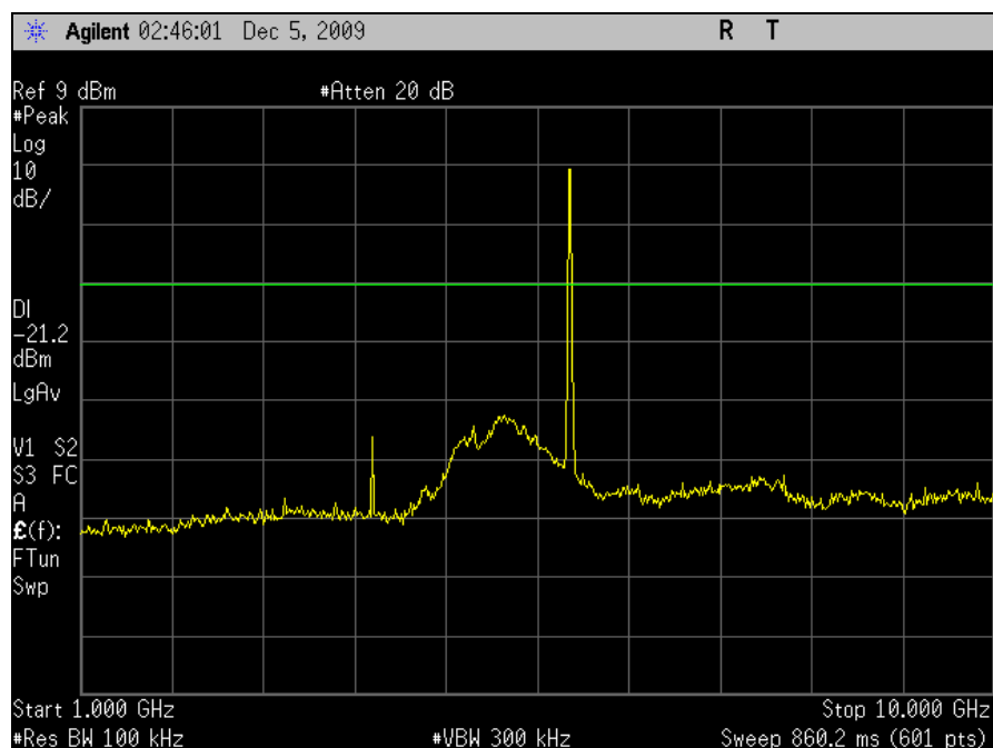
Plot 53. Conducted Emissions, High Channel, 1 GHz – 10 GHz, 802.11a, M25 Radio
