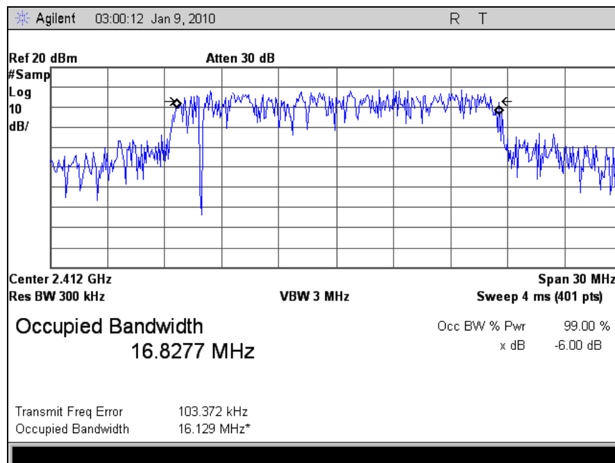
Plot 17. Occupied Bandwidth, Low Channel (2412 MHz), 802.11g, 99% BW, M25 Radio
