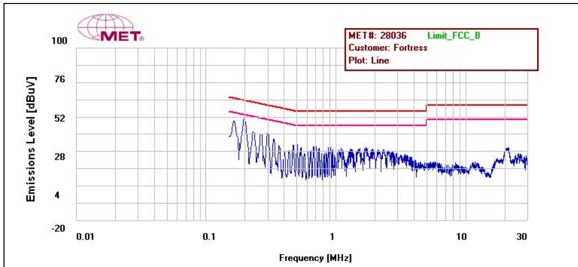
Plot 6. Conducted Emissions, Phase Line, M25 Radio
