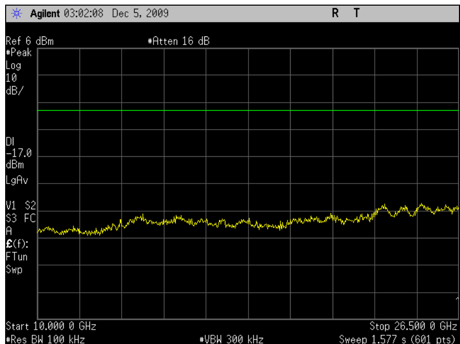
Plot 63. Conducted Emissions, High Channel, 10 GHz – 26.5 GHz, 802.11g, M25 Radio
