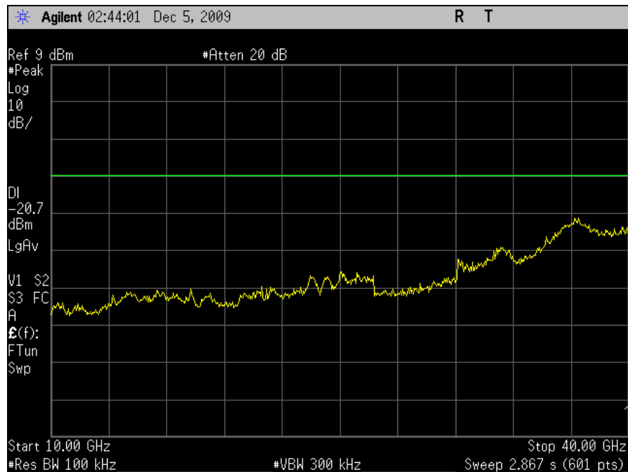
Plot 51. Conducted Emissions, Mid Channel, 10 GHz – 40 GHz, 802.11a, M25 Radio
