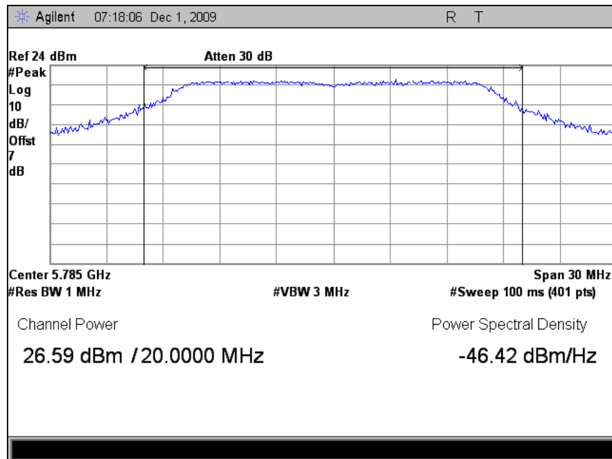
Plot 83. Peak Output Power, Mid Channel (5785MHz), M5 Radio
