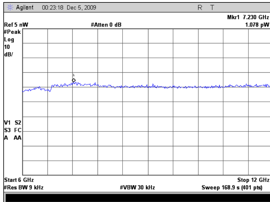
Plot 90. Receiver Spurious Emission, 6 GHz – 12 GHz, M5 Radio
