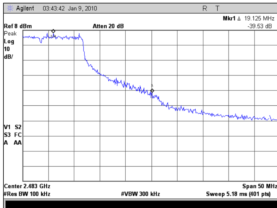
Plot 67. Conducted Band Edge, High, 802.11g, M25 Radio
