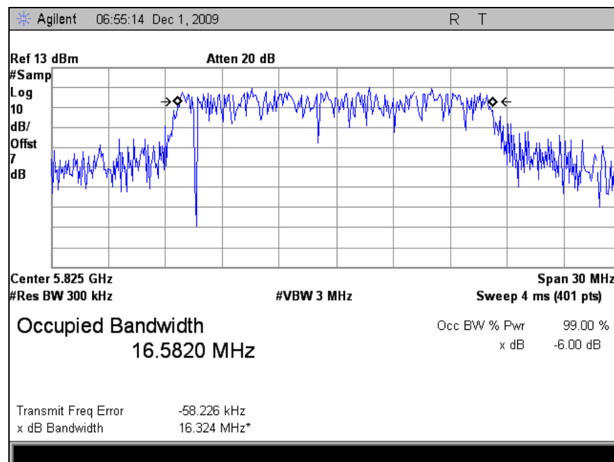
Plot 13. Occupied Bandwidth, High Channel (5825MHz), 802.11a, 99% BW, M25 Radio
