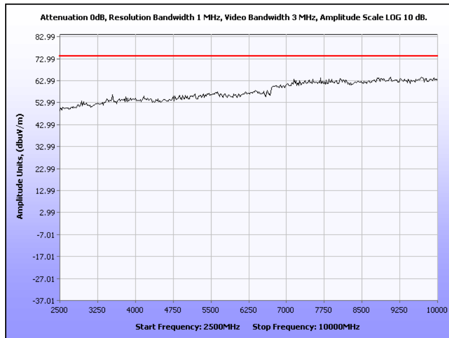
Plot 36. Radiated Spurious Emissions, High Channel, 802.11g, 2.5 GHz – 10 GHz (Peak), M25 Radio
