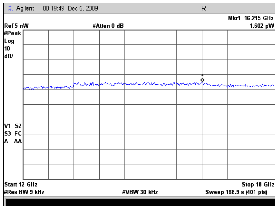
Plot 91. Receiver Spurious Emission, 12 GHz – 18 GHz, M5 Radio
