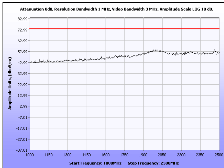
Plot 35. Radiated Spurious Emissions, High Channel, 802.11g, 1 GHz – 2.5 GHz (Peak), M25 Radio
