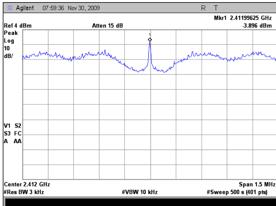
Plot 71. Peak Power Spectral Density, Low Channel, 802.11g, M25 Radio
