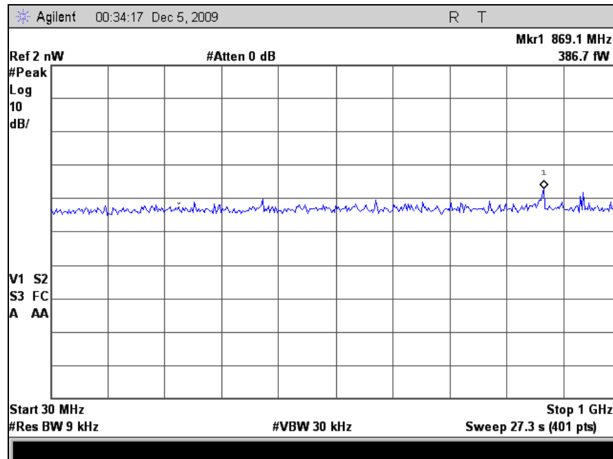
Plot 88. Receiver Spurious Emission, 30 MHz – 1 GHz, M5 Radio
