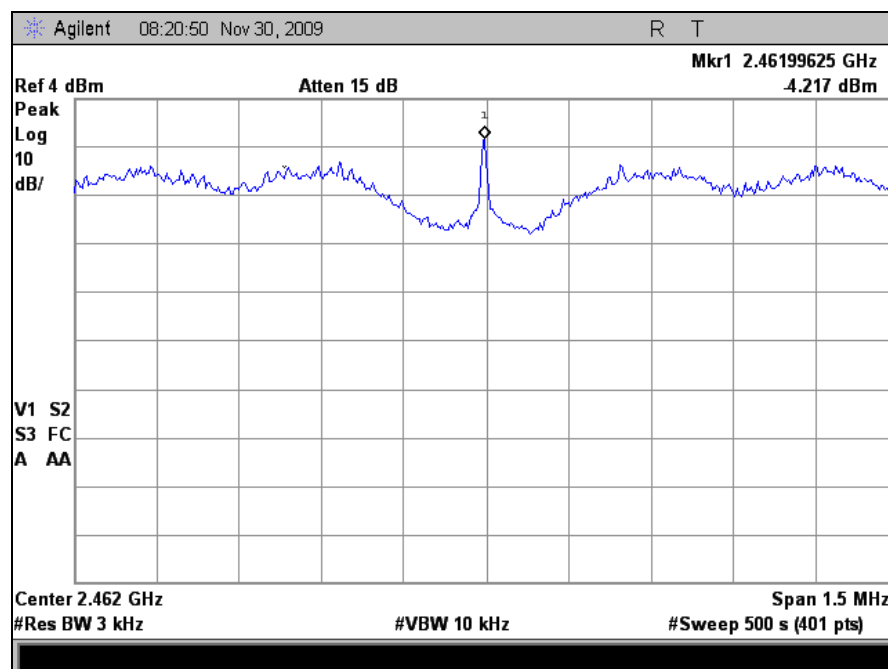
Plot 73. Peak Power Spectral Density, High Channel, 802.11g, M25 Radio
