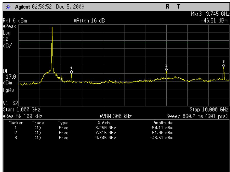
Plot 59. Conducted Emissions, Mid Channel, 1 GHz – 10 GHz, 802.11g, M25 Radio
