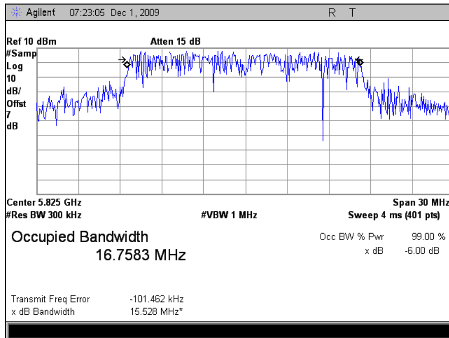
Plot 78. Occupied Bandwidth, High Channel (5825MHz), 99% BW, M5 Radio
