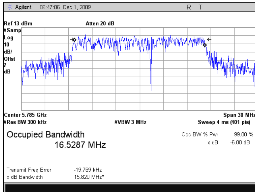
Plot 12. Occupied Bandwidth, Mid Channel (5785MHz), 802.11a, 99% BW, M25 Radio
