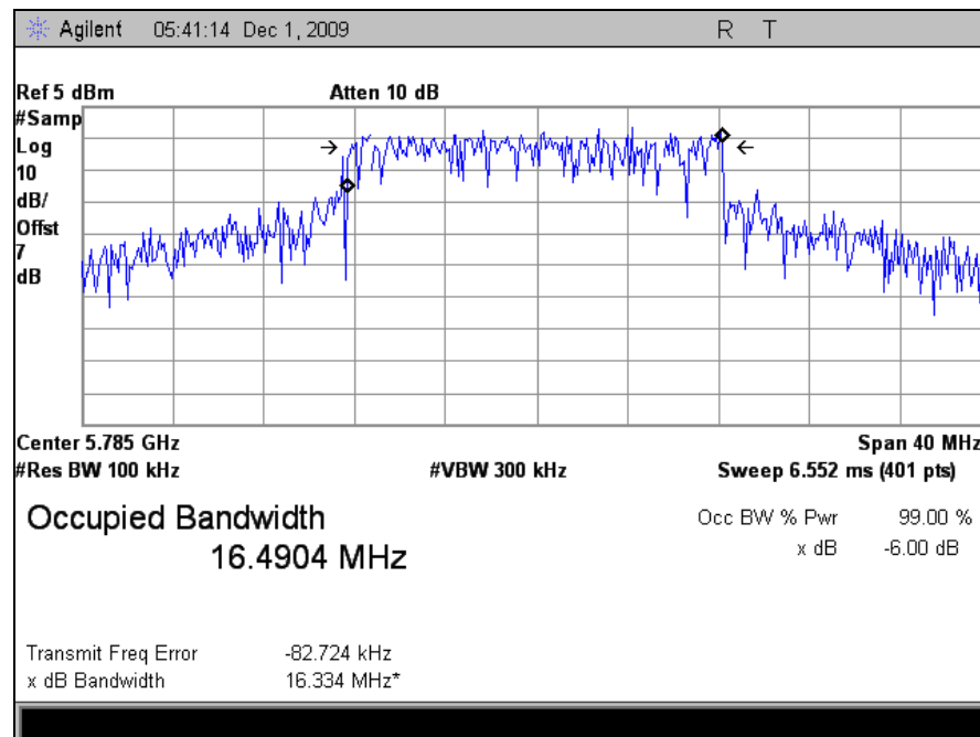
Plot 9. Occupied Bandwidth, Mid Channel (5785MHz), 802.11a, 6dB BW, M25 Radio
