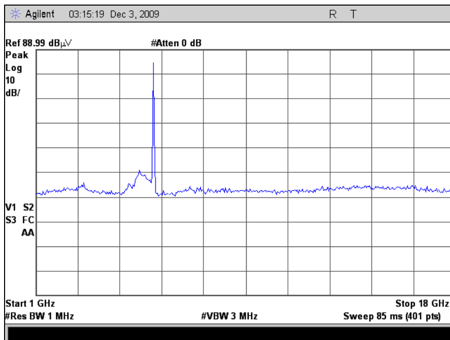
Plot 26. Radiated Spurious Emissions, Low Channel, 802.11a, 1 GHz – 18 GHz, M25 Radio
