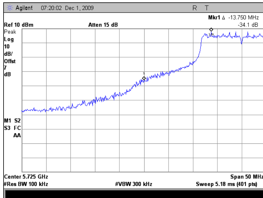
Plot 101. Conducted Band Edge, Low, M5 Radio
