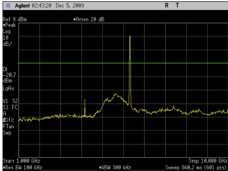
Plot 50. Conducted Emissions, Mid Channel, 1 GHz – 10 GHz, 802.11a, M25 Radio
