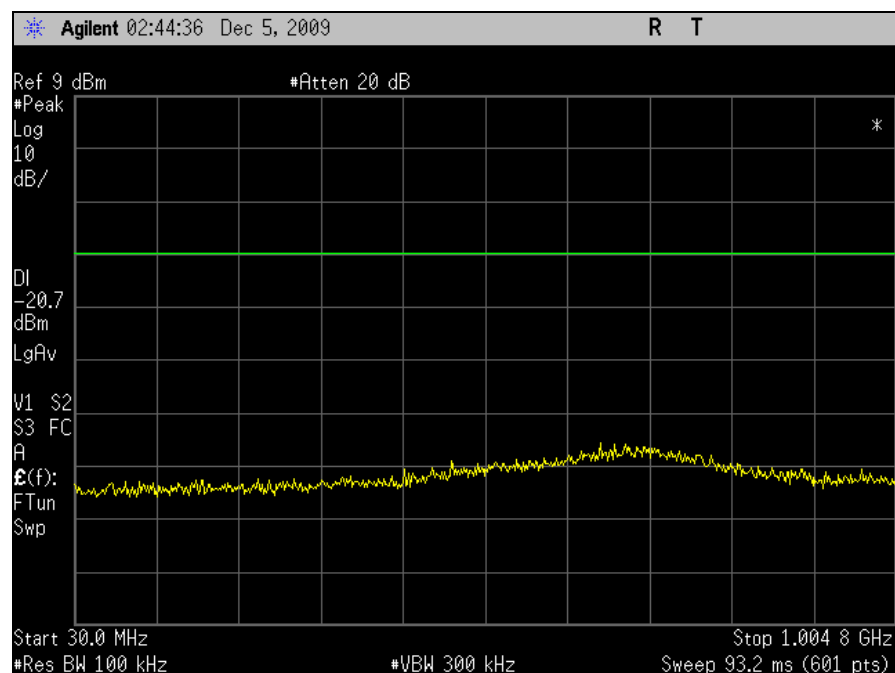
Plot 49. Conducted Emissions, Mid Channel, 30 MHz – 1 GHz, 802.11a, M25 Radio
