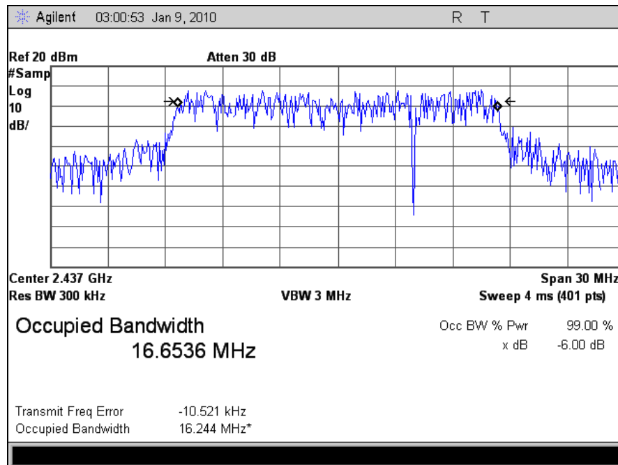
Plot 18. Occupied Bandwidth, Mid Channel (2437 MHz), 802.11g, 99% BW, M25 Radio
