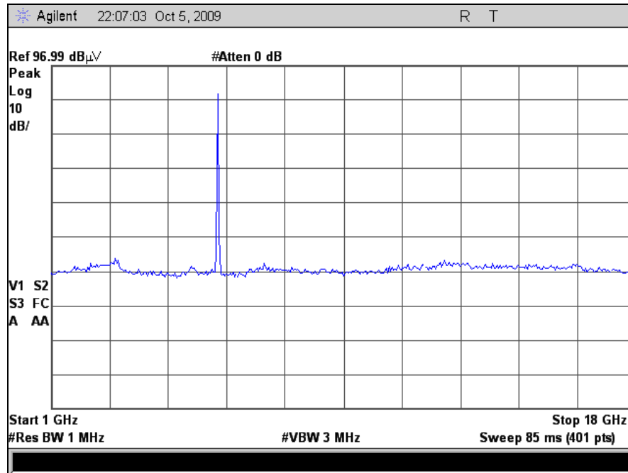
Plot 87. Radiated Spurious Emissions, High Channel, 802.11a, 1 GHz – 18 GHz, M5 Radio
