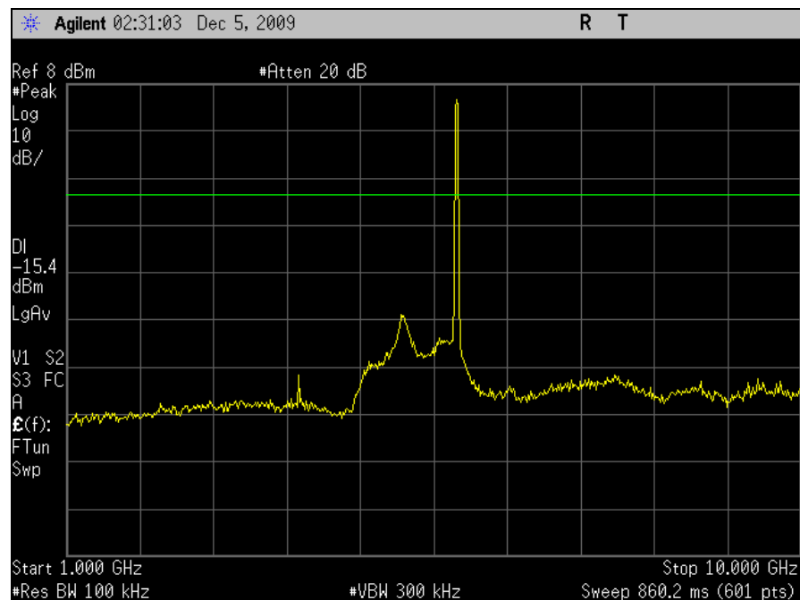
Plot 96. Conducted Emissions, Mid Channel, 1 GHz – 10 GHz, 802.11a, M5 Radio
