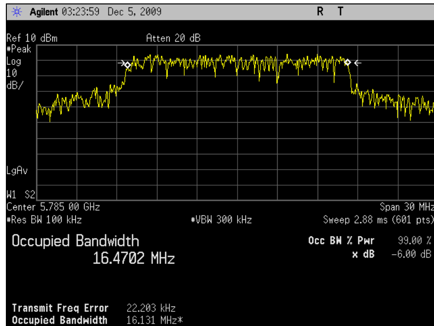
Plot 80. Occupied Bandwidth, Mid Channel (5785MHz), 6dB BW, M5 Radio
