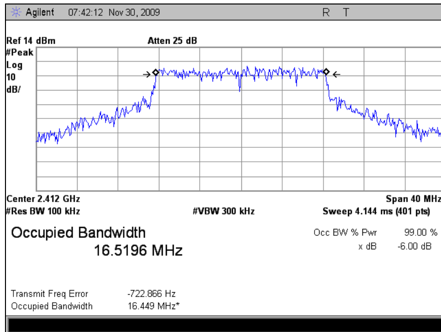
Plot 14. Occupied Bandwidth, Low Channel (2412MHz), 802.11g, 6dB BW, M25 Radio B
