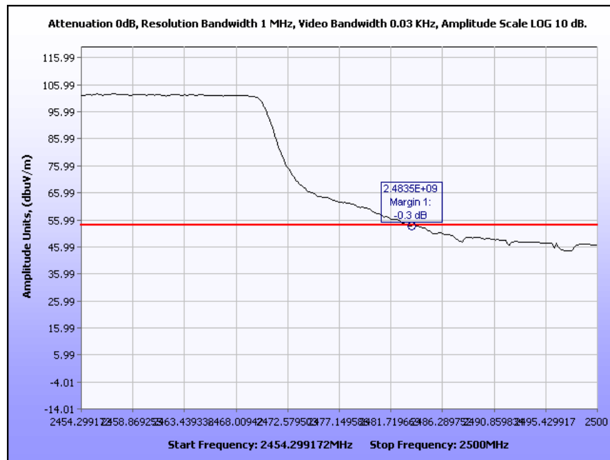
Plot 40. Upper Band Edge, Average, 802.11g, M25 Radio
