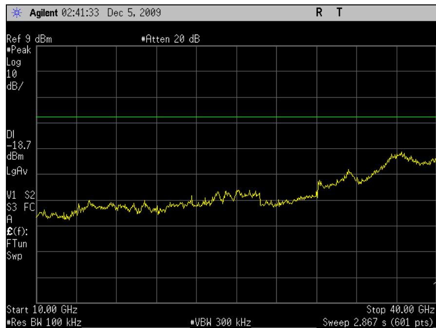
Plot 48. Conducted Emissions, Low Channel, 10 GHz – 40 GHz, 802.11a, M25 Radio
