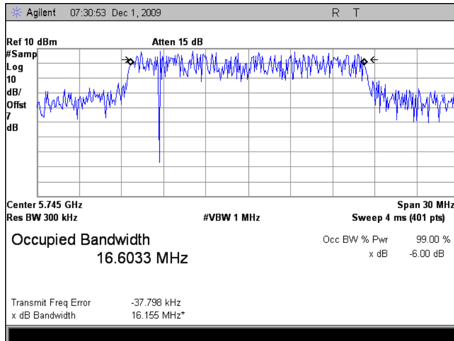
Plot 76. Occupied Bandwidth, Low Channel (5745MHz), 99% BW, M5 Radio
