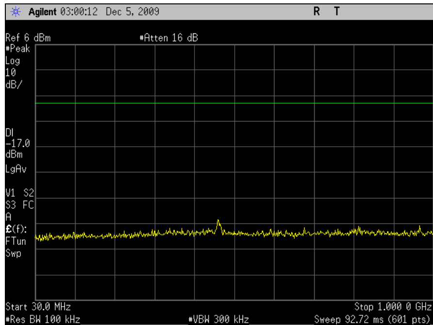
Plot 58. Conducted Emissions, Mid Channel, 30 MHz – 1 GHz, , 802.11g, M25 Radio
