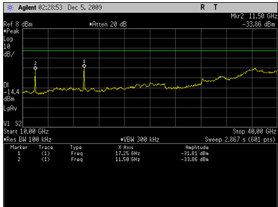
Plot 94. Conducted Emissions, Low Channel, 10 GHz – 40 GHz, 802.11a, M5 Radio
