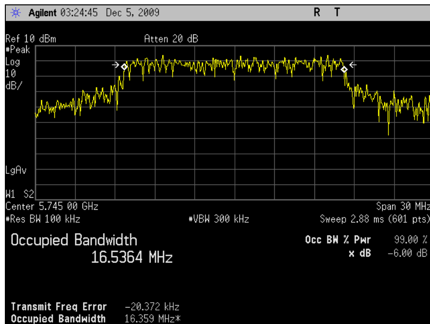
Plot 79. Occupied Bandwidth, Low Channel (5745MHz), 6dB BW, M5 Radio
