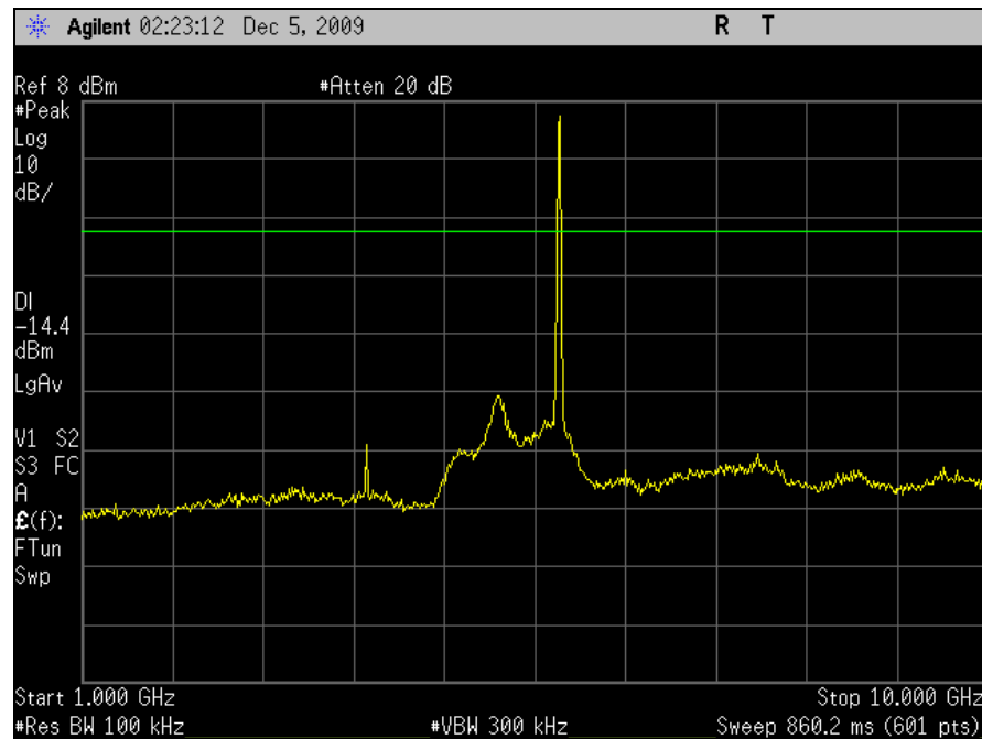
Plot 93. Conducted Emissions, Low Channel, 1 GHz – 10 GHz, 802.11a, M5 Radio
