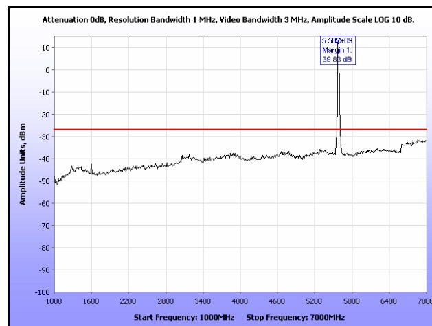
Plot 180. Radiated Spurious, 802.11a, 5580 MHz, 1 GHz – 7 GHz, Omni Antenna
