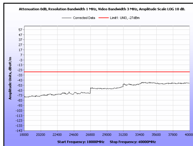
Plot 186. Radiated Spurious, 802.11a, 5700 MHz, 18 GHz – 40 GHz, Omni Antenna
