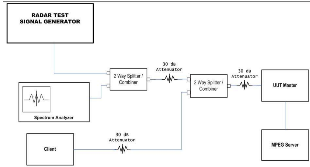
Figure 6. Test Setup Diagram
