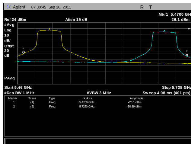
Plot 418. Frequency Stability, 802.11n 40 MHz, 5470 MHz – 5725 MHz @ 50°C, 120 V
