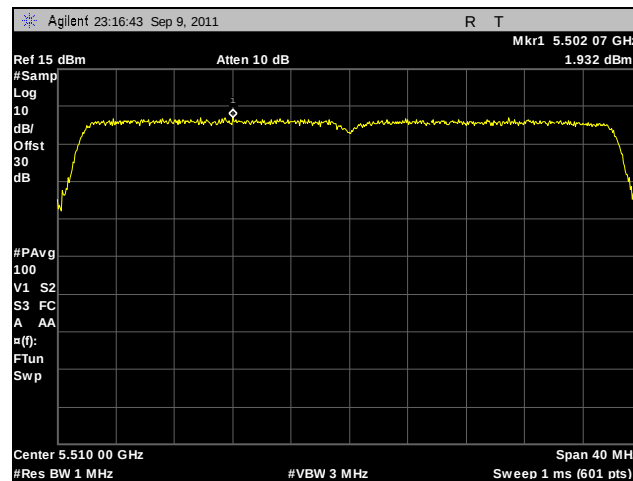
Plot 118. Peak Spectral Density, 802.11n 40 MHz, Port A, 5510 MHz
