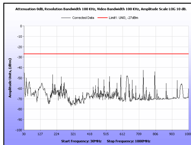
Plot 195. Radiated Spurious, 802.11n 20 MHz, 5320 MHz, 30 MHz – 1 GHz, Omni Antenna
