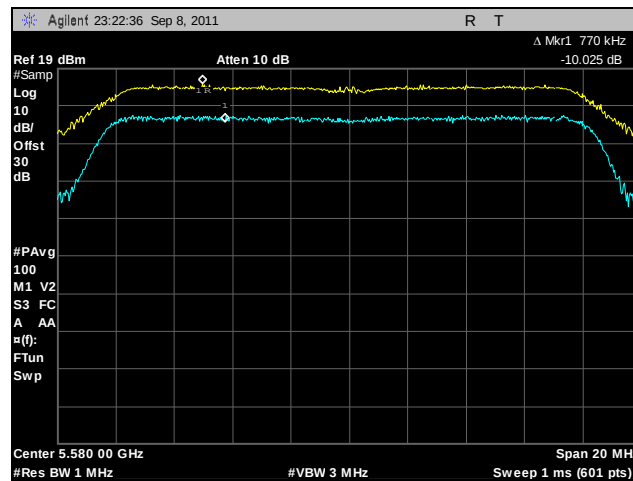
Plot 137. Peak Excursion, 802.11a, 5580 MHz
