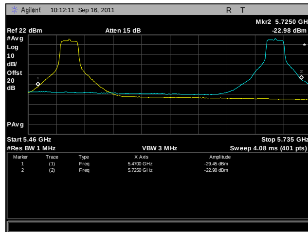
Plot 371. Frequency Stability, 802.11a, 5470 MHz – 5725 MHz @ 20°C, 132 V
