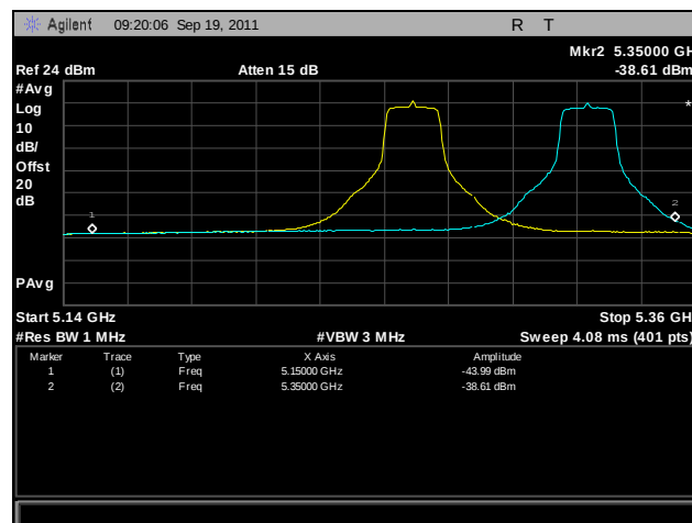
Plot 378. Frequency Stability, 802.11n 20 MHz, 5250 MHz – 5350 MHz @ 0°C, 120 V
