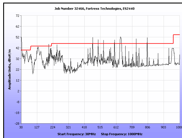
Plot 279. Radiated Spurious, 802.11n 20 MHz, 5700 MHz, 30 MHz – 1 GHz, Sector Antenna
