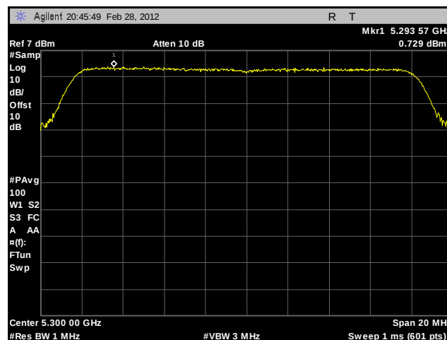
Plot 128. Peak Spectral Density, 802.11a, 5300 MHz, Sector Antenna
