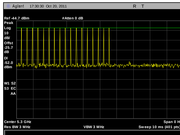
Plot 426. Radar Calibration, Bin 3
