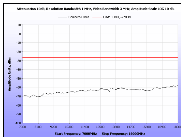
Plot 285. Radiated Spurious, 802.11n 40 MHz, 5270 MHz, 7 GHz – 18 GHz, Sector Antenna
