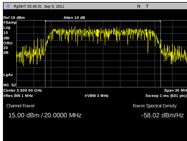
Plot 76. Conducted Output Power, 802.11n 20 MHz, Port A, 5500 MHz
