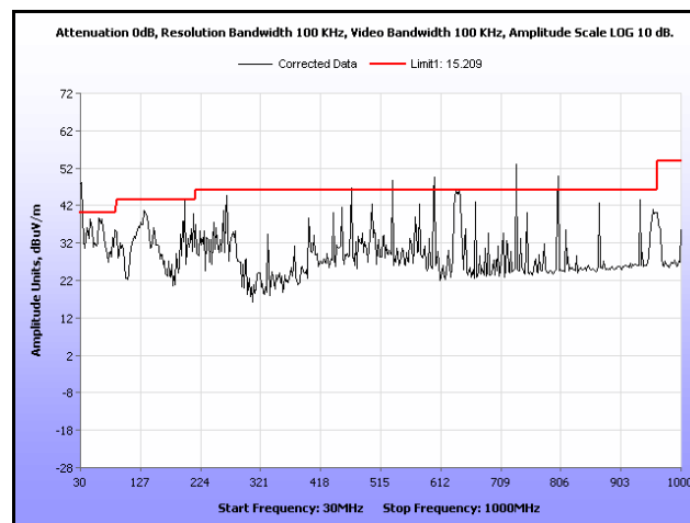
Plot 303. Radiated Spurious, 802.11n 40 MHz, 5690 MHz, 30 MHz – 1 GHz, Sector Antenna
