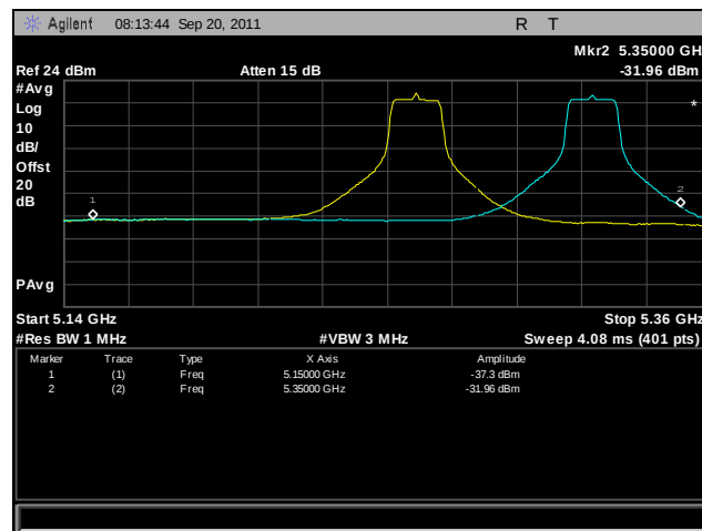
Plot 364. Frequency Stability, 802.11a, 5250 MHz – 5350 MHz @ 55°C, 120 V
