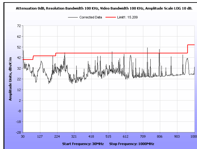
Plot 263. Radiated Spurious, 802.11n 20 MHz, 5300 MHz, 30 MHz – 1 GHz, Sector Antenna
