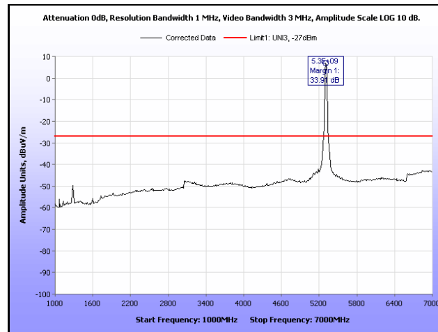
Plot 220. Radiated Spurious, 802.11n 40 MHz, 5310 MHz, 1 GHz – 7 GHz, Omni Antenna
