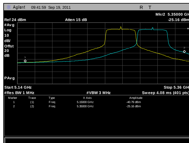
Plot 400. Frequency Stability, 802.11n 40 MHz, 5250 MHz – 5350 MHz @ 0°C, 120 V
