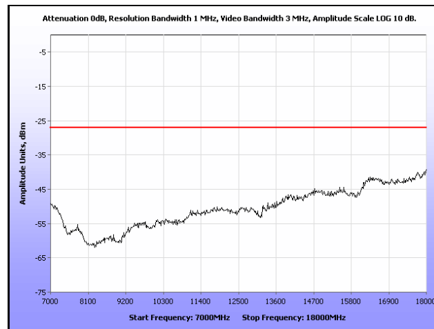
Plot 173. Radiated Spurious, 802.11a, 5320 MHz, 7 GHz – 18 GHz, Omni Antenna
