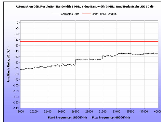
Plot 214. Radiated Spurious, 802.11n 40 MHz, 5270 MHz, 18 GHz – 40 GHz, Omni Antenna
