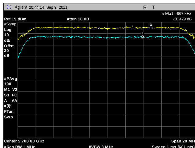
Plot 144. Peak Excursion, 802.11n 20 MHz, Port A, 5700 MHz
