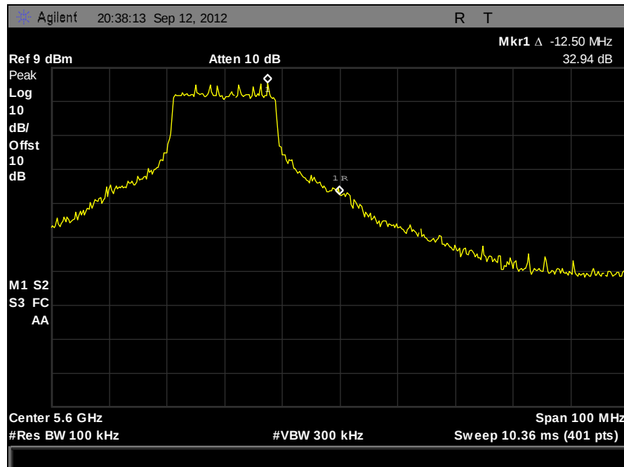
Plot 435. 20 dBc Notched Band, 802.11N 20 MHz, 5580 MHz, Port B
