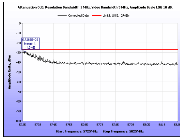
Plot 314. EIRP, 802.11n 20 MHz, 5700 MHz, Band Edge, Omni Antenna
