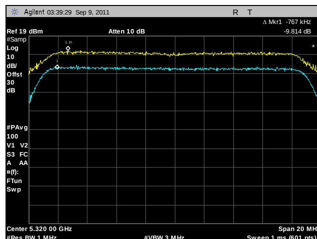
Plot 141. Peak Excursion, 802.11n 20 MHz, Port A, 5320 MHz
