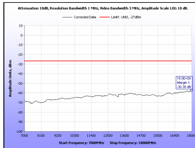
Plot 257. Radiated Spurious, 802.11a, 5700 MHz, 7 GHz – 18 GHz, Sector Antenna
