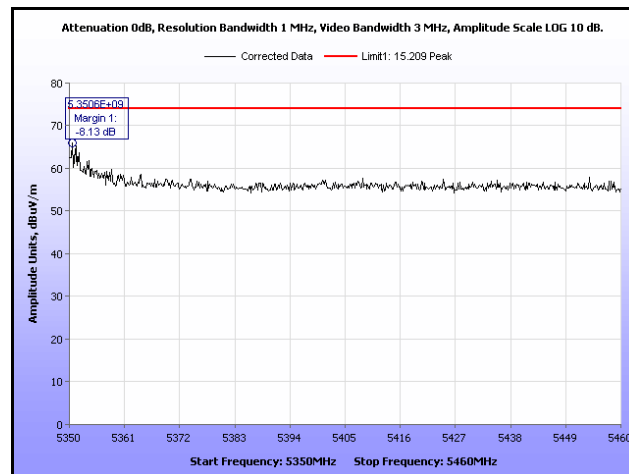
Plot 336. Restricted Band, 802.11n 20 MHz, 5320 MHz, Peak, Omni Antenna
