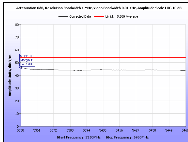
Plot 335. Restricted Band, 802.11n 20 MHz, 5320 MHz, Average, Omni Antenna
