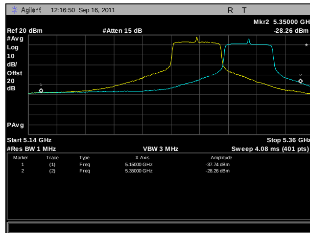
Plot 405. Frequency Stability, 802.11n 40 MHz, 5250 MHz – 5350 MHz @ 30°C, 120 V
