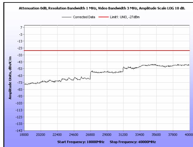
Plot 218. Radiated Spurious, 802.11n 40 MHz, 5300 MHz, 18 GHz – 40 GHz, Omni Antenna
