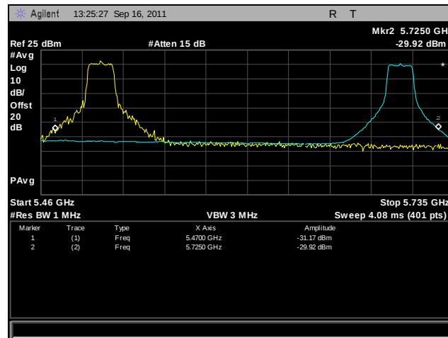
Plot 373. Frequency Stability, 802.11a, 5470 MHz – 5725 MHz @ 40°C, 120 V
