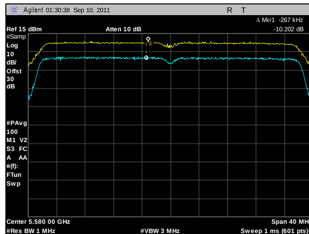
Plot 155. Peak Excursion, 802.11n 40 MHz, Port A, 5580 MHz
