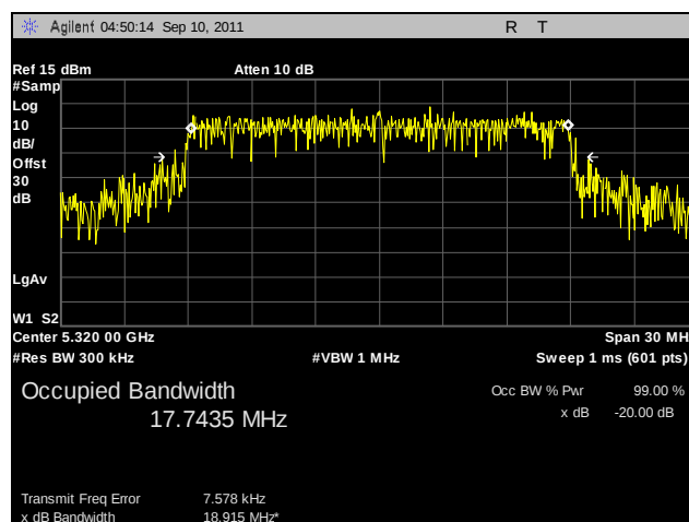
Plot 51. 99% Occupied Bandwidth, 802.11n 20 MHz, Port B, 5320 MHz
