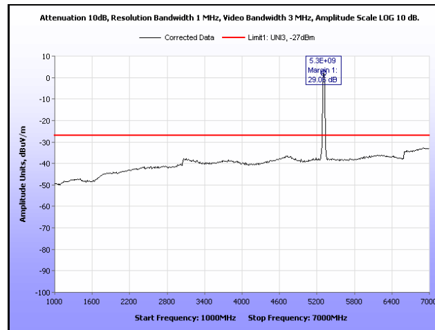
Plot 292. Radiated Spurious, 802.11n 40 MHz, 5310 MHz, 1 GHz – 7 GHz, Sector Antenna
