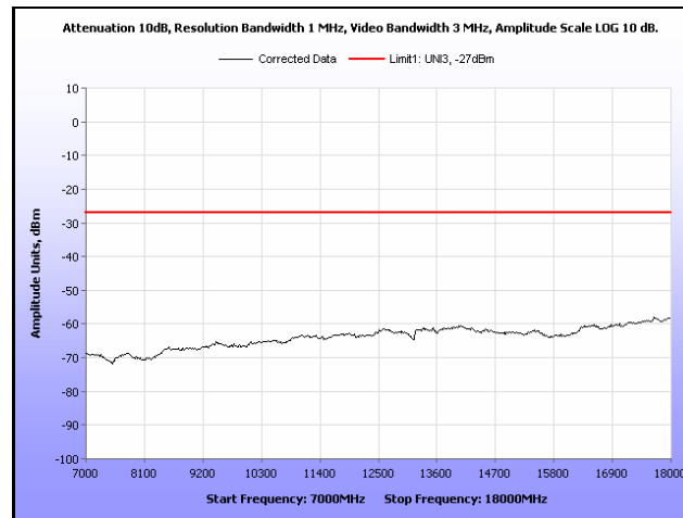
Plot 241. Radiated Spurious, 802.11a, 5300 MHz, 7 GHz – 18 GHz, Sector Antenna
