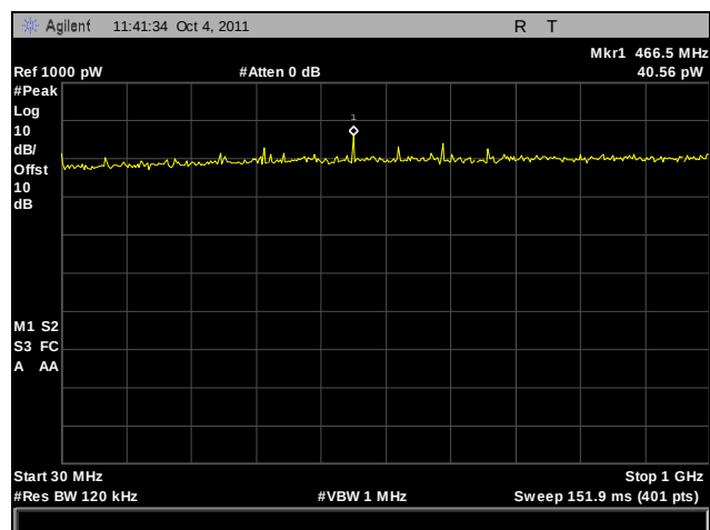
Plot 422. Receiver Spurious Emission, 5.8 GHz, 30 MHz – 1 GHz, Port B
