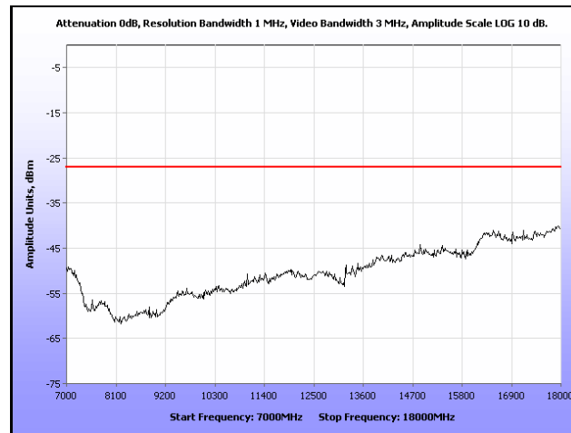
Plot 193. Radiated Spurious, 802.11n 20 MHz, 5300 MHz, 7 GHz – 18 GHz, Omni Antenna
