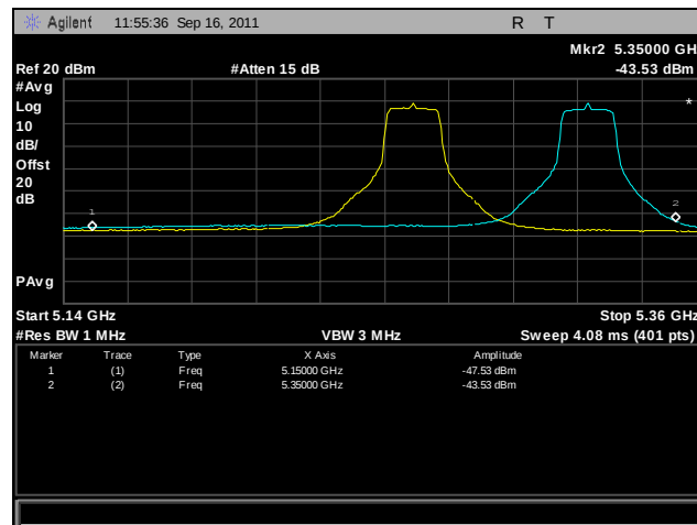
Plot 383. Frequency Stability, 802.11n 20 MHz, 5250 MHz – 5350 MHz @ 30°C, 120 V
