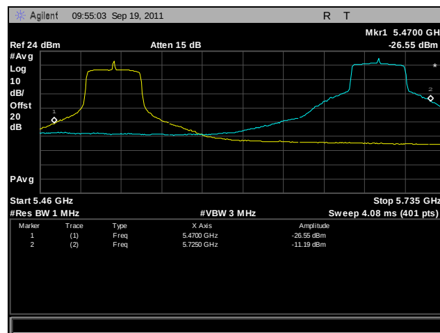
Plot 411. Frequency Stability, 802.11n 40 MHz, 5470 MHz – 5725 MHz @ 0°C, 120 V
