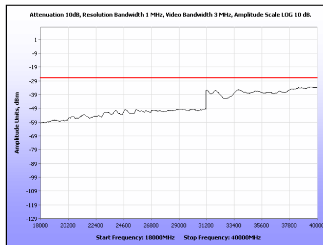
Plot 290. Radiated Spurious, 802.11n 40 MHz, 5300 MHz, 18 GHz – 40 GHz, Sector Antenna
