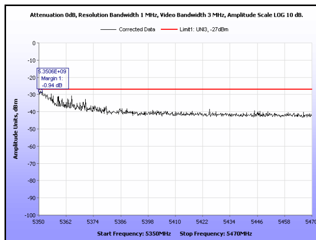
Plot 328. EIRP, 802.11n 40 MHz, 5310 MHz, Band Edge, Sector Antenna
