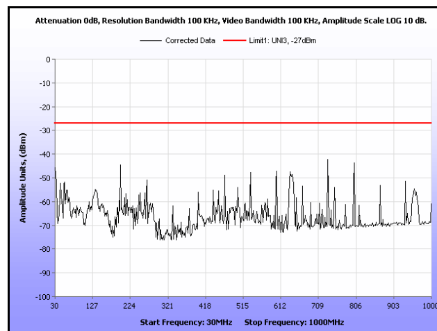
Plot 183. Radiated Spurious, 802.11a, 5700 MHz, 30 MHz – 1 GHz, Omni Antenna
