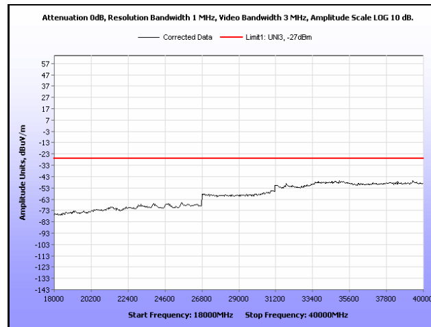
Plot 166. Radiated Spurious, 802.11a, 5260 MHz, 18 GHz – 40 GHz, Omni Antenna
