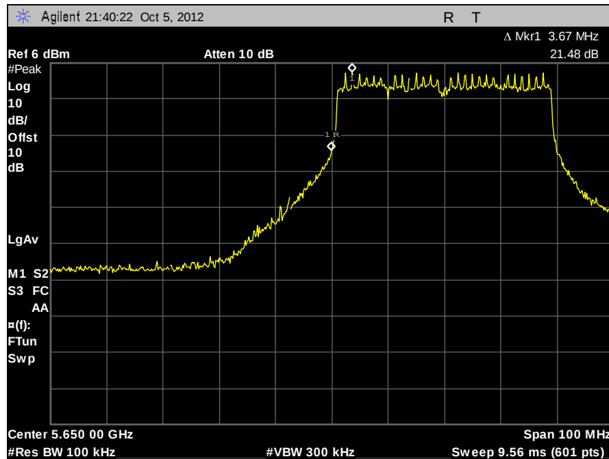
Plot 440. 20 dBc Notched Band, 802.11N 40 MHz, 5670 MHz, Port A
