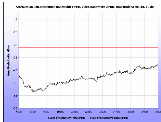
Plot 185. Radiated Spurious, 802.11a, 5700 MHz, 7 GHz – 18 GHz, Omni Antenna
