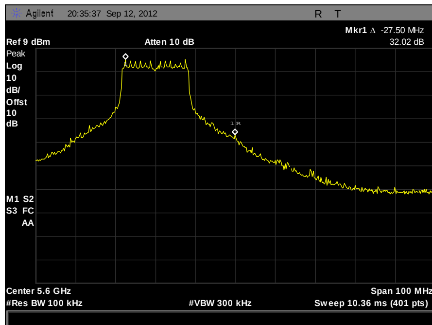
Plot 431. 20 dBc Notched Band, 802.11a, 5580 MHz, Port B
