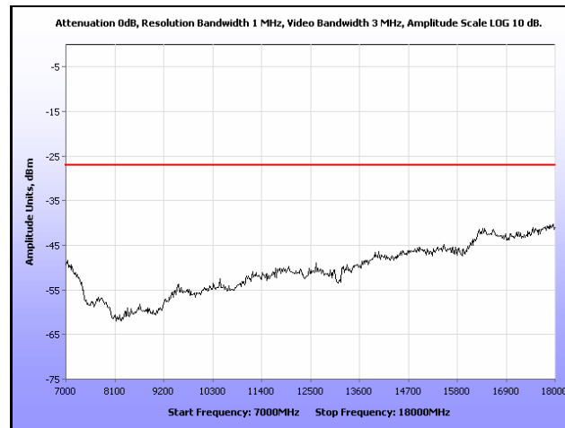
Plot 169. Radiated Spurious, 802.11a, 5300 MHz, 7 GHz – 18 GHz, Omni Antenna
