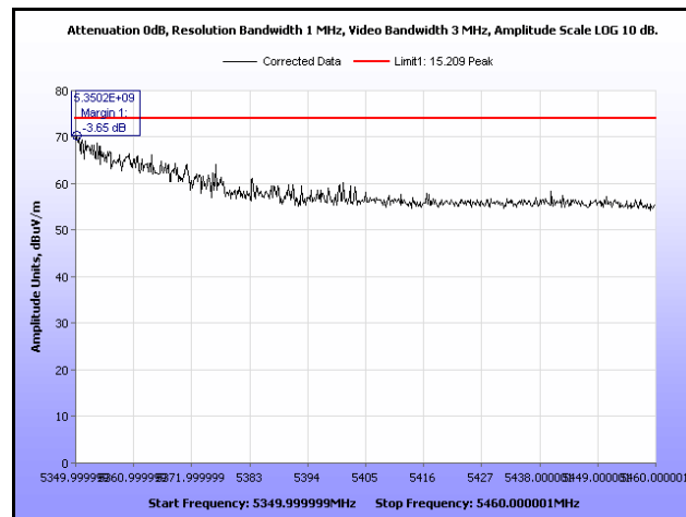
Plot 340. Restricted Band, 802.11n 40 MHz, 5310 MHz, Peak, Omni Antenna
