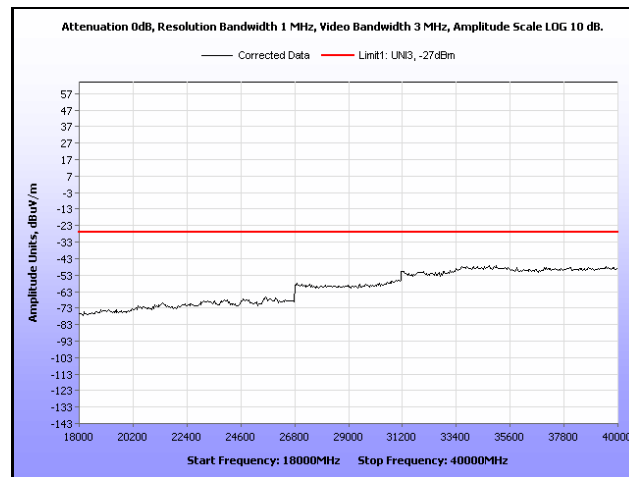
Plot 170. Radiated Spurious, 802.11a, 5300 MHz, 18 GHz – 40 GHz, Omni Antenna
