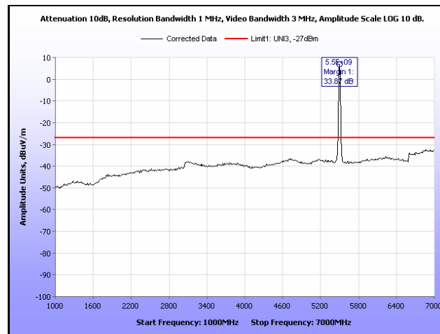
Plot 248. Radiated Spurious, 802.11a, 5500 MHz, 1 GHz – 7 GHz, Sector Antenna
