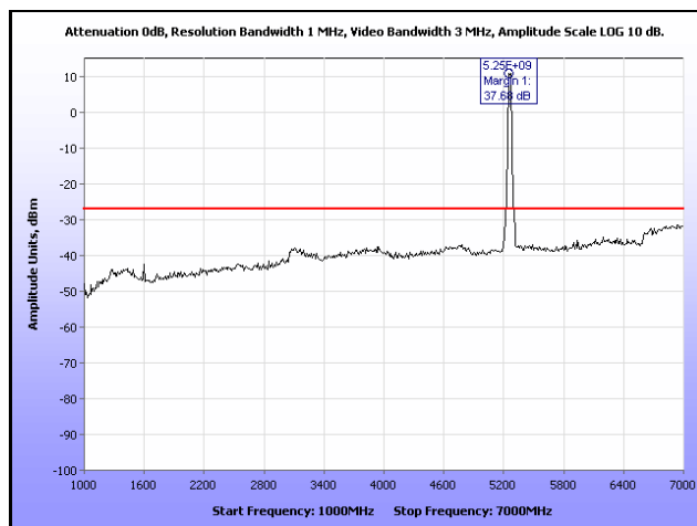
Plot 164. Radiated Spurious, 802.11a, 5260 MHz, 1 GHz – 7 GHz, Omni Antenna
