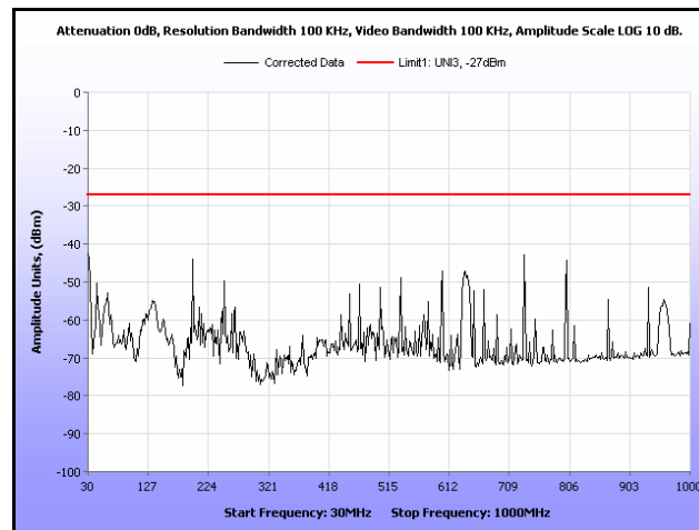
Plot 167. Radiated Spurious, 802.11a, 5300 MHz, 30 MHz – 1 GHz, Omni Antenna
