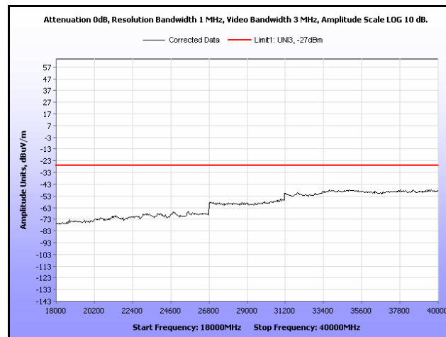
Plot 246. Radiated Spurious, 802.11a, 5320 MHz, 18 GHz – 40 GHz, Sector Antenna
