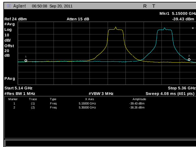
Plot 385. Frequency Stability, 802.11n 20 MHz, 5250 MHz – 5350 MHz @ 50°C, 120 V
