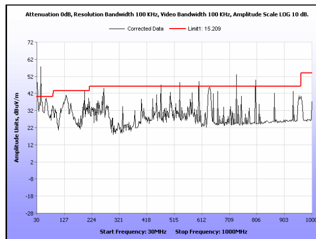
Plot 287. Radiated Spurious, 802.11n 40 MHz, 5300 MHz, 30 MHz – 1 GHz, Sector Antenna
