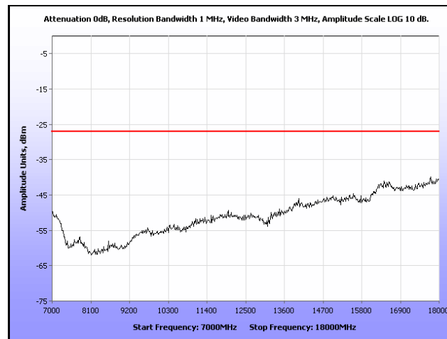
Plot 209. Radiated Spurious, 802.11n 20 MHz, 5700 MHz, 7 GHz – 18 GHz, Omni Antenna
