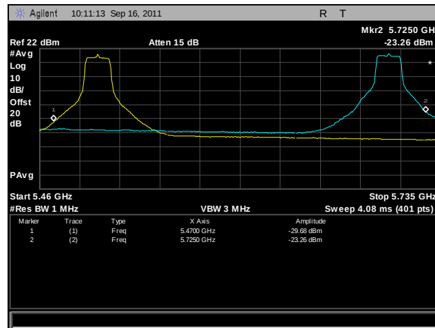
Plot 370. Frequency Stability, 802.11a, 5470 MHz – 5725 MHz @ 20°C, 120 V
