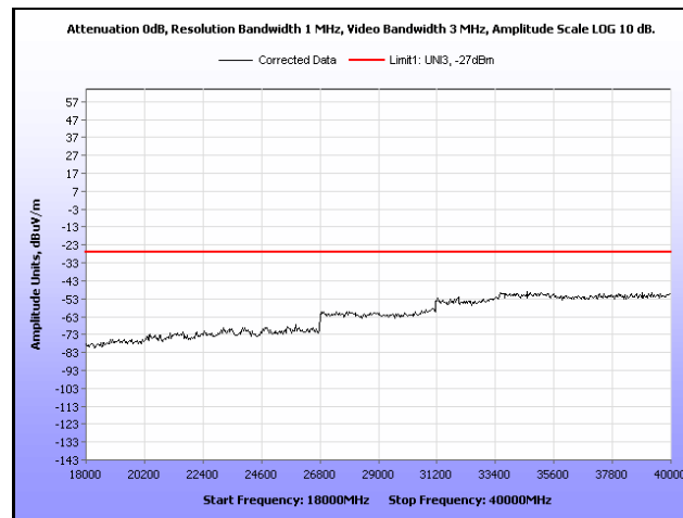
Plot 206. Radiated Spurious, 802.11n 20 MHz, 5580 MHz, 18 GHz – 40 GHz, Omni Antenna
