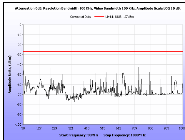
Plot 175. Radiated Spurious, 802.11a, 5500 MHz, 30 MHz – 1 GHz, Omni Antenna
