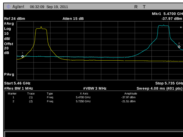
Plot 390. Frequency Stability, 802.11n 20 MHz, 5470 MHz – 5725 MHz @ 10°C, 120 V
