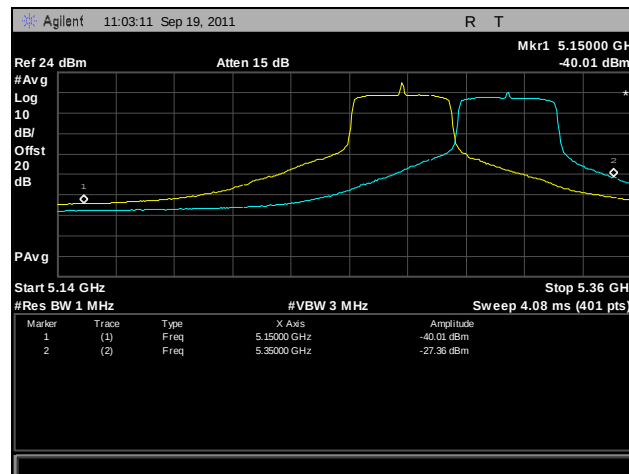
Plot 399. Frequency Stability, 802.11n 40 MHz, 5250 MHz – 5350 MHz @ -10°C, 120 V
