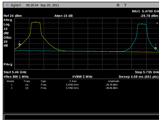
Plot 374. Frequency Stability, 802.11a, 5470 MHz – 5725 MHz @ 50°C, 120 V
