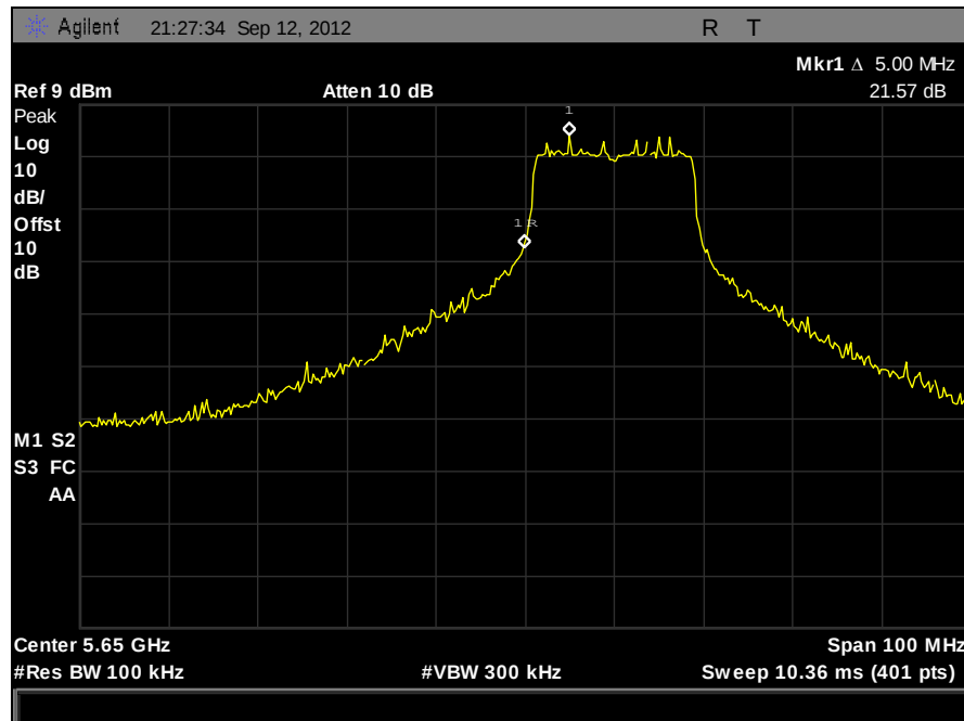
Plot 437. 20 dBc Notched Band, 802.11N 20 MHz, 5660 MHz, Port B
