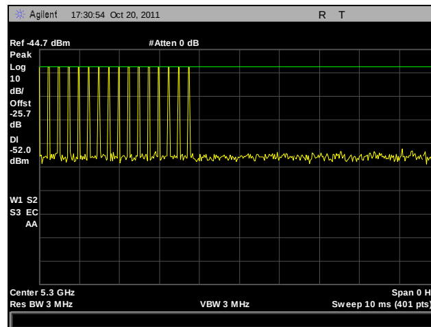
Plot 427. Radar Calibration, Bin 4
