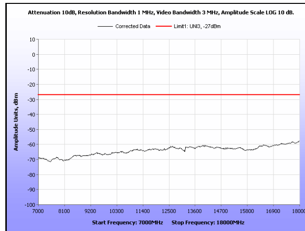
Plot 277. Radiated Spurious, 802.11n 20 MHz, 5580 MHz, 7 GHz – 18 GHz, Sector Antenna
