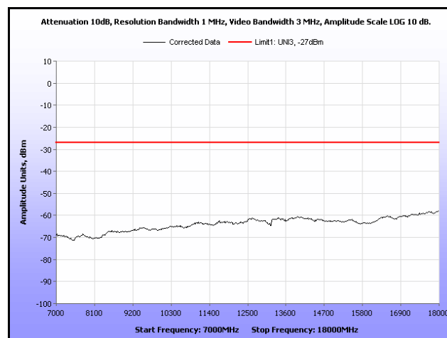
Plot 237. Radiated Spurious, 802.11a, 5260 MHz, 7 GHz – 18 GHz, Sector Antenna
