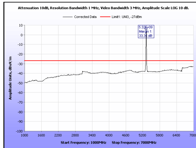
Plot 244. Radiated Spurious, 802.11a, 5320 MHz, 1 GHz – 7 GHz, Sector Antenna
