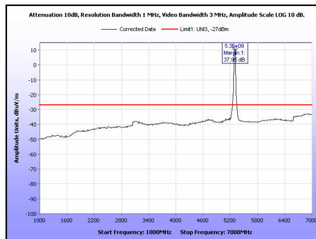
Plot 288. Radiated Spurious, 802.11n 40 MHz, 5300 MHz, 1 GHz – 7 GHz, Sector Antenna
