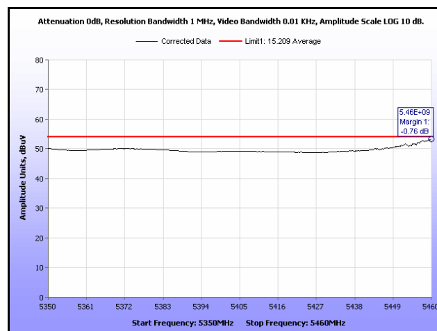
Plot 353. Restricted Band, 802.11n 40 MHz, 5510 MHz, Average, Sector Antenna
