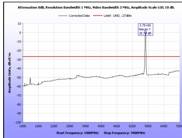
Plot 232. Radiated Spurious, 802.11n 40 MHz, 5690 MHz, 1 GHz – 7 GHz, Omni Antenna
