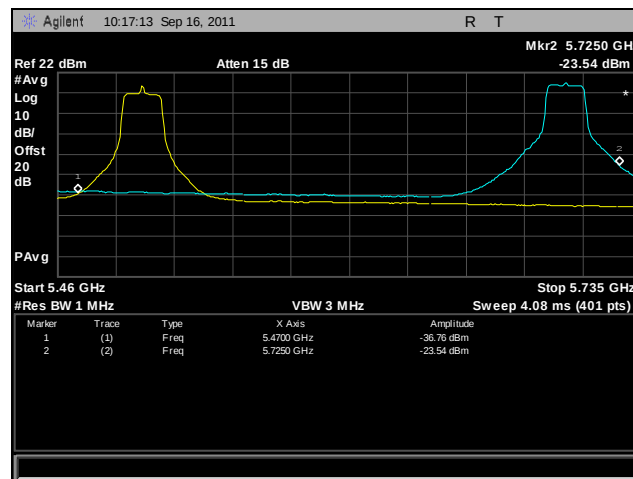
Plot 391. Frequency Stability, 802.11n 20 MHz, 5470 MHz – 5725 MHz @ 20°C, 108 V
