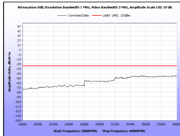
Plot 202. Radiated Spurious, 802.11n 20 MHz, 5500 MHz, 18 MHz – 40 GHz, Omni Antenna
