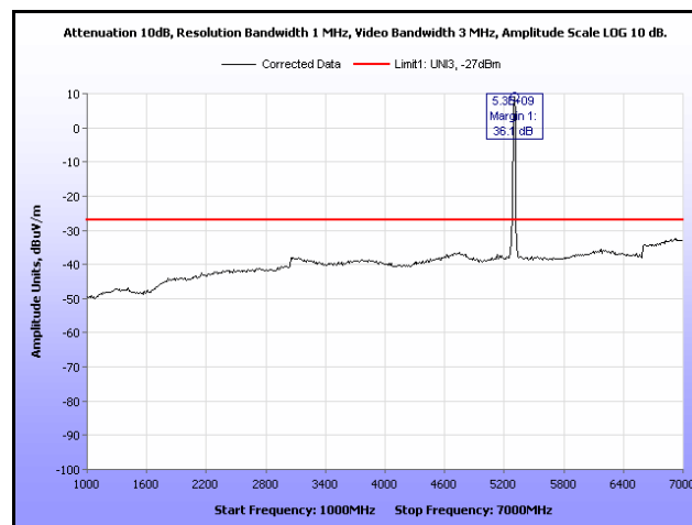
Plot 240. Radiated Spurious, 802.11a, 5300 MHz, 1 GHz – 7 GHz, Sector Antenna
