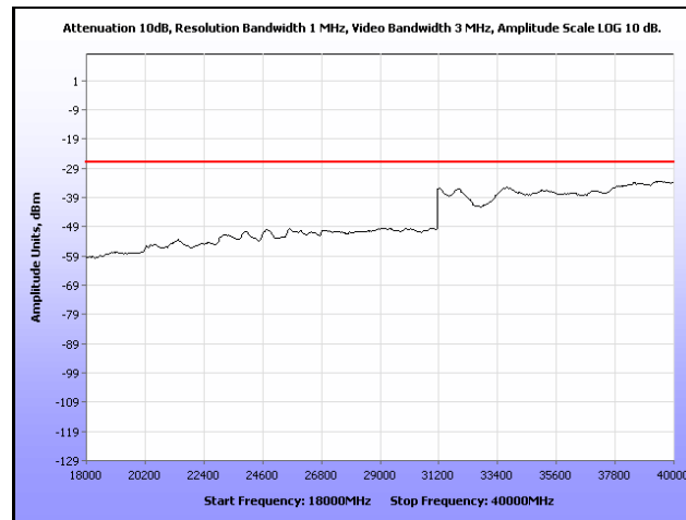
Plot 298. Radiated Spurious, 802.11n 40 MHz, 5510 MHz, 18 MHz – 40 GHz, Sector Antenna
