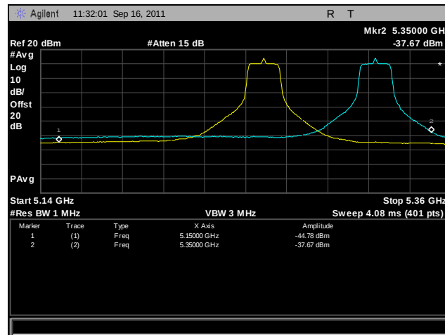
Plot 361. Frequency Stability, 802.11a, 5250 MHz – 5350 MHz @ 30°C, 120 V
