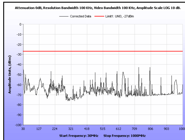
Plot 211. Radiated Spurious, 802.11n 40 MHz, 5270 MHz, 30 MHz – 1 GHz, Omni Antenna
