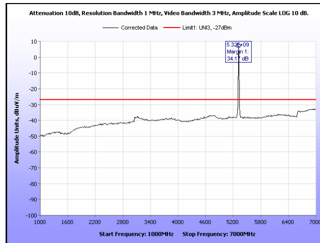
Plot 268. Radiated Spurious, 802.11n 20 MHz, 5320 MHz, 1 GHz – 7 GHz, Sector Antenna
