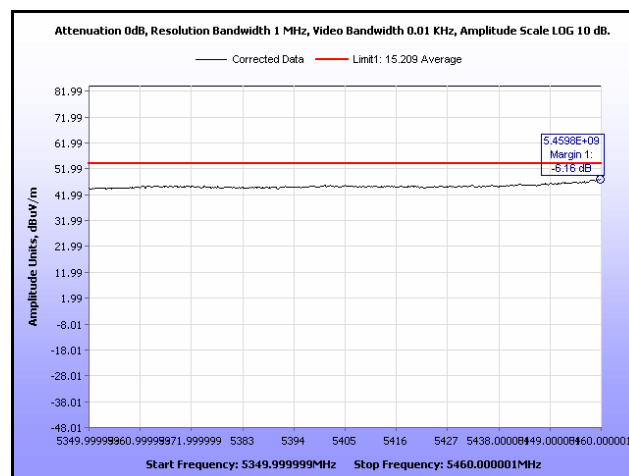
Plot 341. Restricted Band, 802.11n 40 MHz, 5510 MHz, Average, Omni Antenna
