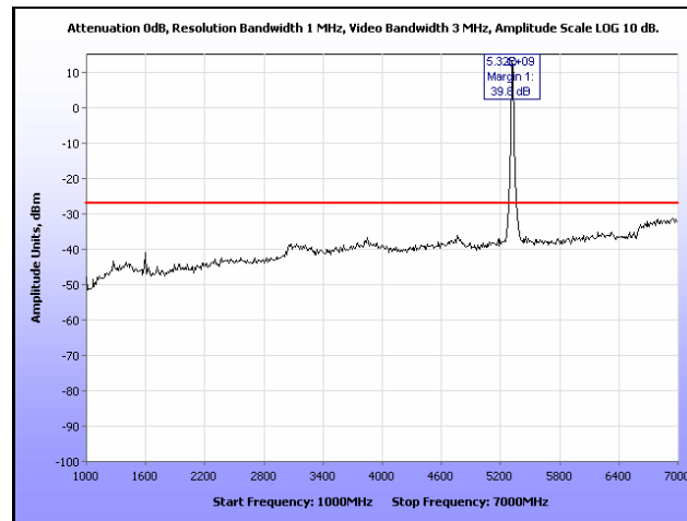
Plot 196. Radiated Spurious, 802.11n 20 MHz, 5320 MHz, 1 GHz – 7 GHz, Omni Antenna
