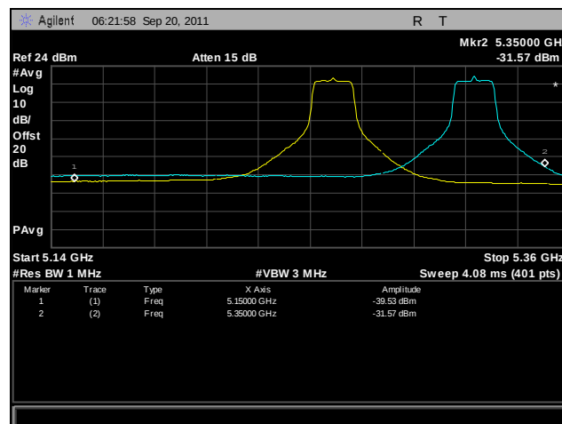
Plot 363. Frequency Stability, 802.11a, 5250 MHz – 5350 MHz @ 50°C, 120 V
