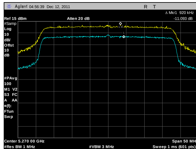
Plot 157. Peak Excursion, 802.11n 40 MHz, Port B, 5270 MHz
