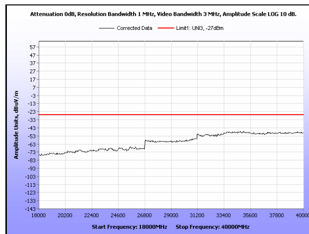
Plot 242. Radiated Spurious, 802.11a, 5300 MHz, 18 GHz – 40 GHz, Sector Antenna
