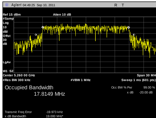
Plot 49. 99% Occupied Bandwidth, 802.11n 20 MHz, Port B, 5260 MHz
