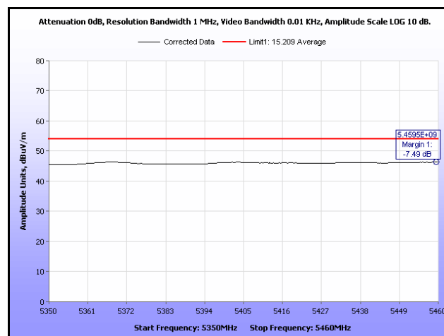
Plot 337. Restricted Band, 802.11n 20 MHz, 5500 MHz, Average, Omni Antenna
