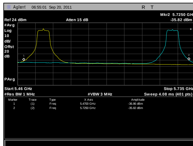
Plot 396. Frequency Stability, 802.11n 20 MHz, 5470 MHz – 5725 MHz @ 50°C, 120 V
