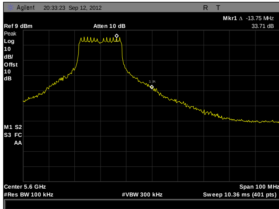
Plot 430. 20 dBc Notched Band, 802.11a, 5580 MHz, Port A
