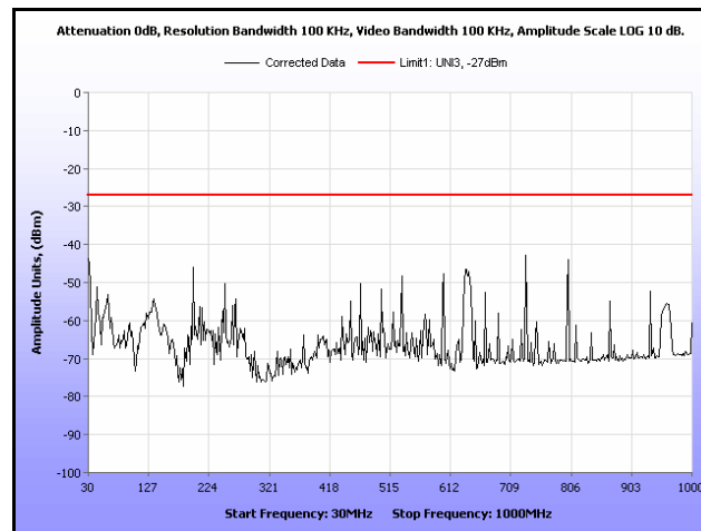
Plot 191. Radiated Spurious, 802.11n 20 MHz, 5300 MHz, 30 MHz – 1 GHz, Omni Antenna
