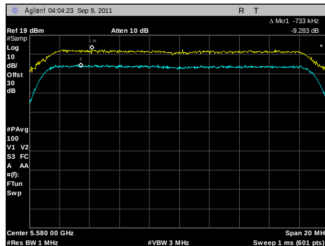
Plot 143. Peak Excursion, 802.11n 20 MHz, Port A, 5580 MHz
