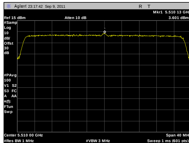
Plot 124. Peak Spectral Density, 802.11n 40 MHz, Port B, 5510 MHz
