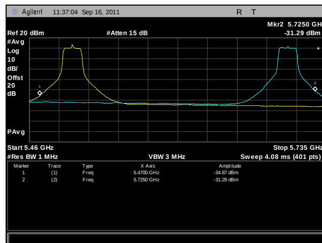
Plot 372. Frequency Stability, 802.11a, 5470 MHz – 5725 MHz @ 30°C, 120 V
