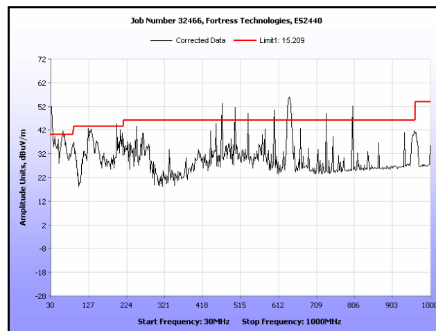
Plot 243. Radiated Spurious, 802.11a, 5320 MHz, 30 MHz – 1 GHz, Sector Antenna
