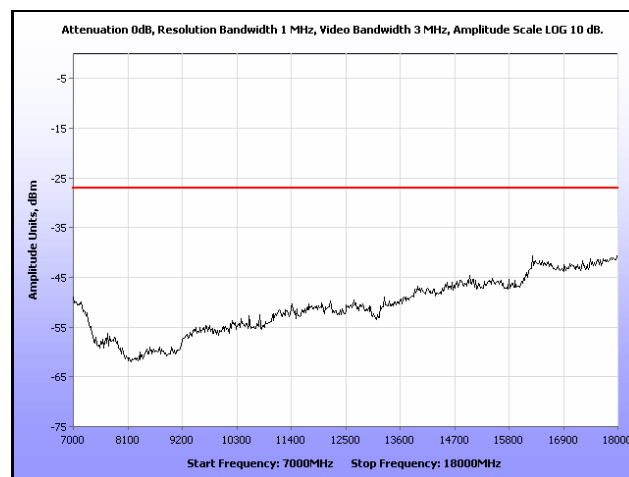
Plot 213. Radiated Spurious, 802.11n 40 MHz, 5270 MHz, 7 GHz – 18 GHz, Omni Antenna
