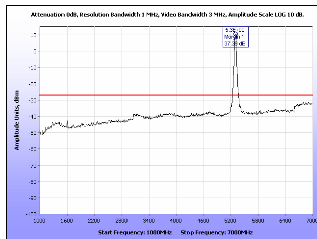
Plot 216. Radiated Spurious, 802.11n 40 MHz, 5300 MHz, 1 GHz – 7 GHz, Omni Antenna
