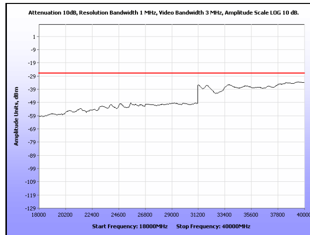
Plot 286. Radiated Spurious, 802.11n 40 MHz, 5270 MHz, 18 GHz – 40 GHz, Sector Antenna
