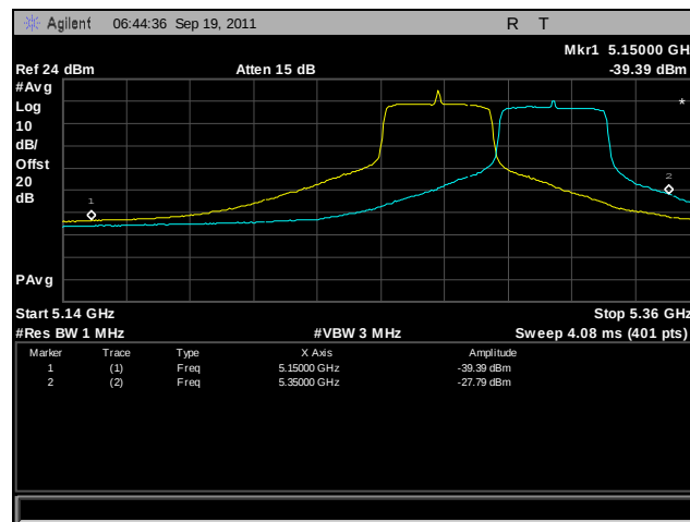
Plot 401. Frequency Stability, 802.11n 40 MHz, 5250 MHz – 5350 MHz @ 10°C, 120 V
