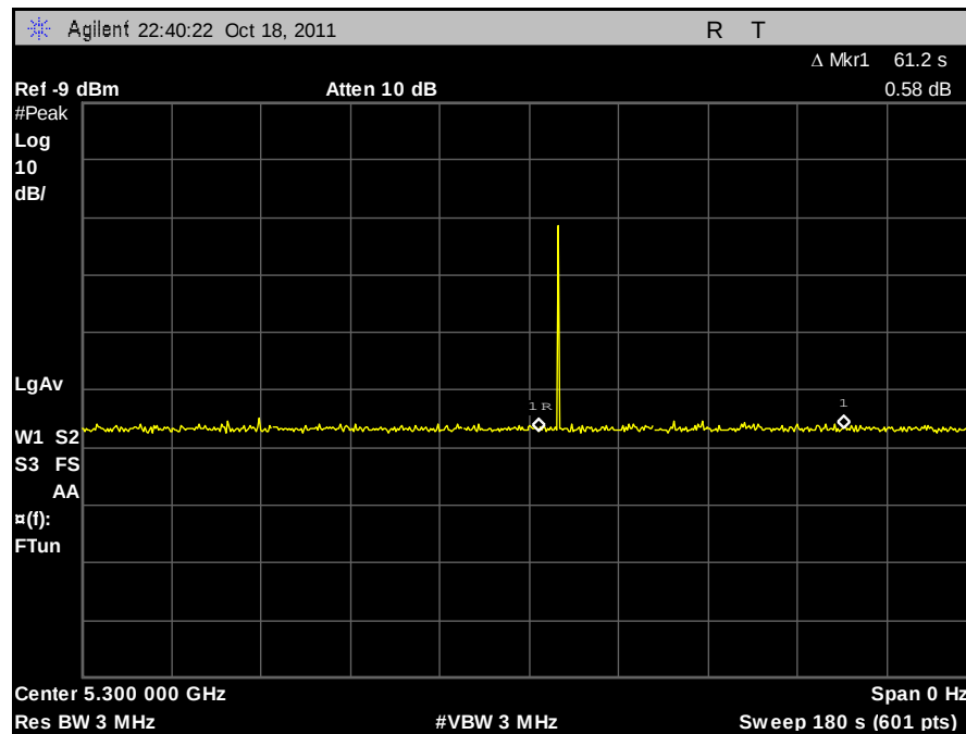
Plot 443. Radar Burst at the Beginning of CACT
