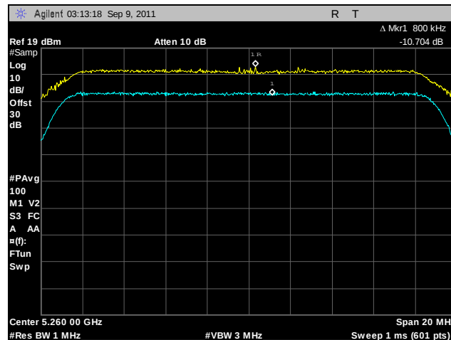
Plot 139. Peak Excursion, 802.11n 20 MHz, Port A, 5260 MHz
