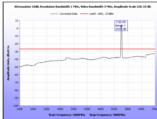
Plot 296. Radiated Spurious, 802.11n 40 MHz, 5510 MHz, 1 GHz – 7 GHz, Sector Antenna
