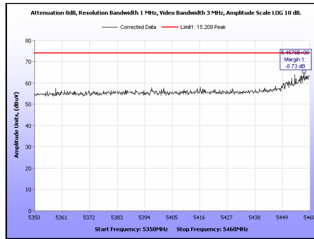
Plot 346. Restricted Band, 802.11a, 5500 MHz, Peak, Sector Antenna
