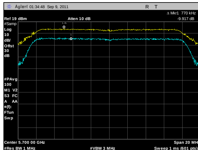
Plot 138. Peak Excursion, 802.11a, 5700 MHz
