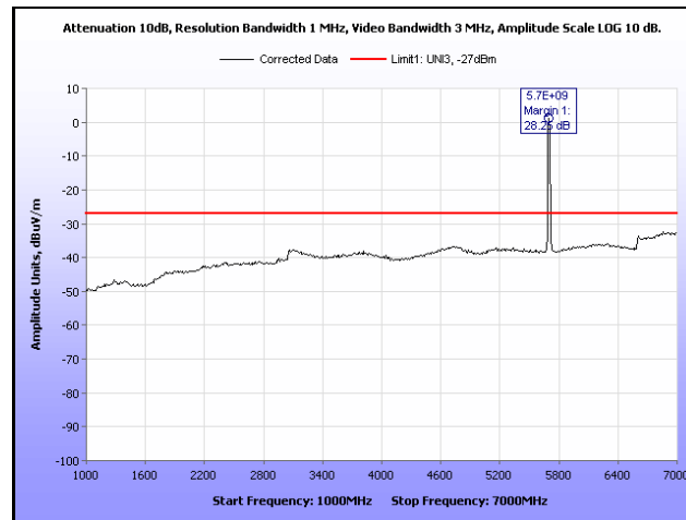
Plot 256. Radiated Spurious, 802.11a, 5700 MHz, 1 GHz – 7 GHz, Sector Antenna
