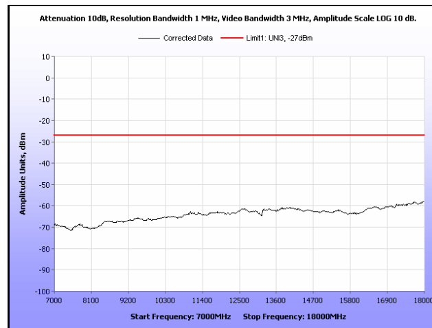
Plot 305. Radiated Spurious, 802.11n 40 MHz, 5690 MHz, 7 GHz – 18 GHz, Sector Antenna
