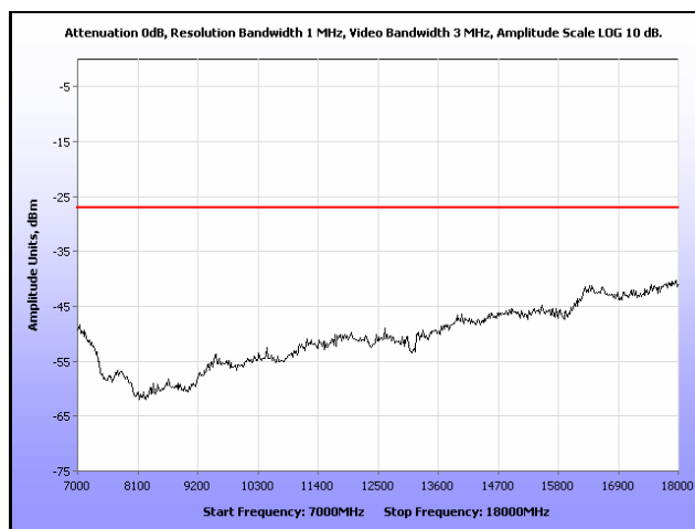
Plot 165. Radiated Spurious, 802.11a, 5260 MHz, 7 GHz – 18 GHz, Omni Antenna
