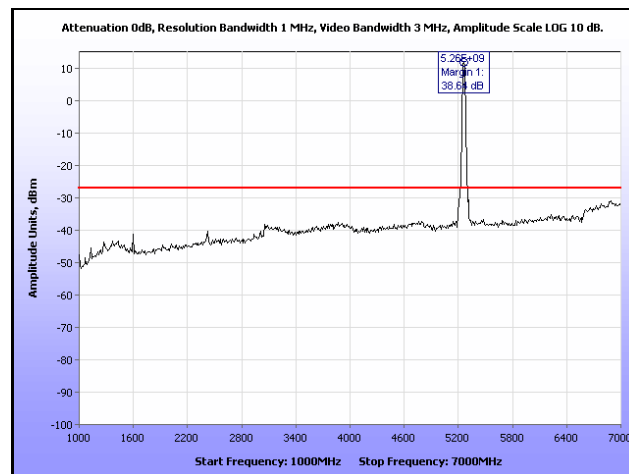
Plot 188. Radiated Spurious, 802.11n 20 MHz, 5260 MHz, 1 GHz – 7 GHz, Omni Antenna
