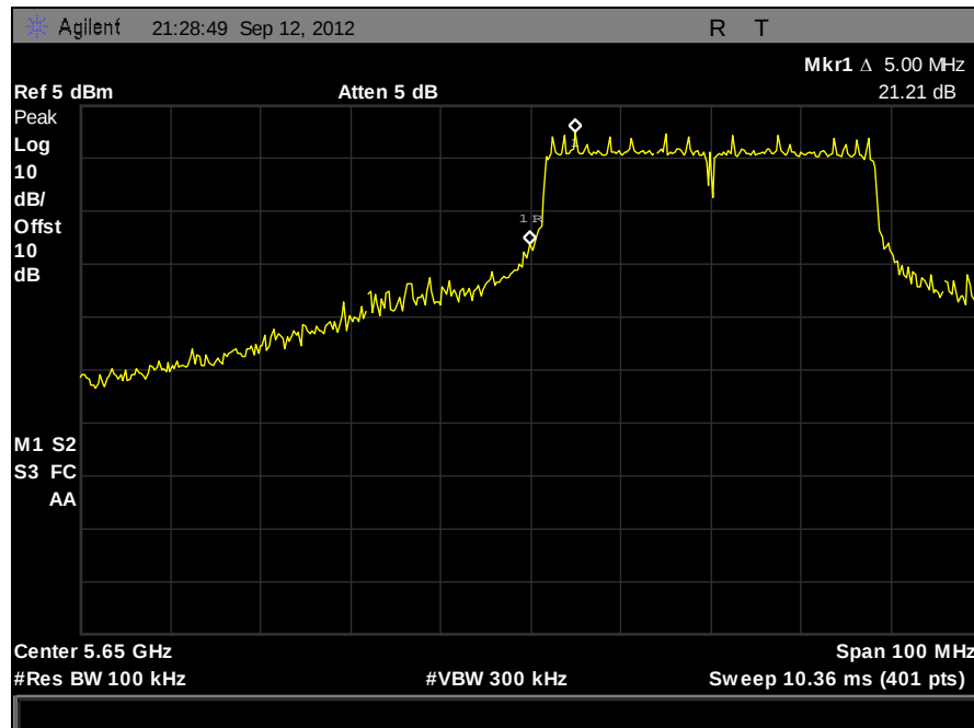
Plot 441. 20 dBc Notched Band, 802.11N 40 MHz, 5670 MHz, Port B
