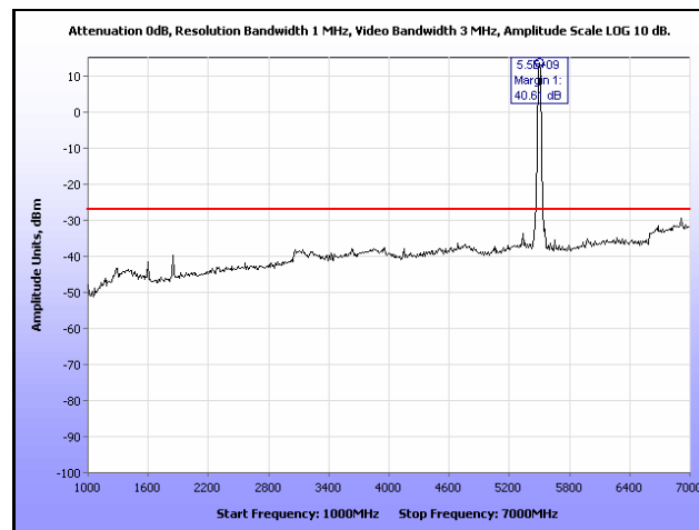
Plot 176. Radiated Spurious, 802.11a, 5500 MHz, 1 GHz – 7 GHz, Omni Antenna
