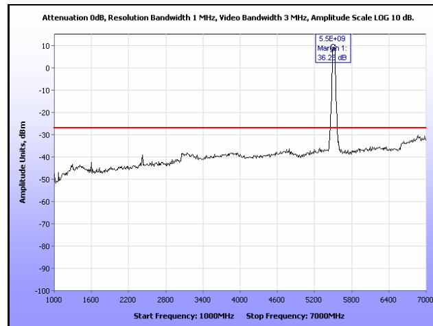
Plot 224. Radiated Spurious, 802.11n 40 MHz, 5510 MHz, 1 GHz – 7 GHz, Omni Antenna
