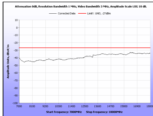
Plot 221. Radiated Spurious, 802.11n 40 MHz, 5310 MHz, 7 GHz – 18 GHz, Omni Antenna
