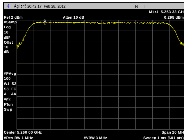
Plot 127. Peak Spectral Density, 802.11a, 5260 MHz, Sector Antenna
