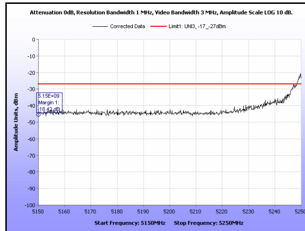
Plot 307. EIRP, 802.11a, 5260 MHz, Band Edge, Omni Antenna
