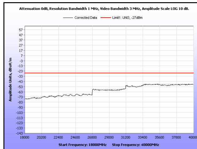
Plot 210. Radiated Spurious, 802.11n 20 MHz, 5700 MHz, 18 GHz – 40 GHz, Omni Antenna
