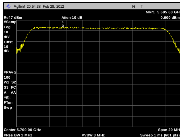
Plot 132. Peak Spectral Density, 802.11a, 5700 MHz, Sector Antenna
