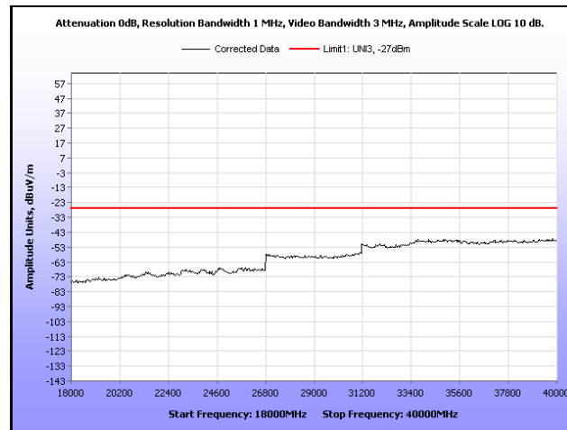
Plot 190. Radiated Spurious, 802.11n 20 MHz, 5260 MHz, 18 GHz – 40 GHz, Omni Antenna
