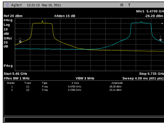
Plot 416. Frequency Stability, 802.11n 40 MHz, 5470 MHz – 5725 MHz @ 30°C, 120 V
