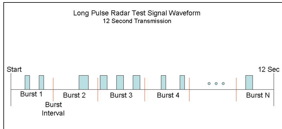
Figure 4. Long Pulse Radar Test Signal Waveform
