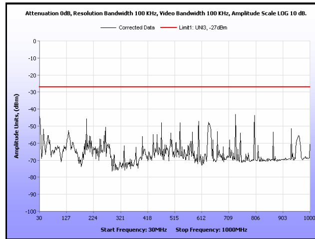
Plot 223. Radiated Spurious, 802.11n 40 MHz, 5510 MHz, 30 MHz – 1 GHz, Omni Antenna
