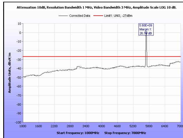
Plot 304. Radiated Spurious, 802.11n 40 MHz, 5690 MHz, 1 GHz – 7 GHz, Sector Antenna
