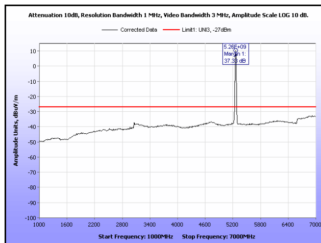
Plot 260. Radiated Spurious, 802.11n 20 MHz, 5260 MHz, 1 GHz – 7 GHz, Sector Antenna
