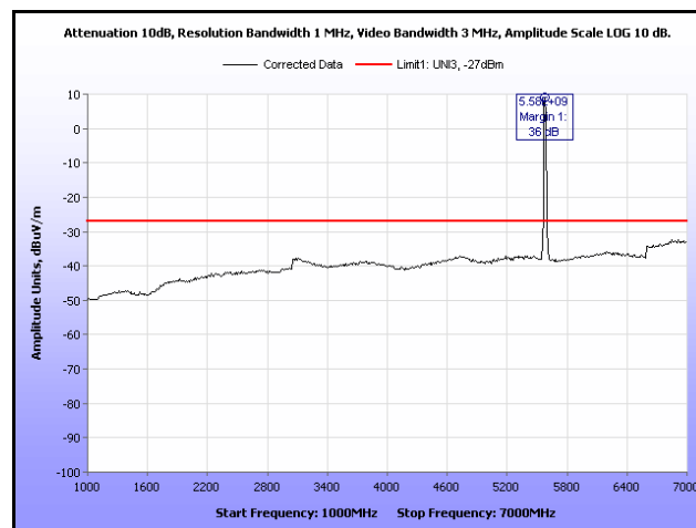
Plot 276. Radiated Spurious, 802.11n 20 MHz, 5580 MHz, 1 GHz – 7 GHz, Sector Antenna
