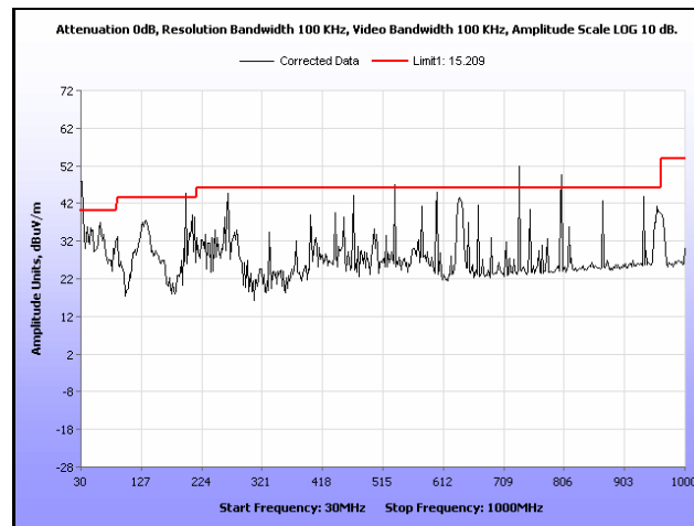
Plot 239. Radiated Spurious, 802.11a, 5300 MHz, 30 MHz – 1 GHz, Sector Antenna
