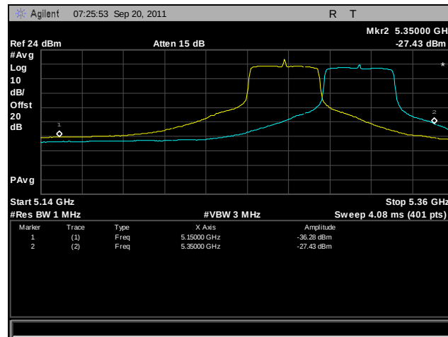
Plot 407. Frequency Stability, 802.11n 40 MHz, 5250 MHz – 5350 MHz @ 50°C, 120 V
