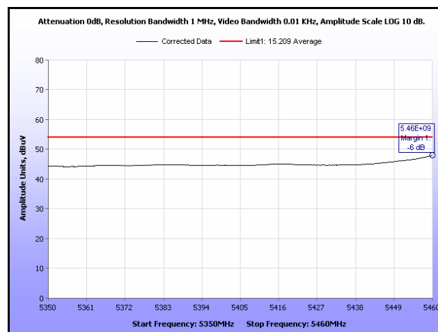
Plot 345. Restricted Band, 802.11a, 5500 MHz, Average, Sector Antenna
