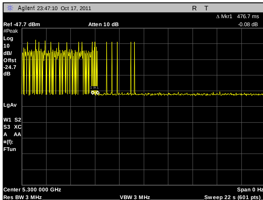
Plot 446. Channel Move Time, Bin 5
