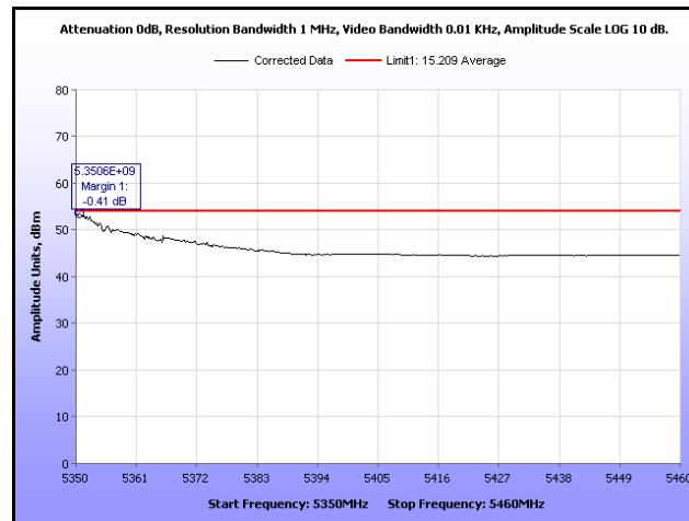
Plot 351. Restricted Band, 802.11n 40 MHz, 5310 MHz, Average, Sector Antenna
