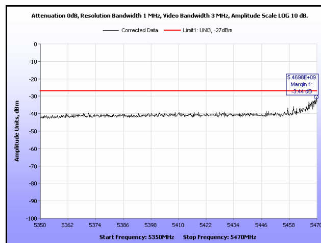
Plot 313. EIRP, 802.11n 20 MHz, 5500 MHz, Band Edge, Omni Antenna
