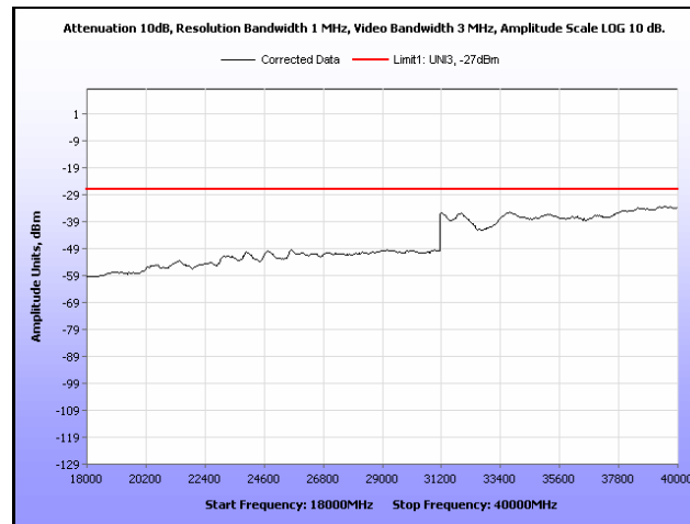
Plot 262. Radiated Spurious, 802.11n 20 MHz, 5260 MHz, 18 GHz – 40 GHz, Sector Antenna
