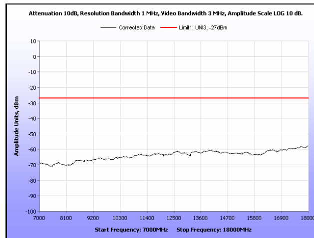
Plot 269. Radiated Spurious, 802.11n 20 MHz, 5320 MHz, 7 GHz – 18 GHz, Sector Antenna
