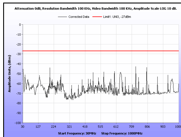
Plot 219. Radiated Spurious, 802.11n 40 MHz, 5310 MHz, 30 MHz – 1 GHz, Omni Antenna
