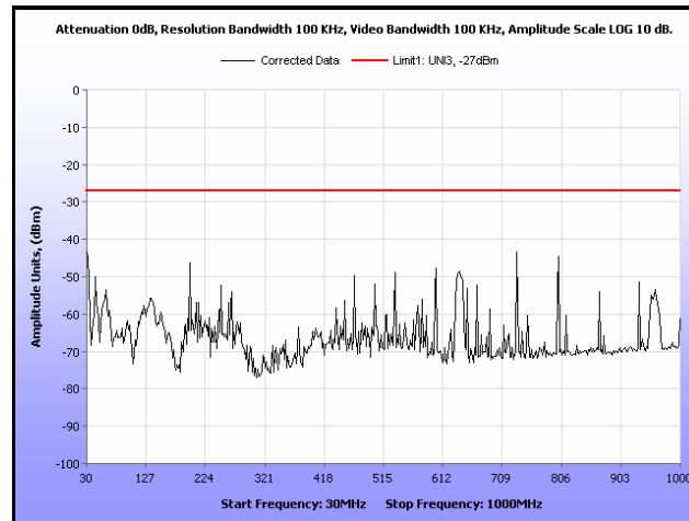
Plot 187. Radiated Spurious, 802.11n 20 MHz, 5260 MHz, 30 MHz – 1 GHz, Omni Antenna
