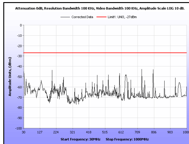
Plot 179. Radiated Spurious, 802.11a, 5580 MHz, 30 MHz – 1 GHz, Omni Antenna
