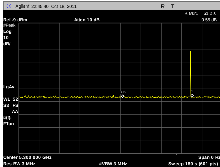
Plot 444. Radar Burst at the End of CACT
