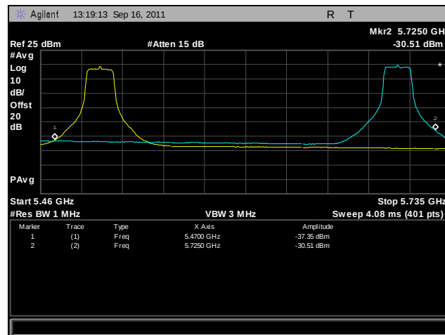
Plot 395. Frequency Stability, 802.11n 20 MHz, 5470 MHz – 5725 MHz @ 40°C, 120 V
