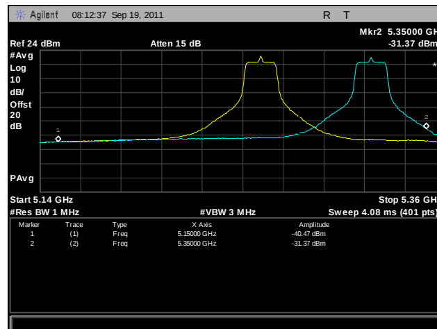
Plot 356. Frequency Stability, 802.11a, 5250 MHz – 5350 MHz @ 0°C, 120 V
