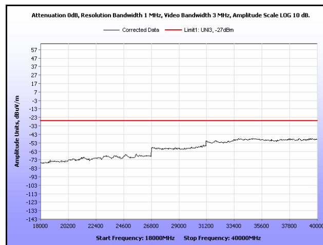
Plot 174. Radiated Spurious, 802.11a, 5320 MHz, 18 GHz – 40 GHz, Omni Antenna
