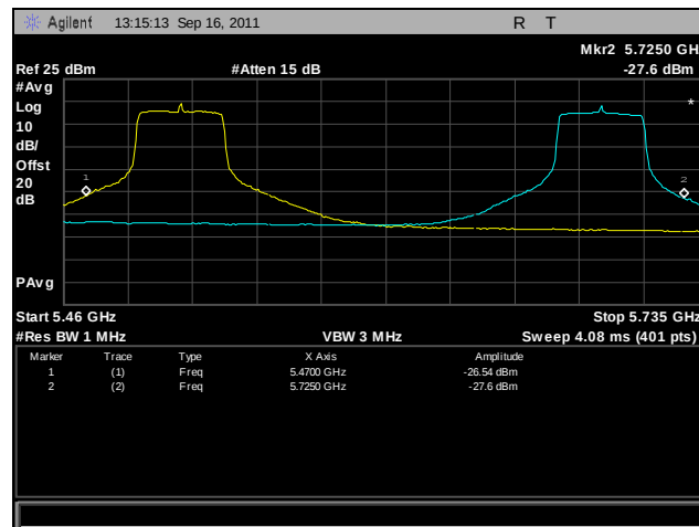
Plot 417. Frequency Stability, 802.11n 40 MHz, 5470 MHz – 5725 MHz @ 40°C, 120 V
