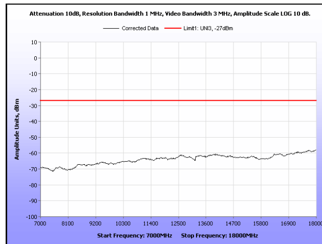
Plot 245. Radiated Spurious, 802.11a, 5320 MHz, 7 GHz – 18 GHz, Sector Antenna
