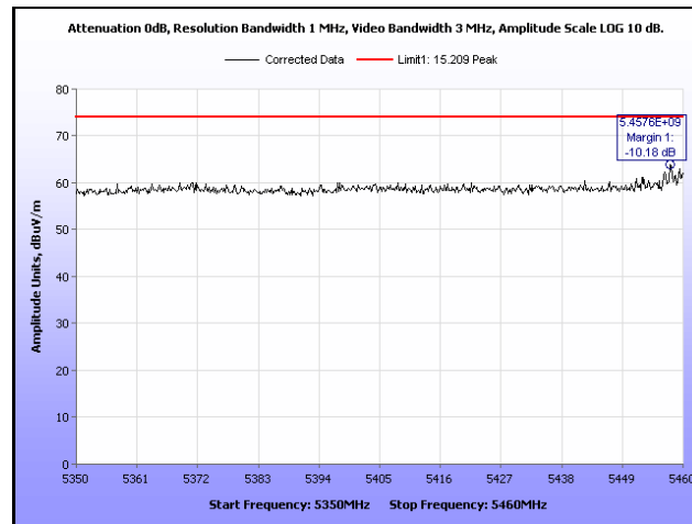
Plot 338. Restricted Band, 802.11n 20 MHz, 5500 MHz, Peak, Omni Antenna
