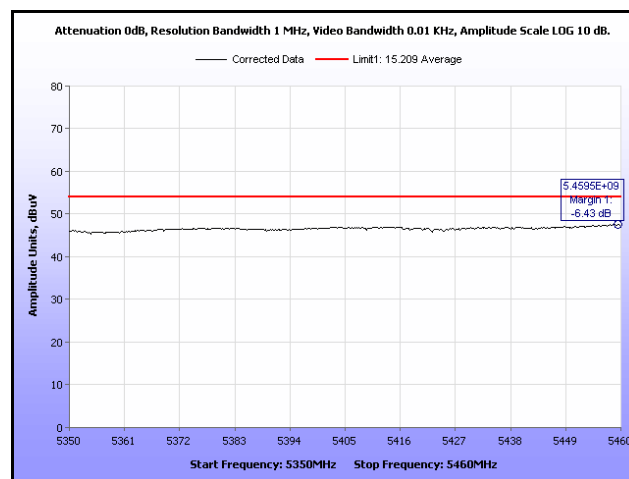
Plot 349. Restricted Band, 802.11n 20 MHz, 5500 MHz, Average, Sector Antenna
