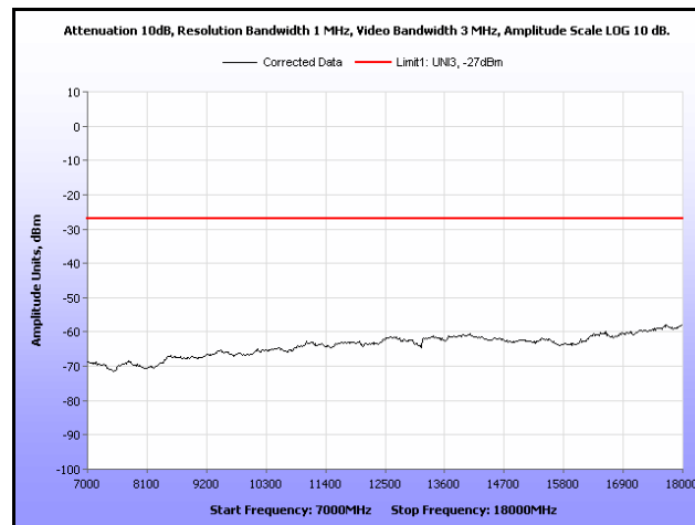
Plot 273. Radiated Spurious, 802.11n 20 MHz, 5500 MHz, 7 GHz – 18 GHz, Sector Antenna
