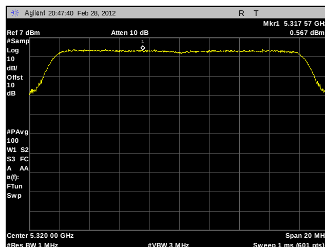
Plot 129. Peak Spectral Density, 802.11a, 5320 MHz, Sector Antenna
