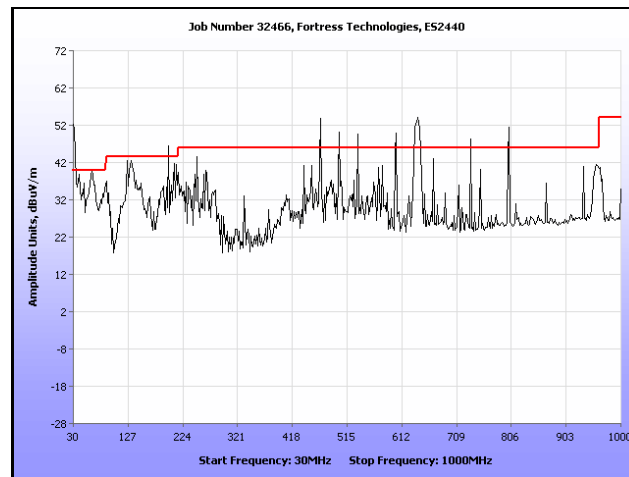
Plot 275. Radiated Spurious, 802.11n 20 MHz, 5580 MHz, 30 MHz – 1 GHz, Sector Antenna
