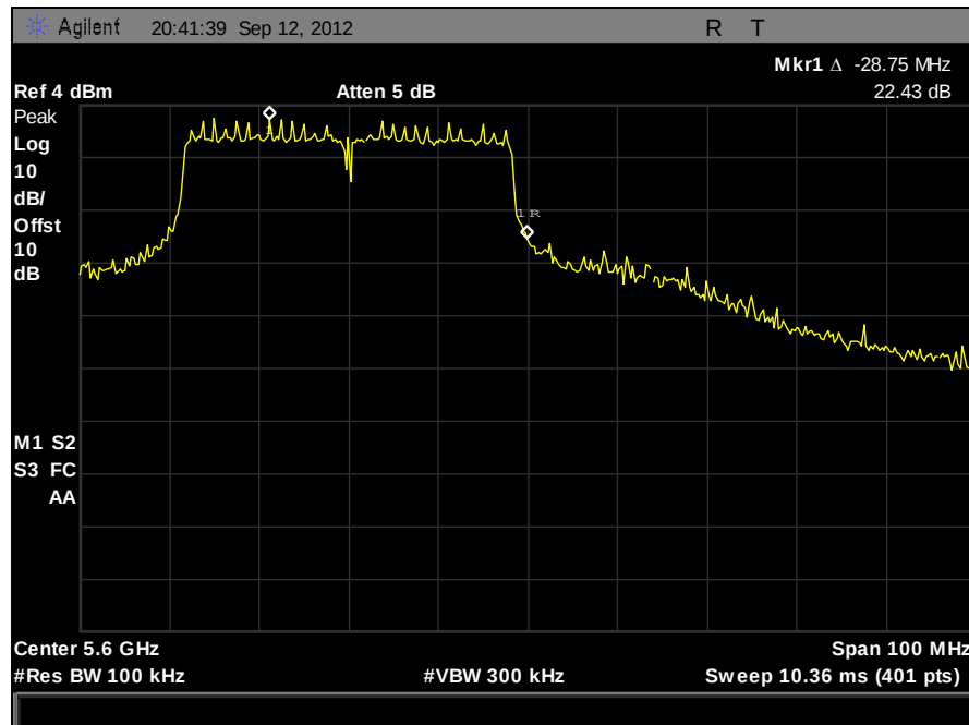
Plot 439. 20 dBc Notched Band, 802.11N 40 MHz, 5580 MHz, Port B
