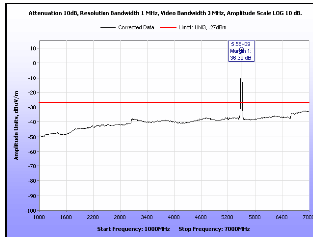
Plot 272. Radiated Spurious, 802.11n 20 MHz, 5500 MHz, 1 GHz – 7 GHz, Sector Antenna
