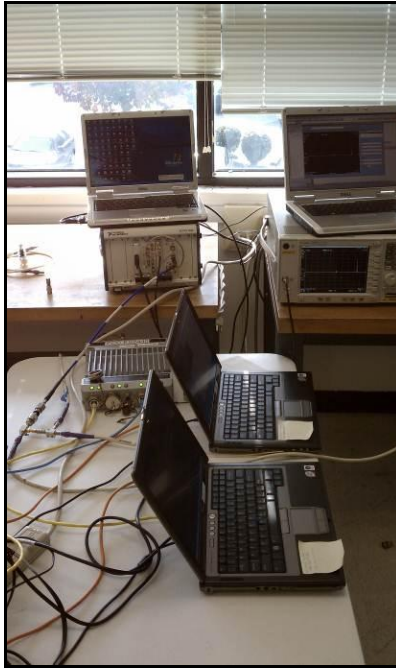
Photograph 5. DFS Test Setup
