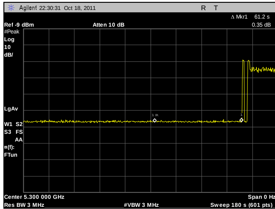
Plot 442. Initial Channel Availability Check Time
