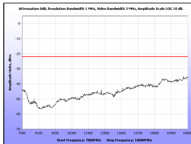
Plot 177. Radiated Spurious, 802.11a, 5500 MHz, 7 GHz – 18 GHz, Omni Antenna
