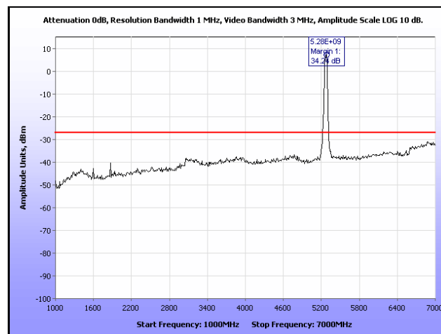
Plot 212. Radiated Spurious, 802.11n 40 MHz, 5270 MHz, 1 GHz – 7 GHz, Omni Antenna
