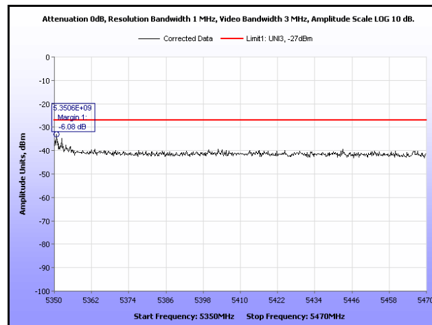
Plot 312. EIRP, 802.11n 20 MHz, 5320 MHz, Band Edge, Omni Antenna
