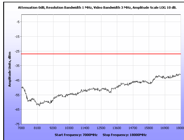
Plot 205. Radiated Spurious, 802.11n 20 MHz, 5580 MHz, 7 GHz – 18 GHz, Omni Antenna
