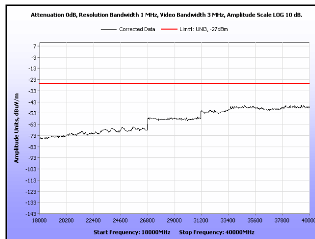
Plot 222. Radiated Spurious, 802.11n 40 MHz, 5310 MHz, 18 GHz – 40 GHz, Omni Antenna
