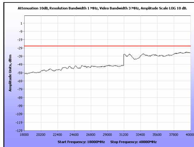
Plot 266. Radiated Spurious, 802.11n 20 MHz, 5300 MHz, 18 GHz – 40 GHz, Sector Antenna
