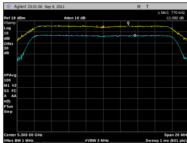
Plot 134. Peak Excursion, 802.11a, 5300 MHz
