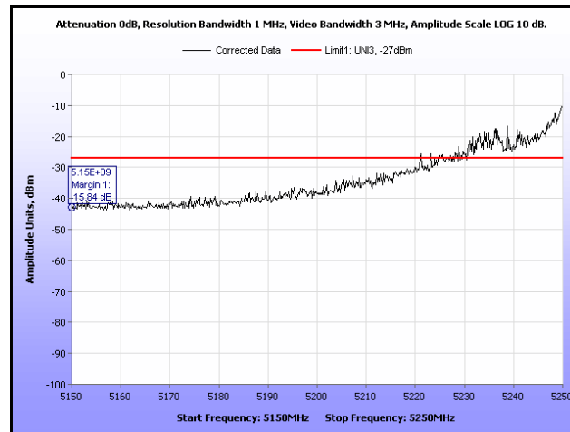
Plot 315. EIRP, 802.11n 40 MHz, 5270 MHz, Band Edge, Omni Antenna
