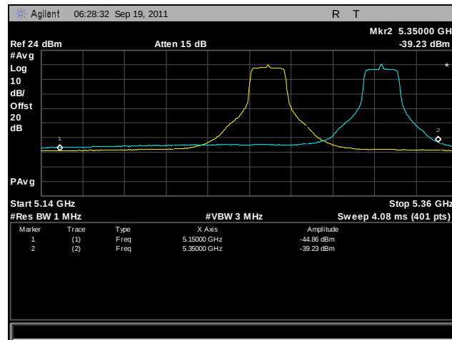
Plot 379. Frequency Stability, 802.11n 20 MHz, 5250 MHz – 5350 MHz @ 10°C, 120 V
