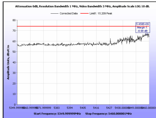
Plot 342. Restricted Band, 802.11n 40 MHz, 5510 MHz, Peak, Omni Antenna
