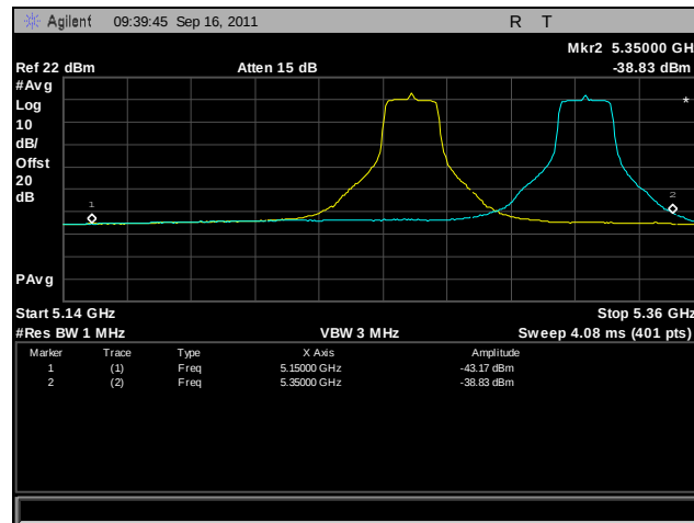
Plot 382. Frequency Stability, 802.11n 20 MHz, 5250 MHz – 5350 MHz @ 20°C, 132 V
