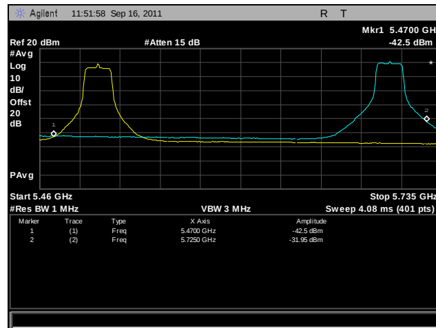
Plot 394. Frequency Stability, 802.11n 20 MHz, 5470 MHz – 5725 MHz @ 30°C, 120 V
