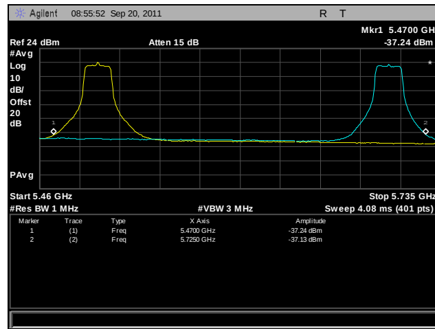
Plot 397. Frequency Stability, 802.11n 20 MHz, 5470 MHz – 5725 MHz @ 55°C, 120 V
