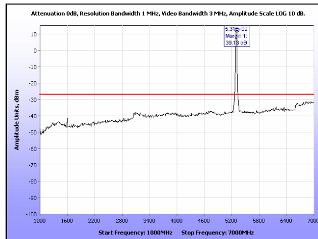
Plot 168. Radiated Spurious, 802.11a, 5300 MHz, 1 GHz – 7 GHz, Omni Antenna
