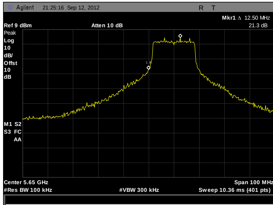
Plot 432. 20 dBc Notched Band, 802.11a, 5660 MHz, Port A
