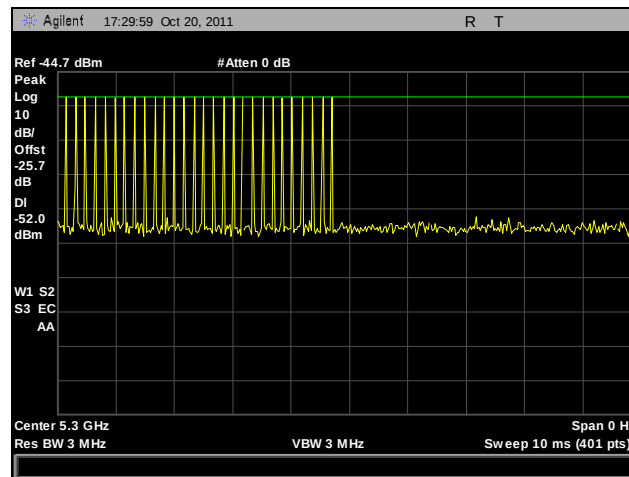
Plot 425. Radar Calibration, Bin 2
