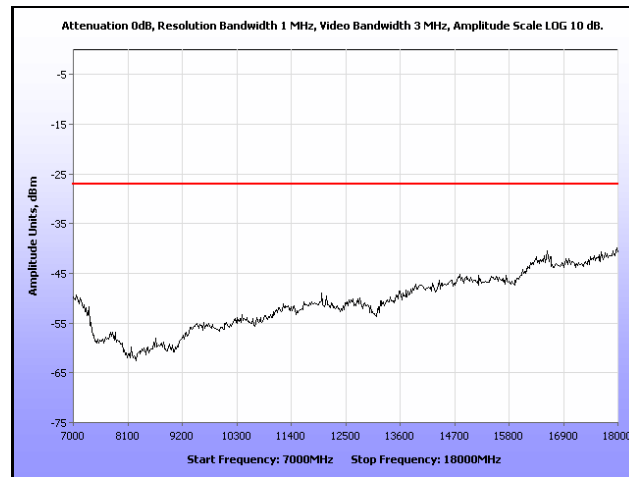
Plot 229. Radiated Spurious, 802.11n 40 MHz, 5580 MHz, 7 GHz – 18 GHz, Omni Antenna
