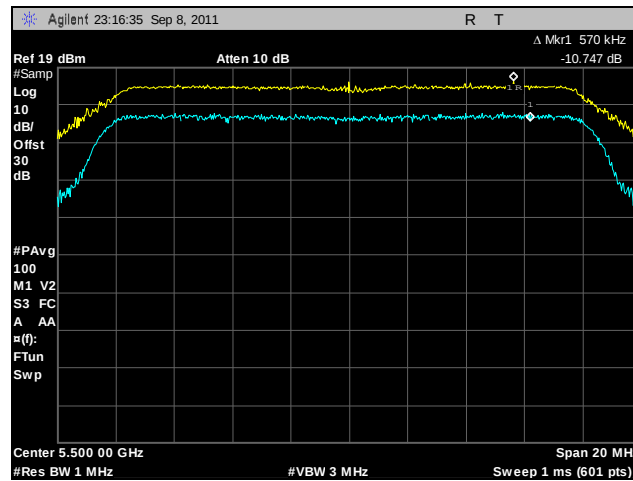
Plot 136. Peak Excursion, 802.11a, 5500 MHz
