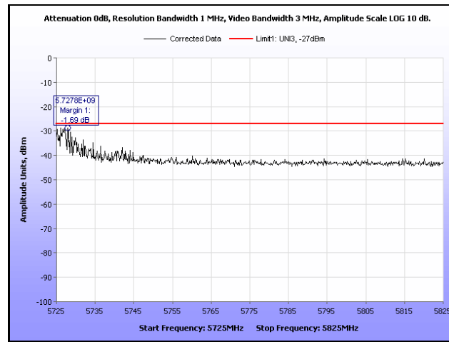
Plot 330. EIRP, 802.11n 40 MHz, 5690 MHz, Band Edge, Sector Antenna
