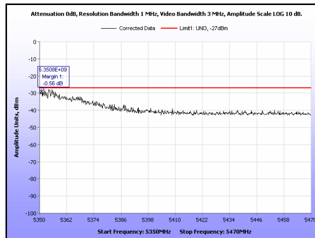
Plot 316. EIRP, 802.11n 40 MHz, 5310 MHz, Band Edge, Omni Antenna
