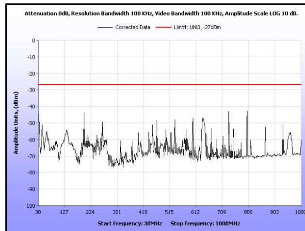
Plot 215. Radiated Spurious, 802.11n 40 MHz, 5300 MHz, 30 MHz – 1 GHz, Omni Antenna
