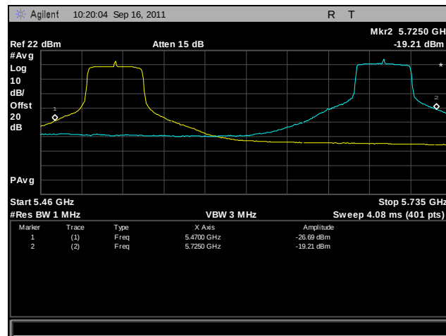
Plot 414. Frequency Stability, 802.11n 40 MHz, 5470 MHz – 5725 MHz @ 20°C, 120 V
