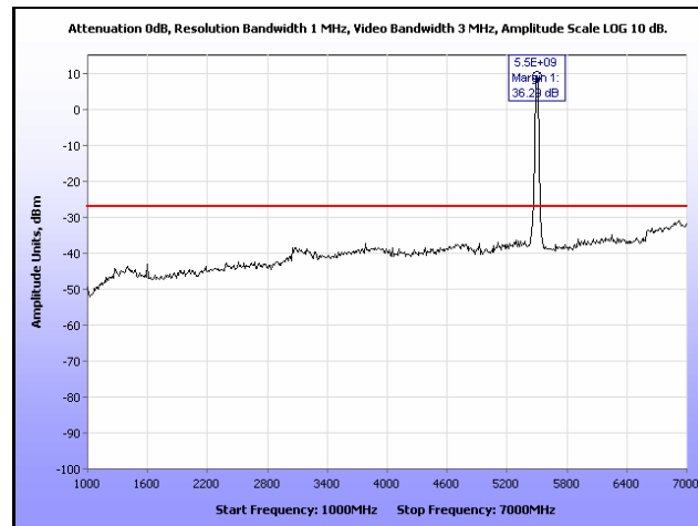
Plot 200. Radiated Spurious, 802.11n 20 MHz, 5500 MHz, 1 GHz – 7 GHz, Omni Antenna
