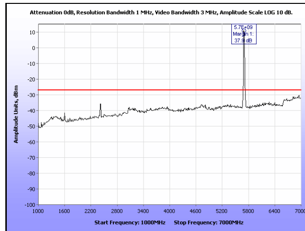
Plot 208. Radiated Spurious, 802.11n 20 MHz, 5700 MHz, 1 GHz – 7 GHz, Omni Antenna
