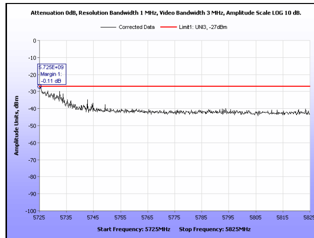
Plot 326. EIRP, 802.11n 20 MHz, 5700 MHz, Band Edge, Sector Antenna
