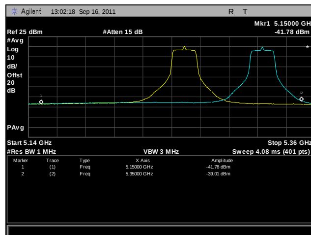
Plot 384. Frequency Stability, 802.11n 20 MHz, 5250 MHz – 5350 MHz @ 40°C, 120 V
