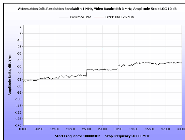
Plot 234. Radiated Spurious, 802.11n 40 MHz, 5690 MHz, 18 GHz – 40 GHz, Omni Antenna
