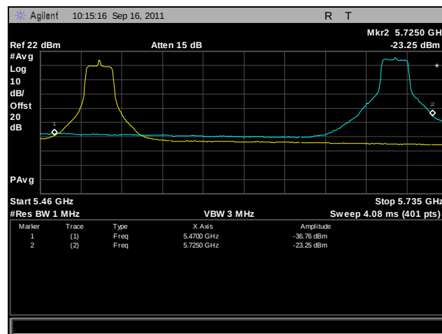
Plot 392. Frequency Stability, 802.11n 20 MHz, 5470 MHz – 5725 MHz @ 20°C, 120 V
