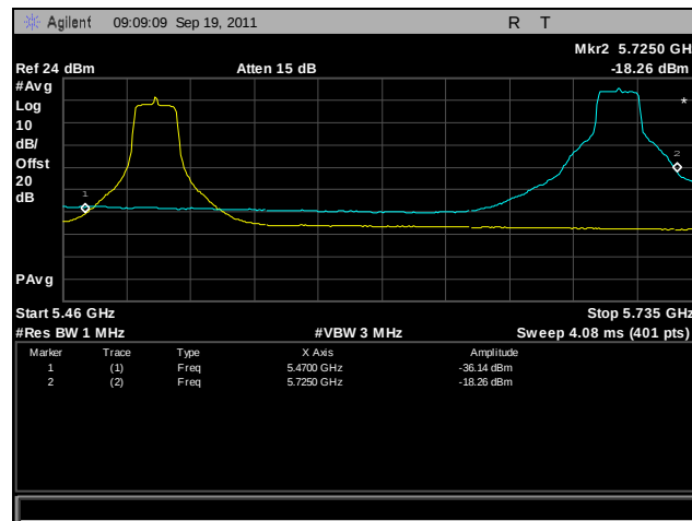
Plot 389. Frequency Stability, 802.11n 20 MHz, 5470 MHz – 5725 MHz @ 0°C, 120 V
