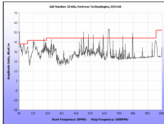
Plot 271. Radiated Spurious, 802.11n 20 MHz, 5500 MHz, 30 MHz – 1 GHz, Sector Antenna
