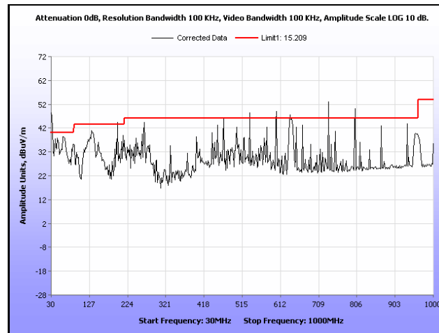
Plot 295. Radiated Spurious, 802.11n 40 MHz, 5510 MHz, 30 MHz – 1 GHz, Sector Antenna
