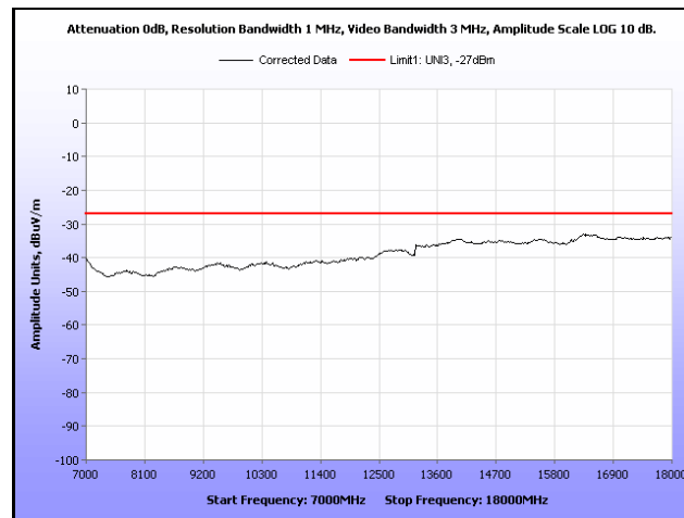
Plot 233. Radiated Spurious, 802.11n 40 MHz, 5690 MHz, 7 GHz – 18 GHz, Omni Antenna
