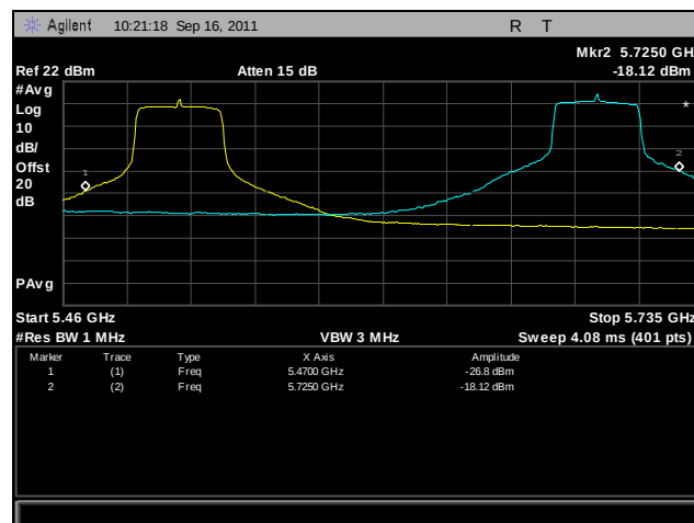
Plot 415. Frequency Stability, 802.11n 40 MHz, 5470 MHz – 5725 MHz @ 20°C, 132 V
