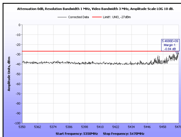
Plot 329. EIRP, 802.11n 40 MHz, 5510 MHz, Band Edge, Sector Antenna
