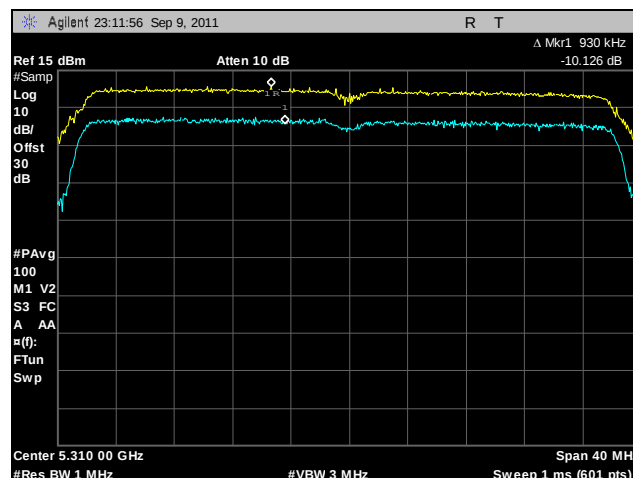
Plot 153. Peak Excursion, 802.11n 40 MHz, Port A, 5310 MHz
