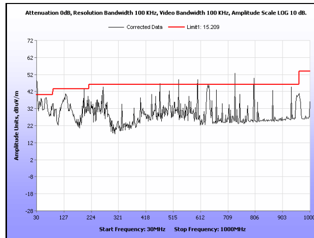
Plot 247. Radiated Spurious, 802.11a, 5500 MHz, 30 MHz – 1 GHz, Sector Antenna
