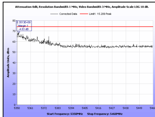
Plot 352. Restricted Band, 802.11n 40 MHz, 5310 MHz, Peak, Sector Antenna
