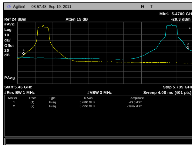
Plot 367. Frequency Stability, 802.11a, 5470 MHz – 5725 MHz @ 0°C, 120 V
