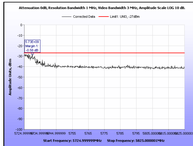
Plot 322. EIRP, 802.11a, 5700 MHz, Band Edge, Sector Antenna
