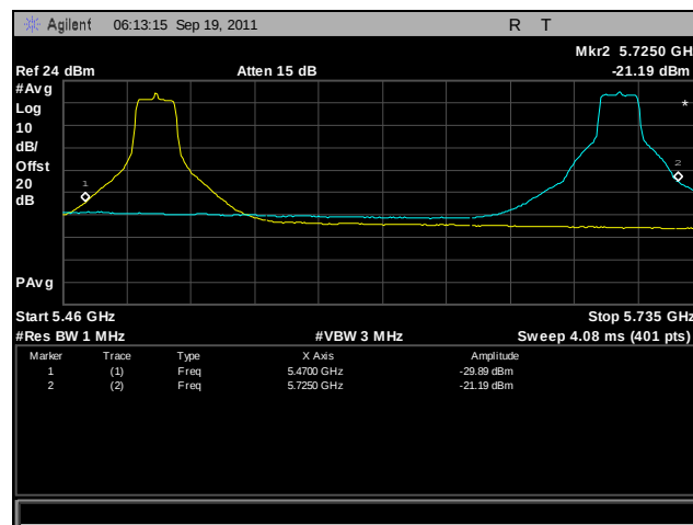
Plot 368. Frequency Stability, 802.11a, 5470 MHz – 5725 MHz @ 10°C, 120 V
