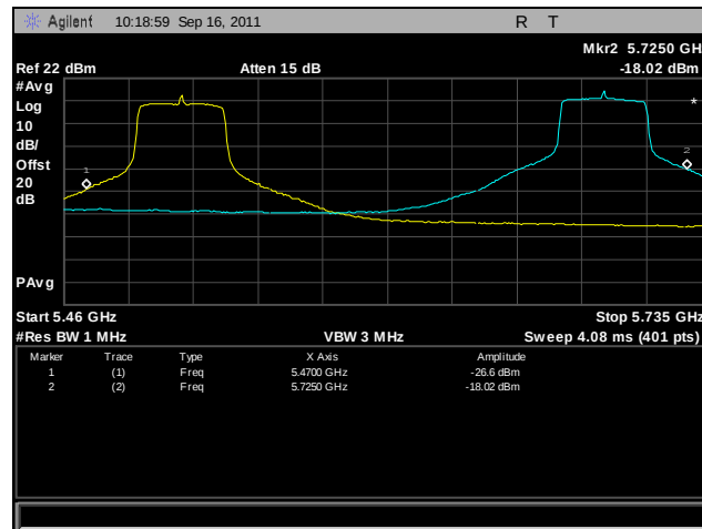
Plot 413. Frequency Stability, 802.11n 40 MHz, 5470 MHz – 5725 MHz @ 20°C, 108 V
