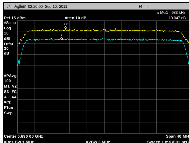
Plot 162. Peak Excursion, 802.11n 40 MHz, Port B, 5690 MHz
