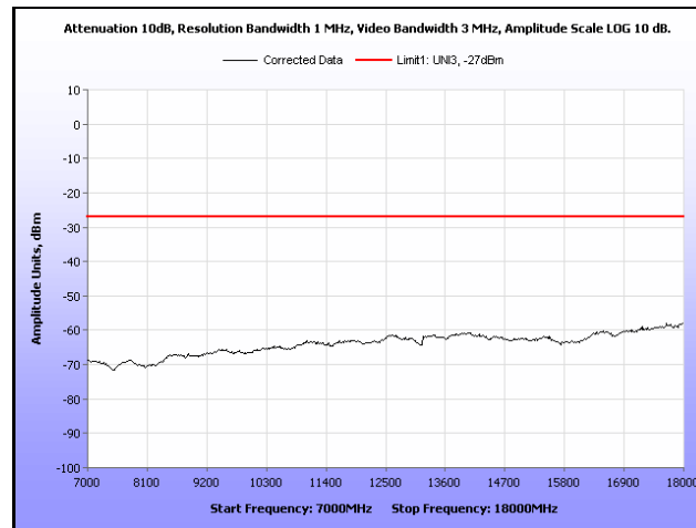
Plot 265. Radiated Spurious, 802.11n 20 MHz, 5300 MHz, 7 GHz – 18 GHz, Sector Antenna
