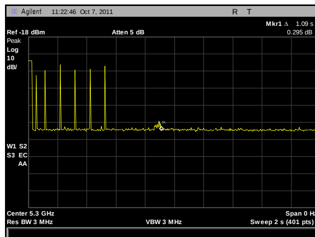
Plot 449. Channel Closing Transmission Time, 3
