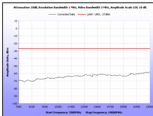
Plot 261. Radiated Spurious, 802.11n 20 MHz, 5260 MHz, 7 GHz – 18 GHz, Sector Antenna
