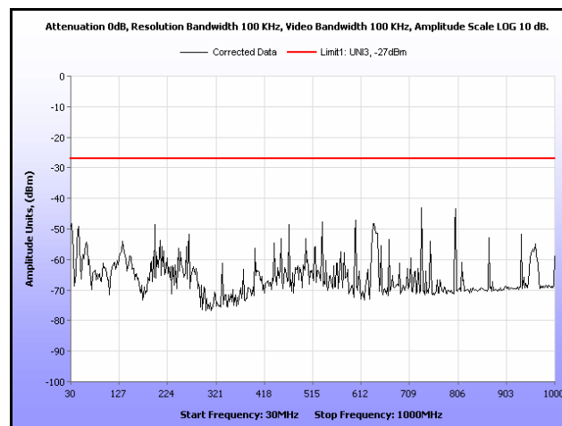
Plot 231. Radiated Spurious, 802.11n 40 MHz, 5690 MHz, 30 MHz – 1 GHz, Omni Antenna
