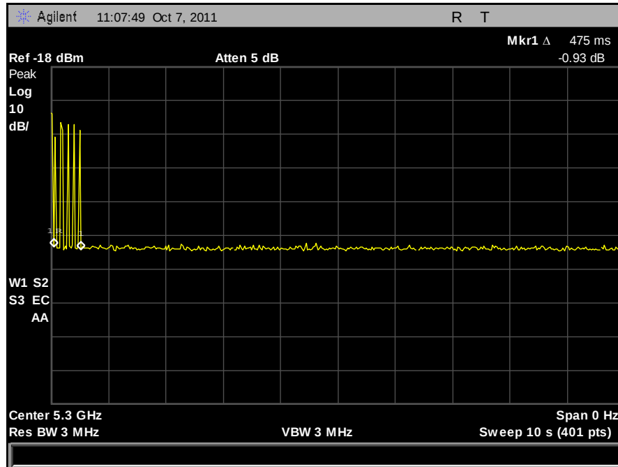
Plot 445. Channel Move Time
