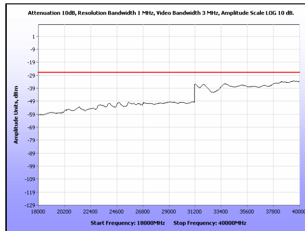
Plot 302. Radiated Spurious, 802.11n 40 MHz, 5580 MHz, 18 GHz – 40 GHz, Sector Antenna
