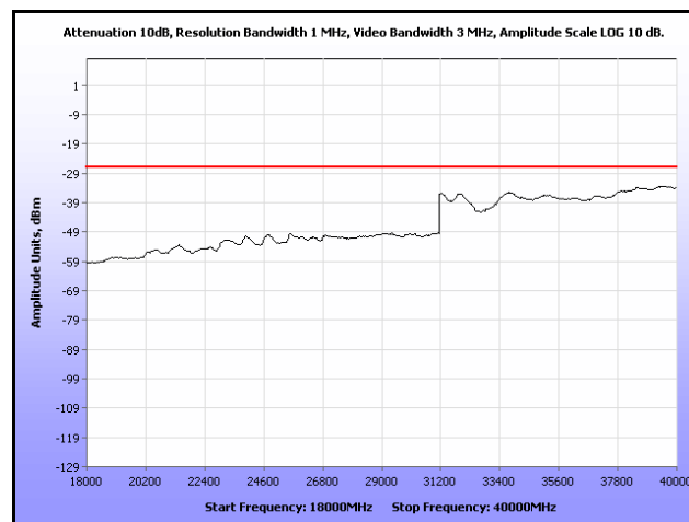
Plot 294. Radiated Spurious, 802.11n 40 MHz, 5310 MHz, 18 GHz – 40 GHz, Sector Antenna
