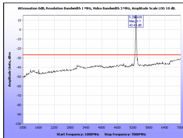
Plot 192. Radiated Spurious, 802.11n 20 MHz, 5300 MHz, 1 GHz – 7 GHz, Omni Antenna
