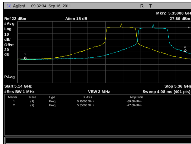
Plot 404. Frequency Stability, 802.11n 40 MHz, 5250 MHz – 5350 MHz @ 20°C, 132 V
