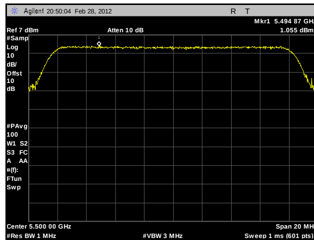
Plot 130. Peak Spectral Density, 802.11a, 5500 MHz, Sector Antenna
