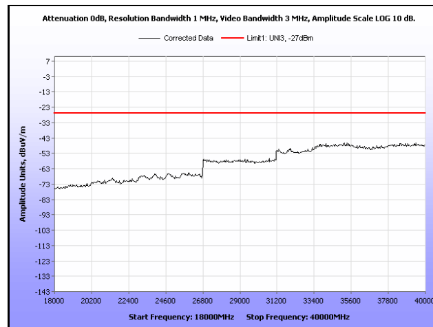
Plot 230. Radiated Spurious, 802.11n 40 MHz, 5580 MHz, 18 GHz – 40 GHz, Omni Antenna
