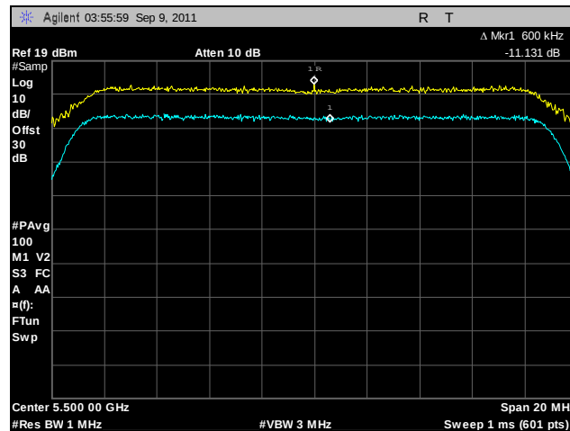
Plot 142. Peak Excursion, 802.11n 20 MHz, Port A, 5500 MHz
