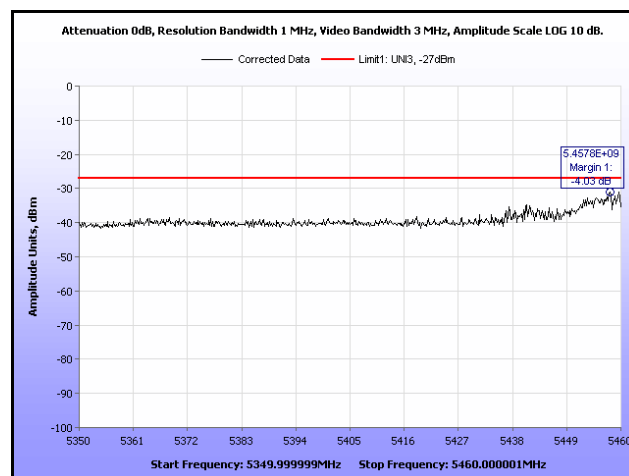
Plot 317. EIRP, 802.11n 40 MHz, 5510 MHz, Band Edge, Omni Antenna
