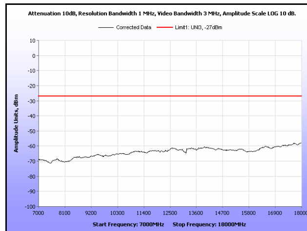
Plot 249. Radiated Spurious, 802.11a, 5500 MHz, 7 GHz – 18 GHz, Sector Antenna
