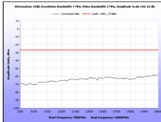
Plot 301. Radiated Spurious, 802.11n 40 MHz, 5580 MHz, 7 GHz – 18 GHz, Sector Antenna
