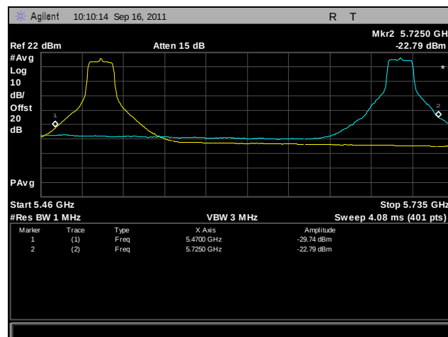
Plot 369. Frequency Stability, 802.11a, 5470 MHz – 5725 MHz @ 20°C, 108 V
