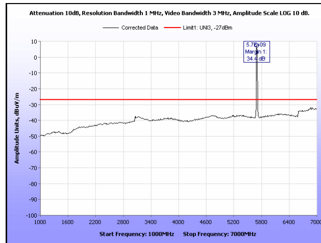
Plot 280. Radiated Spurious, 802.11n 20 MHz, 5700 MHz, 1 GHz – 7 GHz, Sector Antenna
