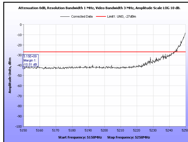
Plot 311. EIRP, 802.11n 20 MHz, 5260 MHz, Band Edge, Omni Antenna
