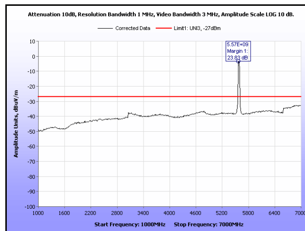
Plot 300. Radiated Spurious, 802.11n 40 MHz, 5580 MHz, 1 GHz – 7 GHz, Sector Antenna
