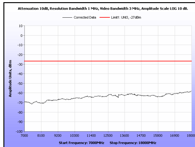
Plot 297. Radiated Spurious, 802.11n 40 MHz, 5510 MHz, 7 GHz – 18 GHz, Sector Antenna
