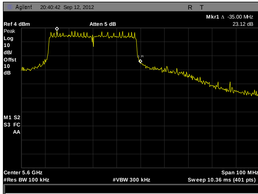
Plot 438. 20 dBc Notched Band, 802.11N 40 MHz, 5580 MHz, Port A
