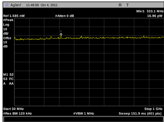
Plot 420. Receiver Spurious Emission, 5.8 GHz, 30 MHz – 1 GHz, Port A
