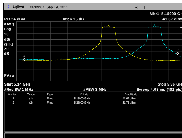
Plot 357. Frequency Stability, 802.11a, 5250 MHz – 5350 MHz @ 10°C, 120 V
