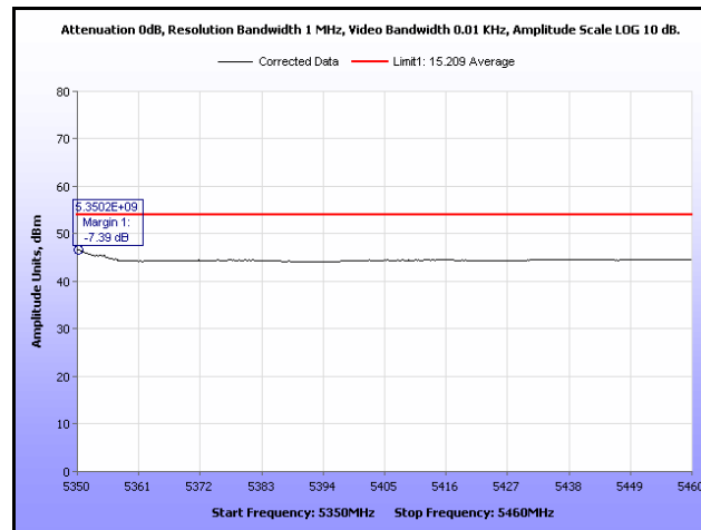
Plot 347. Restricted Band, 802.11n 20 MHz, 5320 MHz, Average, Sector Antenna
