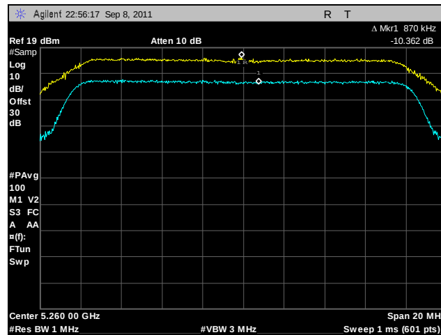
Plot 133. Peak Excursion, 802.11a, 5260 MHz
