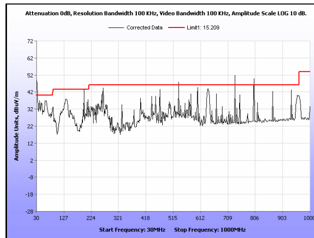
Plot 251. Radiated Spurious, 802.11a, 5580 MHz, 30 MHz – 1 GHz, Sector Antenna
