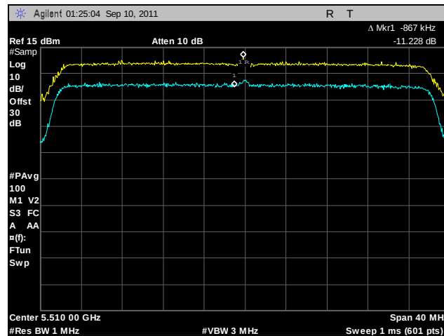
Plot 160. Peak Excursion, 802.11n 40 MHz, Port B, 5510 MHz
