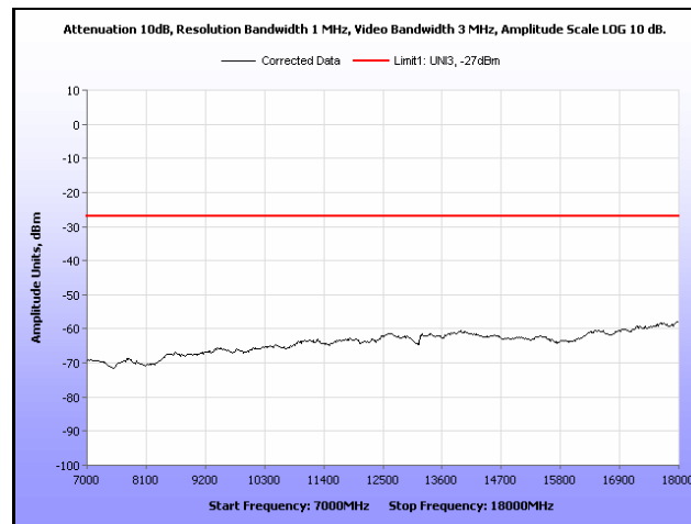
Plot 293. Radiated Spurious, 802.11n 40 MHz, 5310 MHz, 7 GHz – 18 GHz, Sector Antenna
