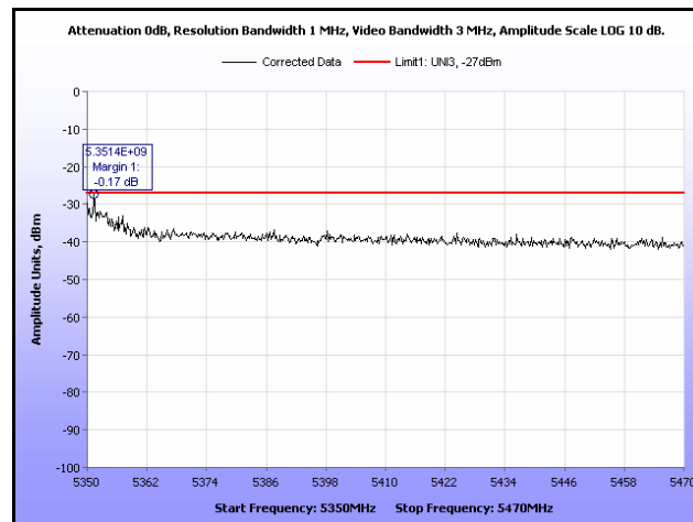
Plot 324. EIRP, 802.11n 20 MHz, 5320 MHz, Band Edge, Sector Antenna
