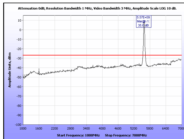
Plot 228. Radiated Spurious, 802.11n 40 MHz, 5580 MHz, 1 GHz – 7 GHz, Omni Antenna
