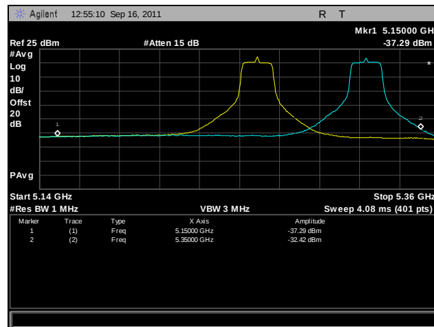
Plot 362. Frequency Stability, 802.11a, 5250 MHz – 5350 MHz @ 40°C, 120 V
