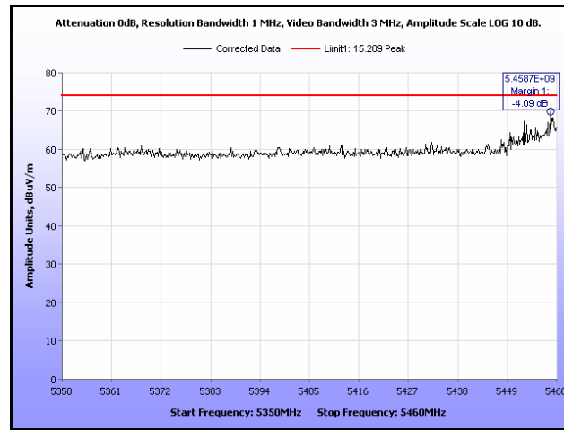
Plot 334. Restricted Band, 802.11a, 5500 MHz, Peak, Omni Antenna
