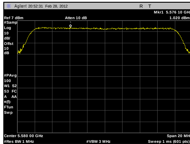
Plot 131. Peak Spectral Density, 802.11a, 5580 MHz, Sector Antenna
