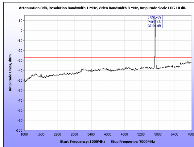
Plot 184. Radiated Spurious, 802.11a, 5700 MHz, 1 GHz – 7 GHz, Omni Antenna
