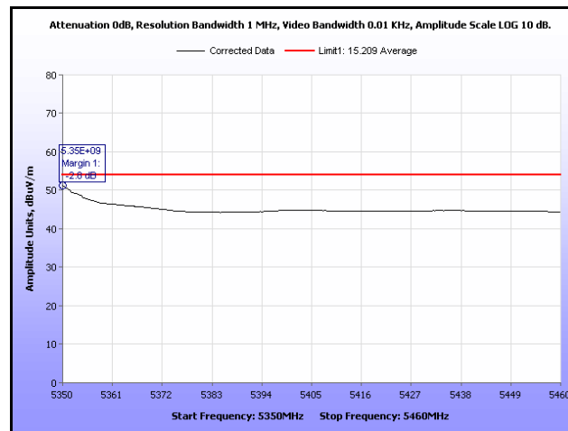
Plot 331. Restricted Band, 802.11a, 5320 MHz, Average, Omni Antenna
