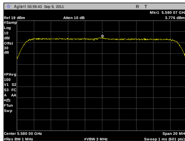
Plot 113. Peak Spectral Density, 802.11n 20 MHz, Port B, 5580 MHz
