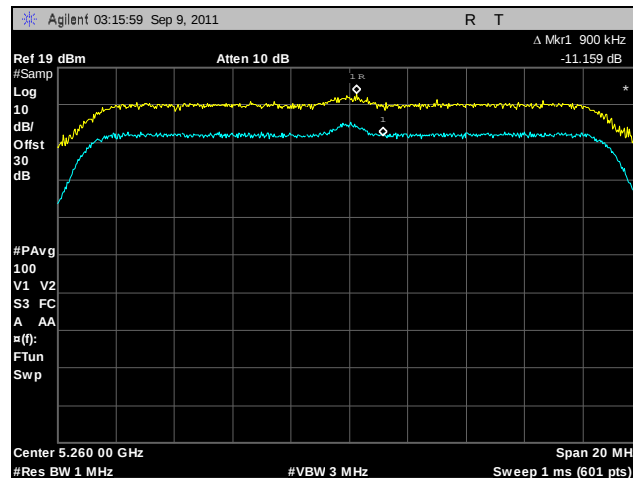
Plot 145. Peak Excursion, 802.11n 20 MHz, Port B, 5260 MHz
