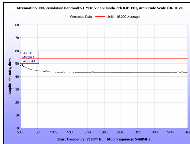
Plot 343. Restricted Band, 802.11a, 5320 MHz, Average, Sector Antenna
