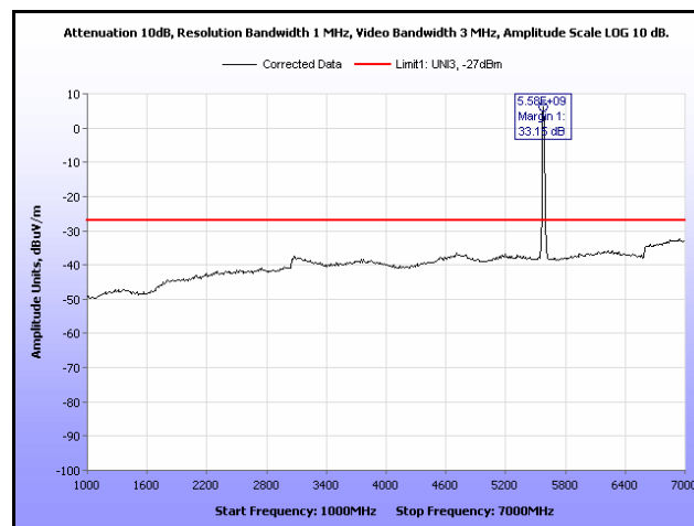
Plot 252. Radiated Spurious, 802.11a, 5580 MHz, 1 GHz – 7 GHz, Sector Antenna
