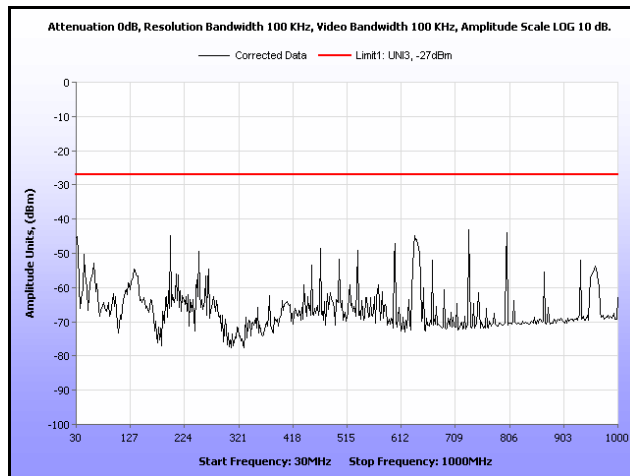
Plot 163. Radiated Spurious, 802.11a, 5260 MHz, 30 MHz – 1 GHz, Omni Antenna
