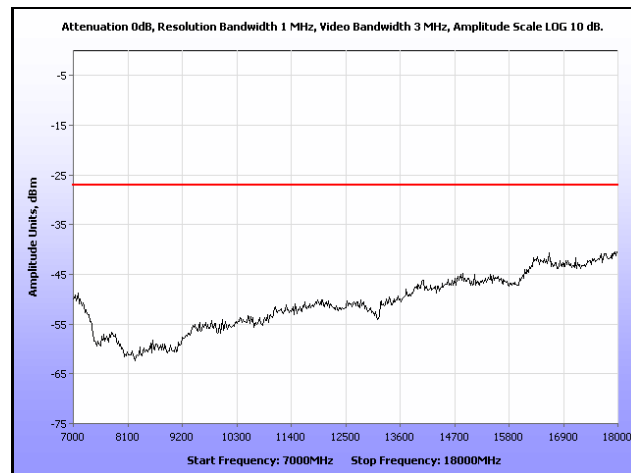
Plot 225. Radiated Spurious, 802.11n 40 MHz, 5510 MHz, 7 GHz – 18 GHz, Omni Antenna
