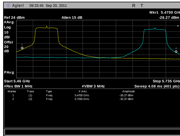
Plot 419. Frequency Stability, 802.11n 40 MHz, 5470 MHz – 5725 MHz @ 55°C, 120 V
