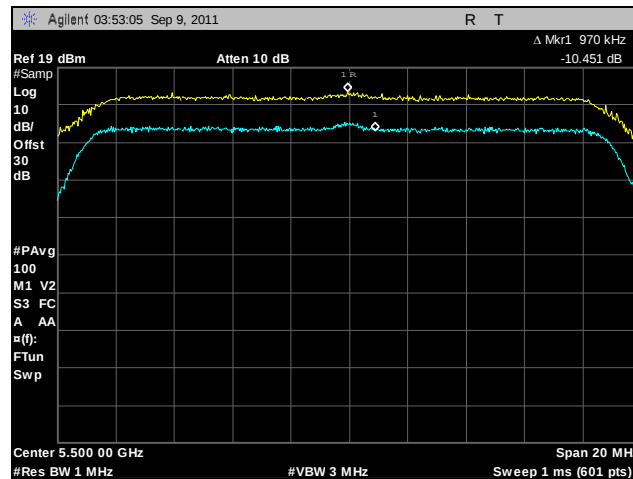
Plot 148. Peak Excursion, 802.11n 20 MHz, Port B, 5500 MHz
