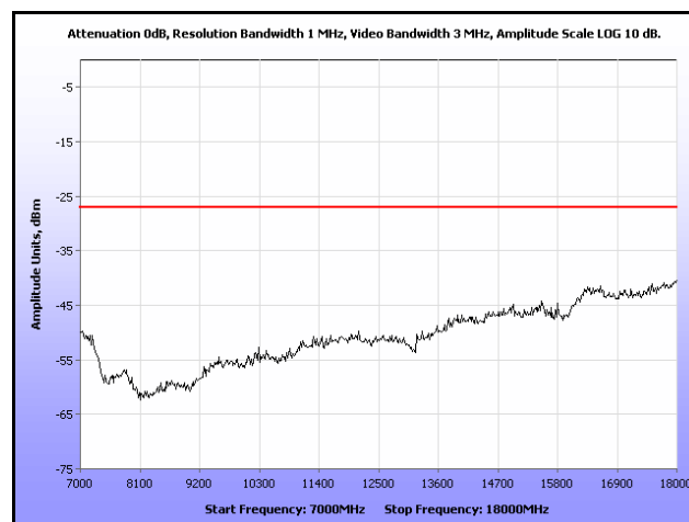
Plot 189. Radiated Spurious, 802.11n 20 MHz, 5260 MHz, 7 GHz – 18 GHz, Omni Antenna
