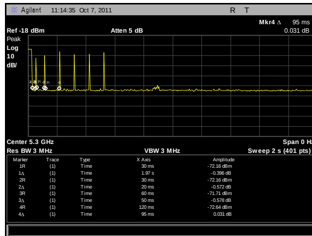
Plot 447. Channel Closing Transmission Time, 1
