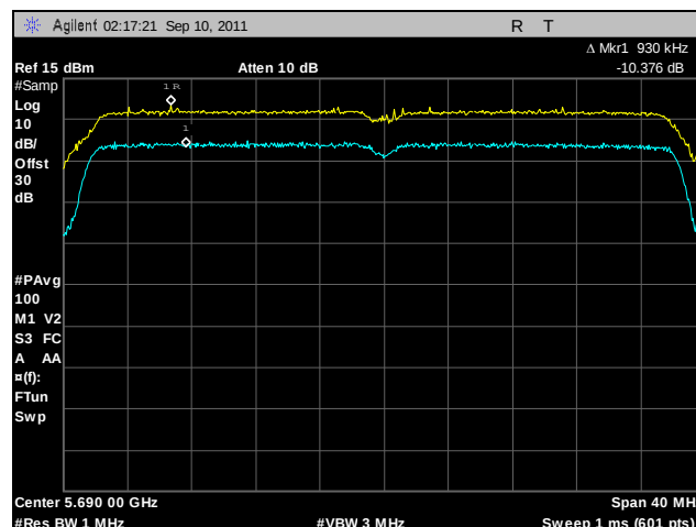
Plot 156. Peak Excursion, 802.11n 40 MHz, Port A, 5690 MHz
