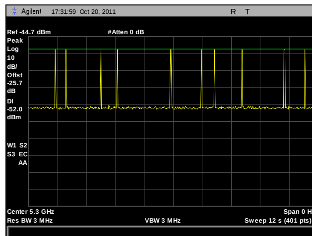
Plot 428. Radar Calibration, Bin 5
