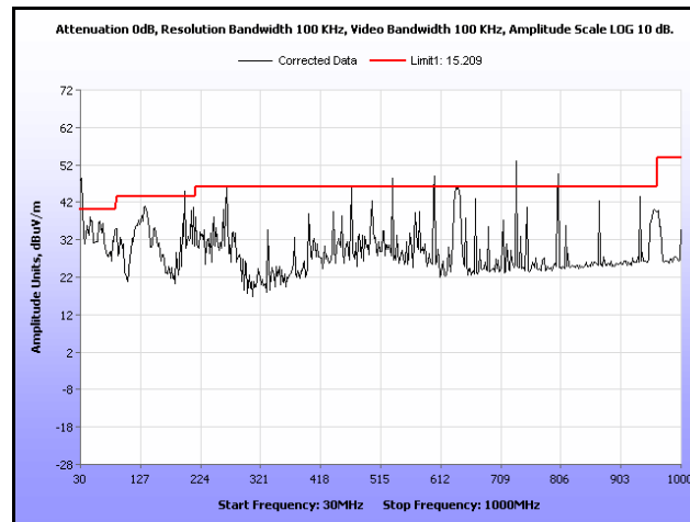
Plot 235. Radiated Spurious, 802.11a, 5260 MHz, 30 MHz – 1 GHz, Sector Antenna
