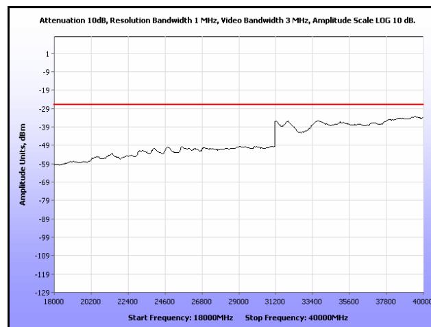
Plot 270. Radiated Spurious, 802.11n 20 MHz, 5320 MHz, 18 GHz – 40 GHz, Sector Antenna
