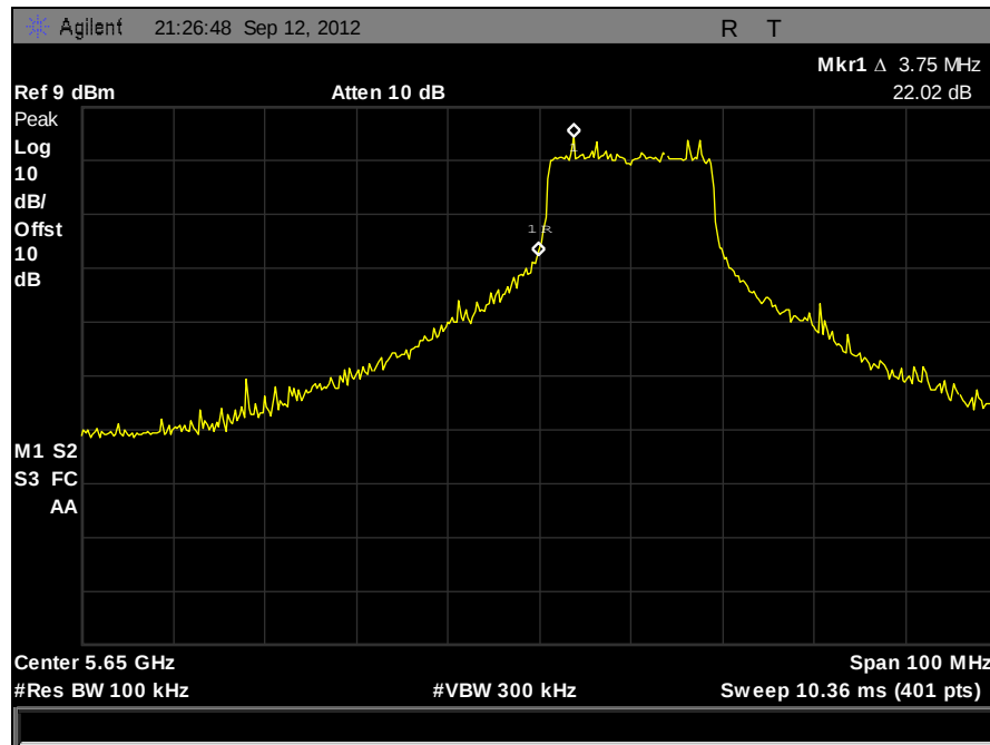
Plot 436. 20 dBc Notched Band, 802.11N 20 MHz, 5660 MHz, Port A
