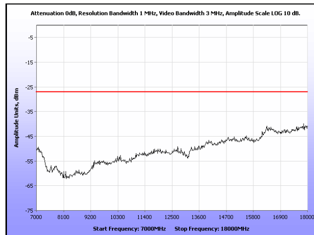
Plot 201. Radiated Spurious, 802.11n 20 MHz, 5500 MHz, 7 GHz – 18 GHz, Omni Antenna
