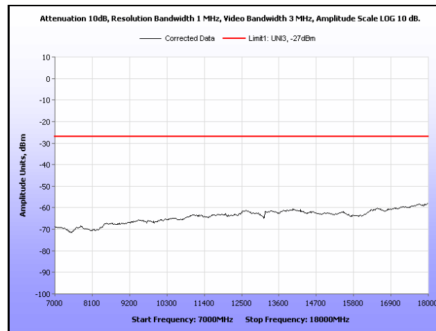
Plot 281. Radiated Spurious, 802.11n 20 MHz, 5700 MHz, 7 GHz – 18 GHz, Sector Antenna
