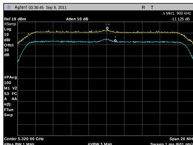
Plot 147. Peak Excursion, 802.11n 20 MHz, Port B, 5320 MHz
