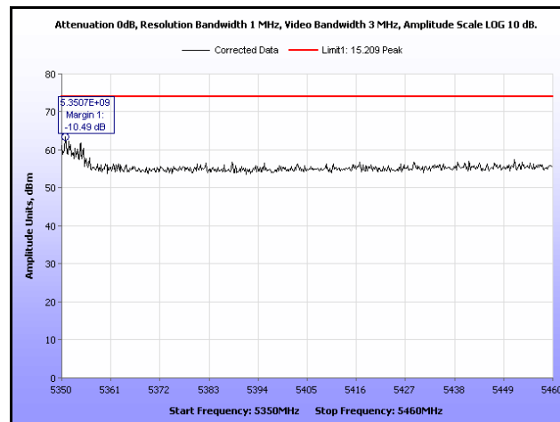
Plot 348. Restricted Band, 802.11n 20 MHz, 5320 MHz, Peak, Sector Antenna
