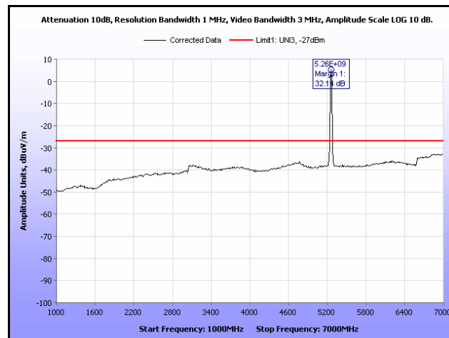
Plot 236. Radiated Spurious, 802.11a, 5260 MHz, 1 GHz – 7 GHz, Sector Antenna
