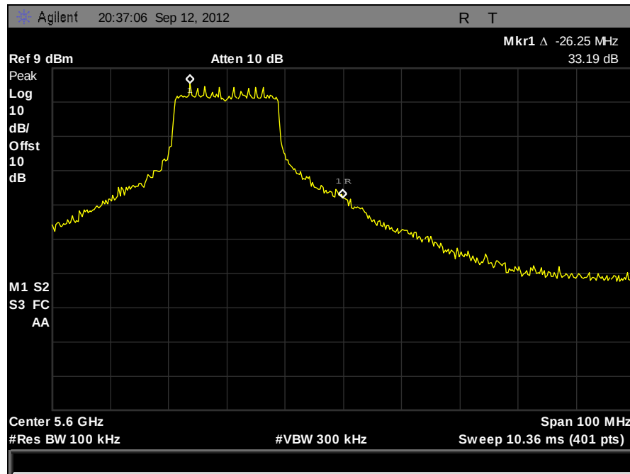
Plot 434. 20 dBc Notched Band, 802.11N 20 MHz, 5580 MHz, Port A
