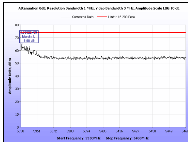
Plot 344. Restricted Band, 802.11a, 5320 MHz, Peak, Sector Antenna
