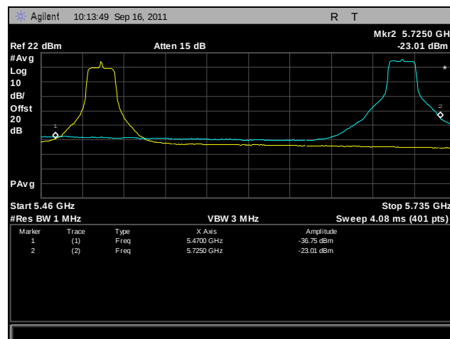
Plot 393. Frequency Stability, 802.11n 20 MHz, 5470 MHz – 5725 MHz @ 20°C, 132 V
