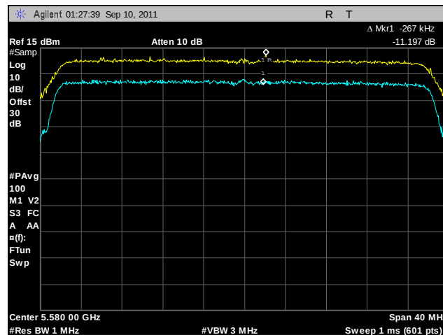
Plot 161. Peak Excursion, 802.11n 40 MHz, Port B, 5580 MHz
