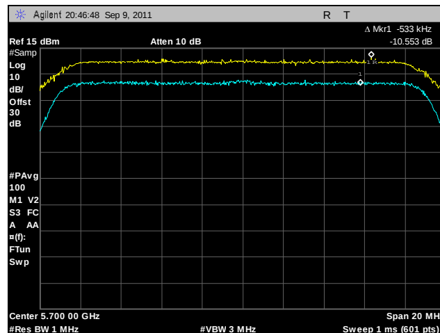
Plot 150. Peak Excursion, 802.11n 20 MHz, Port B, 5700 MHz
