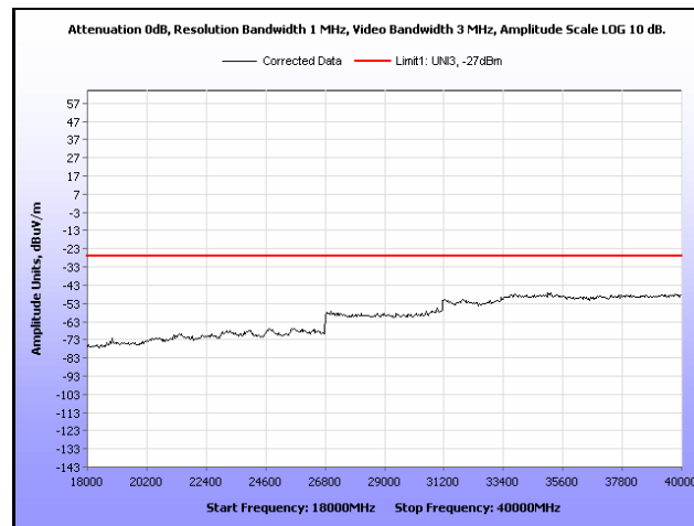
Plot 194. Radiated Spurious, 802.11n 20 MHz, 5300 MHz, 18 GHz – 40 GHz, Omni Antenna
