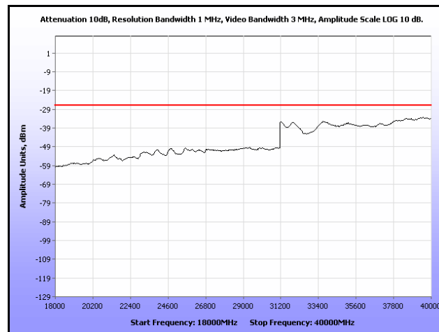
Plot 306. Radiated Spurious, 802.11n 40 MHz, 5690 MHz, 18 GHz – 40 GHz, Sector Antenna
