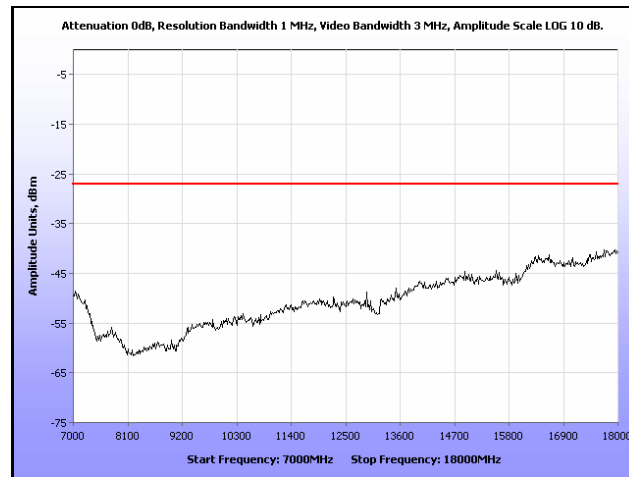
Plot 181. Radiated Spurious, 802.11a, 5580 MHz, 7 GHz – 18 GHz, Omni Antenna
