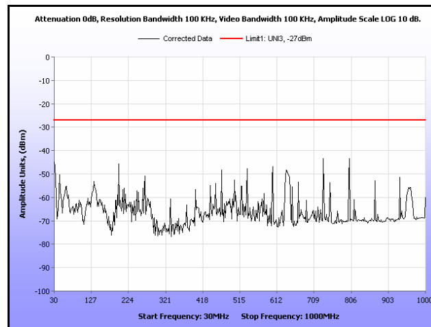
Plot 203. Radiated Spurious, 802.11n 20 MHz, 5580 MHz, 30 MHz – 1 GHz, Omni Antenna
