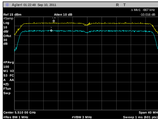
Plot 154. Peak Excursion, 802.11n 40 MHz, Port A, 5510 MHz
