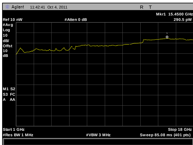
Plot 423. Receiver Spurious Emission, 5.8 GHz, 1 GHz – 18 GHz, Port B
