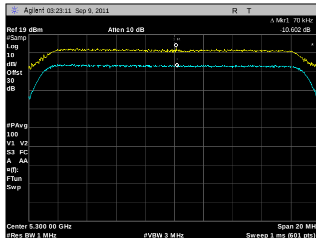
Plot 140. Peak Excursion, 802.11n 20 MHz, Port A, 5300 MHz
