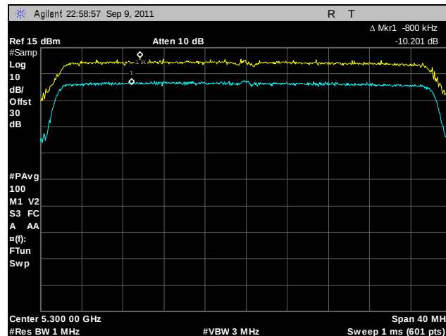
Plot 158. Peak Excursion, 802.11n 40 MHz, Port B, 5300 MHz
