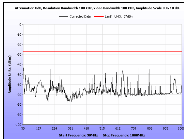
Plot 171. Radiated Spurious, 802.11a, 5320 MHz, 30 MHz – 1 GHz, Omni Antenna
