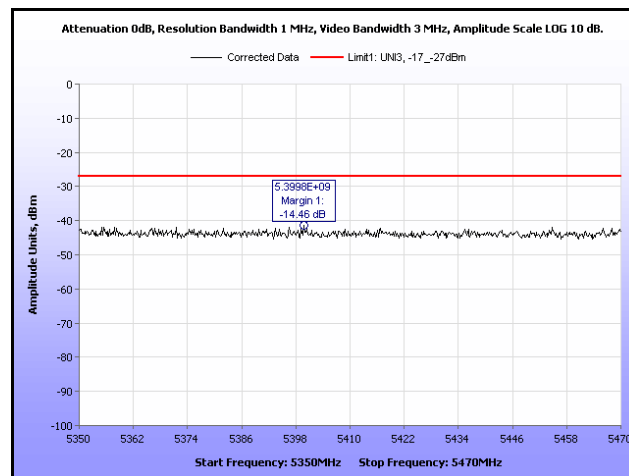
Plot 308. EIRP, 802.11a, 5320 MHz, Band Edge, Omni Antenna
