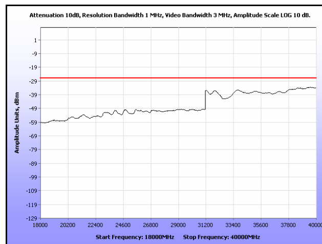
Plot 282. Radiated Spurious, 802.11n 20 MHz, 5700 MHz, 18 GHz – 40 GHz, Sector Antenna
