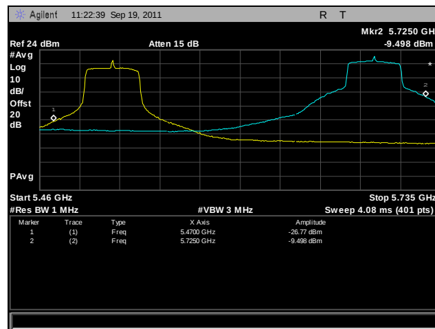
Plot 410. Frequency Stability, 802.11n 40 MHz, 5470 MHz – 5725 MHz @ -10°C, 120 V
