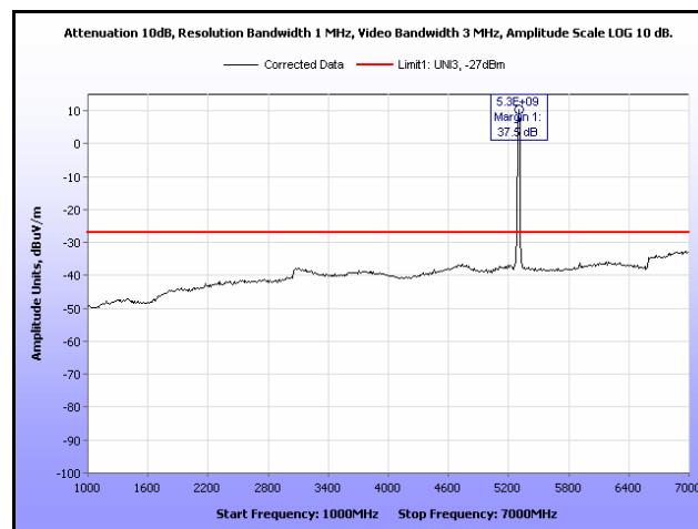
Plot 264. Radiated Spurious, 802.11n 20 MHz, 5300 MHz, 1 GHz – 7 GHz, Sector Antenna
