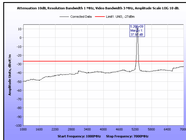
Plot 284. Radiated Spurious, 802.11n 40 MHz, 5270 MHz, 1 GHz – 7 GHz, Sector Antenna
