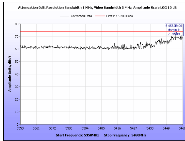
Plot 354. Restricted Band, 802.11n 40 MHz, 5510 MHz, Peak, Sector Antenna
