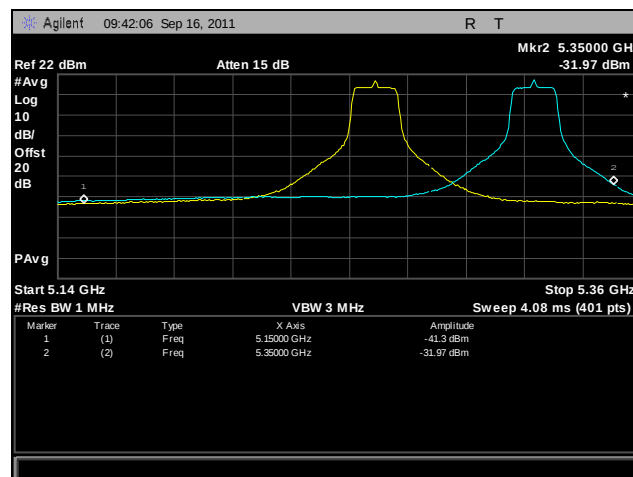
Plot 360. Frequency Stability, 802.11a, 5250 MHz – 5350 MHz @ 20°C, 132 V
