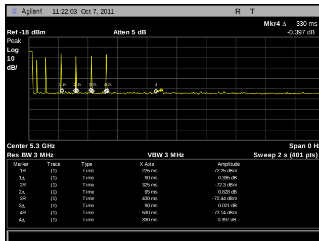
Plot 448. Channel Closing Transmission Time, 2
