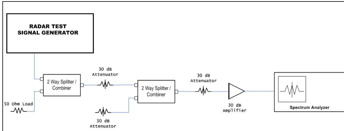
Figure 5. DFS Radar Waveform Calibration Setup
