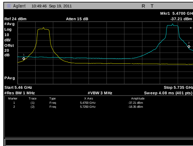
Plot 388. Frequency Stability, 802.11n 20 MHz, 5470 MHz – 5725 MHz @ -10°C, 120 V
