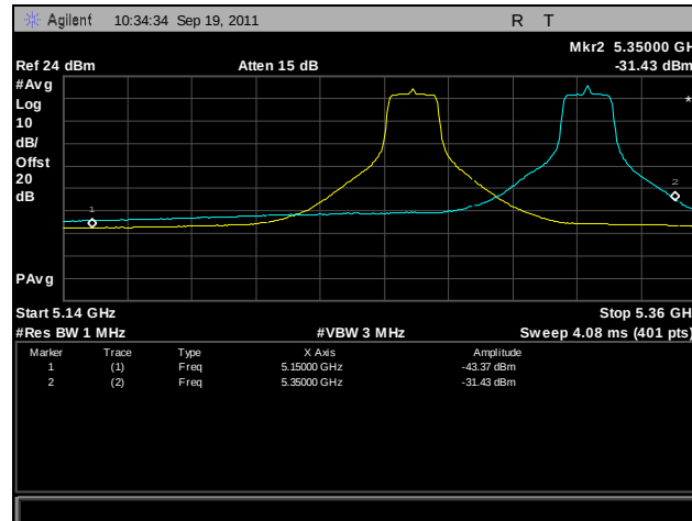
Plot 355. Frequency Stability, 802.11a, 5250 MHz – 5350 MHz @ -10°C, 120 V
