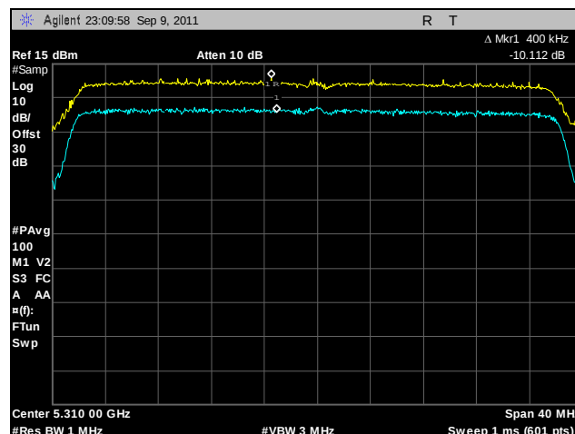
Plot 159. Peak Excursion, 802.11n 40 MHz, Port B, 5310 MHz
