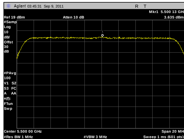
Plot 112. Peak Spectral Density, 802.11n 20 MHz, Port B, 5500 MHz
