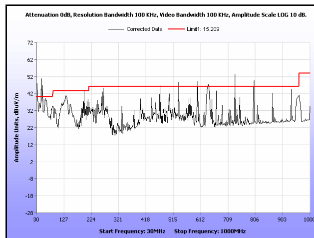
Plot 267. Radiated Spurious, 802.11n 20 MHz, 5320 MHz, 30 MHz – 1 GHz, Sector Antenna
