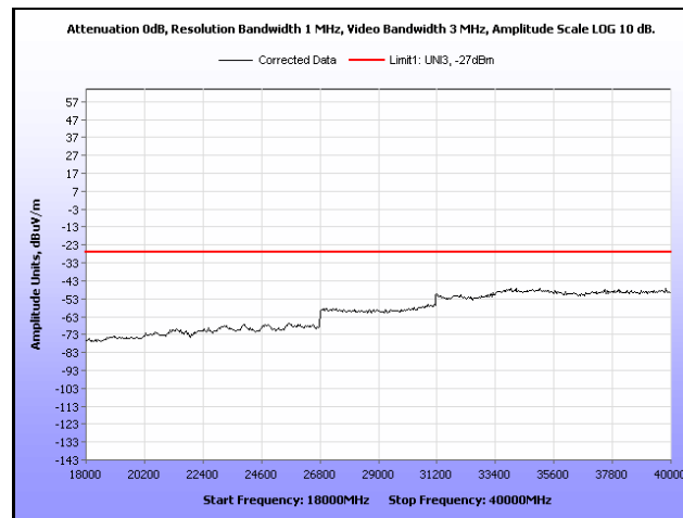
Plot 182. Radiated Spurious, 802.11a, 5580 MHz, 18 GHz – 40 GHz, Omni Antenna
