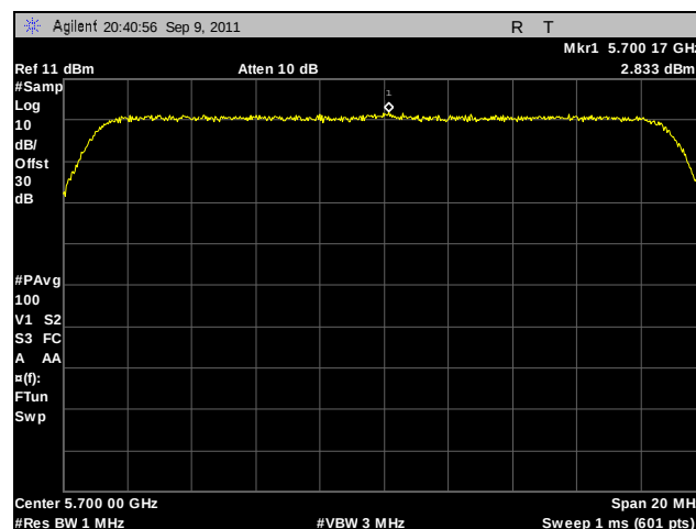
Plot 114. Peak Spectral Density, 802.11n 20 MHz, Port B, 5700 MHz
