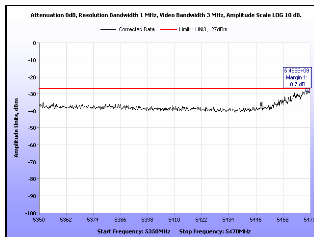
Plot 321. EIRP, 802.11a, 5500 MHz, Band Edge, Sector Antenna
