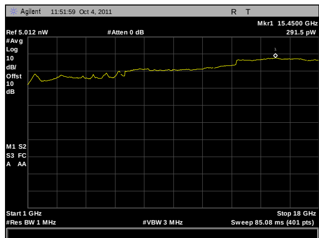
Plot 421. Receiver Spurious Emission, 5.8 GHz, 1 GHz – 18 GHz, Port A
