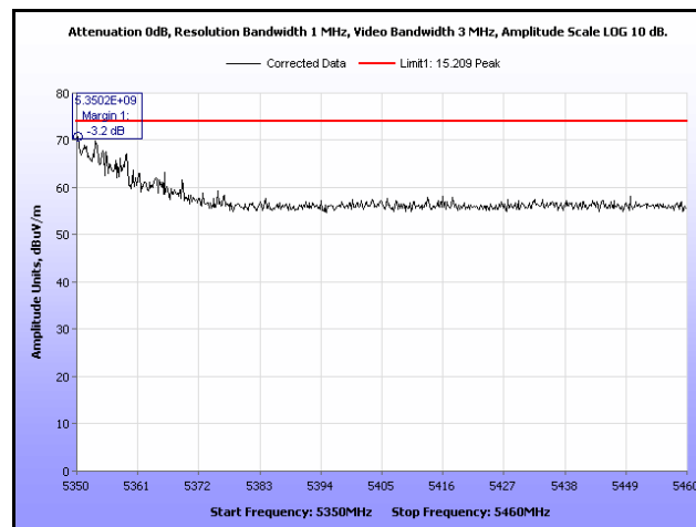
Plot 332. Restricted Band, 802.11a, 5320 MHz, Peak, Omni Antenna
