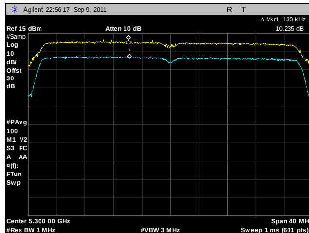
Plot 152. Peak Excursion, 802.11n 40 MHz, Port A, 5300 MHz
