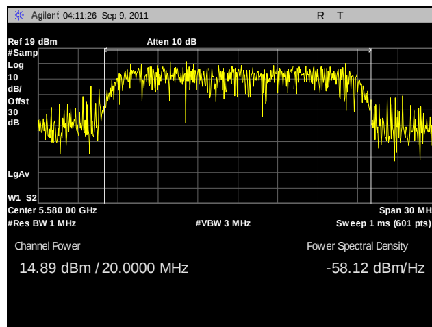
Plot 77. Conducted Output Power, 802.11n 20 MHz, Port A, 5580 MHz
