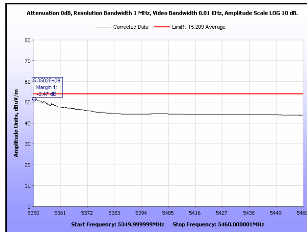
Plot 339. Restricted Band, 802.11n 40 MHz, 5310 MHz, Average, Omni Antenna
