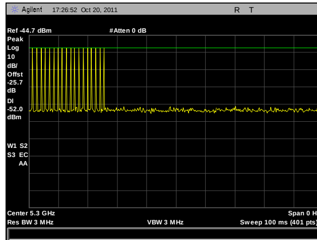
Plot 424. Radar Calibration, Bin 1
