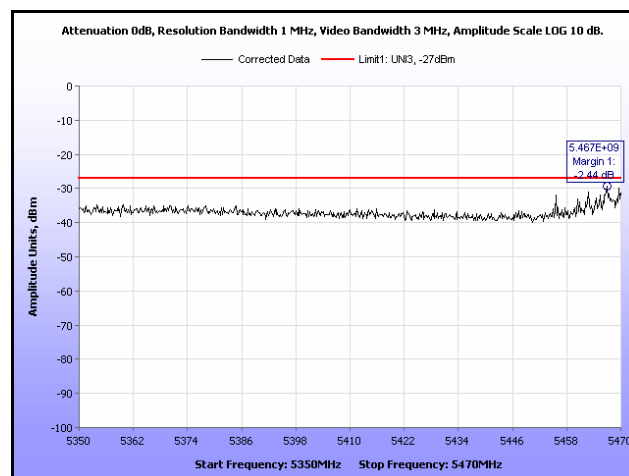
Plot 325. EIRP, 802.11n 20 MHz, 5500 MHz, Band Edge, Sector Antenna
