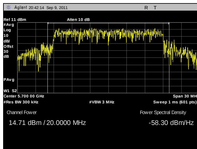
Plot 78. Conducted Output Power, 802.11n 20 MHz, Port A, 5700 MHz
