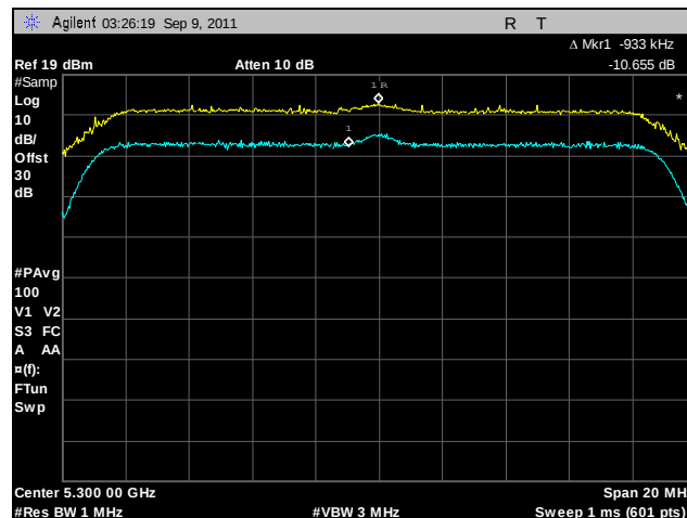
Plot 146. Peak Excursion, 802.11n 20 MHz, Port B, 5300 MHz
