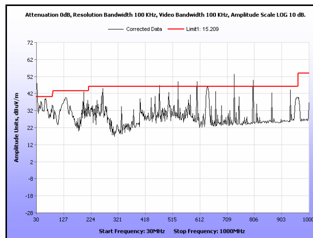
Plot 255. Radiated Spurious, 802.11a, 5700 MHz, 30 MHz – 1 GHz, Sector Antenna
