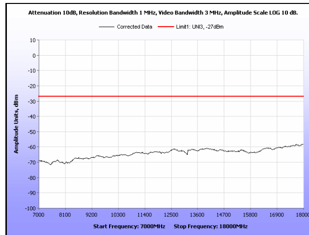
Plot 289. Radiated Spurious, 802.11n 40 MHz, 5300 MHz, 7 GHz – 18 GHz, Sector Antenna
