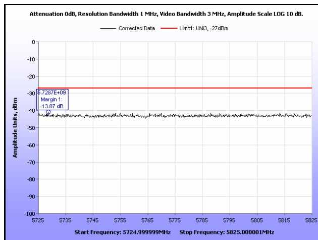
Plot 310. EIRP, 802.11a, 5700 MHz, Band Edge, Omni Antenna
