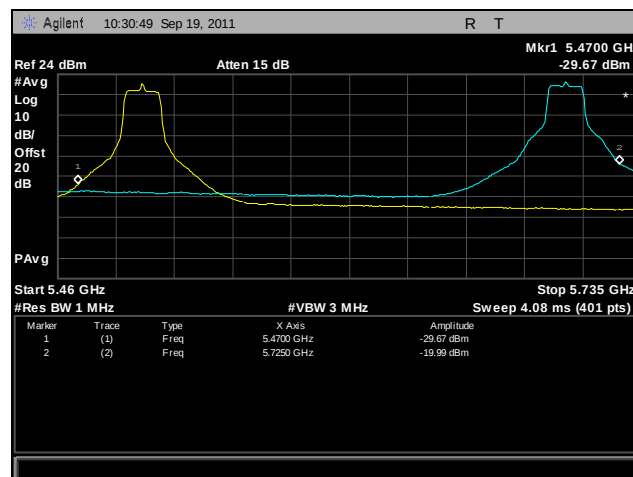
Plot 366. Frequency Stability, 802.11a, 5470 MHz – 5725 MHz @ -10°C, 120 V
