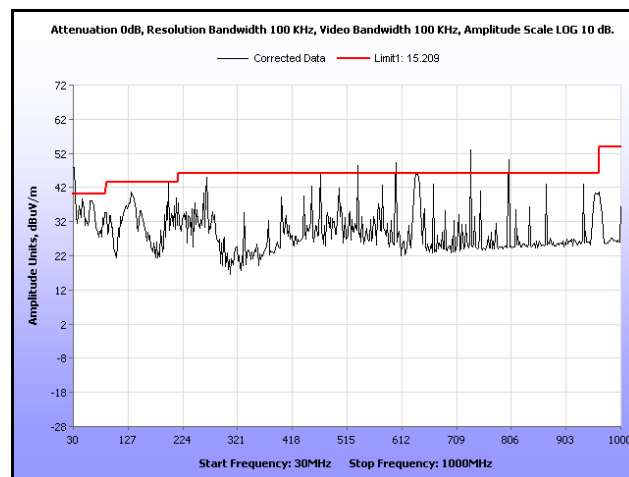
Plot 291. Radiated Spurious, 802.11n 40 MHz, 5310 MHz, 30 MHz – 1 GHz, Sector Antenna
