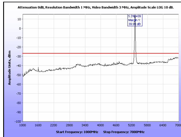
Plot 172. Radiated Spurious, 802.11a, 5320 MHz, 1 GHz – 7 GHz, Omni Antenna
