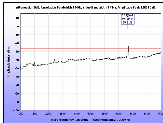
Plot 204. Radiated Spurious, 802.11n 20 MHz, 5580 MHz, 1 GHz – 7 GHz, Omni Antenna
