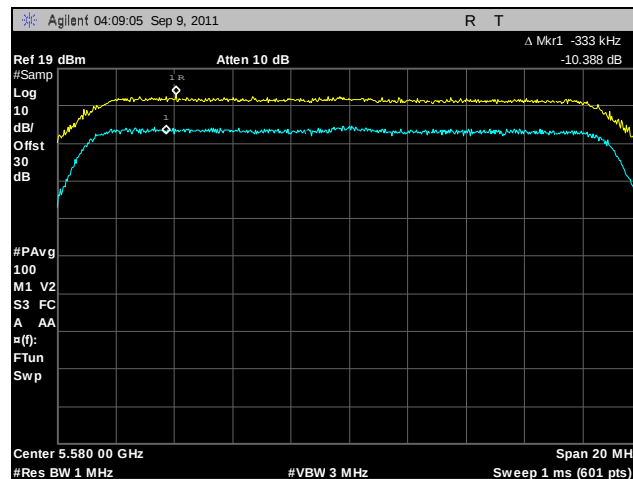
Plot 149. Peak Excursion, 802.11n 20 MHz, Port B, 5580 MHz
