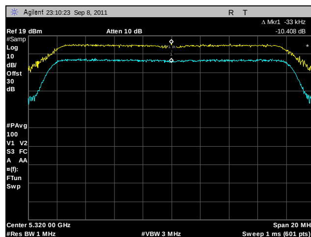
Plot 135. Peak Excursion, 802.11a, 5320 MHz
