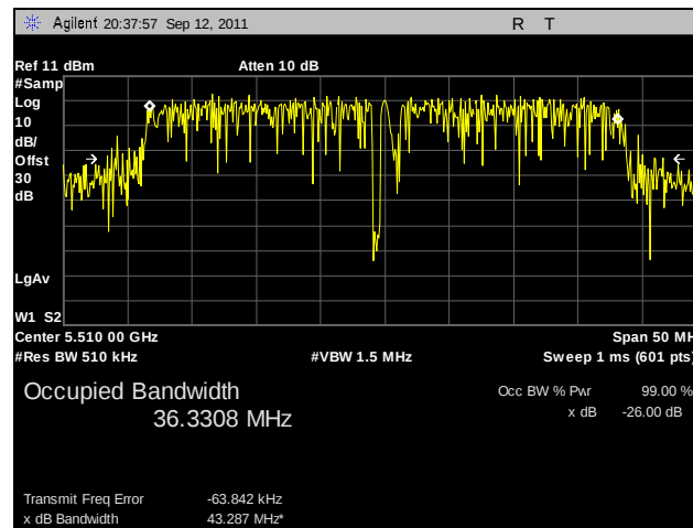
Plot 64. 99% Occupied Bandwidth, 802.11n 40 MHz, Port B, 5510 MHz
