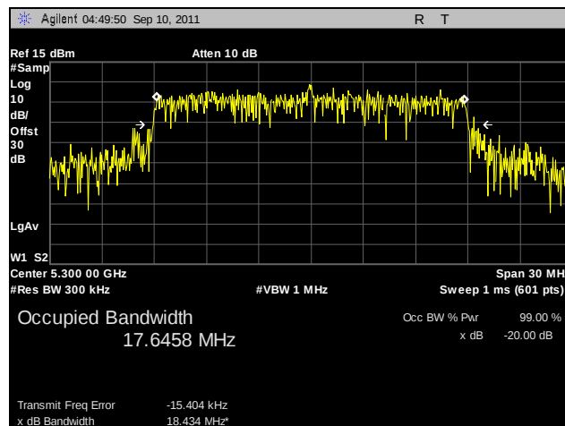
Plot 50. 99% Occupied Bandwidth, 802.11n 20 MHz, Port B, 5300 MHz
