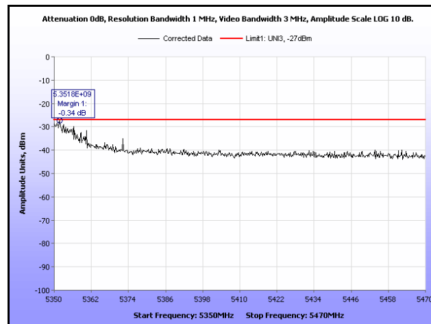
Plot 320. EIRP, 802.11a, 5320 MHz, Band Edge, Sector Antenna
