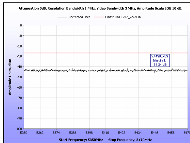
Plot 309. EIRP, 802.11a, 5500 MHz, Band Edge, Omni Antenna
