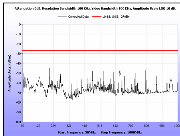
Plot 207. Radiated Spurious, 802.11n 20 MHz, 5700 MHz, 30 MHz – 1 GHz, Omni Antenna
