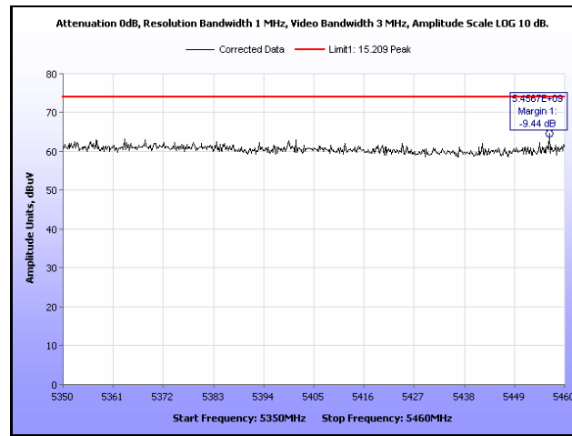
Plot 350. Restricted Band, 802.11n 20 MHz, 5500 MHz, Peak, Sector Antenna
