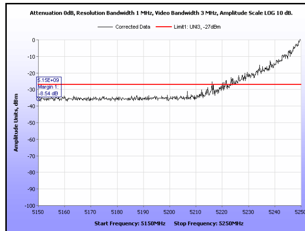
Plot 319. EIRP, 802.11a, 5260 MHz, Band Edge, Sector Antenna
