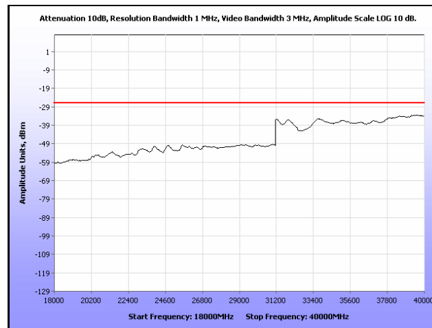
Plot 278. Radiated Spurious, 802.11n 20 MHz, 5580 MHz, 18 GHz – 40 GHz, Sector Antenna
