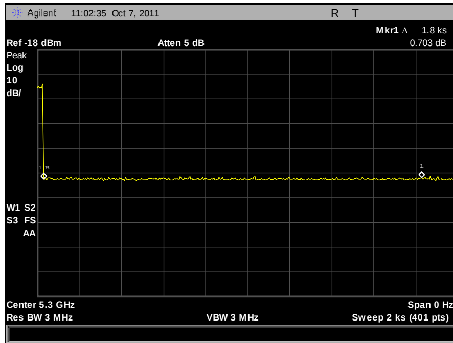
Plot 450. Non-Occupancy Period
