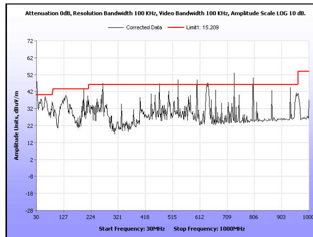
Plot 299. Radiated Spurious, 802.11n 40 MHz, 5580 MHz, 30 MHz – 1 GHz, Sector Antenna
