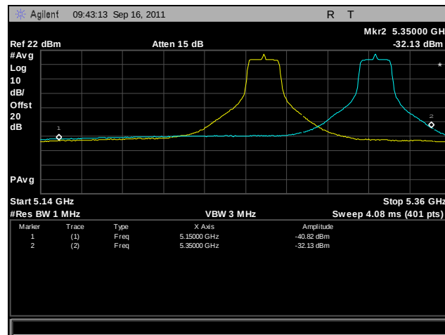
Plot 359. Frequency Stability, 802.11a, 5250 MHz – 5350 MHz @ 20°C, 120 V
