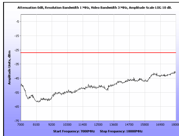
Plot 197. Radiated Spurious, 802.11n 20 MHz, 5320 MHz, 7 GHz – 18 GHz, Omni Antenna
