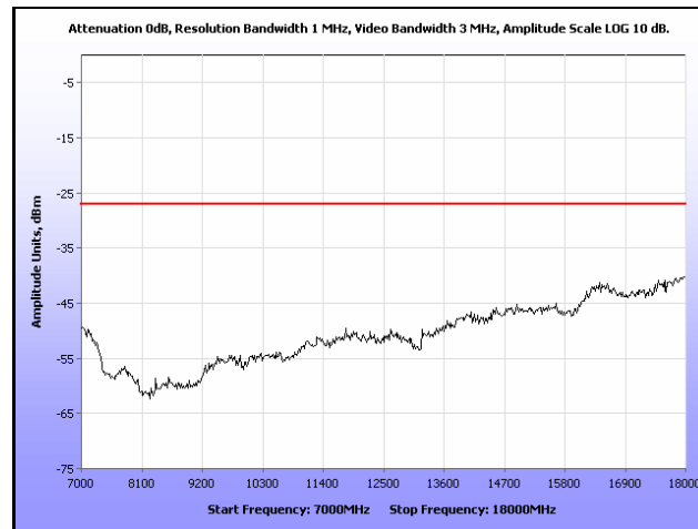
Plot 217. Radiated Spurious, 802.11n 40 MHz, 5300 MHz, 7 GHz – 18 GHz, Omni Antenna
