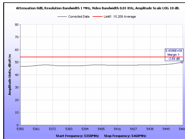
Plot 333. Restricted Band, 802.11a, 5500 MHz, Average, Omni Antenna
