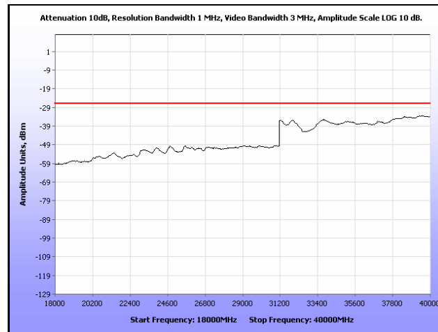
Plot 274. Radiated Spurious, 802.11n 20 MHz, 5500 MHz, 18 MHz – 40 GHz, Sector Antenna
