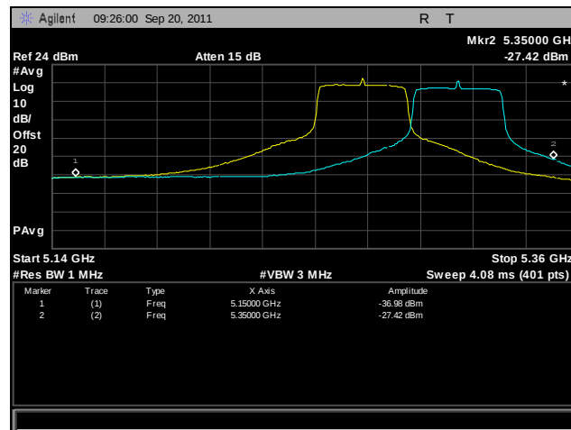
Plot 408. Frequency Stability, 802.11n 40 MHz, 5250 MHz – 5350 MHz @ 55°C, 120 V
