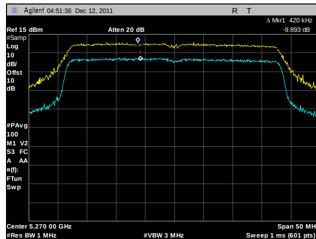
Plot 151. Peak Excursion, 802.11n 40 MHz, Port A, 5270 MHz
