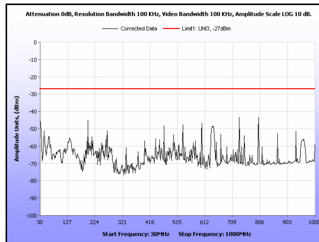
Plot 227. Radiated Spurious, 802.11n 40 MHz, 5580 MHz, 30 MHz – 1 GHz, Omni Antenna
