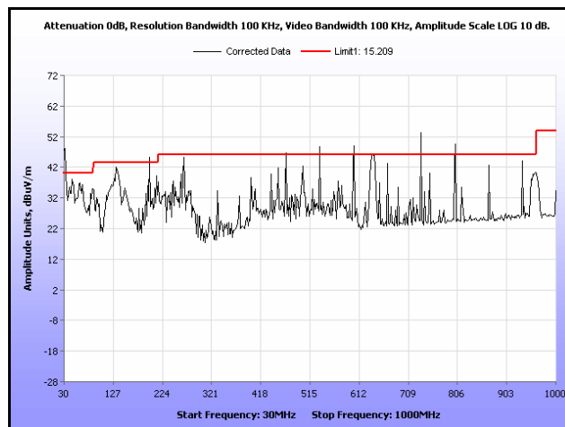
Plot 259. Radiated Spurious, 802.11n 20 MHz, 5260 MHz, 30 MHz – 1 GHz, Sector Antenna
