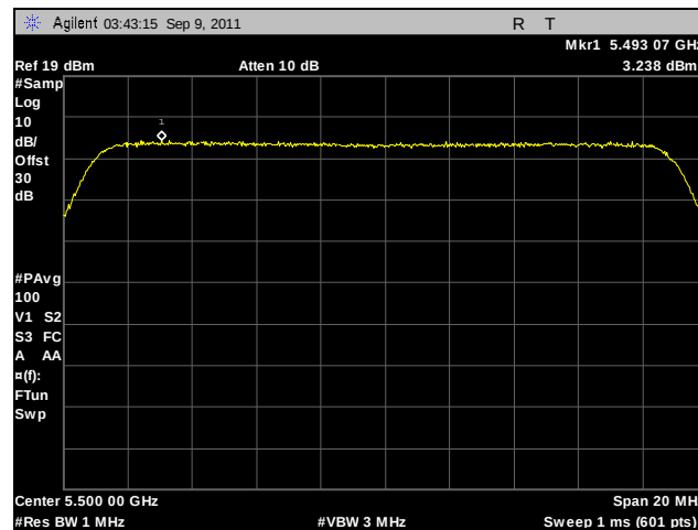
Plot 106. Peak Spectral Density, 802.11n 20 MHz, Port A, 5500 MHz
