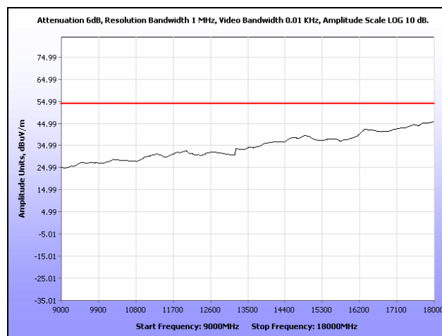
Plot 72. Radiated Spurious Emissions, Low Channel, 802.11a, Omni Antenna, 9 GHz – 18 GHz, Average
