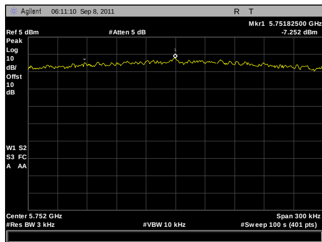
Plot 265. Peak Power Spectral Density, Low Channel, 802.11a, Port A
