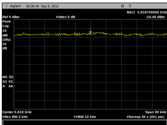
Plot 275. Peak Power Spectral Density, High Channel, 802.11a 20 MHz, Port A
