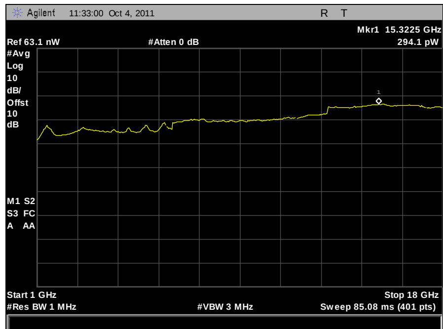
Plot 325. Receiver Spurious Emission, 1 GHz – 18 GHz, Port A
