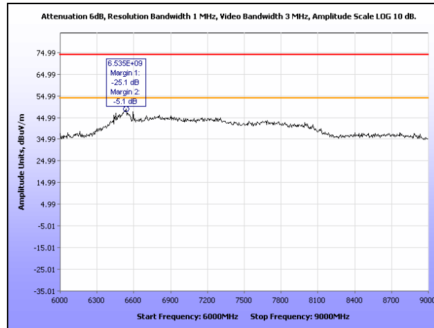
Plot 88. Radiated Spurious Emissions, High Channel, 802.11a, Omni Antenna, 6 GHz – 9 GHz
