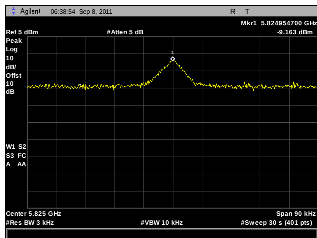
Plot 281. Peak Power Spectral Density, High Channel, 802.11a 20 MHz, Port B
