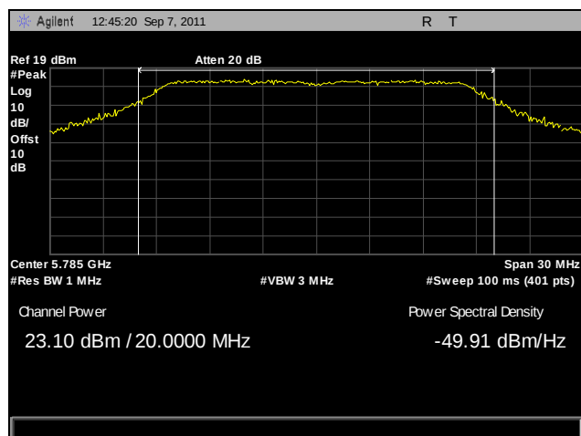
Plot 41. Peak Power Output, Mid Channel, 802.11n 20 MHz, Port A
