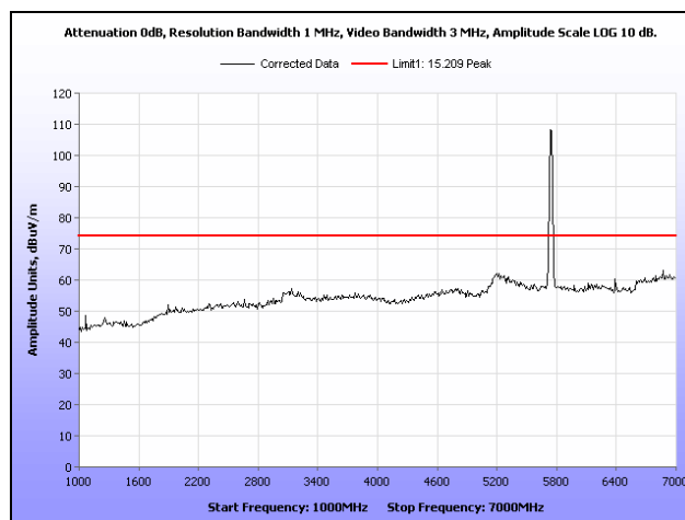
Plot 143. Radiated Spurious Emissions, Low Channel, 802.11a, Sector Antenna, 1 GHz – 7 GHz, Peak
