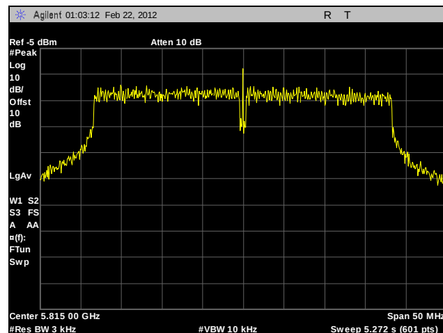
Plot 316. Peak Power Spectral Density, High Channel, 802.11a 40 MHz, Port A, Sector Antenna, Determination
