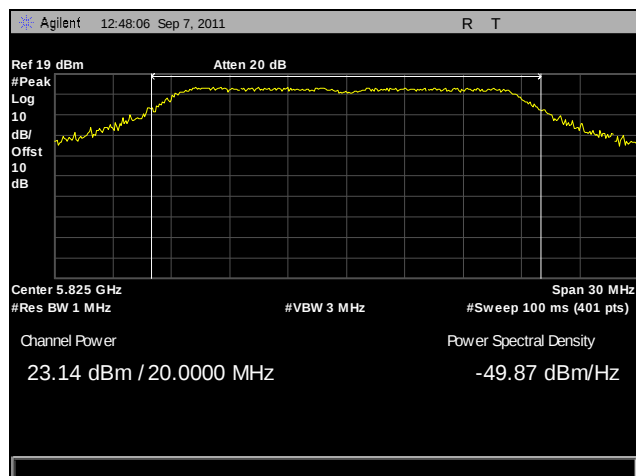
Plot 42. Peak Power Output, High Channel, 802.11n 20 MHz, Port A
