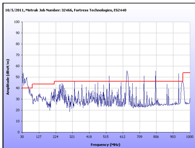
Plot 133. Radiated Spurious Emissions, High Channel, 802.11n 40 MHz, Omni Antenna, 30 MHz – 1 GHz Note: Emissions which exceed the limit are digital emissions.
