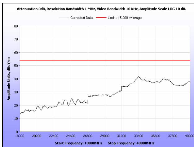
Plot 91. Radiated Spurious Emissions, High Channel, 802.11a, Omni Antenna, 18 GHz – 40 GHz, Average
