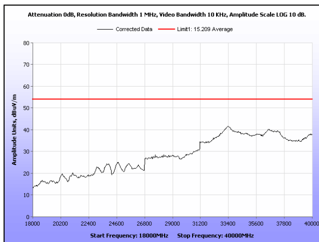
Plot 131. Radiated Spurious Emissions, Mid Channel, 802.11n 40 MHz, Omni Antenna, 18 GHz – 40 GHz, Average
