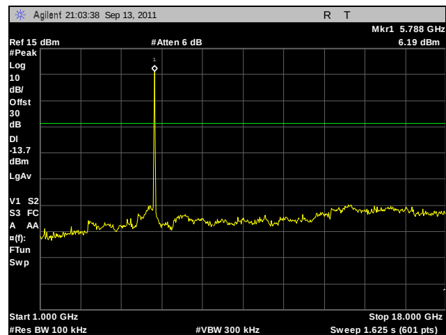
Plot 213. Conducted Spurious Emissions, Mid Channel, 802.11a, Port A, 1 GHz – 18 GHz
