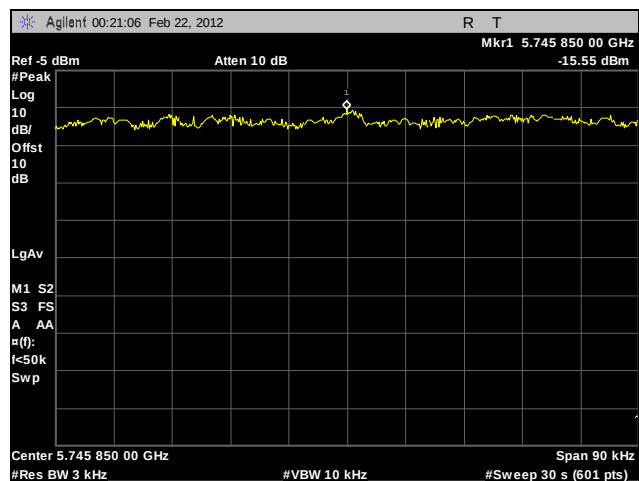
Plot 301. Peak Power Spectral Density, Low Channel, 802.11a 20 MHz, Port A, Sector Antenna
