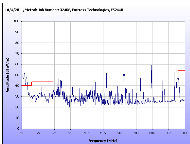
Plot 101. Radiated Spurious Emissions, Mid Channel, 802.11n 20 MHz, Omni Antenna, 30 MHz – 1 GHz Note: Emissions which exceed the limit are digital emissions.
