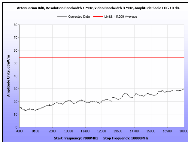
Plot 166. Radiated Spurious Emissions, Low Channel, 802.11n 20 MHz, Sector Antenna, 7 GHz – 18 GHz, Average
