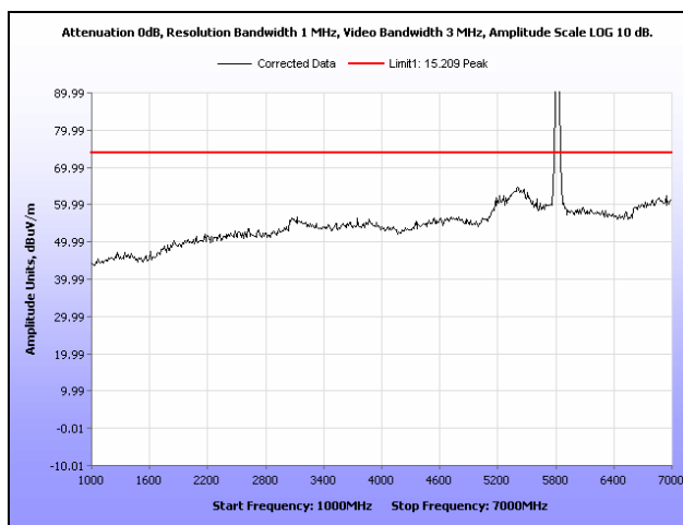
Plot 204. Radiated Spurious Emissions, High Channel, 802.11n 40 MHz, Sector Antenna, 1 GHz – 7 GHz, Peak
