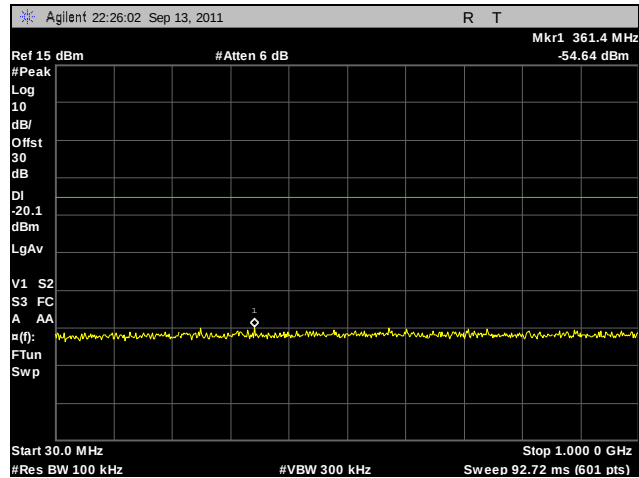
Plot 230. Conducted Spurious Emissions, Mid Channel, 802.11n 20 MHz, Port B, 30 MHz – 1 GHz
