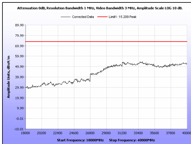
Plot 169. Radiated Spurious Emissions, Low Channel, 802.11n 20 MHz, Sector Antenna, 18 GHz – 40 GHz, Peak
