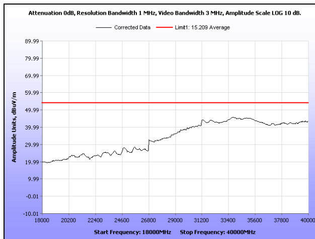
Plot 161. Radiated Spurious Emissions, High Channel, 802.11a, Sector Antenna, 18 GHz – 40 GHz, Average
