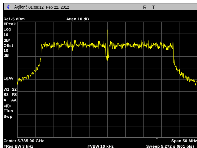
Plot 320. Peak Power Spectral Density, Mid Channel, 802.11a 40 MHz, Port B, Sector Antenna, Determination
