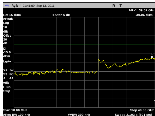
Plot 217. Conducted Spurious Emissions, High Channel, 802.11a, Port A, 18 GHz – 40 GHz
