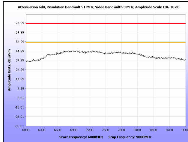
Plot 96. Radiated Spurious Emissions, Low Channel, 802.11n 20 MHz, Omni Antenna, 6 GHz – 9 GHz
