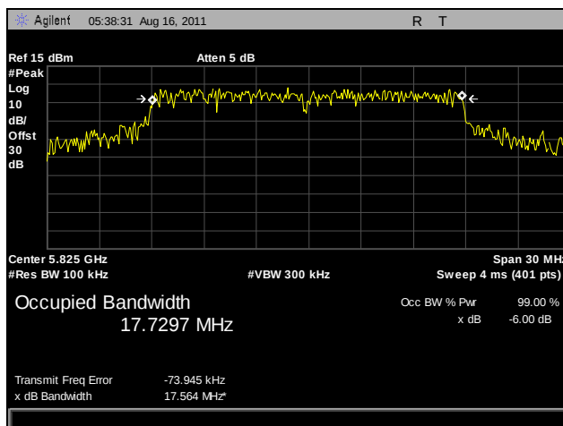
Plot 12. 6 dB Occupied Bandwidth, High Channel, 802.11n 20 MHz, Port A
