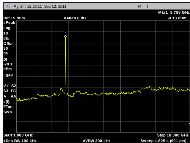
Plot 231. Conducted Spurious Emissions, Mid Channel, 802.11n 20 MHz, Port B, 1 GHz – 18 GHz
