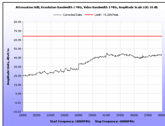
Plot 176. Radiated Spurious Emissions, Mid Channel, 802.11n 20 MHz, Sector Antenna, 18 GHz – 40 GHz, Peak
