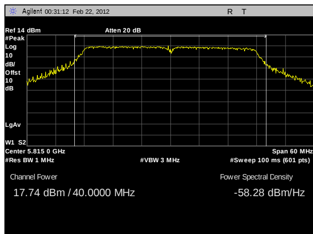
Plot 63. Peak Power Output, High Channel, 802.11n 40 MHz, Port A, Sector Antenna
