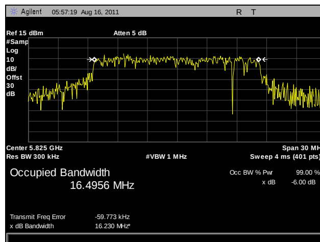
Plot 24. 99% Occupied Bandwidth, High Channel, 802.11a, Port B
