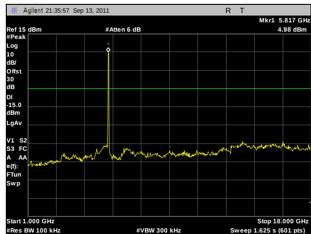
Plot 216. Conducted Spurious Emissions, High Channel, 802.11a, Port A, 1 GHz – 18 GHz
