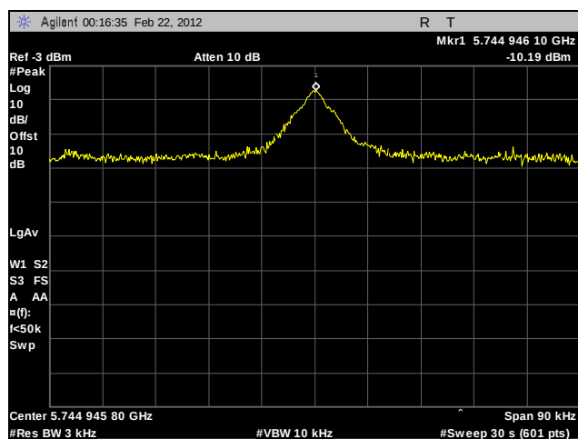
Plot 307. Peak Power Spectral Density, Low Channel, 802.11a 20 MHz, Port B, Sector Antenna
