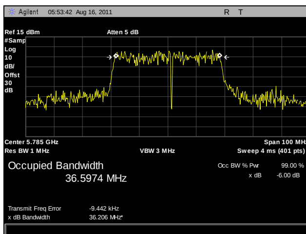
Plot 35. 99% Occupied Bandwidth, Mid Channel, 802.11n 40 MHz, Port B
