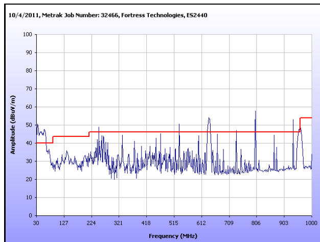
Plot 193. Radiated Spurious Emissions, Mid Channel, 802.11n 40 MHz, Sector Antenna, 30 MHz – 1 GHz Note: Emissions which exceed the limit are digital emissions.
