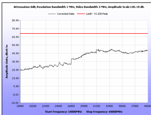
Plot 208. Radiated Spurious Emissions, High Channel, 802.11n 40 MHz, Sector Antenna, 18 GHz – 40 GHz, Peak
