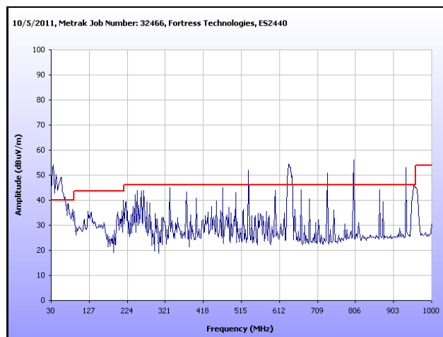
Plot 117. Radiated Spurious Emissions, Low Channel, 802.11n 40 MHz, Omni Antenna, 30 MHz – 1 GHz Note: Emissions which exceed the limit are digital emissions.
