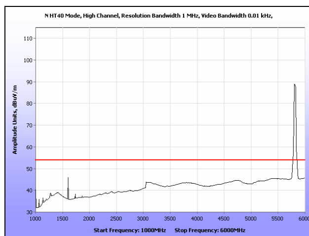
Plot 134. Radiated Spurious Emissions, High Channel, 802.11n 40 MHz, Omni Antenna, 1 GHz – 6 GHz, Average
