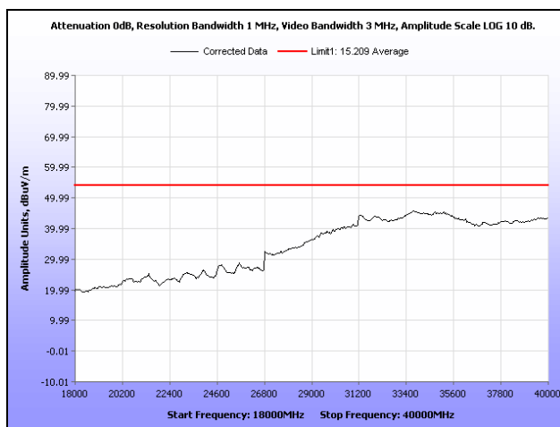
Plot 168. Radiated Spurious Emissions, Low Channel, 802.11n 20 MHz, Sector Antenna, 18 GHz – 40 GHz, Average
