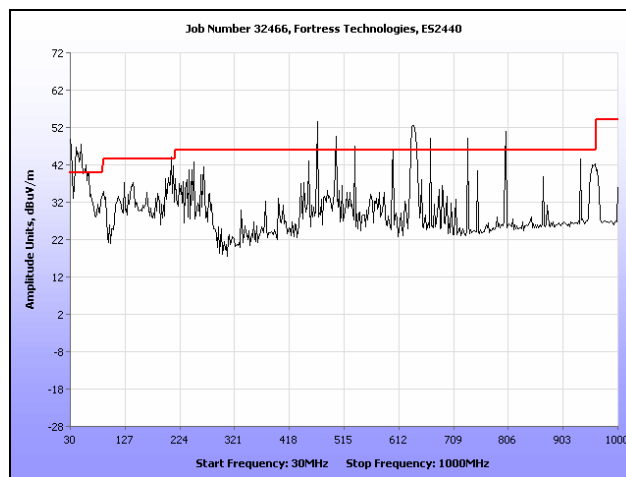
Plot 141. Radiated Spurious Emissions, Low Channel, 802.11a, Sector Antenna, 30 MHz – 1 GHz Note: Emissions which exceed the limit are digital emissions.
