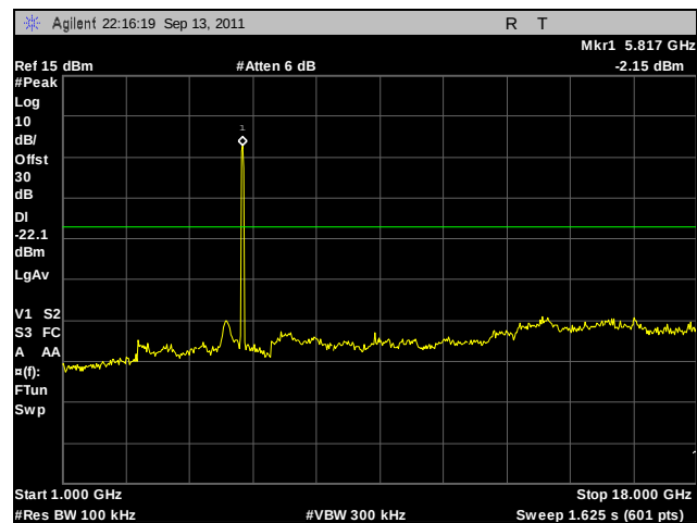
Plot 252. Conducted Spurious Emissions, High Channel, 802.11n 40 MHz, Port B, 1 GHz – 18 GHz
