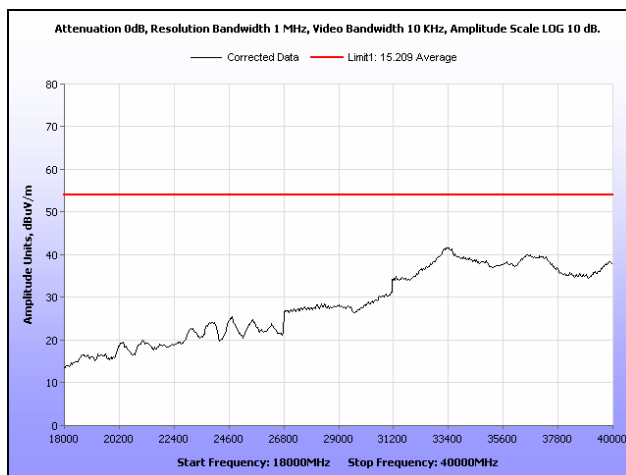
Plot 123. Radiated Spurious Emissions, Low Channel, 802.11n 40 MHz, Omni Antenna, 18 GHz – 40 GHz, Average
