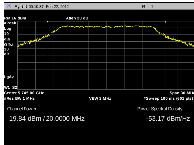
Plot 52. Peak Power Output, Low Channel, 802.11a, Port A, Sector Antenna
