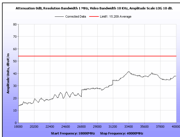
Plot 139. Radiated Spurious Emissions, High Channel, 802.11n 40 MHz, Omni Antenna, 18 GHz – 40 GHz, Average
