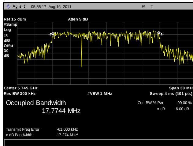
Plot 28. 99% Occupied Bandwidth, Low Channel, 802.11n 20 MHz, Port B
