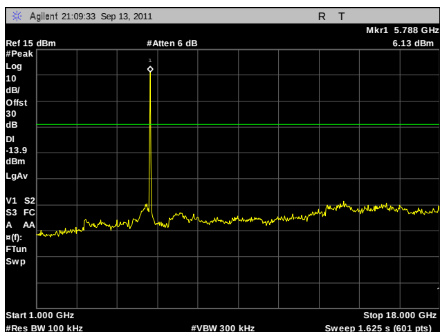
Plot 222. Conducted Spurious Emissions, Mid Channel, 802.11n 20 MHz, Port A, 1 GHz – 18 GHz
