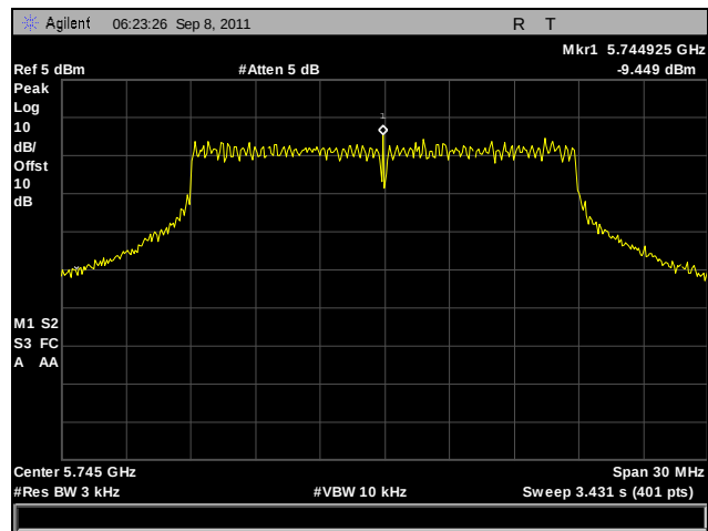
Plot 270. Peak Power Spectral Density, Low Channel, 802.11a 20 MHz, Port A, Determination
