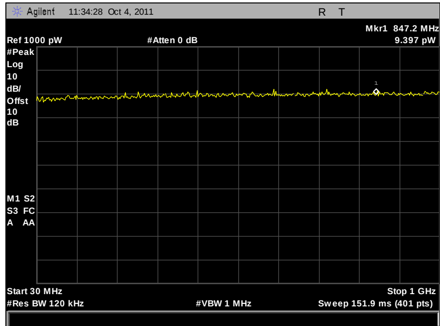
Plot 324. Receiver Spurious Emission, 30 MHz – 1 GHz, Port A
