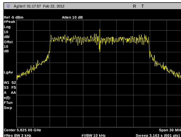
Plot 310. Peak Power Spectral Density, High Channel, 802.11a 20 MHz, Port B, Sector Antenna, Determination
