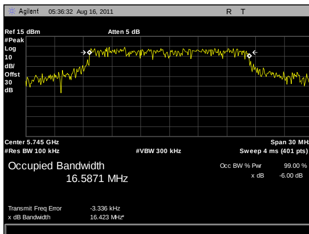
Plot 7. 6 dB Occupied Bandwidth, Low Channel, 802.11a, Port A
