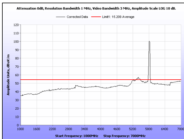
Plot 202. Radiated Spurious Emissions, High Channel, 802.11n 40 MHz, Sector Antenna, 1 GHz – 7 GHz, Average
