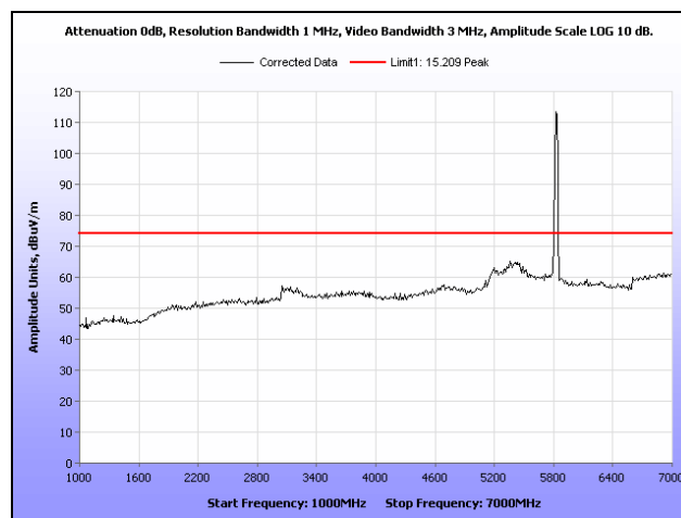
Plot 180. Radiated Spurious Emissions, High Channel, 802.11n 20 MHz, Sector Antenna, 1 GHz – 7 GHz, Peak
