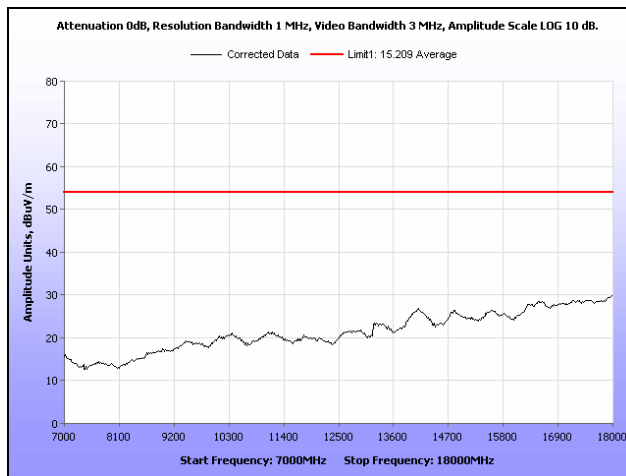
Plot 205. Radiated Spurious Emissions, High Channel, 802.11n 40 MHz, Sector Antenna, 7 GHz – 18 GHz, Average
