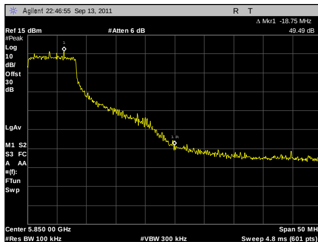
Plot 255. Conducted Band Edge, High Channel, 802.11a, Port A
