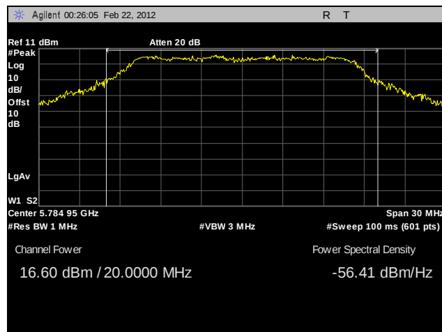
Plot 59. Peak Power Output, Mid Channel, 802.11n 20 MHz, Port B, Sector Antenna
