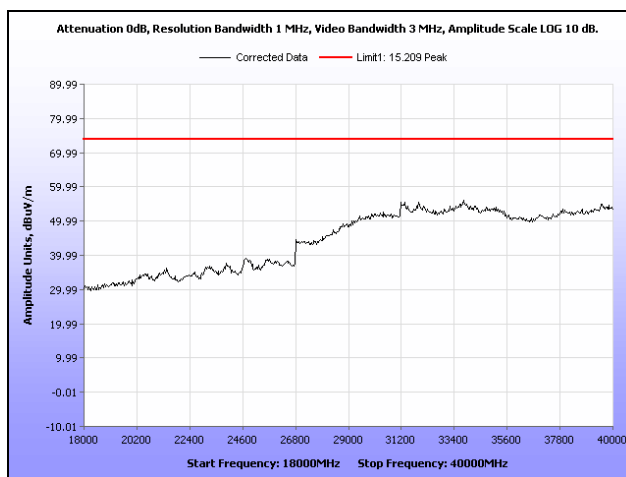
Plot 155. Radiated Spurious Emissions, Mid Channel, 802.11a, Sector Antenna, 18 GHz – 40 GHz, Peak
