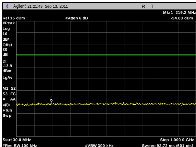
Plot 221. Conducted Spurious Emissions, Mid Channel, 802.11n 20 MHz, Port A, 30 MHz – 1 GHz
