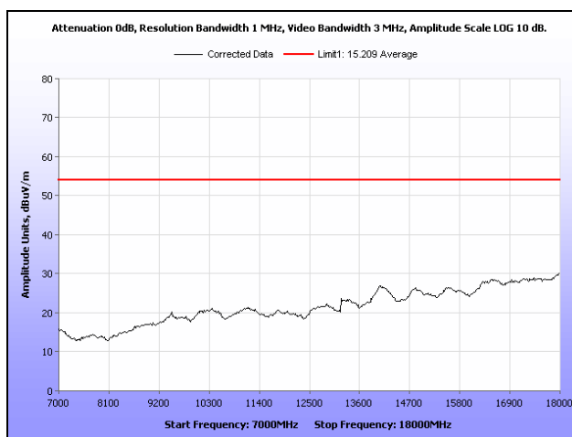
Plot 189. Radiated Spurious Emissions, Low Channel, 802.11n 40 MHz, Sector Antenna, 7 GHz – 18 GHz, Average
