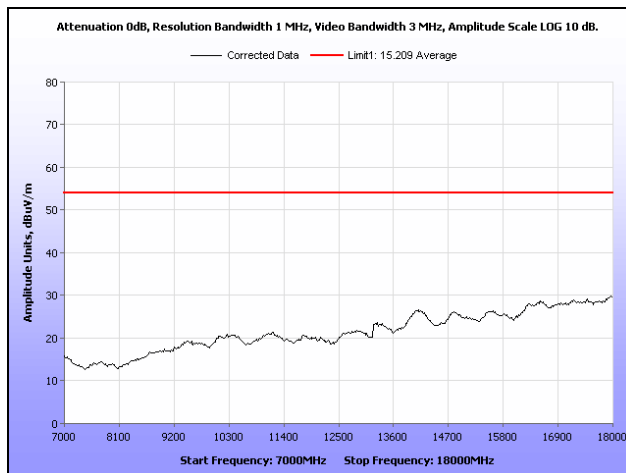
Plot 181. Radiated Spurious Emissions, High Channel, 802.11n 20 MHz, Sector Antenna, 7 GHz – 18 GHz, Average
