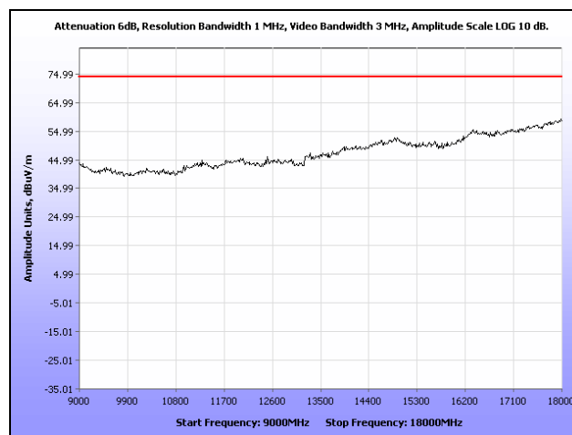
Plot 90. Radiated Spurious Emissions, High Channel, 802.11a, Omni Antenna, 9 GHz – 18 GHz, Peak
