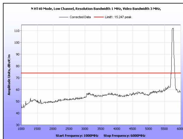
Plot 119. Radiated Spurious Emissions, Low Channel, 802.11n 40 MHz, Omni Antenna, 1 GHz – 6 GHz, Peak
