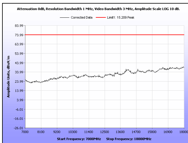
Plot 145. Radiated Spurious Emissions, Low Channel, 802.11a, Sector Antenna, 7 GHz – 18 GHz, Peak
