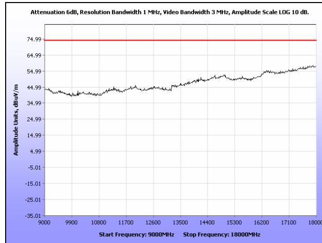
Plot 73. Radiated Spurious Emissions, Low Channel, 802.11a, Omni Antenna, 9 GHz – 18 GHz, Peak
