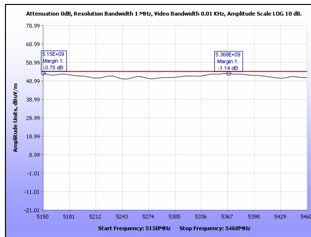
Plot 179. Radiated Spurious Emissions, High Channel, 802.11n 20 MHz, Sector Antenna, Smaller Span
