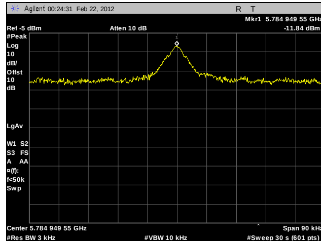
Plot 309. Peak Power Spectral Density, Mid Channel, 802.11a 20 MHz, Port B, Sector Antenna
