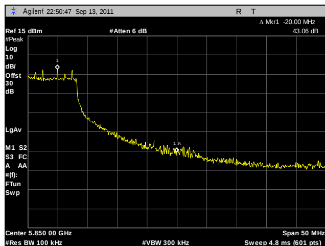
Plot 263. Conducted Band Edge, High Channel, 802.11n 40 MHz, Port B
