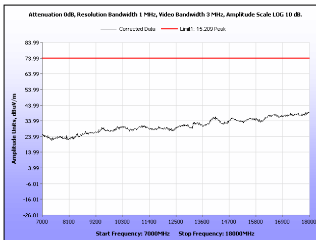
Plot 206. Radiated Spurious Emissions, High Channel, 802.11n 40 MHz, Sector Antenna, 7 GHz – 18 GHz, Peak
