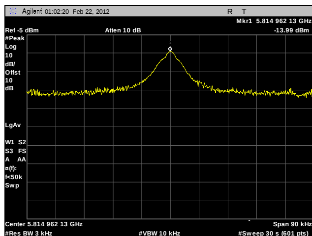
Plot 323. Peak Power Spectral Density, High Channel, 802.11a 40 MHz, Port B, Sector Antenna
