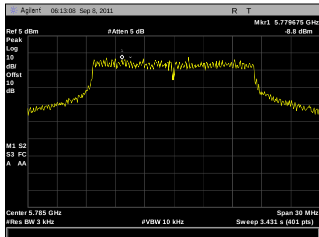
Plot 266. Peak Power Spectral Density, Mid Channel, 802.11a, Port A, Determination
