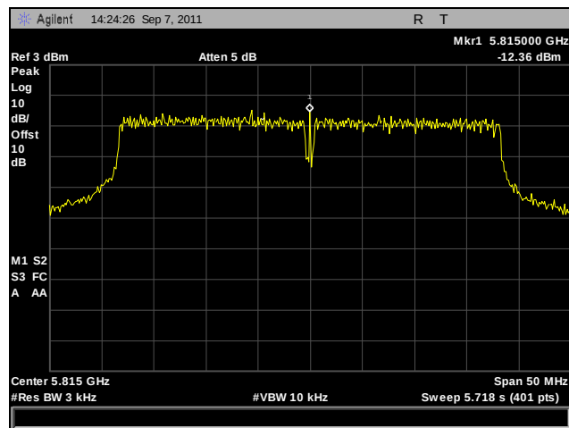
Plot 286. Peak Power Spectral Density, High Channel, 802.11a 40 MHz, Port A, Determination
