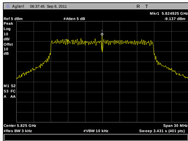
Plot 280. Peak Power Spectral Density, High Channel, 802.11a 20 MHz, Port B, Determination
