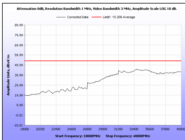
Plot 207. Radiated Spurious Emissions, High Channel, 802.11n 40 MHz, Sector Antenna, 18 GHz – 40 GHz, Average
