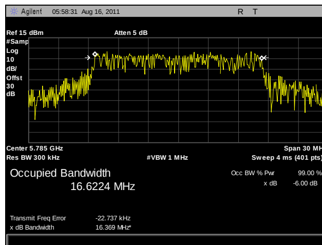
Plot 23. 99% Occupied Bandwidth, Mid Channel, 802.11a, Port B
