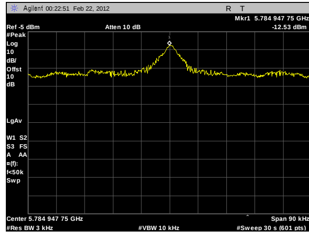
Plot 303. Peak Power Spectral Density, Mid Channel, 802.11a 20 MHz, Port A, Sector Antenna
