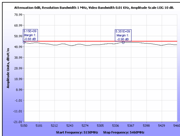
Plot 150. Radiated Spurious Emissions, Mid Channel, 802.11a, Sector Antenna, Smaller Span
