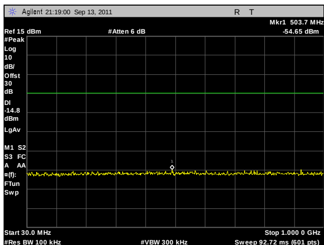
Plot 236. Conducted Spurious Emissions, Low Channel, 802.11n 40 MHz, Port A, 30 MHz – 1 GHz
