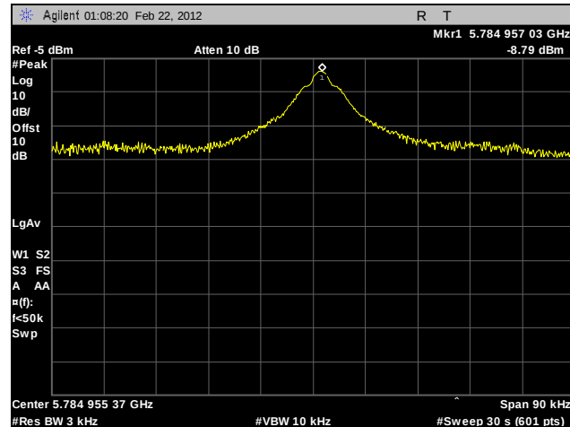
Plot 315. Peak Power Spectral Density, Mid Channel, 802.11a 40 MHz, Port A, Sector Antenna
