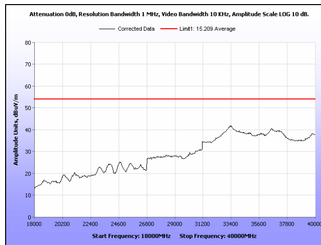
Plot 83. Radiated Spurious Emissions, Mid Channel, 802.11a, Omni Antenna, 18 GHz – 40 GHz, Average
