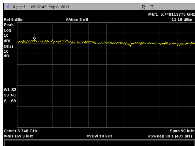
Plot 277. Peak Power Spectral Density, Low Channel, 802.11a 20 MHz, Port B
