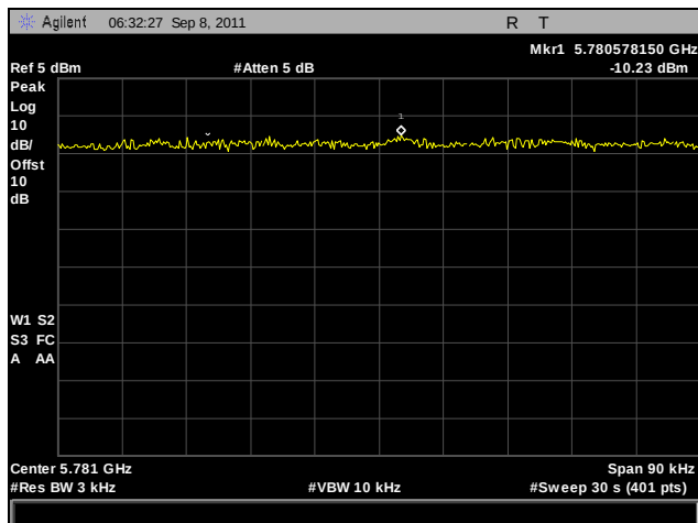
Plot 273. Peak Power Spectral Density, Mid Channel, 802.11a 20 MHz, Port A
