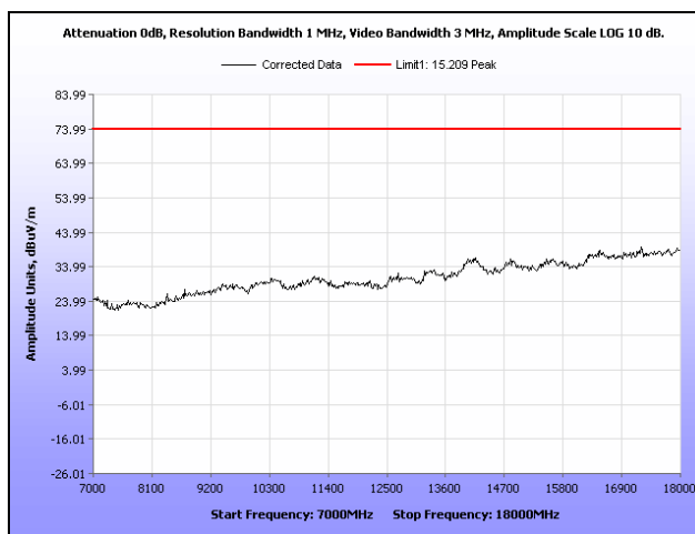
Plot 182. Radiated Spurious Emissions, High Channel, 802.11n 20 MHz, Sector Antenna, 7 GHz – 18 GHz, Peak
