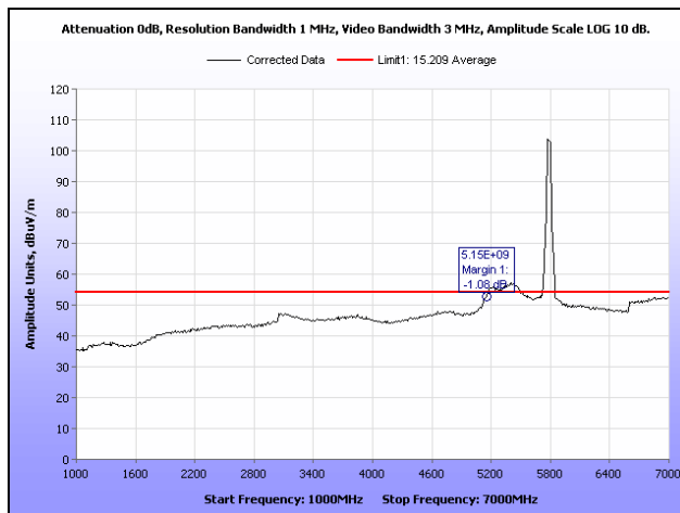
Plot 194. Radiated Spurious Emissions, Mid Channel, 802.11n 40 MHz, Sector Antenna, 1 GHz – 7 GHz, Average
