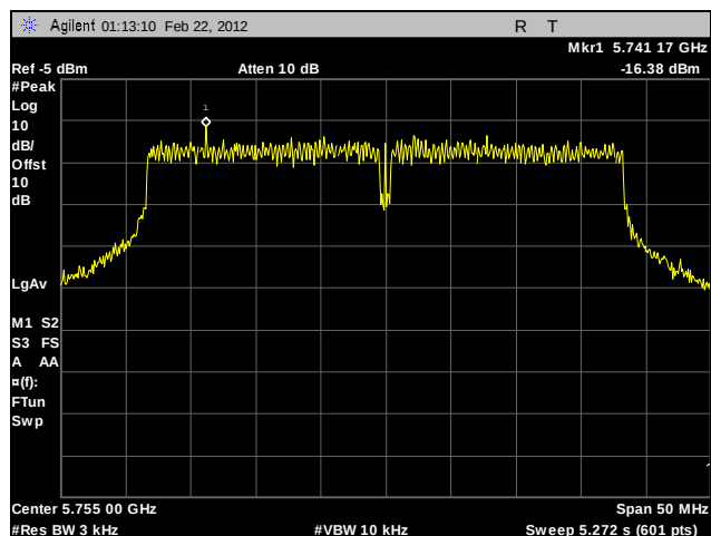
Plot 312. Peak Power Spectral Density, Low Channel, 802.11a 40 MHz, Port A, Sector Antenna, Determination
