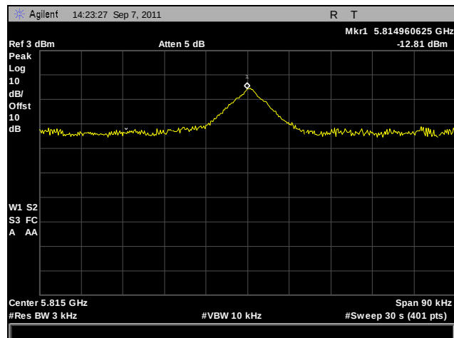
Plot 293. Peak Power Spectral Density, High Channel, 802.11a 40 MHz, Port B
