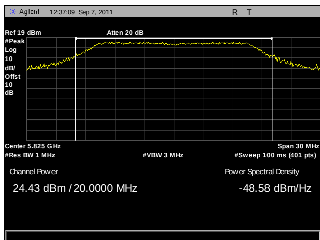
Plot 39. Peak Power Output, High Channel, 802.11a, Port A
