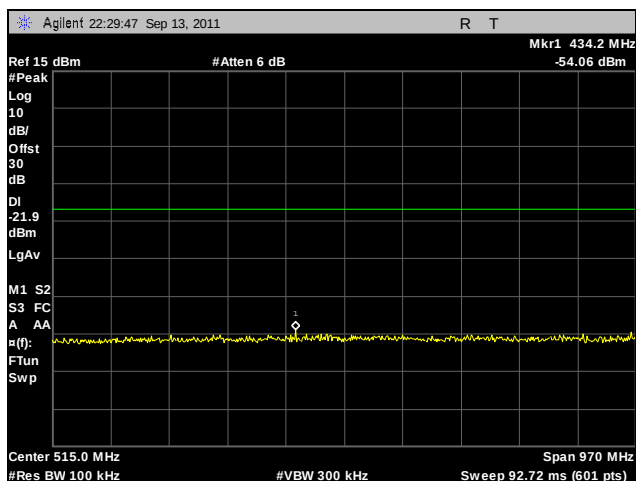
Plot 227. Conducted Spurious Emissions, Low Channel, 802.11n 20 MHz, Port B, 30 MHz – 1 GHz
