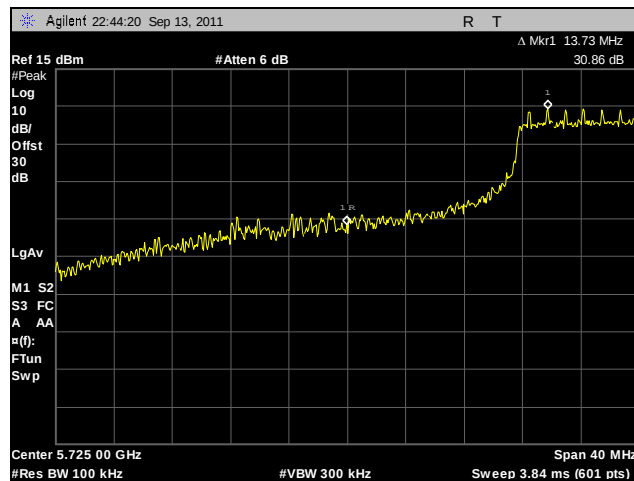
Plot 260. Conducted Band Edge, Low Channel, 802.11n 40 MHz, Port A
