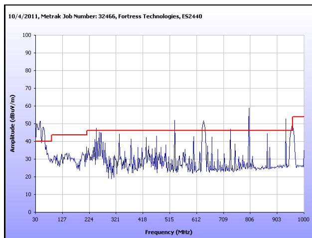
Plot 67. Radiated Spurious Emissions, Low Channel, 802.11a, Omni Antenna, 30 MHz – 1 GHz
