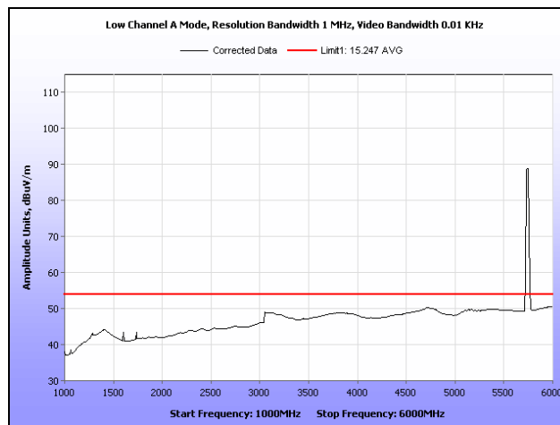
Plot 68. Radiated Spurious Emissions, Low Channel, 802.11a, Omni Antenna, 1 GHz – 6 GHz, Average
