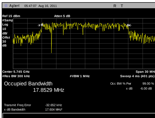
Plot 25. 99% Occupied Bandwidth, Low Channel, 802.11n 20 MHz, Port A
