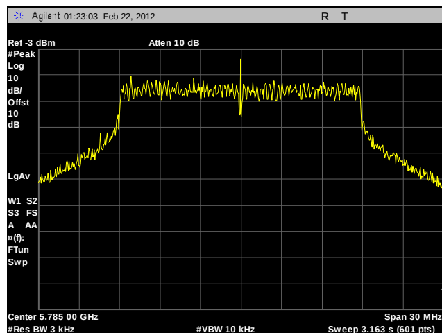
Plot 296. Peak Power Spectral Density, Mid Channel, 802.11a, Port A, Sector Antenna, Determination
