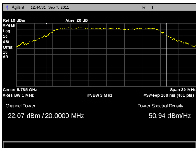
Plot 44. Peak Power Output, Mid Channel, 802.11n 20 MHz, Port B
