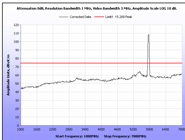
Plot 188. Radiated Spurious Emissions, Low Channel, 802.11n 40 MHz, Sector Antenna, 1 GHz – 7 GHz, Peak
