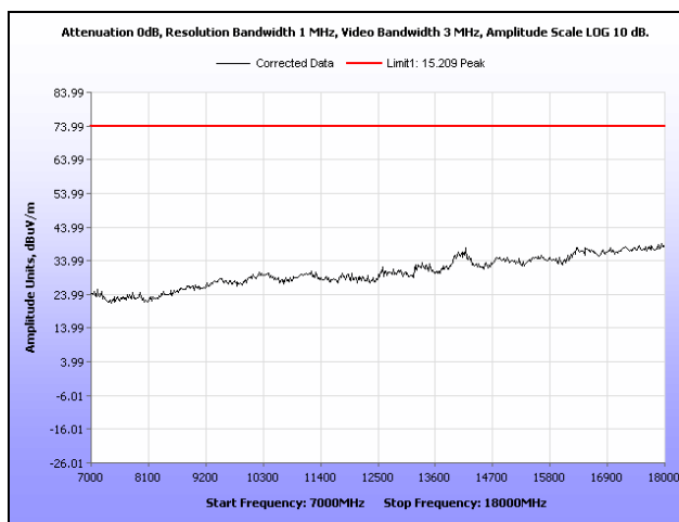
Plot 160. Radiated Spurious Emissions, High Channel, 802.11a, Sector Antenna, 7 GHz – 18 GHz, Peak
