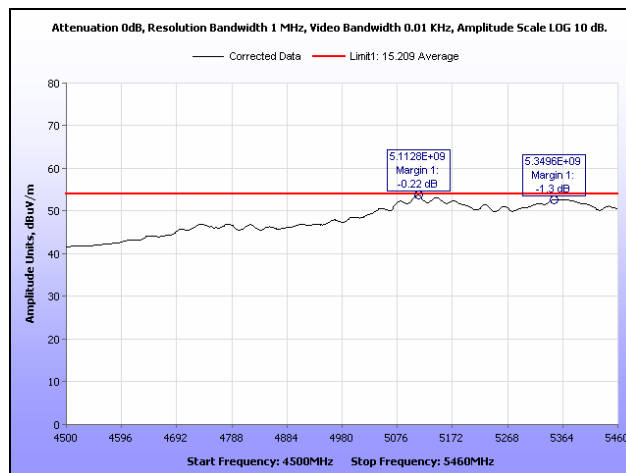
Plot 187. Radiated Spurious Emissions, Low Channel, 802.11n 40 MHz, Sector Antenna, Smaller Span
