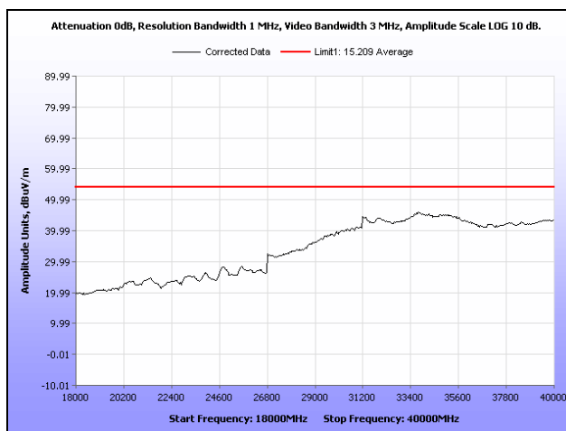
Plot 199. Radiated Spurious Emissions, Mid Channel, 802.11n 40 MHz, Sector Antenna, 18 GHz – 40 GHz, Average
