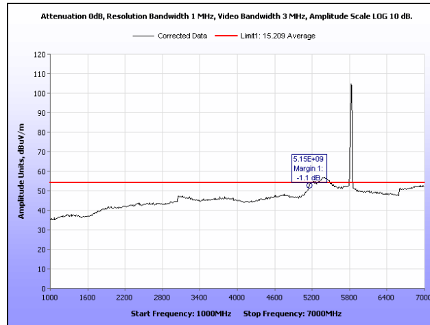
Plot 178. Radiated Spurious Emissions, High Channel, 802.11n 20 MHz, Sector Antenna, 1 GHz – 7 GHz, Average
