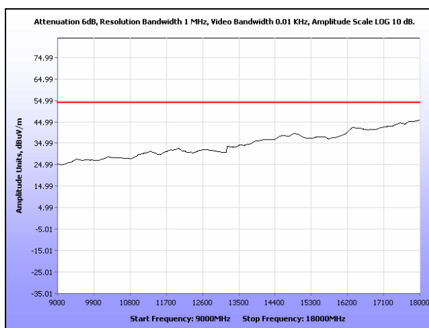
Plot 113. Radiated Spurious Emissions, High Channel, 802.11n 20 MHz, Omni Antenna, 9 GHz – 18 GHz, Average
