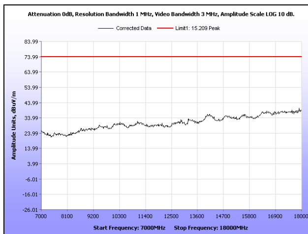
Plot 190. Radiated Spurious Emissions, Low Channel, 802.11n 40 MHz, Sector Antenna, 7 GHz – 18 GHz, Peak
