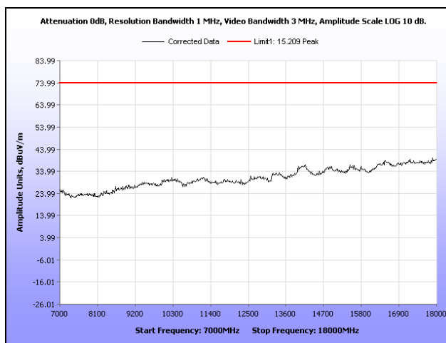
Plot 198. Radiated Spurious Emissions, Mid Channel, 802.11n 40 MHz, Sector Antenna, 7 GHz – 18 GHz, Peak
