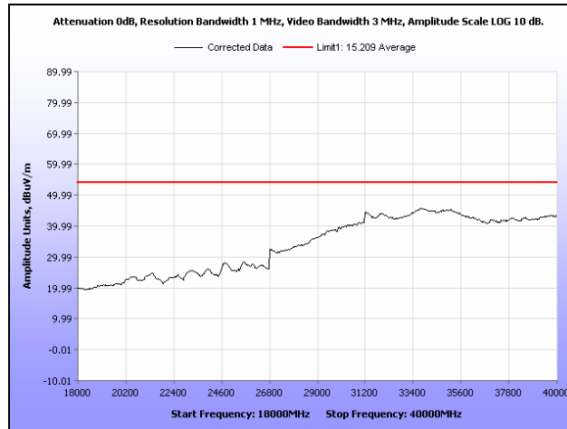
Plot 191. Radiated Spurious Emissions, Low Channel, 802.11n 40 MHz, Sector Antenna, 18 GHz – 40 GHz, Average
