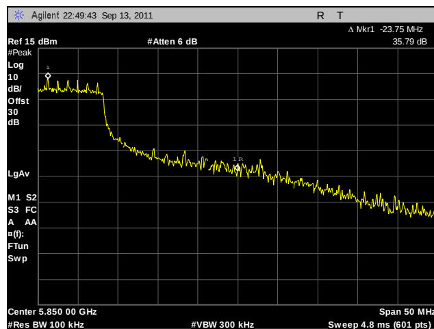
Plot 261. Conducted Band Edge, High Channel, 802.11n 40 MHz, Port A
