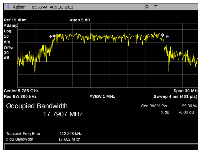
Plot 29. 99% Occupied Bandwidth, Mid Channel, 802.11n 20 MHz, Port B
