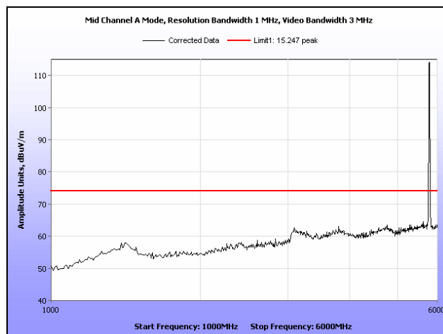
Plot 78. Radiated Spurious Emissions, Mid Channel, 802.11a, Omni Antenna, 1 GHz – 6 GHz, Peak
