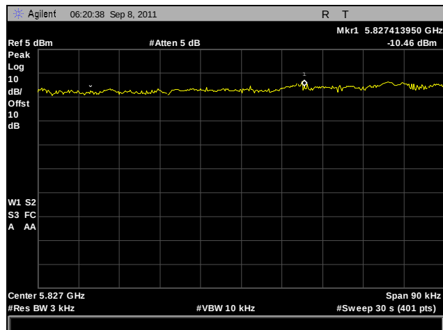
Plot 269. Peak Power Spectral Density, High Channel, 802.11a, Port A
