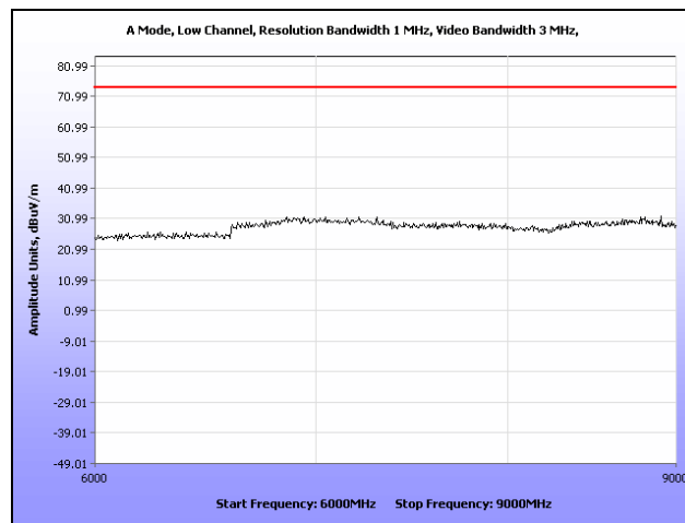
Plot 71. Radiated Spurious Emissions, Low Channel, 802.11a, Omni Antenna, 6 GHz – 9 GHz, Peak
