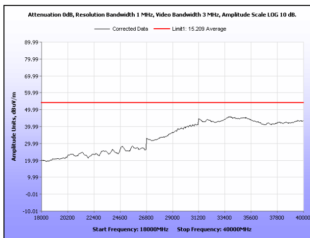
Plot 154. Radiated Spurious Emissions, Mid Channel, 802.11a, Sector Antenna, 18 GHz – 40 GHz, Average
