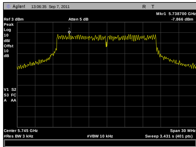
Plot 264. Peak Power Spectral Density, Low Channel, 802.11a, Port A, Determination
