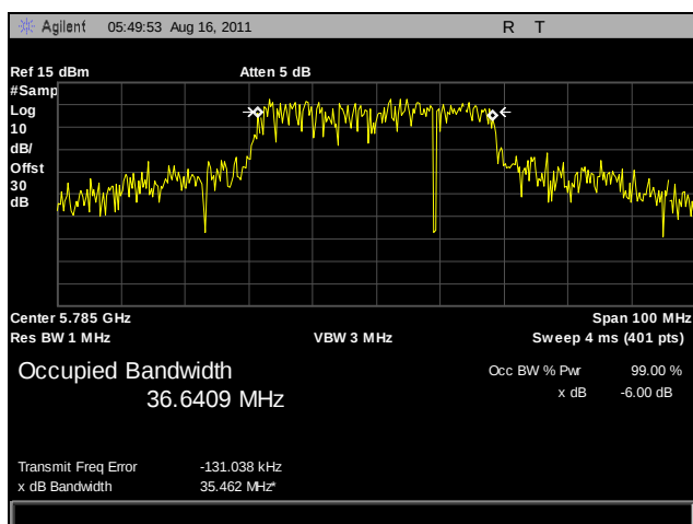
Plot 32. 99% Occupied Bandwidth, Mid Channel, 802.11n 40 MHz, Port A
