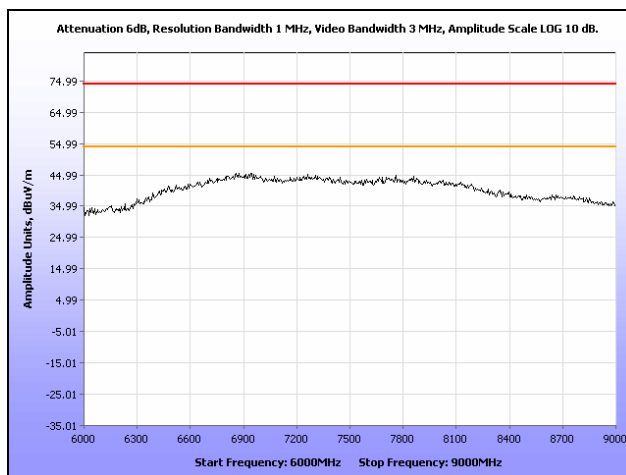
Plot 120. Radiated Spurious Emissions, Low Channel, 802.11n 40 MHz, Omni Antenna, 6 GHz – 9 GHz
