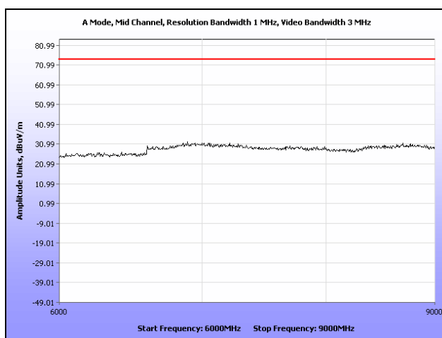
Plot 80. Radiated Spurious Emissions, Mid Channel, 802.11a, Omni Antenna, 6 GHz – 9 GHz, Peak
