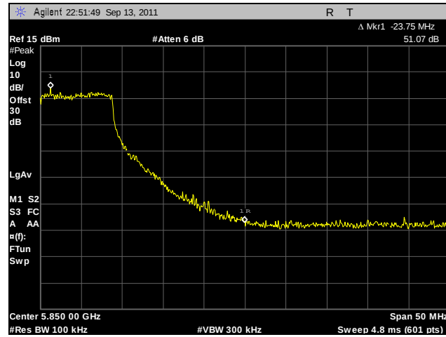
Plot 259. Conducted Band Edge, High Channel, 802.11n 20 MHz, Port B
