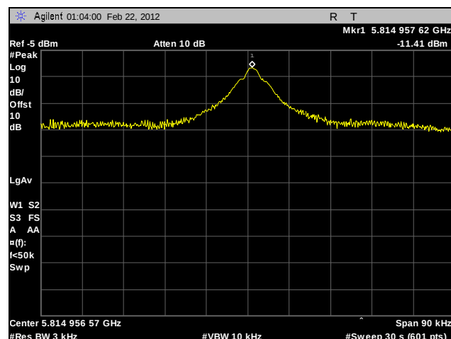
Plot 317. Peak Power Spectral Density, High Channel, 802.11a 40 MHz, Port A, Sector Antenna
