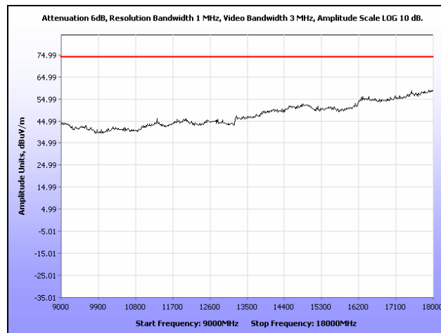
Plot 98. Radiated Spurious Emissions, Low Channel, 802.11n 20 MHz, Omni Antenna, 9 GHz – 18 GHz, Peak
