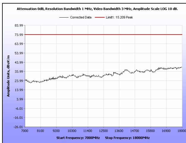
Plot 167. Radiated Spurious Emissions, Low Channel, 802.11n 20 MHz, Sector Antenna, 7 GHz – 18 GHz, Peak
