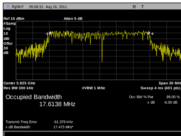
Plot 30. 99% Occupied Bandwidth, High Channel, 802.11n 20 MHz, Port B
