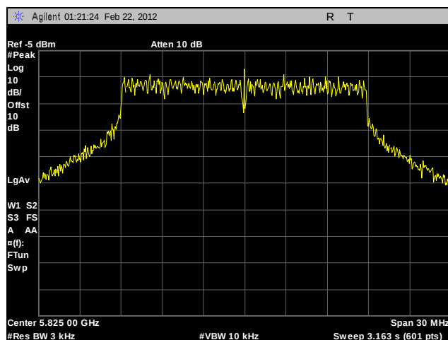
Plot 298. Peak Power Spectral Density, High Channel, 802.11a, Port A, Sector Antenna, Determination
