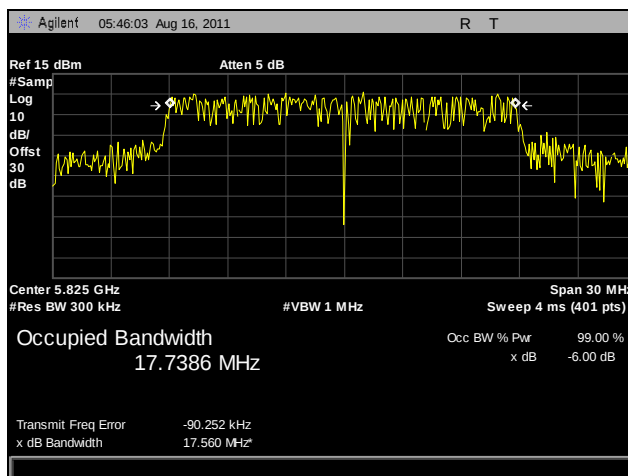
Plot 27. 99% Occupied Bandwidth, High Channel, 802.11n 20 MHz, Port A
