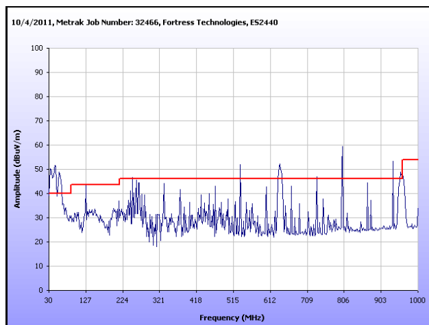
Plot 85. Radiated Spurious Emissions, High Channel, 802.11a, Omni Antenna, 30 MHz – 1 GHz
