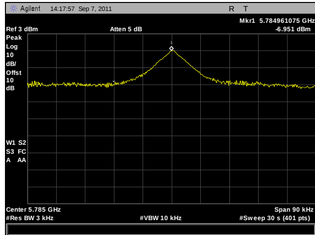
Plot 285. Peak Power Spectral Density, Mid Channel, 802.11a 40 MHz, Port A
