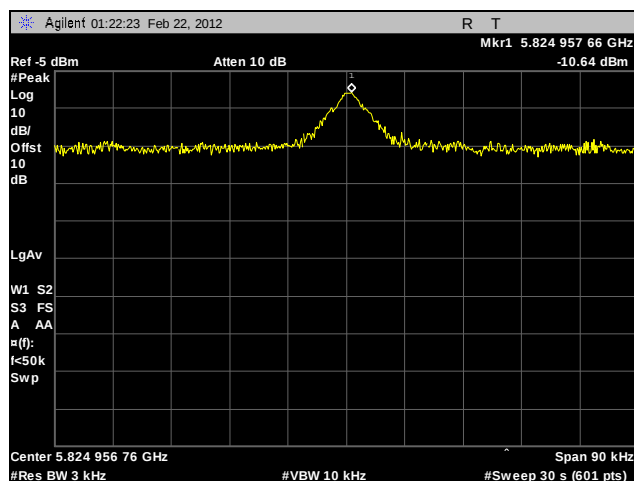
Plot 299. Peak Power Spectral Density, High Channel, 802.11a, Port A, Sector Antenna
