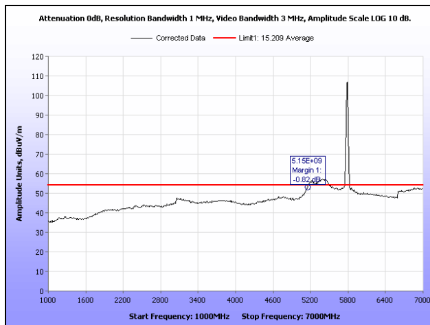
Plot 171. Radiated Spurious Emissions, Mid Channel, 802.11n 20 MHz, Sector Antenna, 1 GHz – 7 GHz, Average
