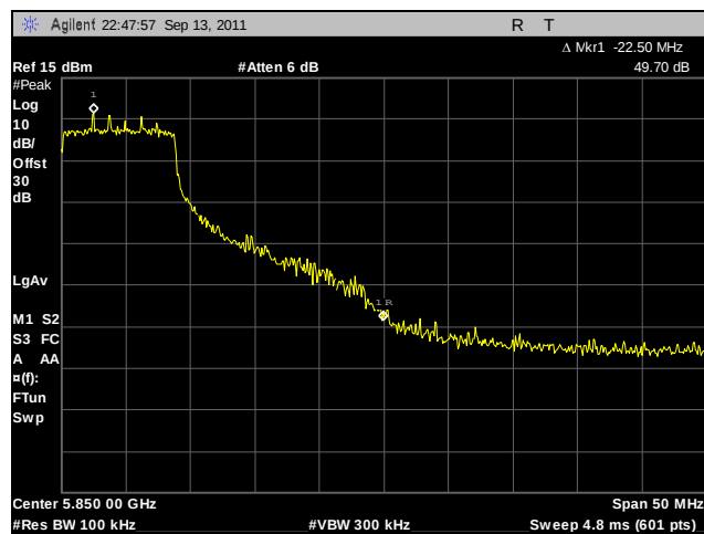
Plot 257. Conducted Band Edge, High Channel, 802.11n 20 MHz, Port A
