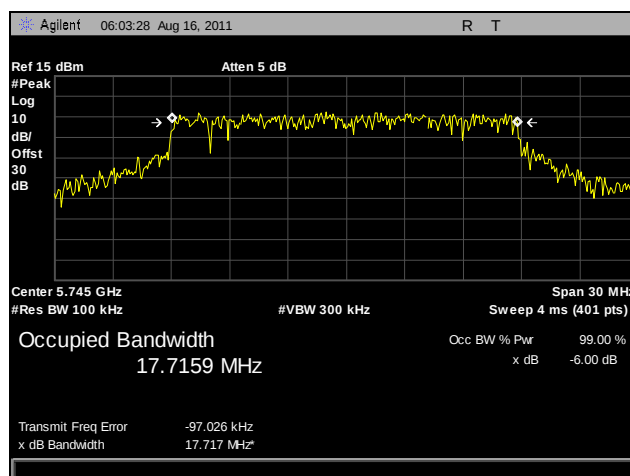
Plot 13. 6 dB Occupied Bandwidth, Low Channel, 802.11n 20 MHz, Port B
