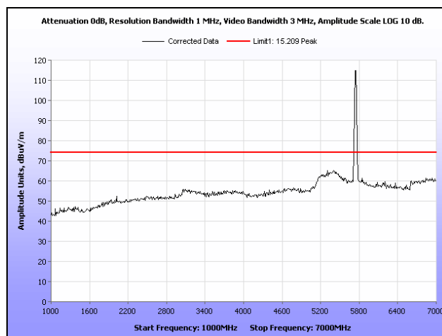
Plot 165. Radiated Spurious Emissions, Low Channel, 802.11n 20 MHz, Sector Antenna, 1 GHz – 7 GHz, Peak
