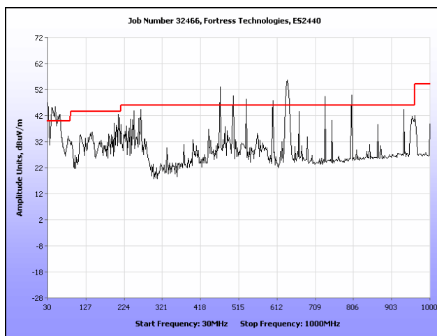
Plot 170. Radiated Spurious Emissions, Mid Channel, 802.11n 20 MHz, Sector Antenna, 30 MHz – 1 GHz Note: Emissions which exceed the limit are digital emissions.
