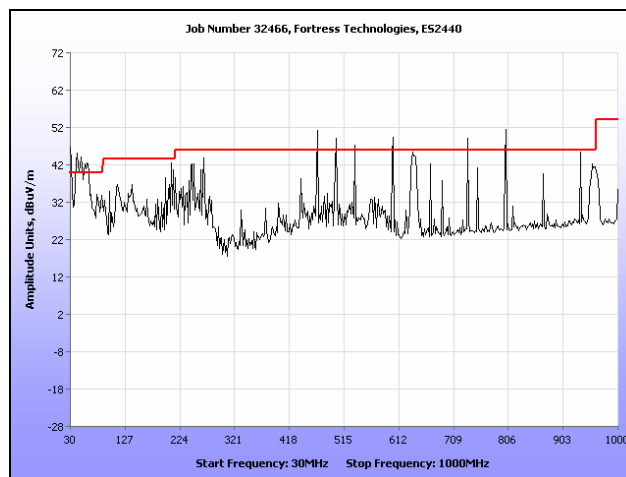
Plot 163. Radiated Spurious Emissions, Low Channel, 802.11n 20 MHz, Sector Antenna, 30 MHz – 1 GHz Note: Emissions which exceed the limit are digital emissions.
