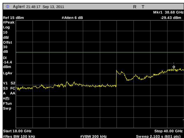
Plot 226. Conducted Spurious Emissions, High Channel, 802.11n 20 MHz, Port A, 18 GHz – 40 GHz
