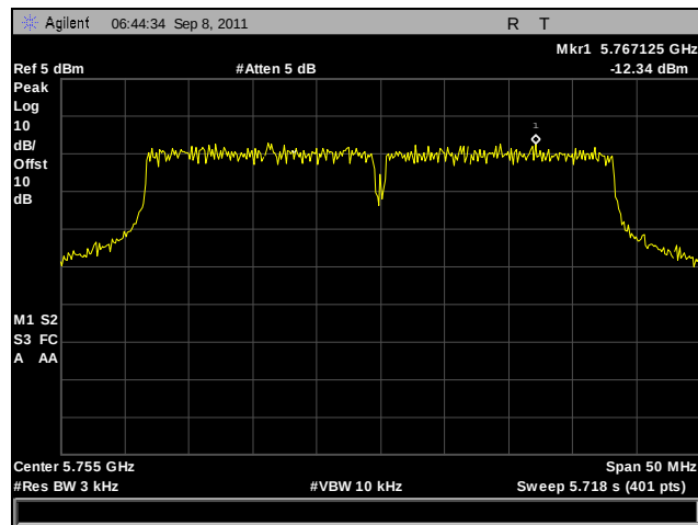
Plot 282. Peak Power Spectral Density, Low Channel, 802.11a 40 MHz, Port A, Determination
