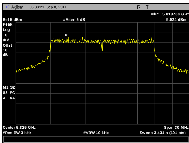
Plot 274. Peak Power Spectral Density, High Channel, 802.11a 20 MHz, Port A, Determination
