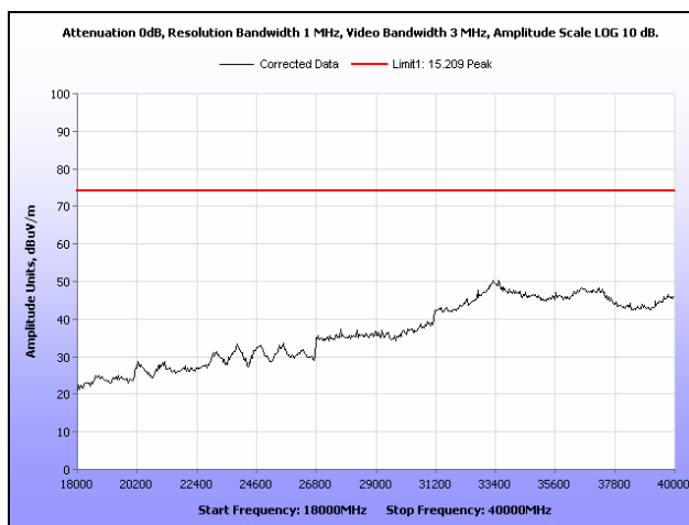
Plot 100. Radiated Spurious Emissions, Low Channel, 802.11n 20 MHz, Omni Antenna, 18 GHz – 40 GHz, Peak
