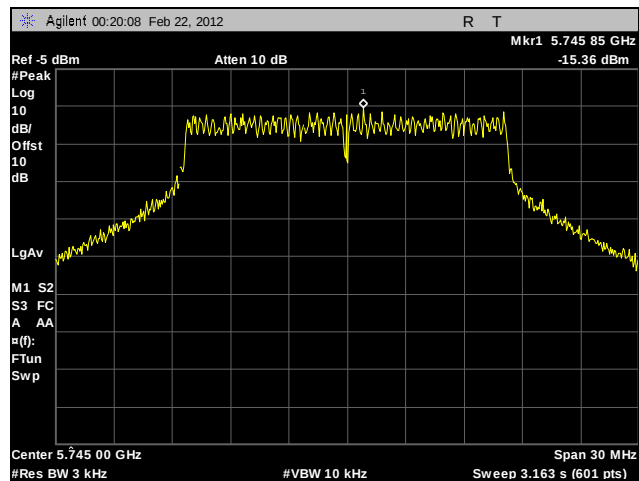
Plot 300. Peak Power Spectral Density, Low Channel, 802.11a 20 MHz, Port A, Sector Antenna, Determination
