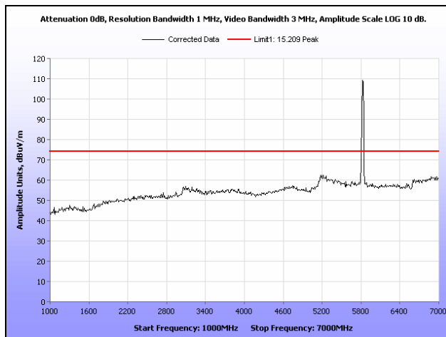
Plot 158. Radiated Spurious Emissions, High Channel, 802.11a, Sector Antenna, 1 GHz – 7 GHz, Peak
