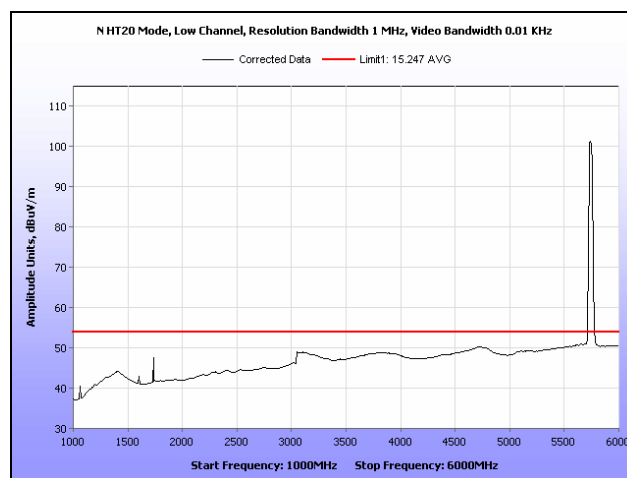
Plot 94. Radiated Spurious Emissions, Low Channel, 802.11n 20 MHz, Omni Antenna, 1 GHz – 6 GHz, Average
