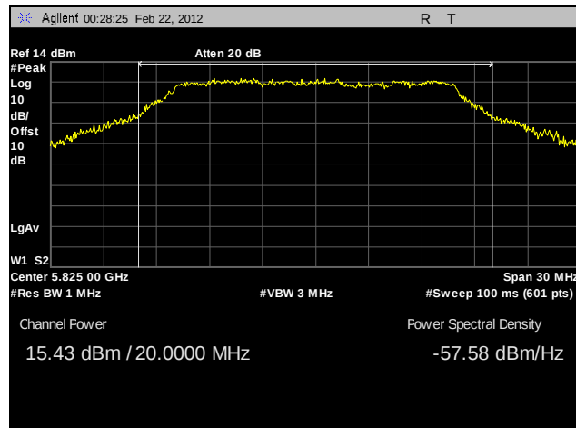
Plot 60. Peak Power Output, High Channel, 802.11n 20 MHz, Port B, Sector Antenna
