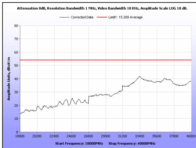
Plot 115. Radiated Spurious Emissions, High Channel, 802.11n 20 MHz, Omni Antenna, 18 GHz – 40 GHz, Average
