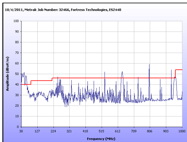
Plot 76. Radiated Spurious Emissions, Mid Channel, 802.11a, Omni Antenna, 30 MHz – 1 GHz
