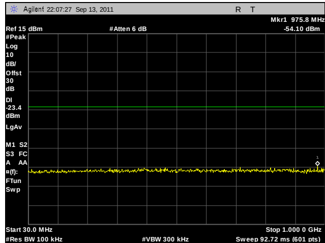
Plot 245. Conducted Spurious Emissions, Low Channel, 802.11n 40 MHz, Port B, 30 MHz – 1 GHz
