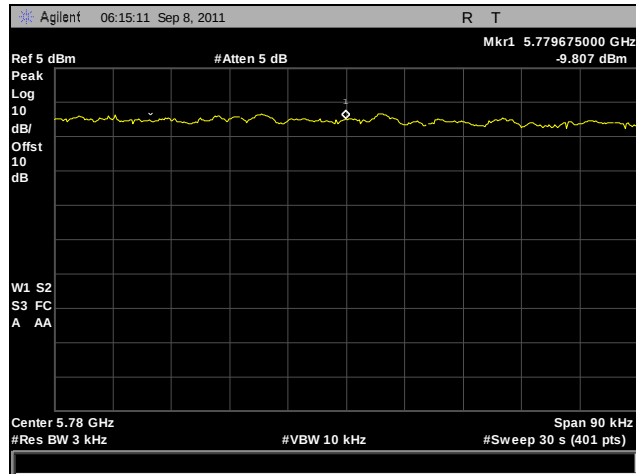
Plot 267. Peak Power Spectral Density, Mid Channel, 802.11a, Port A
