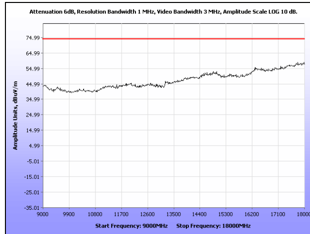
Plot 82. Radiated Spurious Emissions, Mid Channel, 802.11a, Omni Antenna, 9 GHz – 18 GHz, Peak
