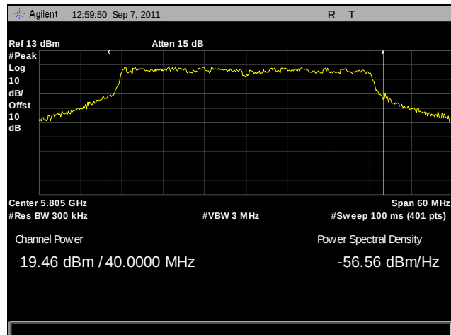
Plot 51. Peak Power Output, High Channel, 802.11n 40 MHz, Port B
