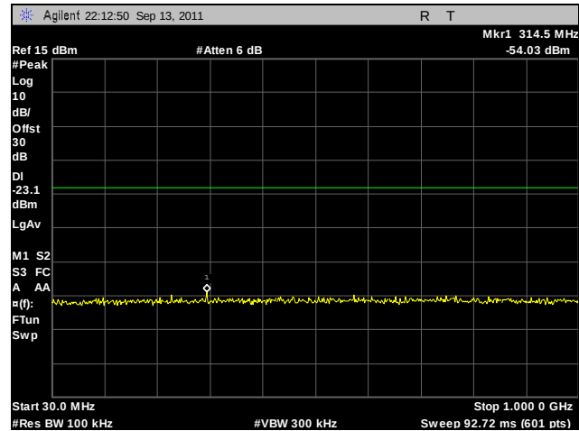
Plot 248. Conducted Spurious Emissions, Mid Channel, 802.11n 40 MHz, Port B, 30 MHz – 1 GHz
