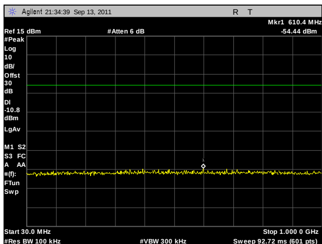
Plot 209. Conducted Spurious Emissions, Low Channel, 802.11a, Port A, 30 MHz – 1 GHz
