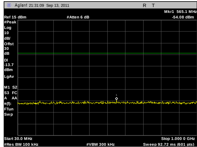
Plot 212. Conducted Spurious Emissions, Mid Channel, 802.11a, Port A, 30 MHz – 1 GHz
