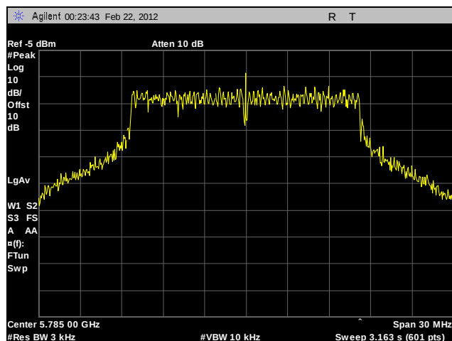
Plot 308. Peak Power Spectral Density, Mid Channel, 802.11a 20 MHz, Port B, Sector Antenna, Determination
