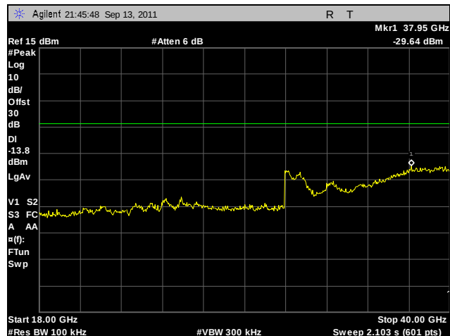
Plot 220. Conducted Spurious Emissions, Low Channel, 802.11n 20 MHz, Port A, 18 GHz – 40 GHz
