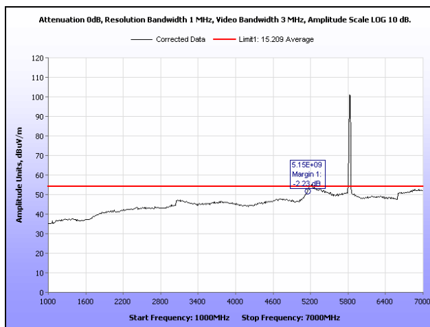
Plot 157. Radiated Spurious Emissions, High Channel, 802.11a, Sector Antenna, 1 GHz – 7 GHz, Average
