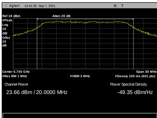
Plot 43. Peak Power Output, Low Channel, 802.11n 20 MHz, Port B
