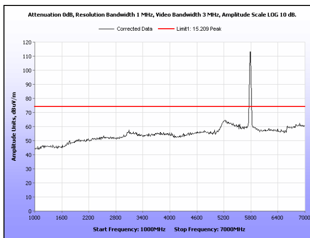
Plot 151. Radiated Spurious Emissions, Mid Channel, 802.11a, Sector Antenna, 1 GHz – 7 GHz, Peak
