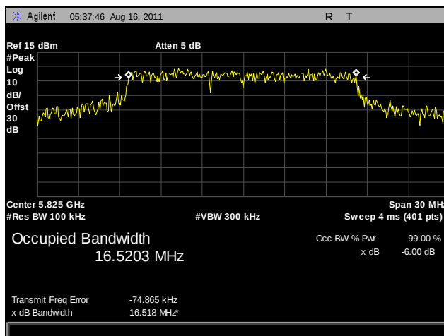
Plot 9. 6 dB Occupied Bandwidth, High Channel, 802.11a, Port A
