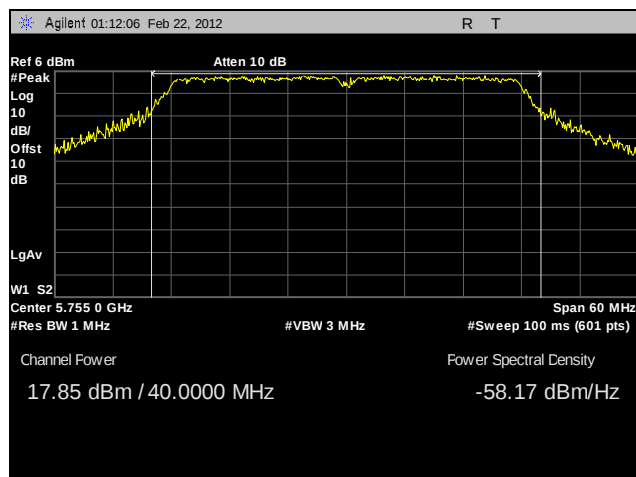
Plot 61. Peak Power Output, Low Channel, 802.11n 40 MHz, Port A, Sector Antenna
