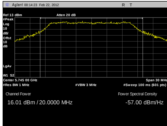
Plot 58. Peak Power Output, Low Channel, 802.11n 20 MHz, Port B, Sector Antenna
