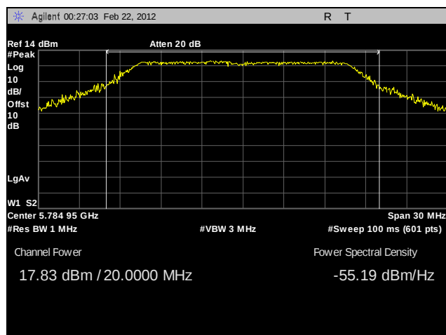
Plot 56. Peak Power Output, Mid Channel, 802.11n 20 MHz, Port A, Sector Antenna
