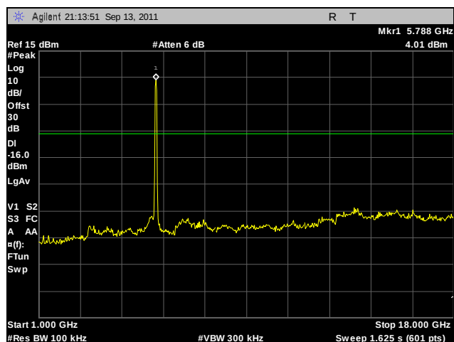
Plot 240. Conducted Spurious Emissions, Mid Channel, 802.11n 40 MHz, Port A, 1 GHz – 18 GHz
