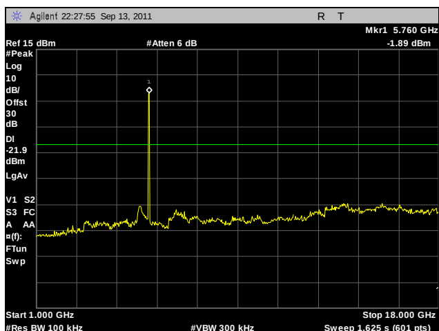
Plot 228. Conducted Spurious Emissions, Low Channel, 802.11n 20 MHz, Port B, 1 GHz – 18 GHz
