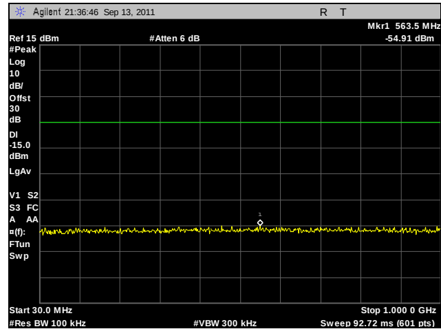
Plot 215. Conducted Spurious Emissions, High Channel, 802.11a, Port A, 30 MHz – 1 GHz
