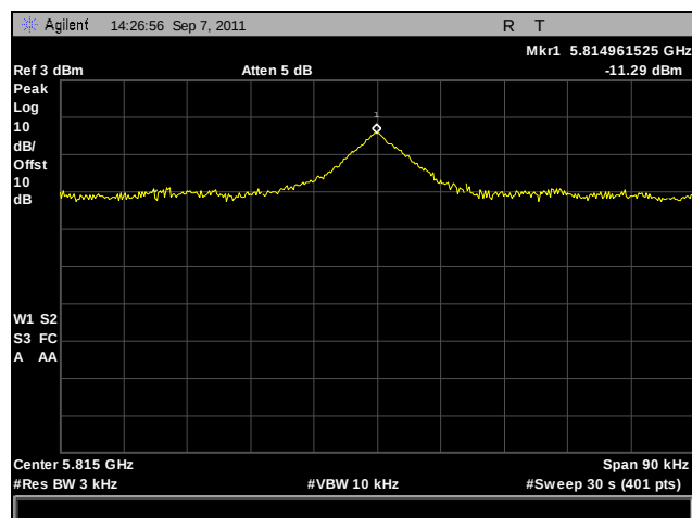
Plot 287. Peak Power Spectral Density, High Channel, 802.11a 40 MHz, Port A
