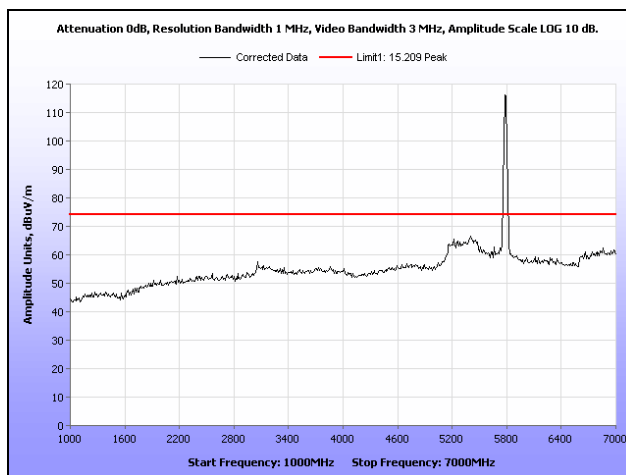
Plot 172. Radiated Spurious Emissions, Mid Channel, 802.11n 20 MHz, Sector Antenna, 1 GHz – 7 GHz, Peak
