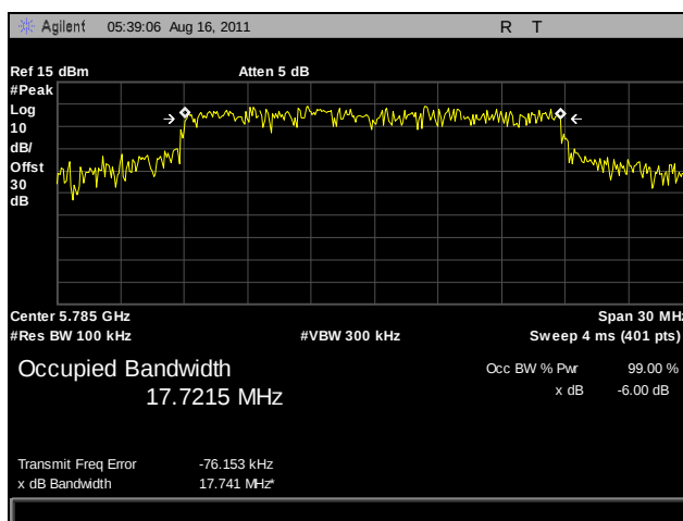
Plot 11. 6 dB Occupied Bandwidth, Mid Channel, 802.11n 20 MHz, Port A
