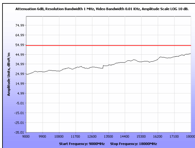
Plot 81. Radiated Spurious Emissions, Mid Channel, 802.11a, Omni Antenna, 9 GHz – 18 GHz, Average
