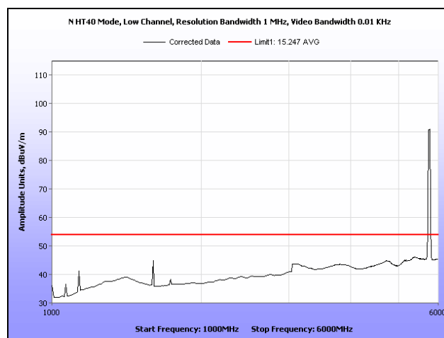
Plot 118. Radiated Spurious Emissions, Low Channel, 802.11n 40 MHz, Omni Antenna, 1 GHz – 6 GHz, Average
