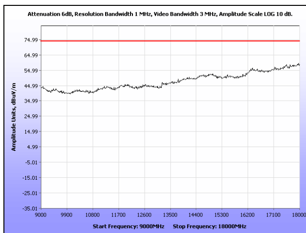
Plot 138. Radiated Spurious Emissions, High Channel, 802.11n 40 MHz, Omni Antenna, 9 GHz – 18 GHz, Peak
