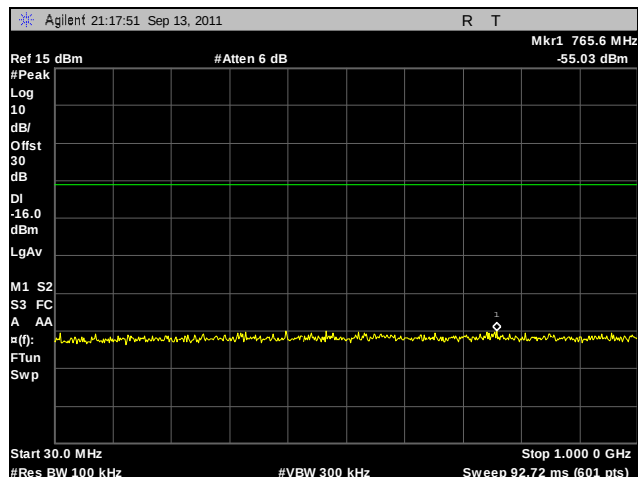
Plot 239. Conducted Spurious Emissions, Mid Channel, 802.11n 40 MHz, Port A, 30 MHz – 1 GHz
