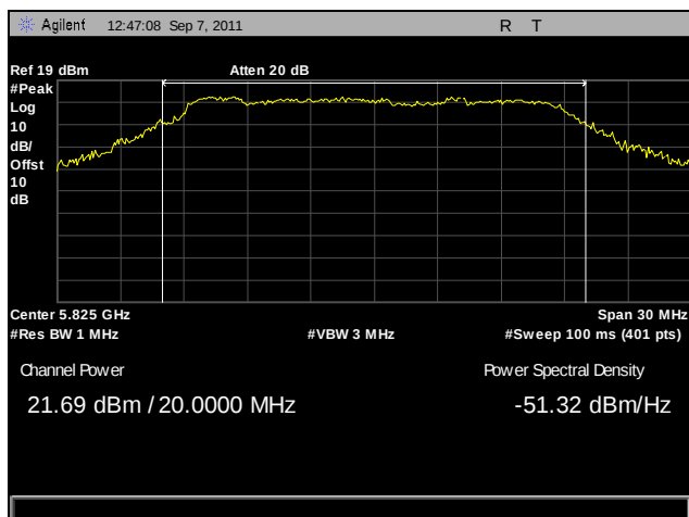
Plot 45. Peak Power Output, High Channel, 802.11n 20 MHz, Port B
