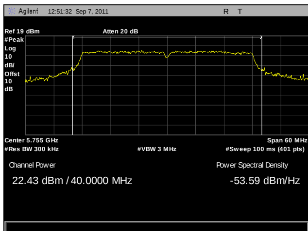
Plot 46. Peak Power Output, Low Channel, 802.11n 40 MHz, Port A
