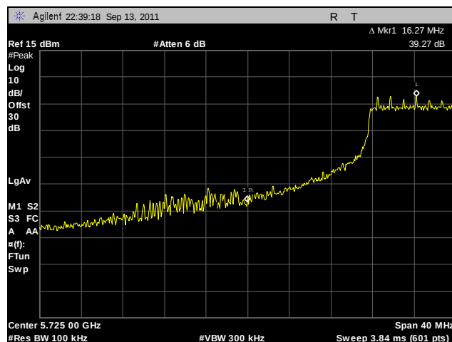
Plot 262. Conducted Band Edge, Low Channel, 802.11n 40 MHz, Port B
