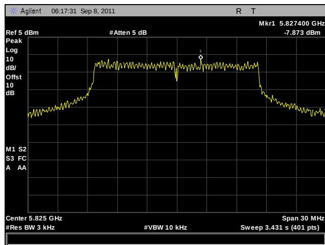
Plot 268. Peak Power Spectral Density, High Channel, 802.11a, Port A, Determination
