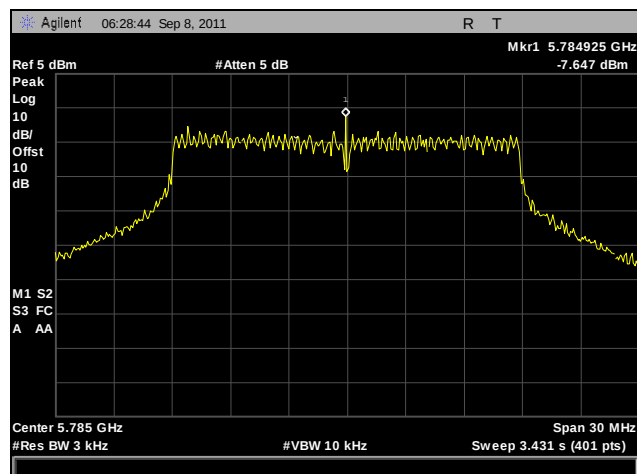
Plot 278. Peak Power Spectral Density, Mid Channel, 802.11a 20 MHz, Port B, Determination
