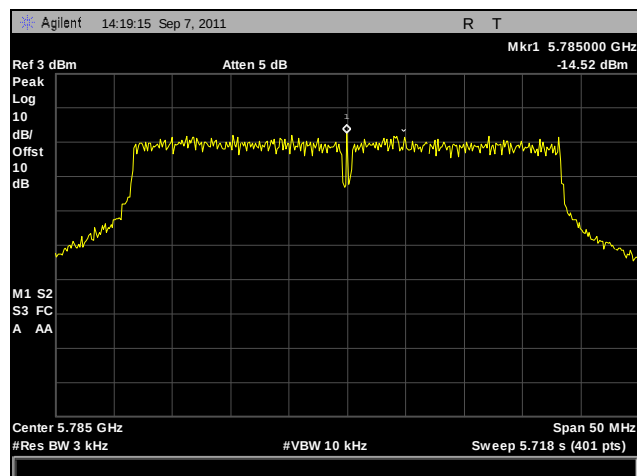
Plot 290. Peak Power Spectral Density, Mid Channel, 802.11a 40 MHz, Port B, Determination
