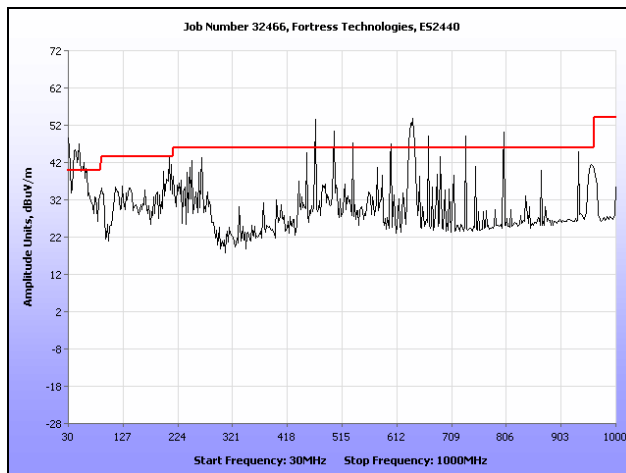
Plot 156. Radiated Spurious Emissions, High Channel, 802.11a, Sector Antenna, 30 MHz – 1 GHz Note: Emissions which exceed the limit are digital emissions.
