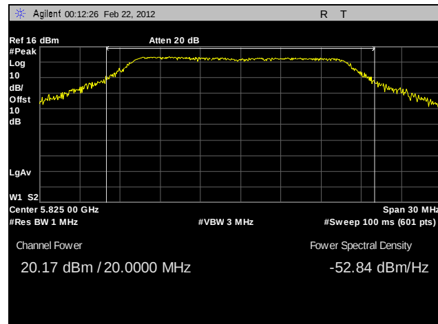
Plot 54. Peak Power Output, High Channel, 802.11a, Port A, Sector Antenna
