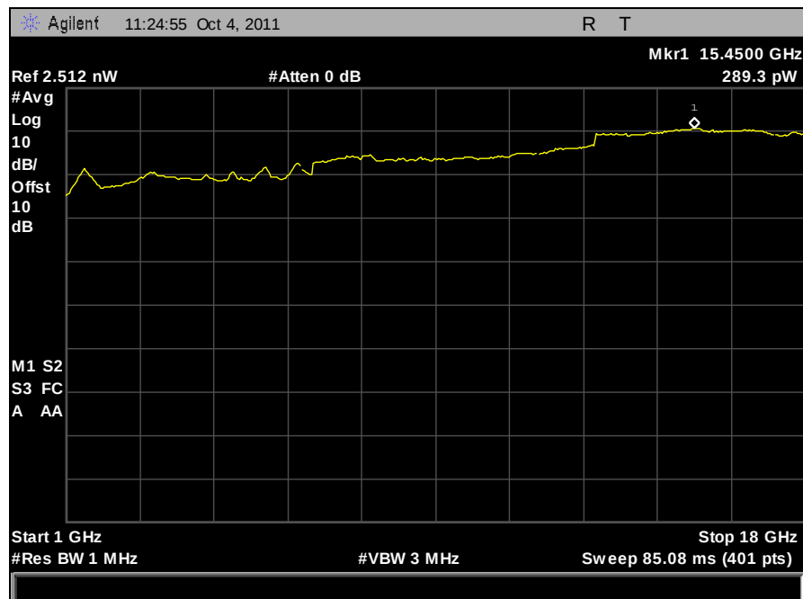
Plot 327. Receiver Spurious Emission, 1 GHz – 18 GHz, Port B
