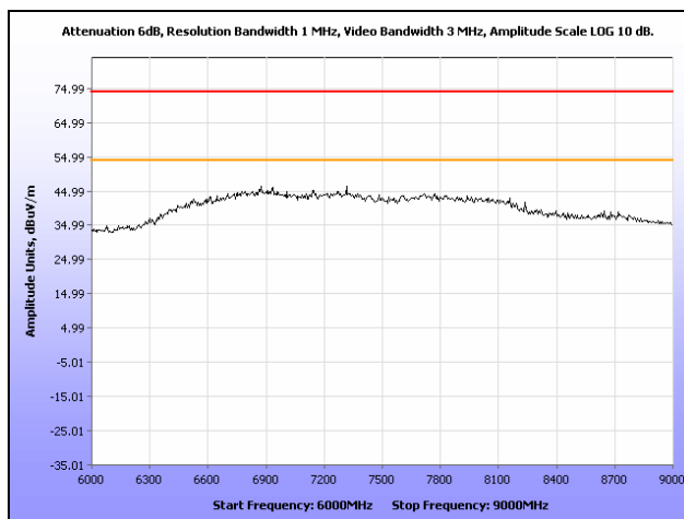
Plot 112. Radiated Spurious Emissions, High Channel, 802.11n 20 MHz, Omni Antenna, 6 GHz – 9 GHz
