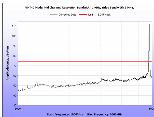
Plot 127. Radiated Spurious Emissions, Mid Channel, 802.11n 40 MHz, Omni Antenna, 1 GHz – 6 GHz, Peak
