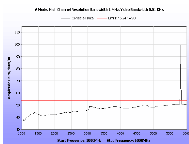
Plot 86. Radiated Spurious Emissions, High Channel, 802.11a, Omni Antenna, 1 GHz – 6 GHz, Average
