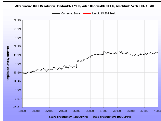
Plot 147. Radiated Spurious Emissions, Low Channel, 802.11a, Sector Antenna, 18 GHz – 40 GHz, Peak
