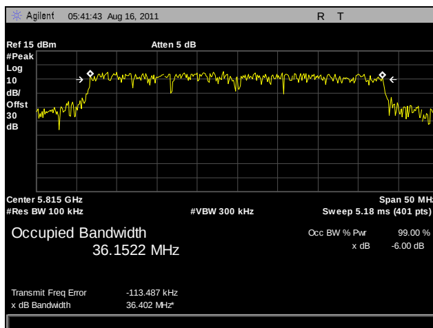
Plot 18. 6 dB Occupied Bandwidth, High Channel, 802.11n 40 MHz, Port A
