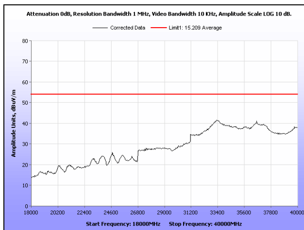
Plot 107. Radiated Spurious Emissions, Mid Channel, 802.11n 20 MHz, Omni Antenna, 18 GHz – 40 GHz, Average
