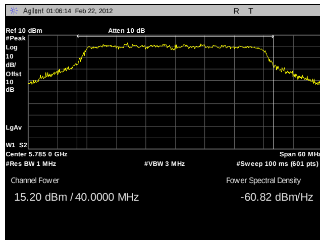
Plot 65. Peak Power Output, Mid Channel, 802.11n 40 MHz, Port B, Sector Antenna
