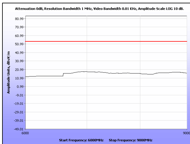
Plot 79. Radiated Spurious Emissions, Mid Channel, 802.11a, Omni Antenna, 6 GHz – 9 GHz, Average
