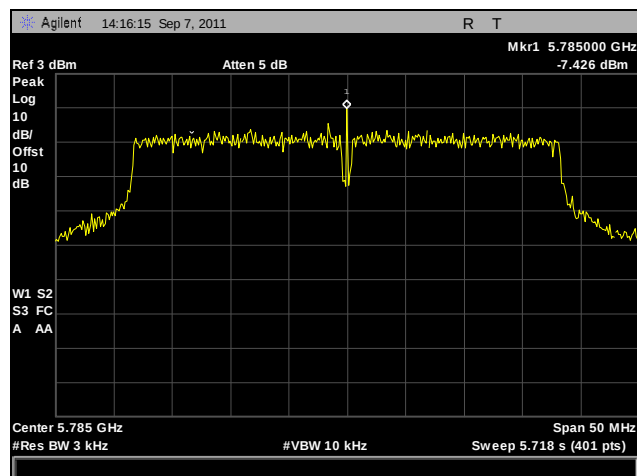
Plot 284. Peak Power Spectral Density, Mid Channel, 802.11a 40 MHz, Port A, Determination
