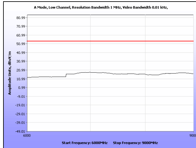
Plot 70. Radiated Spurious Emissions, Low Channel, 802.11a, Omni Antenna, 6 GHz – 9 GHz, Average
