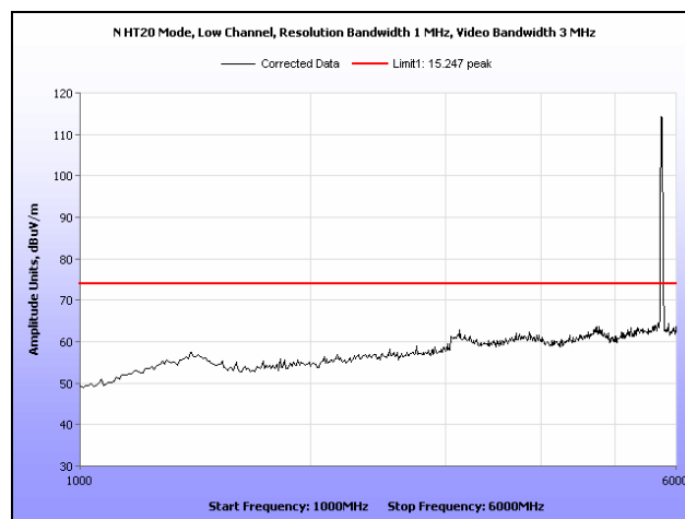
Plot 95. Radiated Spurious Emissions, Low Channel, 802.11n 20 MHz, Omni Antenna, 1 GHz – 6 GHz, Peak
