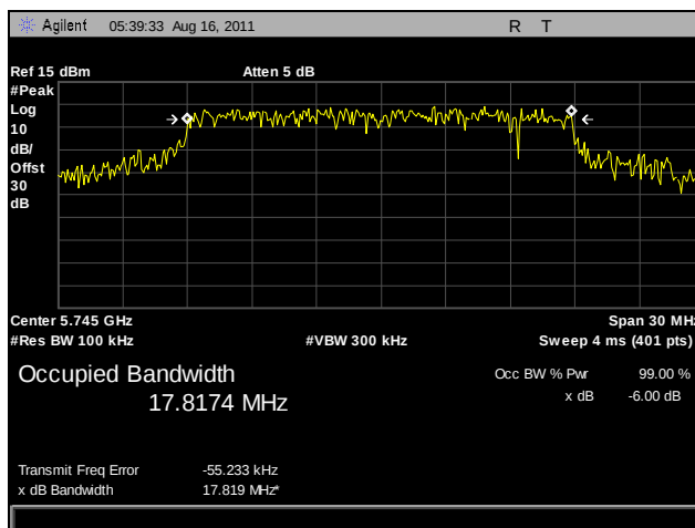
Plot 10. 6 dB Occupied Bandwidth, Low Channel, 802.11n 20 MHz, Port A
