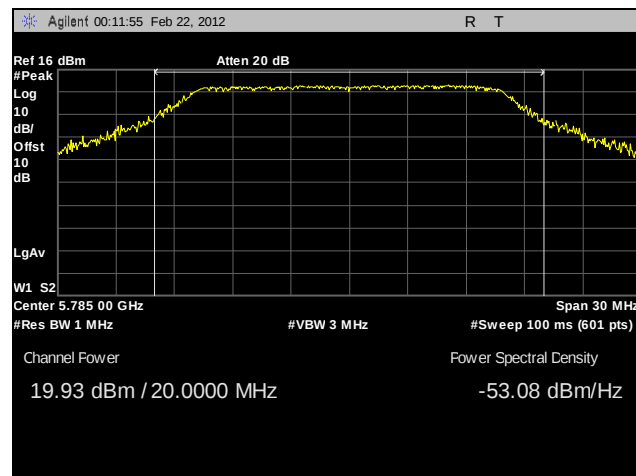
Plot 53. Peak Power Output, Mid Channel, 802.11a, Port A, Sector Antenna
