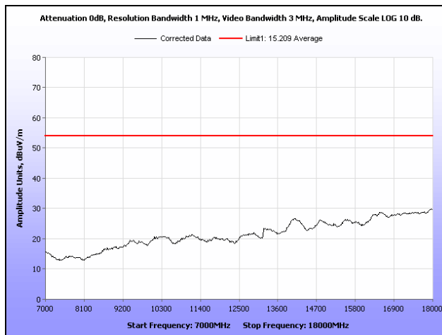
Plot 152. Radiated Spurious Emissions, Mid Channel, 802.11a, Sector Antenna, 7 GHz – 18 GHz, Average
