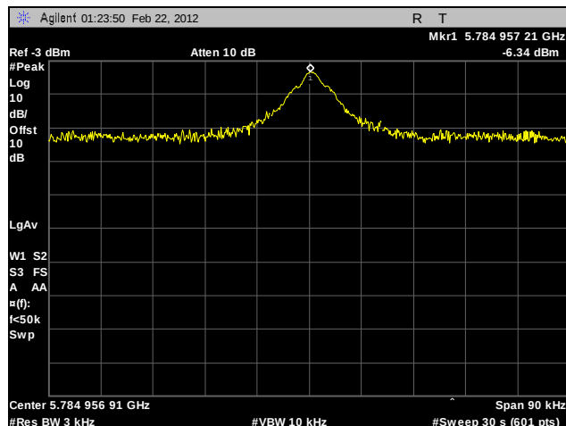
Plot 297. Peak Power Spectral Density, Mid Channel, 802.11a, Port A, Sector Antenna
