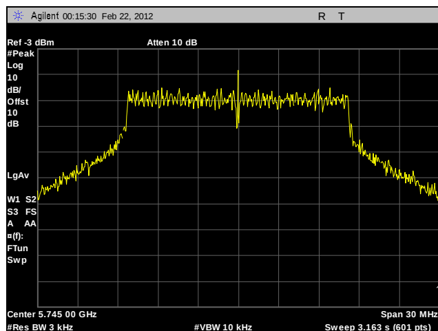
Plot 306. Peak Power Spectral Density, Low Channel, 802.11a 20 MHz, Port B, Sector Antenna, Determination
