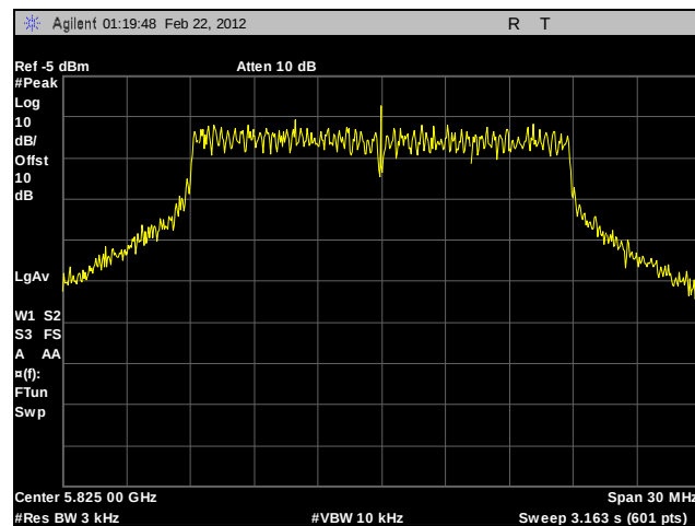
Plot 304. Peak Power Spectral Density, High Channel, 802.11a 20 MHz, Port A, Sector Antenna, Determination
