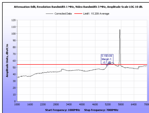
Plot 164. Radiated Spurious Emissions, Low Channel, 802.11n 20 MHz, Sector Antenna, 1 GHz – 7 GHz, Average
