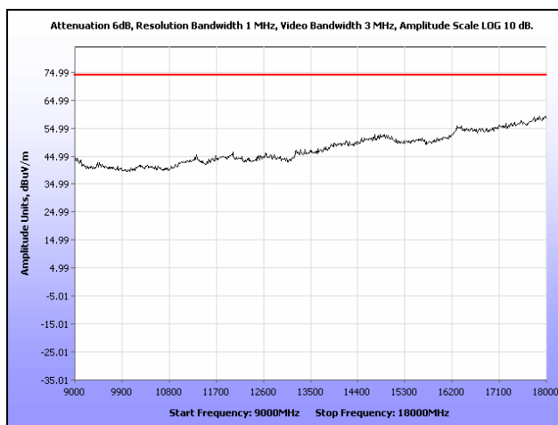
Plot 122. Radiated Spurious Emissions, Low Channel, 802.11n 40 MHz, Omni Antenna, 9 GHz – 18 GHz, Peak
