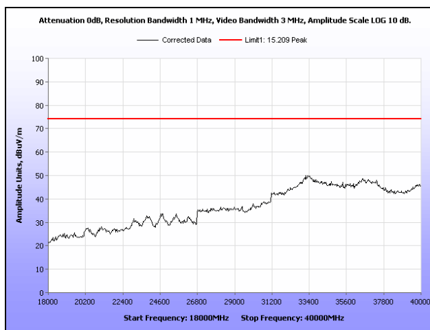
Plot 108. Radiated Spurious Emissions, Mid Channel, 802.11n 20 MHz, Omni Antenna, 18 GHz – 40 GHz, Peak
