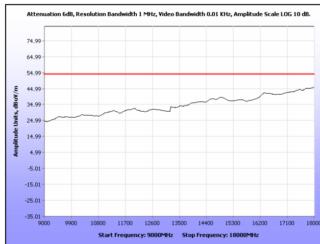
Plot 97. Radiated Spurious Emissions, Low Channel, 802.11n 20 MHz, Omni Antenna, 9 GHz – 18 GHz, Average
