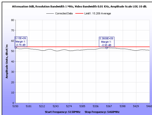
Plot 203. Radiated Spurious Emissions, High Channel, 802.11n 40 MHz, Sector Antenna, Smaller Span
