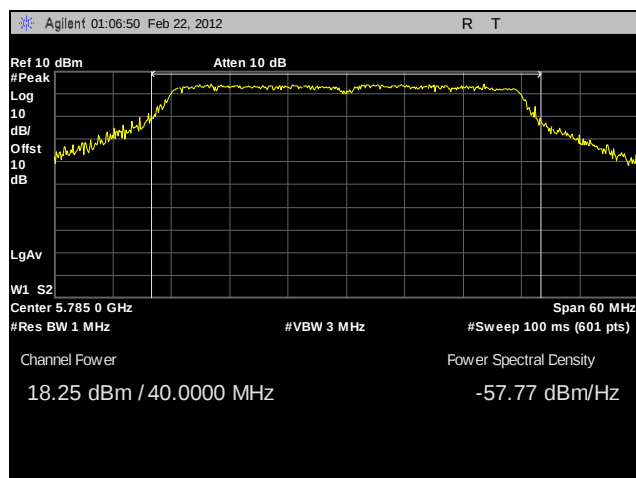
Plot 62. Peak Power Output, Mid Channel, 802.11n 40 MHz, Port A, Sector Antenna
