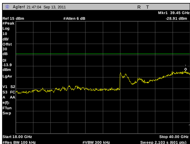
Plot 223. Conducted Spurious Emissions, Mid Channel, 802.11n 20 MHz, Port A, 18 GHz – 40 GHz
