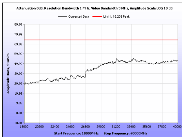
Plot 162. Radiated Spurious Emissions, High Channel, 802.11a, Sector Antenna, 18 GHz – 40 GHz, Peak
