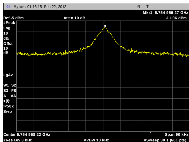
Plot 319. Peak Power Spectral Density, Low Channel, 802.11a 40 MHz, Port B, Sector Antenna
