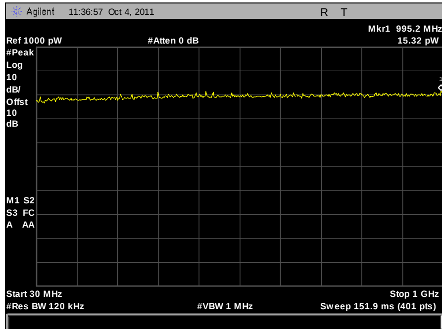
Plot 326. Receiver Spurious Emission, 30 MHz – 1 GHz, Port B
