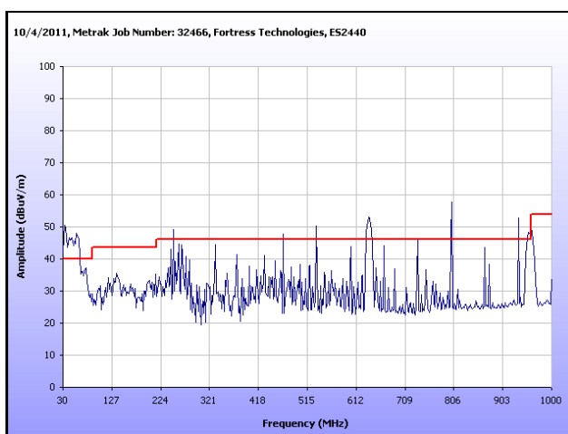
Plot 201. Radiated Spurious Emissions, High Channel, 802.11n 40 MHz, Sector Antenna, 30 MHz – 1 GHz Note: Emissions which exceed the limit are digital emissions.
