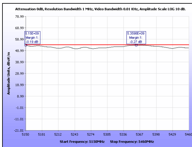
Plot 195. Radiated Spurious Emissions, Mid Channel, 802.11n 40 MHz, Sector Antenna, Smaller Span
