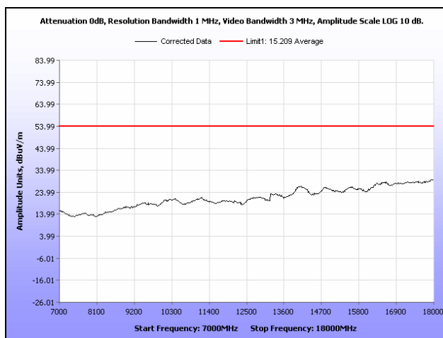
Plot 173. Radiated Spurious Emissions, Mid Channel, 802.11n 20 MHz, Sector Antenna, 7 GHz – 18 GHz, Average
