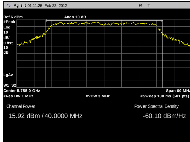
Plot 64. Peak Power Output, Low Channel, 802.11n 40 MHz, Port B, Sector Antenna
