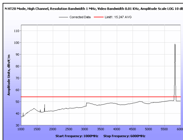
Plot 110. Radiated Spurious Emissions, High Channel, 802.11n 20 MHz, Omni Antenna, 1 GHz – 6 GHz, Average
