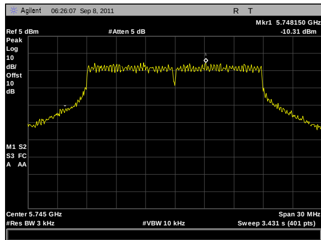
Plot 276. Peak Power Spectral Density, Low Channel, 802.11a 20 MHz, Port B, Determination
