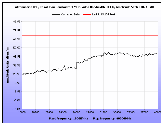
Plot 192. Radiated Spurious Emissions, Low Channel, 802.11n 40 MHz, Sector Antenna, 18 GHz – 40 GHz, Peak
