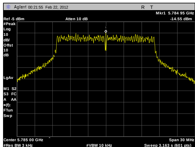
Plot 302. Peak Power Spectral Density, Mid Channel, 802.11a 20 MHz, Port A, Sector Antenna, Determination
