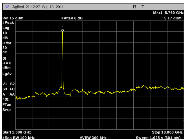
Plot 237. Conducted Spurious Emissions, Low Channel, 802.11n 40 MHz, Port A, 1 GHz – 18 GHz
