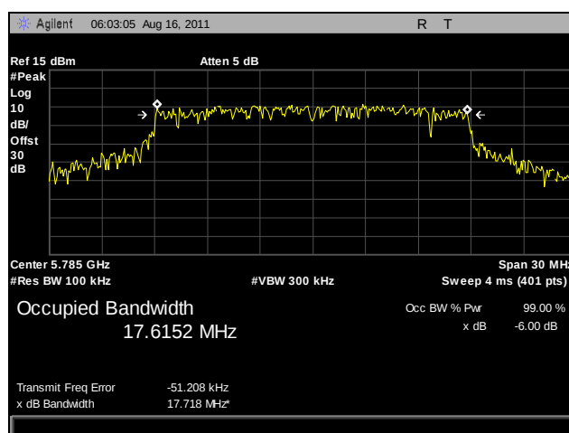
Plot 14. 6 dB Occupied Bandwidth, Mid Channel, 802.11n 20 MHz, Port B
