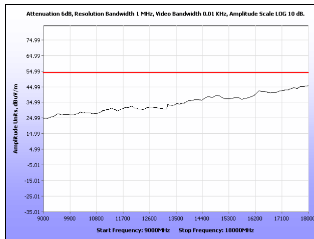
Plot 129. Radiated Spurious Emissions, Mid Channel, 802.11n 40 MHz, Omni Antenna, 9 GHz – 18 GHz, Average
