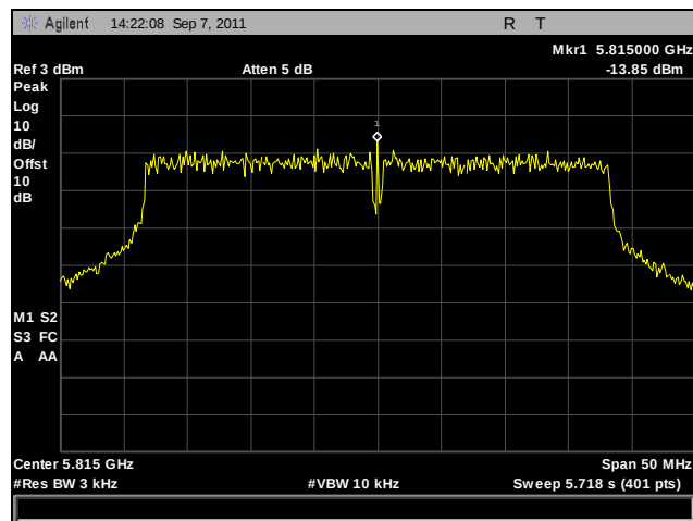
Plot 292. Peak Power Spectral Density, High Channel, 802.11a 40 MHz, Port B, Determination
