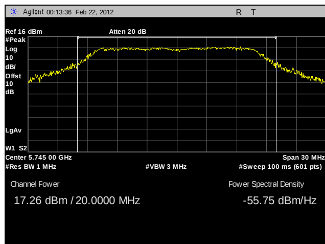
Plot 55. Peak Power Output, Low Channel, 802.11n 20 MHz, Port A, Sector Antenna
