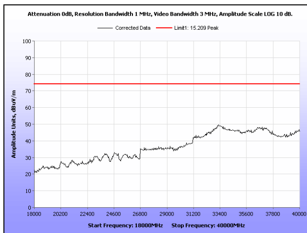
Plot 116. Radiated Spurious Emissions, High Channel, 802.11n 20 MHz, Omni Antenna, 18 GHz – 40 GHz, Peak
