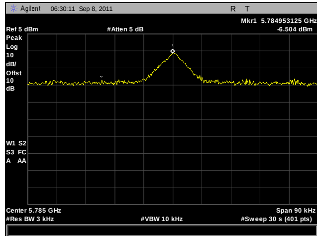
Plot 279. Peak Power Spectral Density, Mid Channel, 802.11a 20 MHz, Port B
