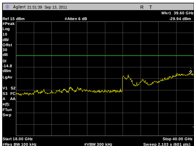
Plot 238. Conducted Spurious Emissions, Low Channel, 802.11n 40 MHz, Port A, 18 GHz – 40 GHz
