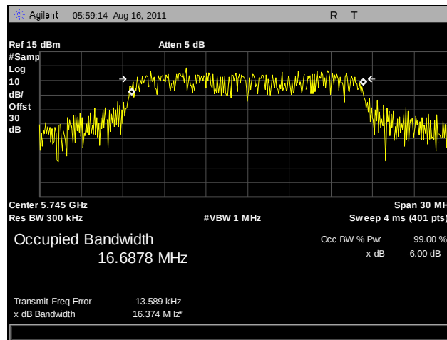
Plot 22. 99% Occupied Bandwidth, Low Channel, 802.11a, Port B
