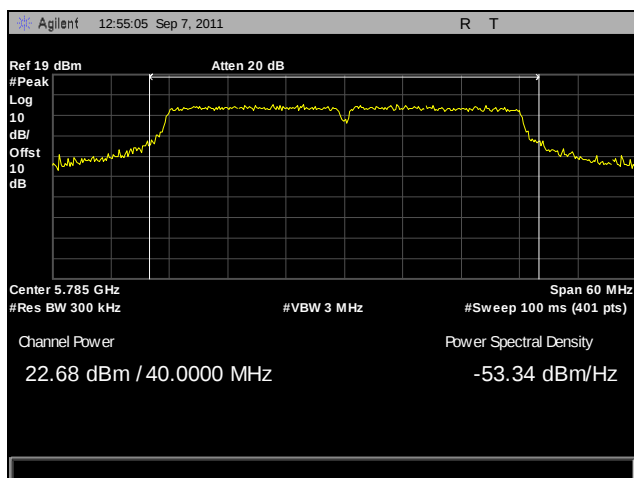
Plot 47. Peak Power Output, Mid Channel, 802.11n 40 MHz, Port A
