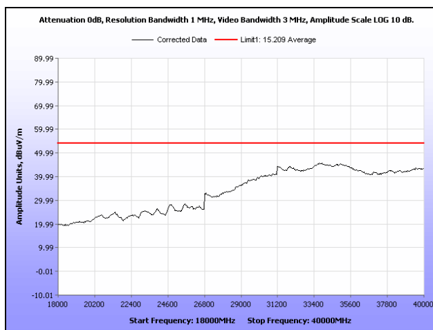
Plot 146. Radiated Spurious Emissions, Low Channel, 802.11a, Sector Antenna, 18 GHz – 40 GHz, Average
