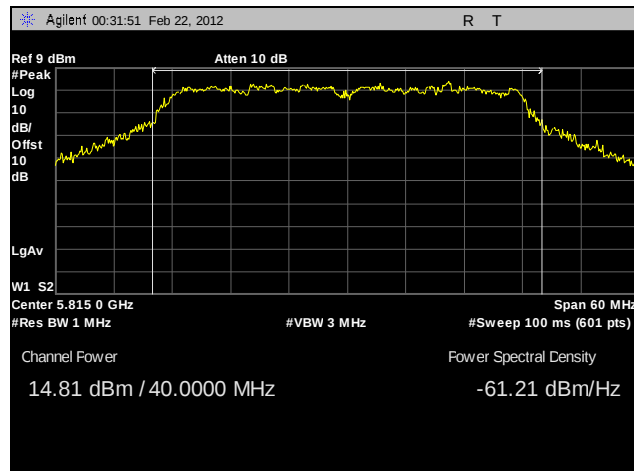
Plot 66. Peak Power Output, High Channel, 802.11n 40 MHz, Port B, Sector Antenna
