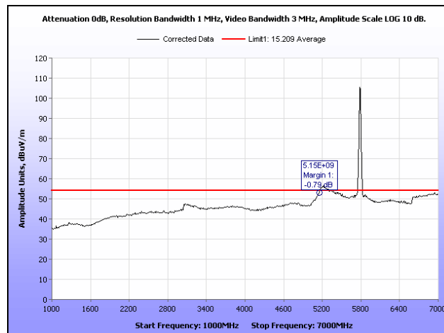
Plot 149. Radiated Spurious Emissions, Mid Channel, 802.11a, Sector Antenna, 1 GHz – 7 GHz, Average
