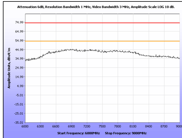
Plot 104. Radiated Spurious Emissions, Mid Channel, 802.11n 20 MHz, Omni Antenna, 6 GHz – 9 GHz
