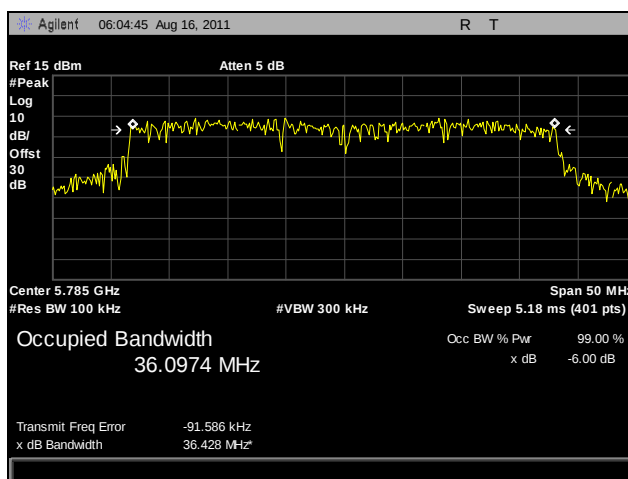
Plot 20. 6 dB Occupied Bandwidth, Mid Channel, 802.11n 40 MHz, Port B
