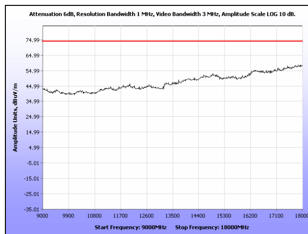
Plot 106. Radiated Spurious Emissions, Mid Channel, 802.11n 20 MHz, Omni Antenna, 9 GHz – 18 GHz, Peak
