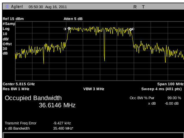
Plot 33. 99% Occupied Bandwidth, High Channel, 802.11n 40 MHz, Port A
