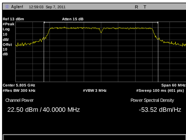
Plot 48. Peak Power Output, High Channel, 802.11n 40 MHz, Port A
