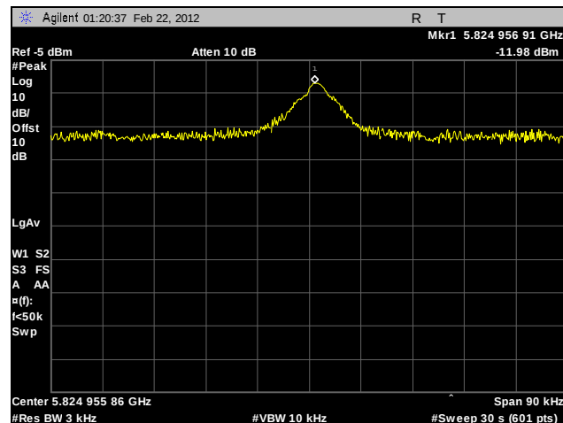
Plot 305. Peak Power Spectral Density, High Channel, 802.11a 20 MHz, Port A, Sector Antenna
