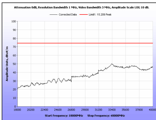
Plot 140. Radiated Spurious Emissions, High Channel, 802.11n 40 MHz, Omni Antenna, 18 GHz – 40 GHz, Peak
