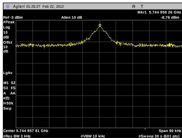
Plot 295. Peak Power Spectral Density, Low Channel, 802.11a, Port A, Sector Antenna
