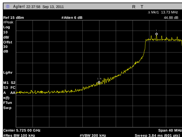
Plot 258. Conducted Band Edge, Low Channel, 802.11n 20 MHz, Port B
