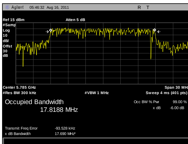
Plot 26. 99% Occupied Bandwidth, Mid Channel, 802.11n 20 MHz, Port A
