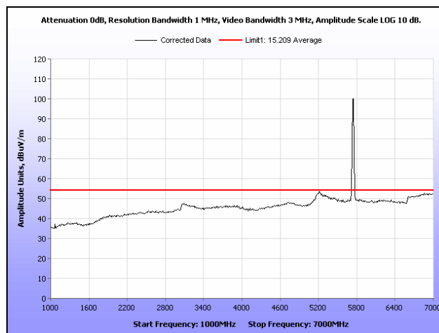
Plot 142. Radiated Spurious Emissions, Low Channel, 802.11a, Sector Antenna, 1 GHz – 7 GHz, Average
