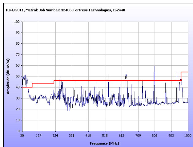
Plot 93. Radiated Spurious Emissions, Low Channel, 802.11n 20 MHz, Omni Antenna, 30 MHz – 1 GHz
