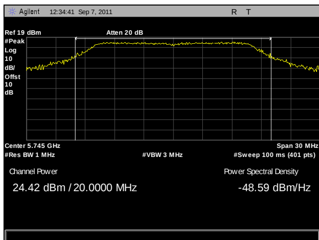
Plot 37. Peak Power Output, Low Channel, 802.11a, Port A
