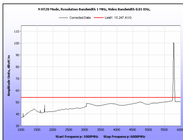
Plot 102. Radiated Spurious Emissions, Mid Channel, 802.11n 20 MHz, Omni Antenna, 1 GHz – 6 GHz, Average
