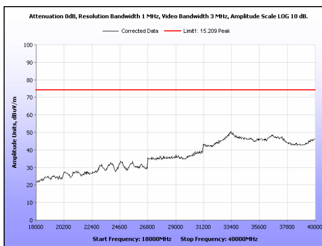
Plot 132. Radiated Spurious Emissions, Mid Channel, 802.11n 40 MHz, Omni Antenna, 18 GHz – 40 GHz, Peak
