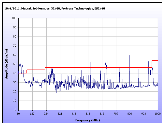
Plot 109. Radiated Spurious Emissions, High Channel, 802.11n 20 MHz, Omni Antenna, 30 MHz – 1 GHz Note: Emissions which exceed the limit are digital emissions.
