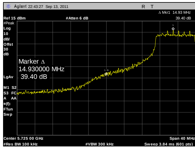
Plot 256. Conducted Band Edge, Low Channel, 802.11n 20 MHz, Port A
