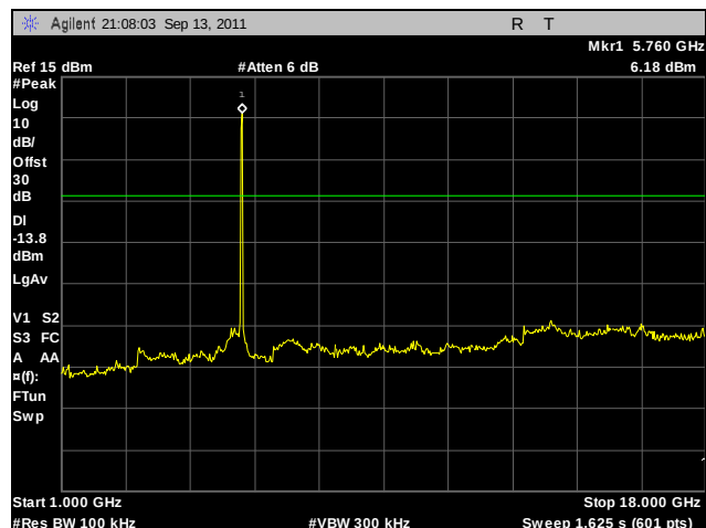
Plot 219. Conducted Spurious Emissions, Low Channel, 802.11n 20 MHz, Port A, 1 GHz – 18 GHz
