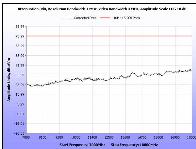
Plot 174. Radiated Spurious Emissions, Mid Channel, 802.11n 20 MHz, Sector Antenna, 7 GHz – 18 GHz, Peak
