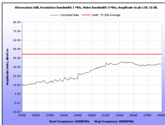
Plot 183. Radiated Spurious Emissions, High Channel, 802.11n 20 MHz, Sector Antenna, 18 GHz – 40 GHz, Average
