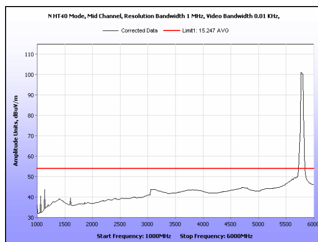
Plot 126. Radiated Spurious Emissions, Mid Channel, 802.11n 40 MHz, Omni Antenna, 1 GHz – 6 GHz, Average
