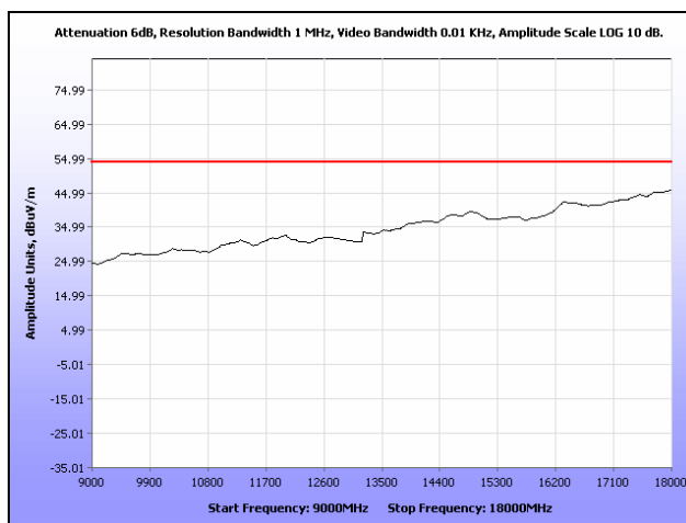
Plot 121. Radiated Spurious Emissions, Low Channel, 802.11n 40 MHz, Omni Antenna, 9 GHz – 18 GHz, Average
