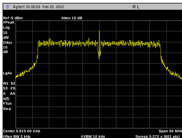
Plot 322. Peak Power Spectral Density, High Channel, 802.11a 40 MHz, Port B, Sector Antenna, Determination
