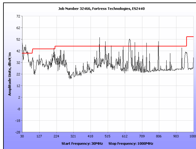
Plot 148. Radiated Spurious Emissions, Mid Channel, 802.11a, Sector Antenna, 30 MHz – 1 GHz Note: Emissions which exceed the limit are digital emissions.
