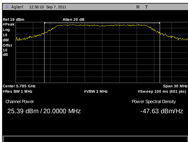
Plot 38. Peak Power Output, Mid Channel, 802.11a, Port A
