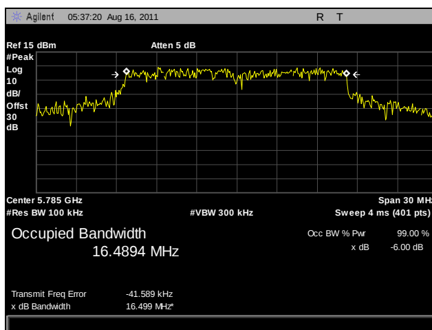
Plot 8. 6 dB Occupied Bandwidth, Mid Channel, 802.11a, Port A
