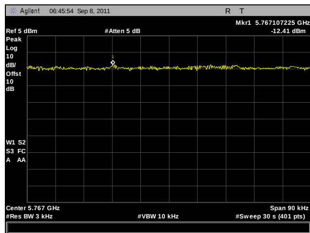
Plot 283. Peak Power Spectral Density, Low Channel, 802.11a 40 MHz, Port A
