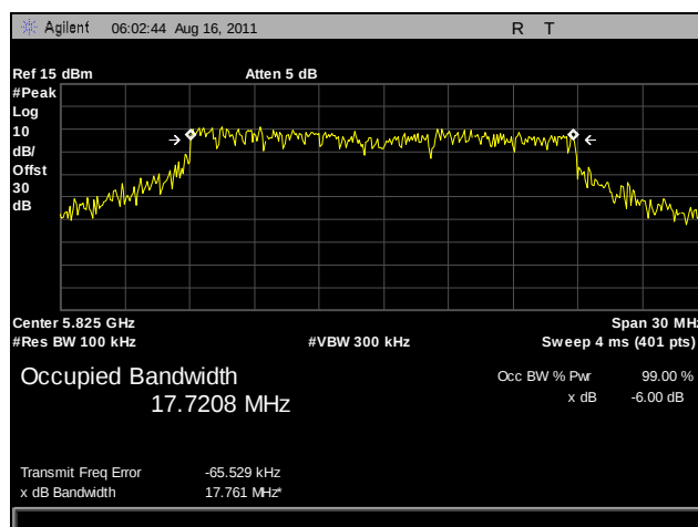
Plot 15. 6 dB Occupied Bandwidth, High Channel, 802.11n 20 MHz, Port B
