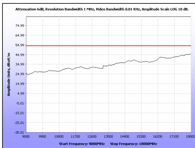
Plot 137. Radiated Spurious Emissions, High Channel, 802.11n 40 MHz, Omni Antenna, 9 GHz – 18 GHz, Average
