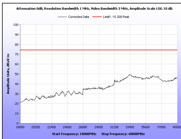
Plot 124. Radiated Spurious Emissions, Low Channel, 802.11n 40 MHz, Omni Antenna, 18 GHz – 40 GHz, Peak
