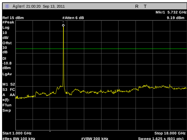
Plot 210. Conducted Spurious Emissions, Low Channel, 802.11a, Port A, 1 GHz – 18 GHz
