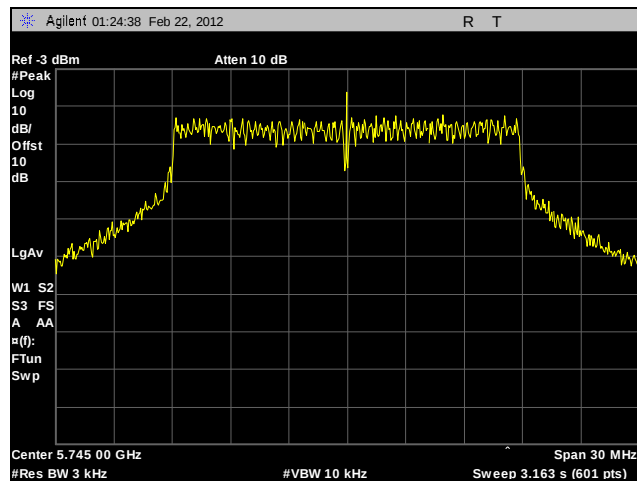
Plot 294. Peak Power Spectral Density, Low Channel, 802.11a, Port A, Sector Antenna, Determination
