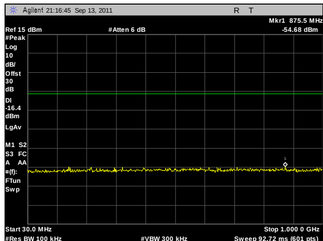
Plot 242. Conducted Spurious Emissions, High Channel, 802.11n 40 MHz, Port A, 30 MHz – 1 GHz
