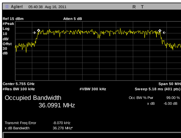
Plot 16. 6 dB Occupied Bandwidth, Low Channel, 802.11n 40 MHz, Port A
