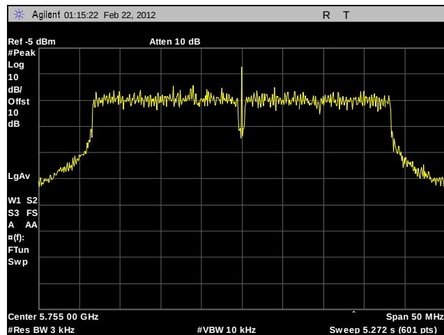
Plot 318. Peak Power Spectral Density, Low Channel, 802.11a 40 MHz, Port B, Sector Antenna, Determination
