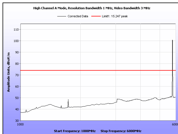
Plot 87. Radiated Spurious Emissions, High Channel, 802.11a, Omni Antenna, 1 GHz – 6 GHz, Peak
