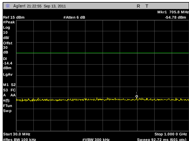
Plot 224. Conducted Spurious Emissions, High Channel, 802.11n 20 MHz, Port A, 30 MHz – 1 GHz
