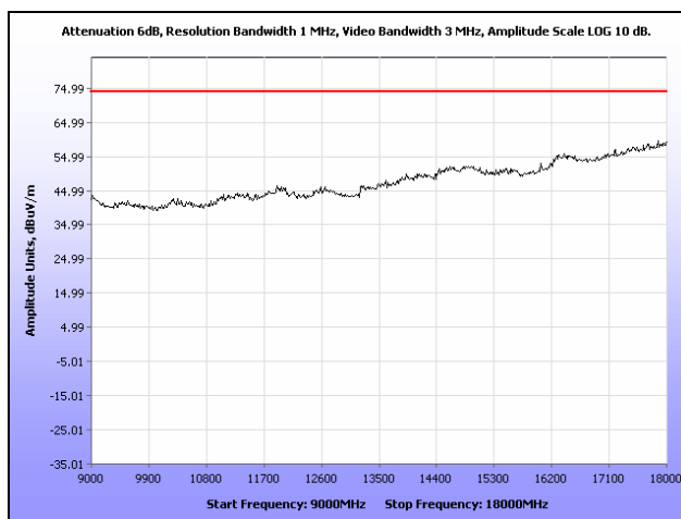
Plot 114. Radiated Spurious Emissions, High Channel, 802.11n 20 MHz, Omni Antenna, 9 GHz – 18 GHz, Peak
