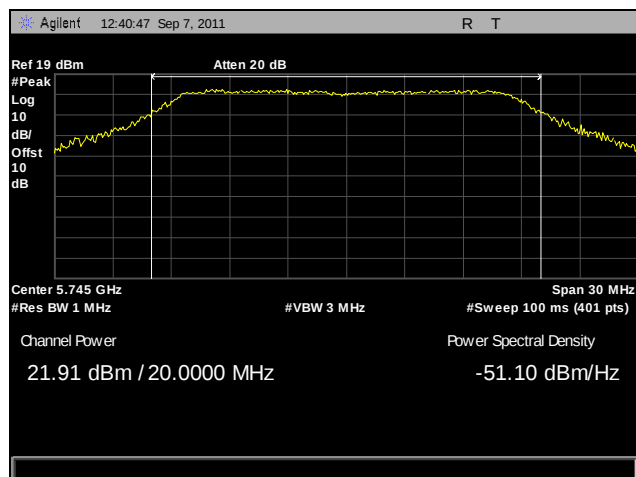
Plot 40. Peak Power Output, Low Channel, 802.11n 20 MHz, Port A
