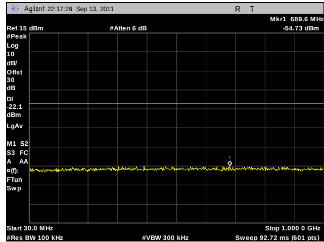
Plot 251. Conducted Spurious Emissions, High Channel, 802.11n 40 MHz, Port B, 30 MHz – 1 GHz
