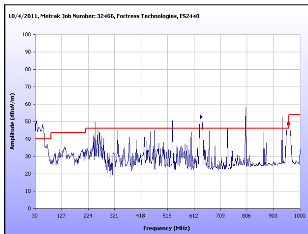
Plot 185. Radiated Spurious Emissions, Low Channel, 802.11n 40 MHz, Sector Antenna, 30 MHz – 1 GHz Note: Emissions which exceed the limit are digital emissions.
