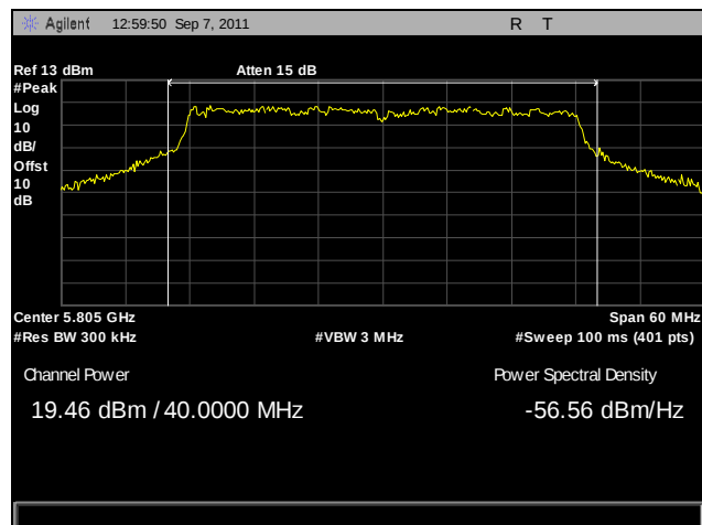
Plot 50. Peak Power Output, Mid Channel, 802.11n 40 MHz, Port B
