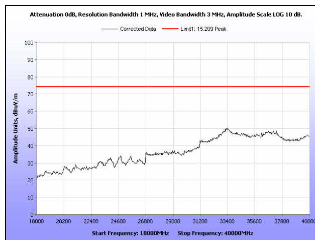
Plot 84. Radiated Spurious Emissions, Mid Channel, 802.11a, Omni Antenna, 18 GHz – 40 GHz, Peak
