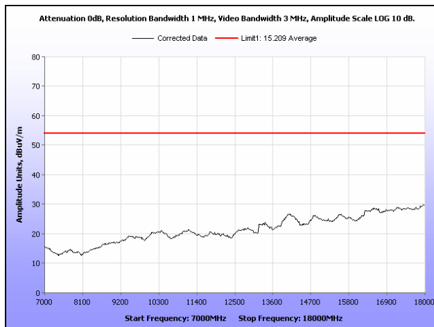
Plot 197. Radiated Spurious Emissions, Mid Channel, 802.11n 40 MHz, Sector Antenna, 7 GHz – 18 GHz, Average
