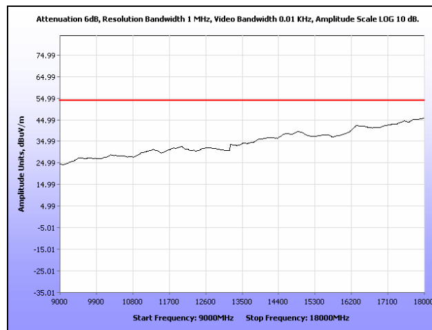
Plot 105. Radiated Spurious Emissions, Mid Channel, 802.11n 20 MHz, Omni Antenna, 9 GHz – 18 GHz, Average
