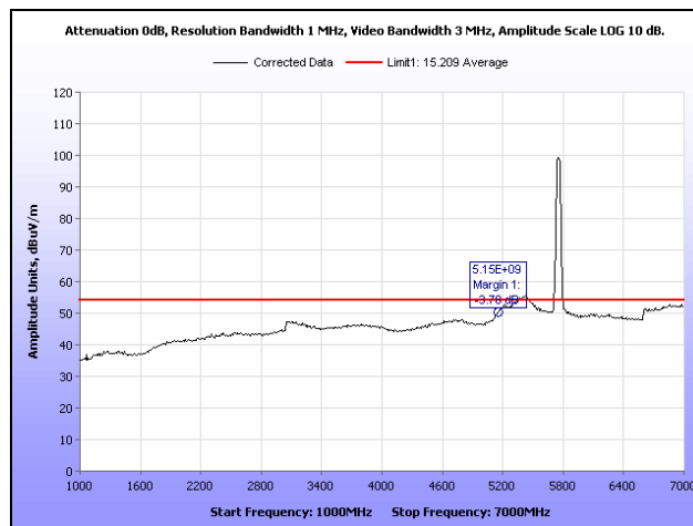
Plot 186. Radiated Spurious Emissions, Low Channel, 802.11n 40 MHz, Sector Antenna, 1 GHz – 7 GHz, Average
