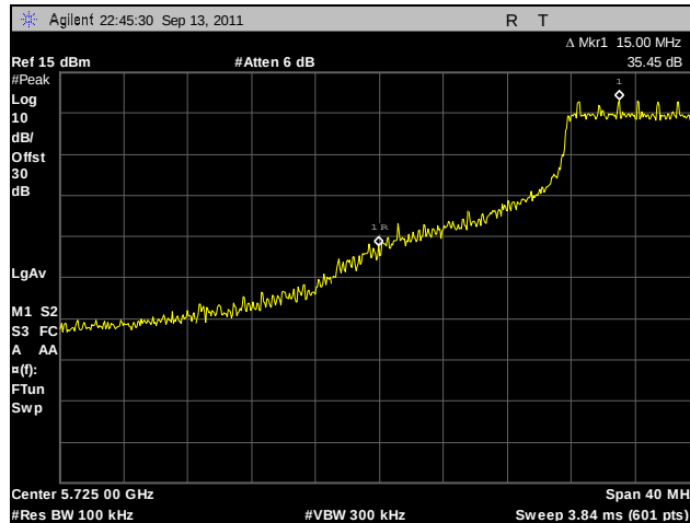
Plot 254. Conducted Band Edge, Low Channel, 802.11a, Port A
