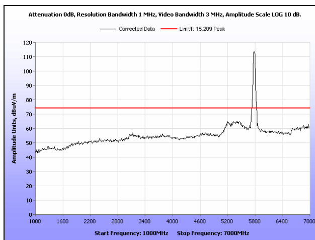
Plot 196. Radiated Spurious Emissions, Mid Channel, 802.11n 40 MHz, Sector Antenna, 1 GHz – 7 GHz, Peak
