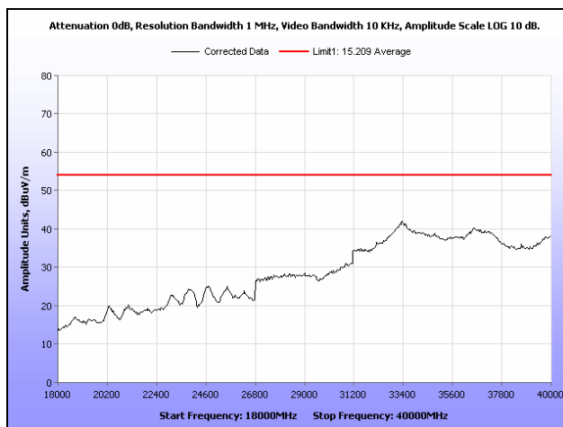
Plot 99. Radiated Spurious Emissions, Low Channel, 802.11n 20 MHz, Omni Antenna, 18 GHz – 40 GHz, Average
