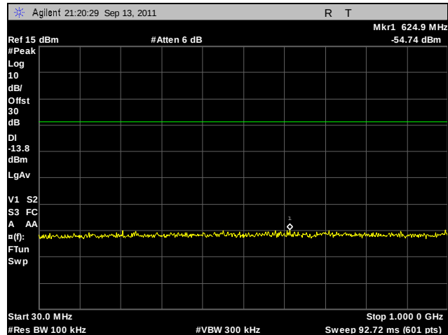
Plot 218. Conducted Spurious Emissions, Low Channel, 802.11n 20 MHz, Port A, 30 MHz – 1 GHz
