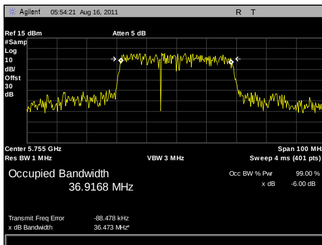
Plot 34. 99% Occupied Bandwidth, Low Channel, 802.11n 40 MHz, Port B
