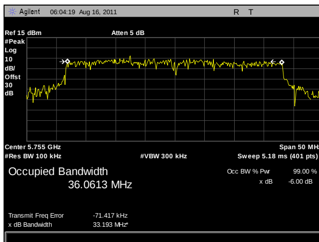
Plot 19. 6 dB Occupied Bandwidth, Low Channel, 802.11n 40 MHz, Port B
