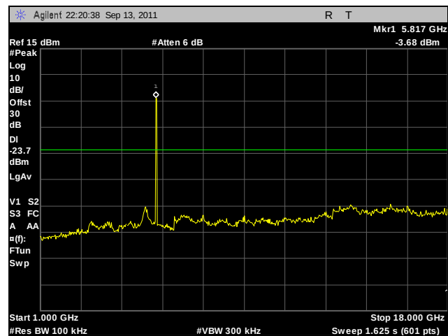
Plot 234. Conducted Spurious Emissions, High Channel, 802.11n 20 MHz, Port B, 1 GHz – 18 GHz
