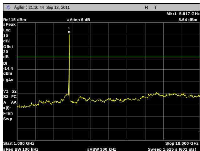
Plot 225. Conducted Spurious Emissions, High Channel, 802.11n 20 MHz, Port A, 1 GHz – 18 GHz
