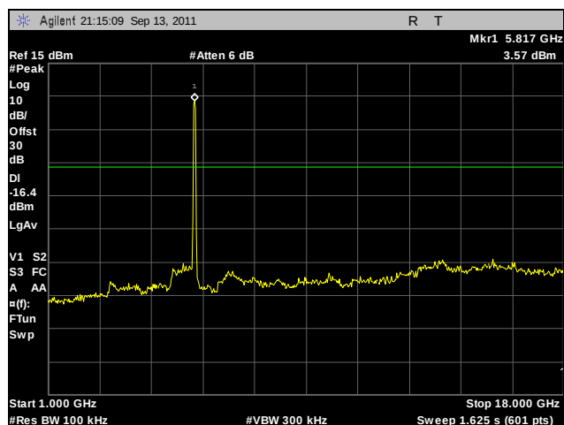
Plot 243. Conducted Spurious Emissions, High Channel, 802.11n 40 MHz, Port A, 1 GHz – 18 GHz
