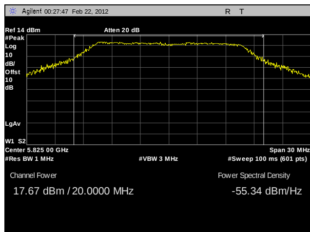
Plot 57. Peak Power Output, High Channel, 802.11n 20 MHz, Port A, Sector Antenna
