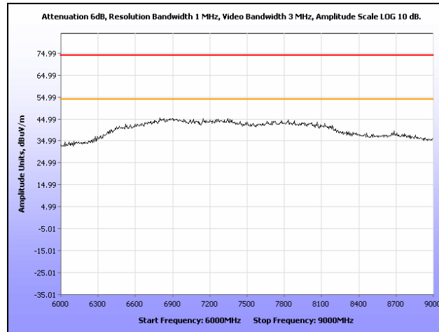
Plot 128. Radiated Spurious Emissions, Mid Channel, 802.11n 40 MHz, Omni Antenna, 6 GHz – 9 GHz
