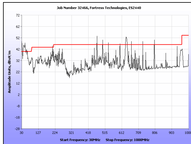
Plot 177. Radiated Spurious Emissions, High Channel, 802.11n 20 MHz, Sector Antenna, 30 MHz – 1 GHz
