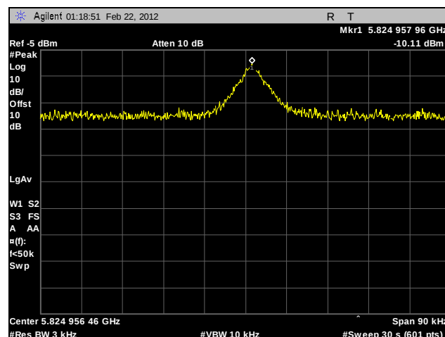
Plot 311. Peak Power Spectral Density, High Channel, 802.11a 20 MHz, Port B, Sector Antenna
