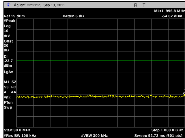
Plot 233. Conducted Spurious Emissions, High Channel, 802.11n 20 MHz, Port B, 30 MHz – 1 GHz
