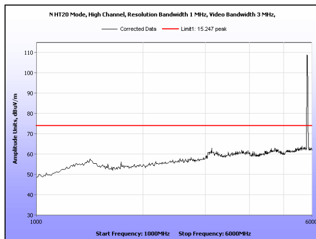
Plot 111. Radiated Spurious Emissions, High Channel, 802.11n 20 MHz, Omni Antenna, 1 GHz – 6 GHz, Peak
