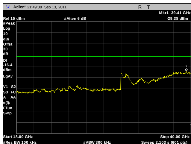
Plot 244. Conducted Spurious Emissions, High Channel, 802.11n 40 MHz, Port A, 18 GHz – 40 GHz
