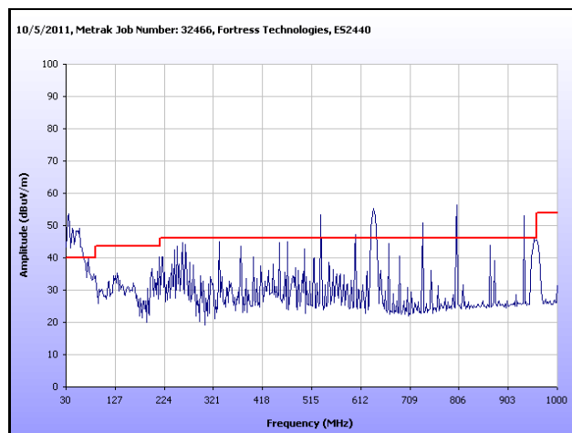
Plot 125. Radiated Spurious Emissions, Mid Channel, 802.11n 40 MHz, Omni Antenna, 30 MHz – 1 GHz Note: Emissions which exceed the limit are digital emissions.
