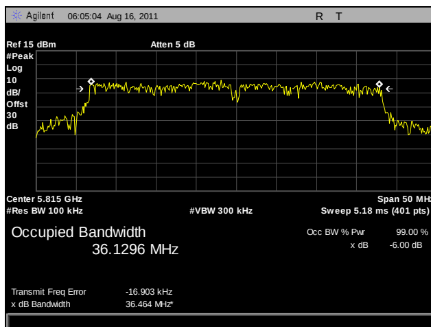
Plot 21. 6 dB Occupied Bandwidth, High Channel, 802.11n 40 MHz, Port B
