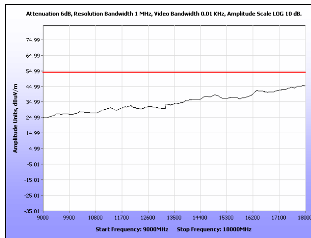
Plot 89. Radiated Spurious Emissions, High Channel, 802.11a, Omni Antenna, 9 GHz – 18 GHz, Average
