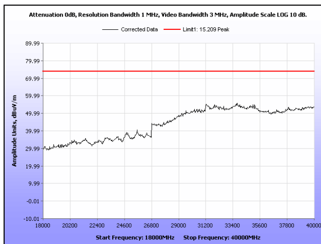
Plot 200. Radiated Spurious Emissions, Mid Channel, 802.11n 40 MHz, Sector Antenna, 18 GHz – 40 GHz, Peak
