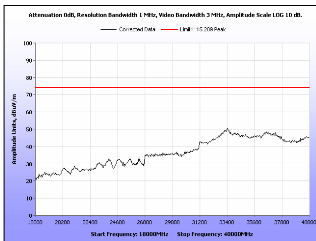
Plot 92. Radiated Spurious Emissions, High Channel, 802.11a, Omni Antenna, 18 GHz – 40 GHz, Peak
