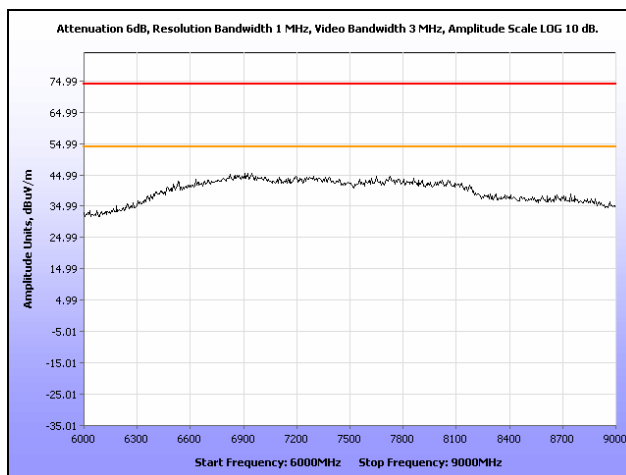
Plot 136. Radiated Spurious Emissions, High Channel, 802.11n 40 MHz, Omni Antenna, 6 GHz – 9 GHz
