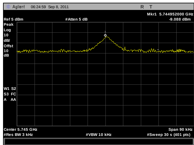
Plot 271. Peak Power Spectral Density, Low Channel, 802.11a 20 MHz, Port A
