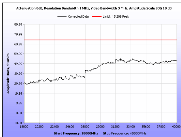
Plot 184. Radiated Spurious Emissions, High Channel, 802.11n 20 MHz, Sector Antenna, 18 GHz – 40 GHz, Peak
