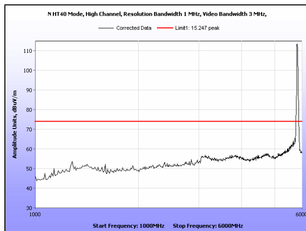
Plot 135. Radiated Spurious Emissions, High Channel, 802.11n 40 MHz, Omni Antenna, 1 GHz – 6 GHz, Peak
