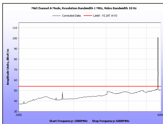
Plot 77. Radiated Spurious Emissions, Mid Channel, 802.11a, Omni Antenna, 1 GHz – 6 GHz, Average
