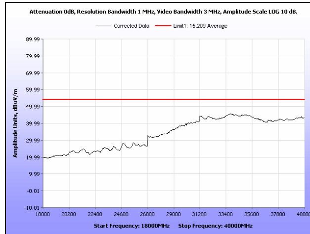
Plot 175. Radiated Spurious Emissions, Mid Channel, 802.11n 20 MHz, Sector Antenna, 18 GHz – 40 GHz, Average
