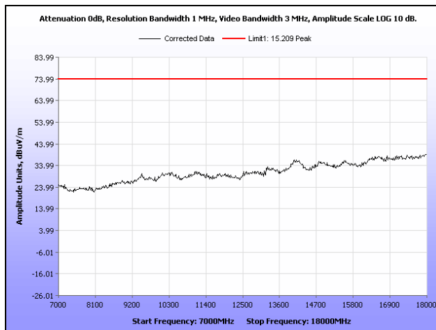
Plot 153. Radiated Spurious Emissions, Mid Channel, 802.11a, Sector Antenna, 7 GHz – 18 GHz, Peak
