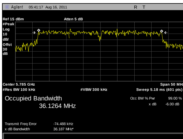
Plot 17. 6 dB Occupied Bandwidth, Mid Channel, 802.11n 40 MHz, Port A
