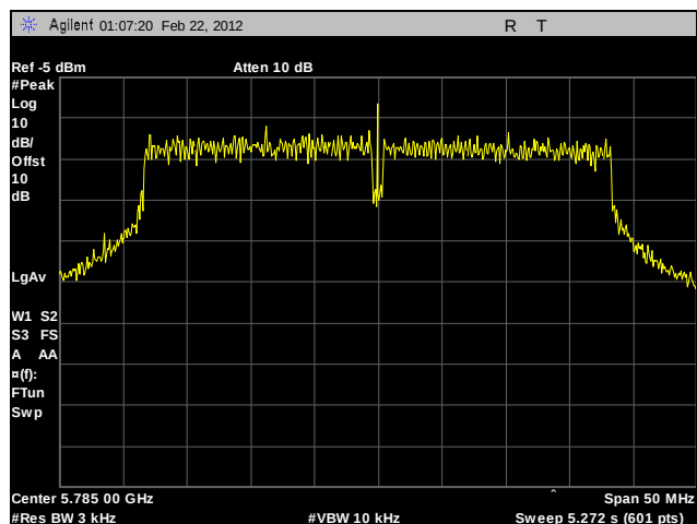
Plot 314. Peak Power Spectral Density, Mid Channel, 802.11a 40 MHz, Port A, Sector Antenna, Determination
