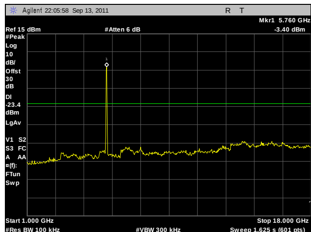
Plot 246. Conducted Spurious Emissions, Low Channel, 802.11n 40 MHz, Port B, 1 GHz – 18 GHz
