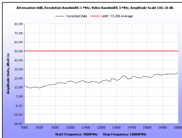
Plot 159. Radiated Spurious Emissions, High Channel, 802.11a, Sector Antenna, 7 GHz – 18 GHz, Average
