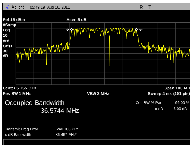
Plot 31. 99% Occupied Bandwidth, Low Channel, 802.11n 40 MHz, Port A
