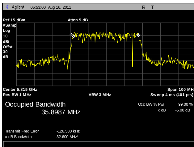
Plot 36. 99% Occupied Bandwidth, High Channel, 802.11n 40 MHz, Port B
