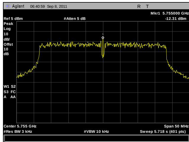
Plot 288. Peak Power Spectral Density, Low Channel, 802.11a 40 MHz, Port B, Determination
