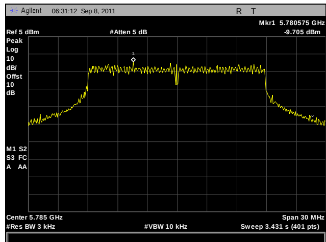
Plot 272. Peak Power Spectral Density, Mid Channel, 802.11a 20 MHz, Port A, Determination
