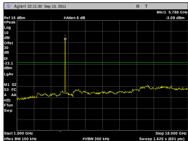
Plot 249. Conducted Spurious Emissions, Mid Channel, 802.11n 40 MHz, Port B, 1 GHz – 18 GHz
