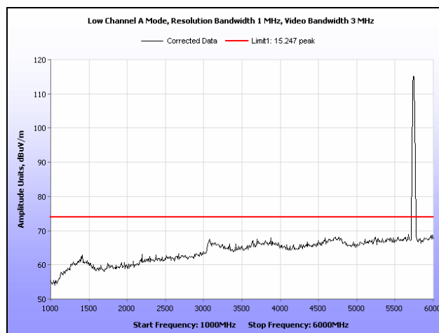
Plot 69. Radiated Spurious Emissions, Low Channel, 802.11a, Omni Antenna, 1 GHz – 6 GHz, Peak
