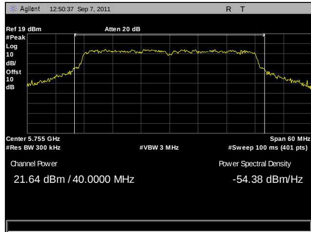
Plot 49. Peak Power Output, Low Channel, 802.11n 40 MHz, Port B
