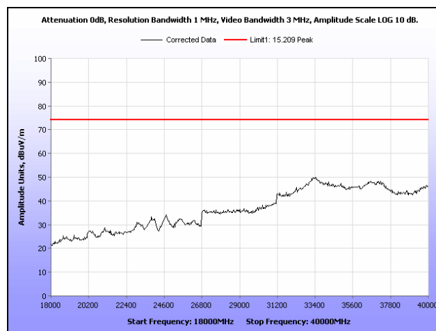
Plot 75. Radiated Spurious Emissions, Low Channel, 802.11a, Omni Antenna, 18 GHz – 40 GHz, Peak
