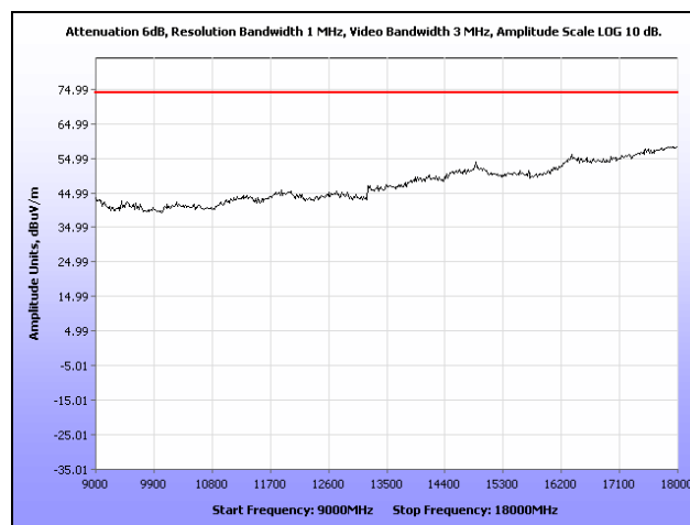
Plot 130. Radiated Spurious Emissions, Mid Channel, 802.11n 40 MHz, Omni Antenna, 9 GHz – 18 GHz, Peak
