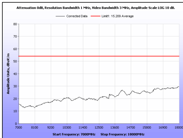
Plot 144. Radiated Spurious Emissions, Low Channel, 802.11a, Sector Antenna, 7 GHz – 18 GHz, Average
