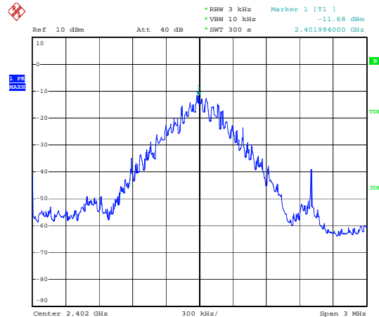
Figure 16. Plot of the Peak Power Spectral Density (Conducted)- DC 3.7V
