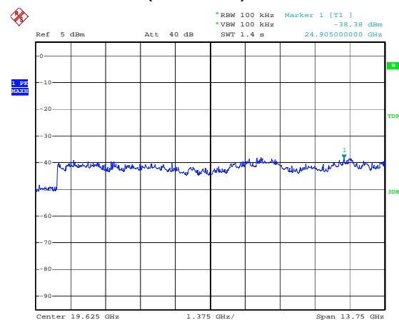
Figure 14. Plot of the Spurious RF conducted emissions – DC 3.7V
