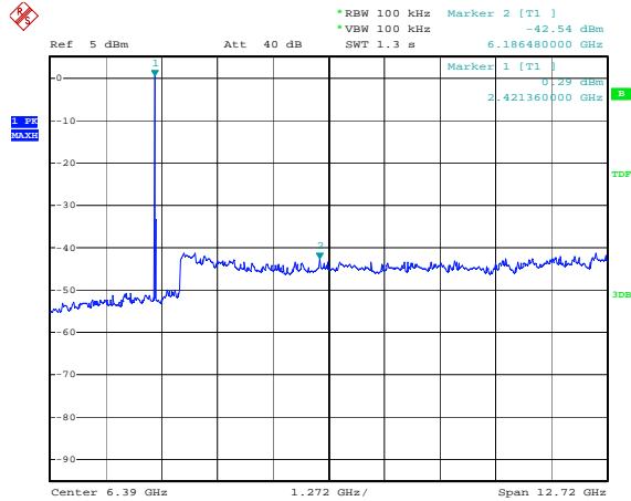
Figure 15. Plot of the Spurious RF conducted emissions – DC 5V
