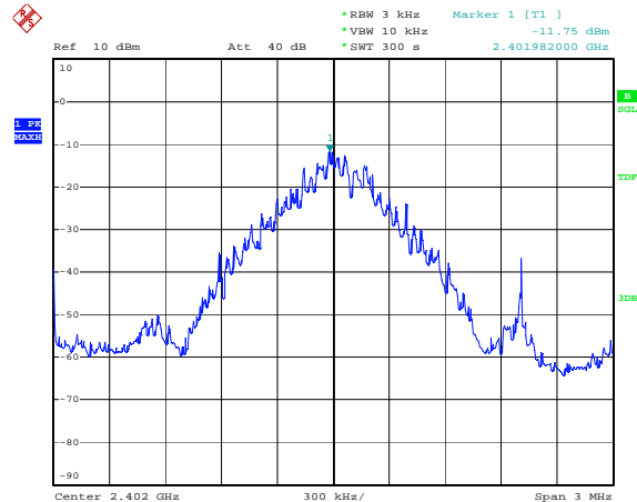
Figure 17. Plot of the Peak Power Spectral Density (Conducted)-DC 5V
