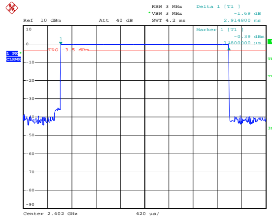
Figure 9. Plot of the Time of Occupancy (Conducted)
