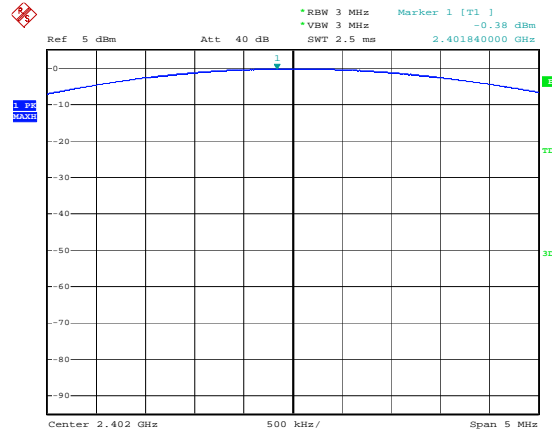
Figure 2. Plot of the Maximum Peak Output Power (Conducted) -DC 5V(charging mode)
