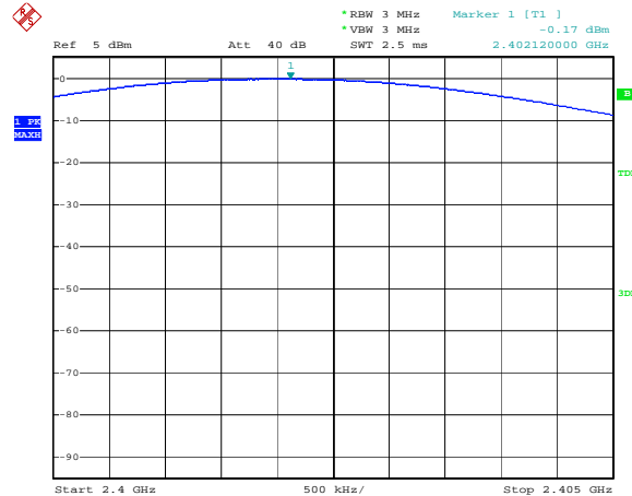
Figure 1. Plot of the Maximum Peak Output Power (Conducted) -DC 3.7V
