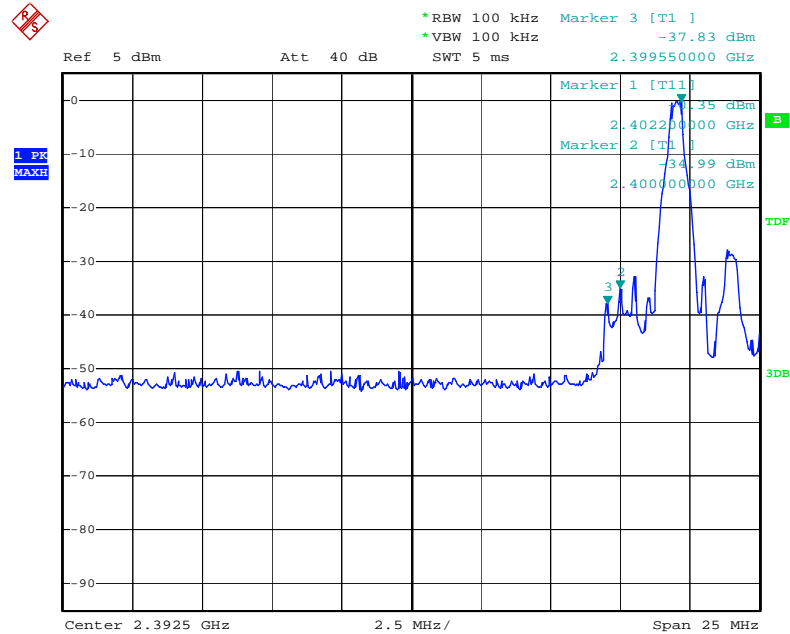
Figure 10. Plot of the Band Edge (Conducted) -DC 3.7V
