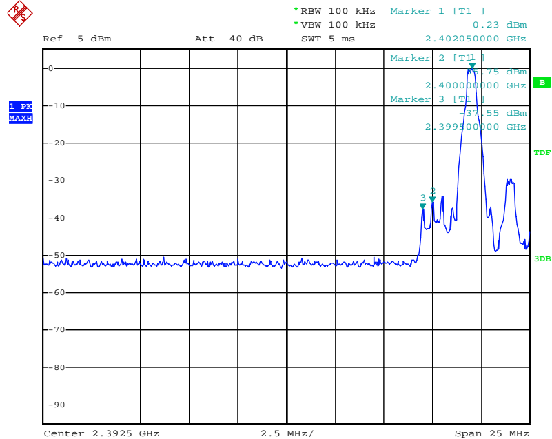
Figure 11. Plot of the Band Edge (Conducted) -DC 5V
