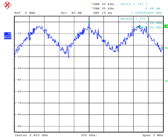
Figure 4. Plot of the Carrier Frequency Separation (Conducted)
