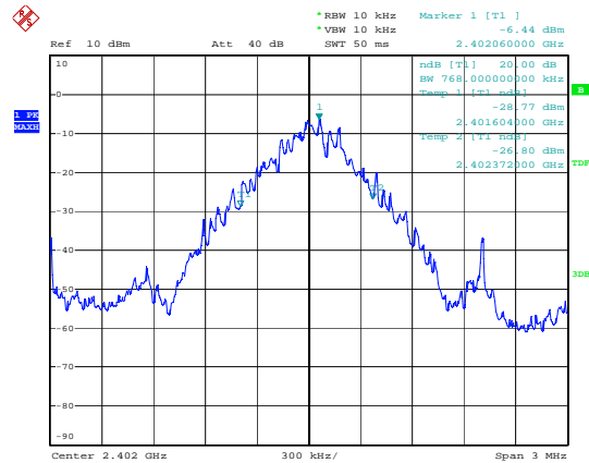
Figure 6. Plot of the 20dB Channel Bandwidth (Conducted)
