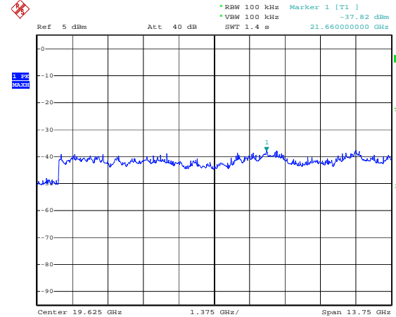
Figure 15. Plot of the Spurious RF conducted emissions – DC 5V
