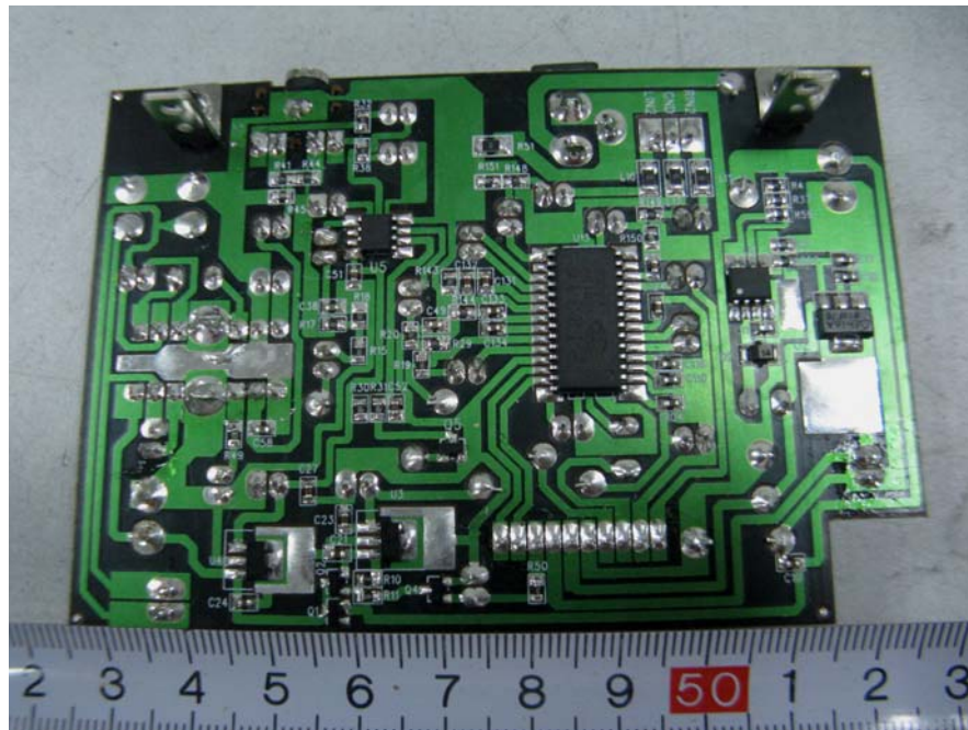
EUT – Audio Output Board Bottom Components View
