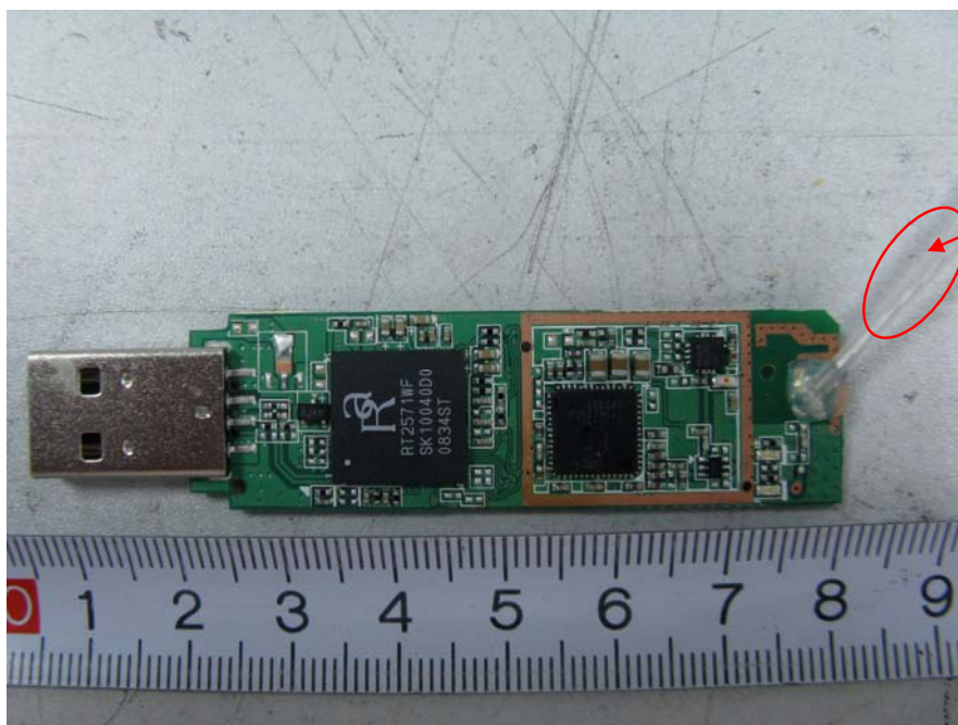
EUT – WIFI Board Top Components View
