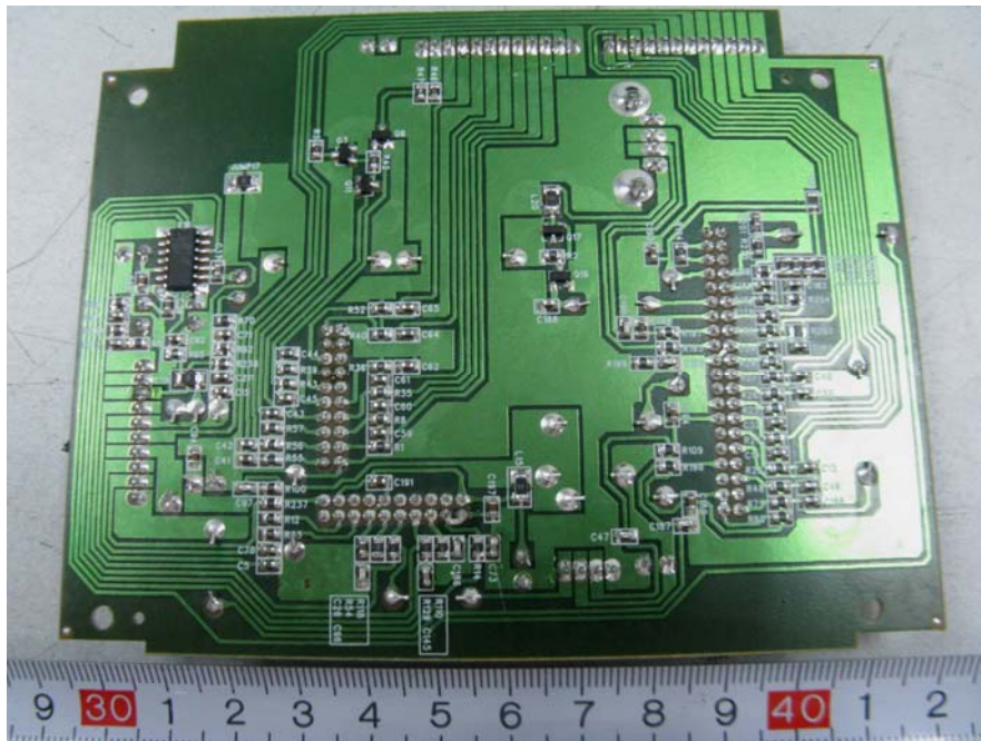
EUT – Main Board 2 Bottom Components View
