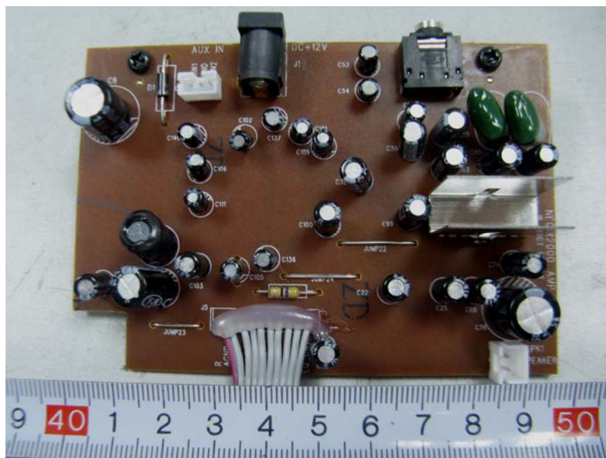
EUT – Audio Output Board Top Components View
