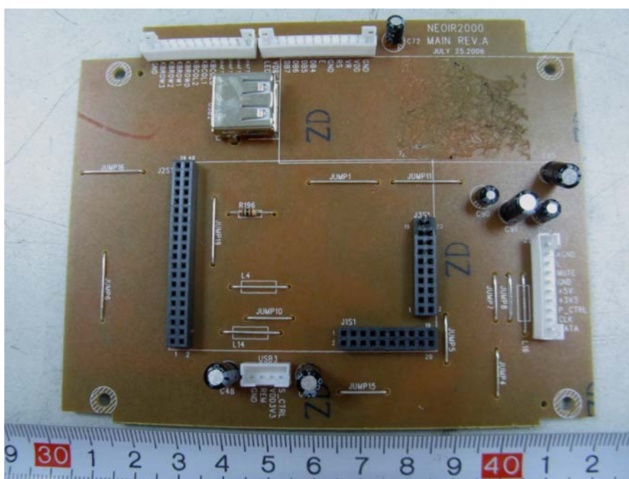
EUT – Main Board 2 Top Components View
