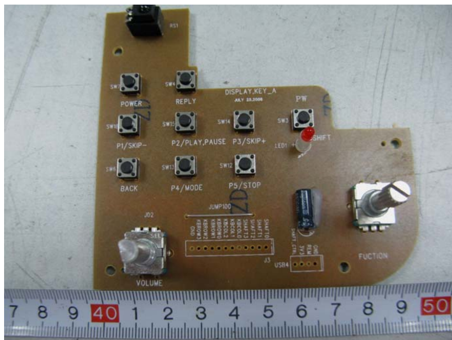
EUT – Control Board Components View
