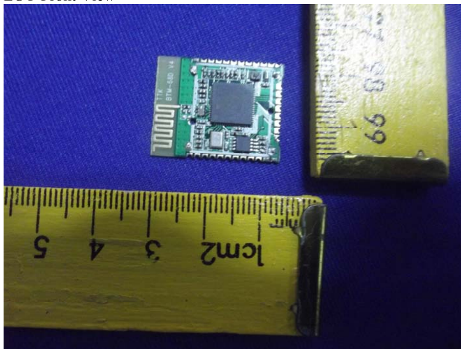
Figure 11 EUT-Front View
