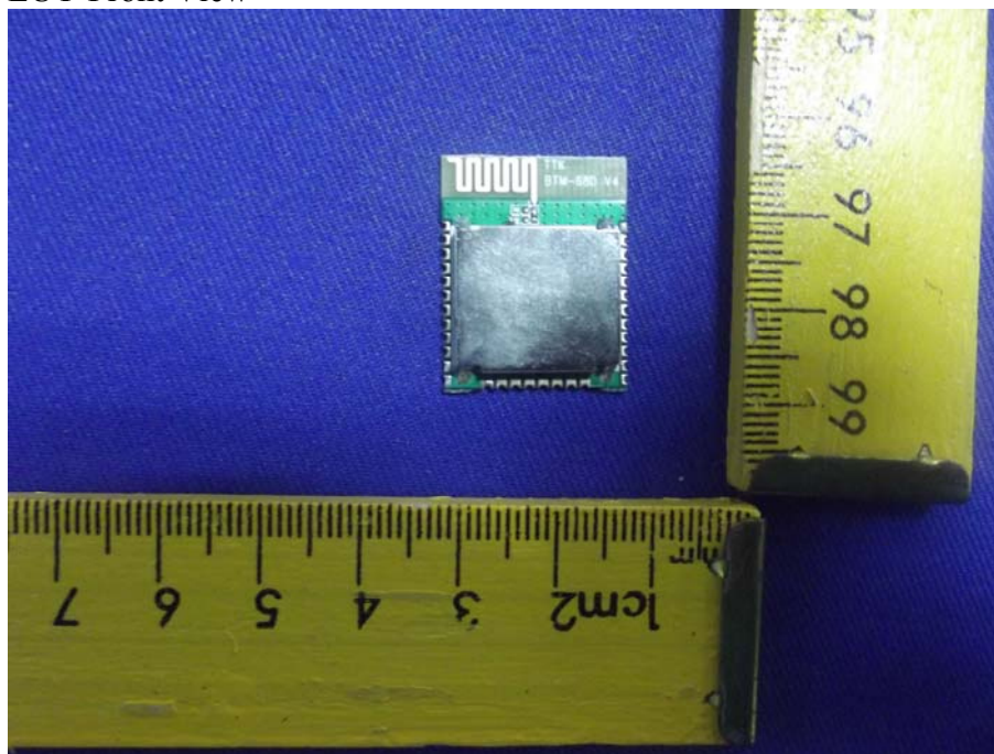
Figure 9 EUT-Front View
