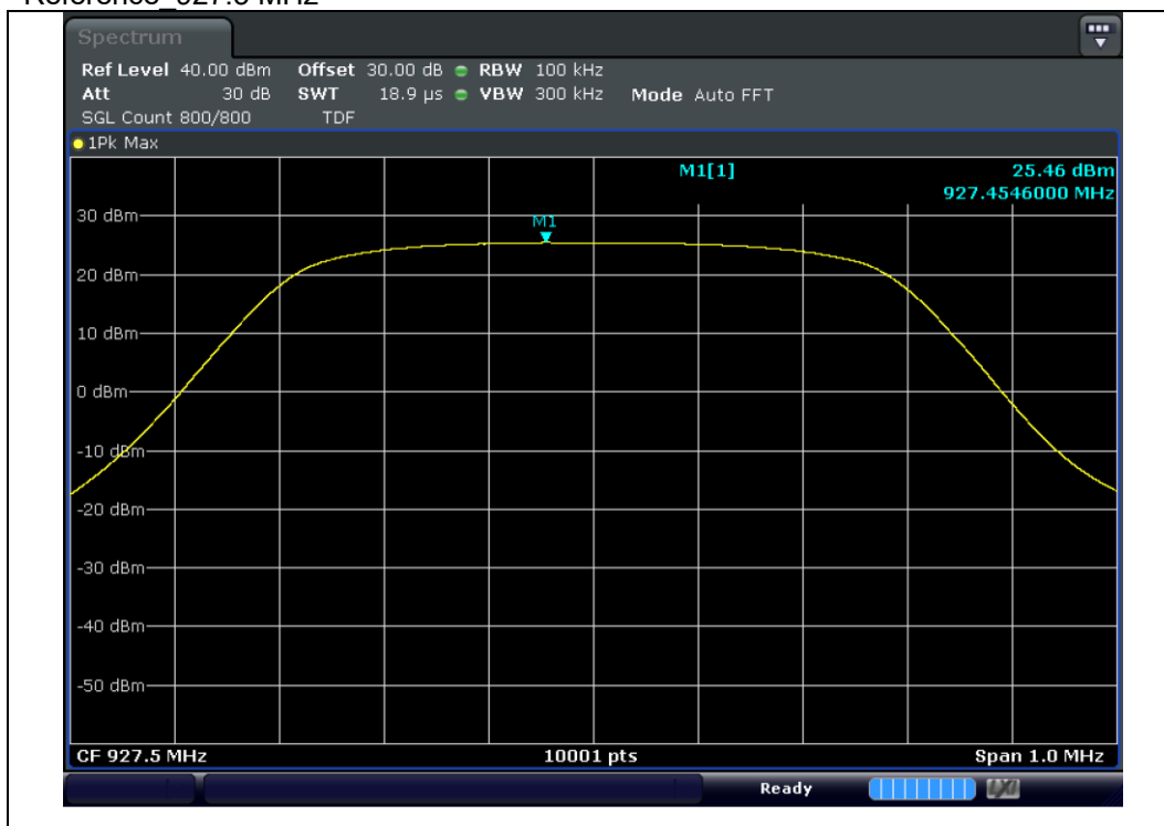
Reference 927.5 MHz
