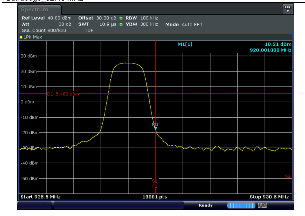
Bandedge 927.5 MHz
