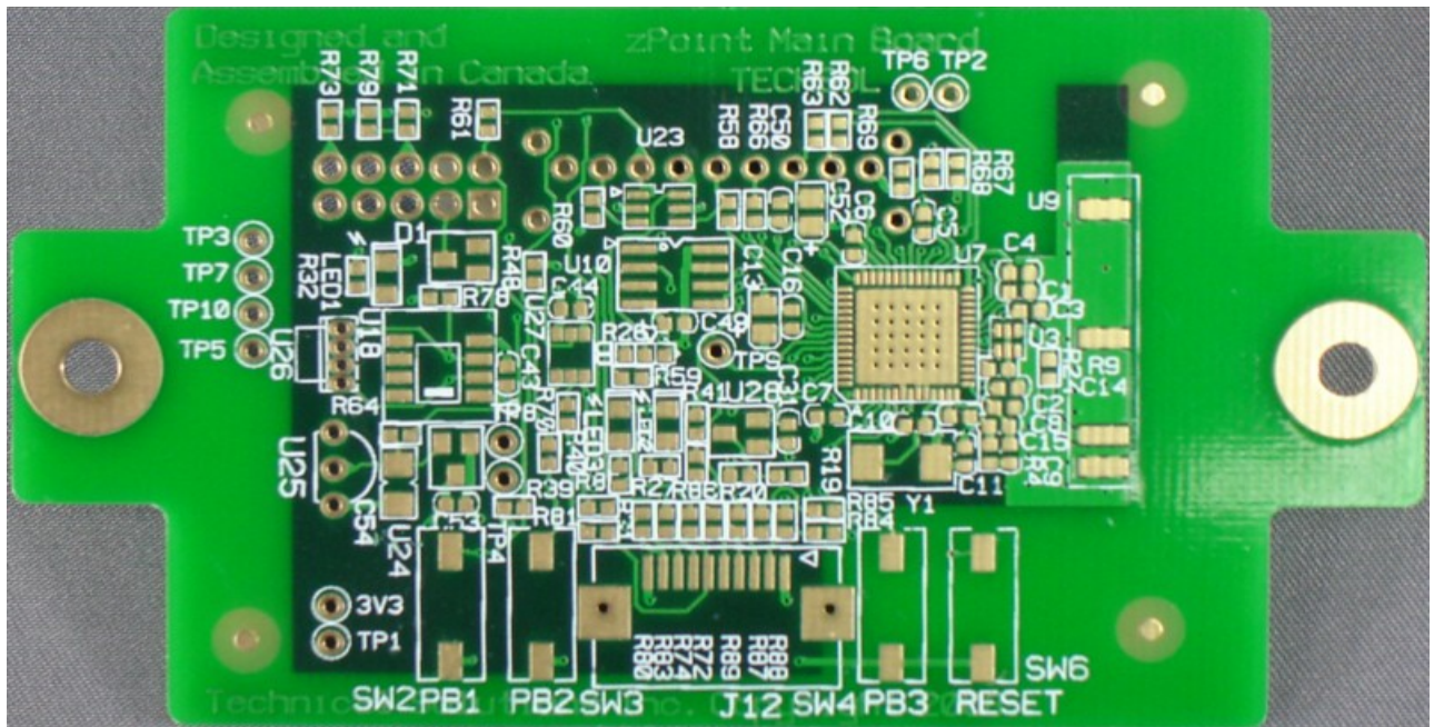
photo 3 Main pcb, Top view
