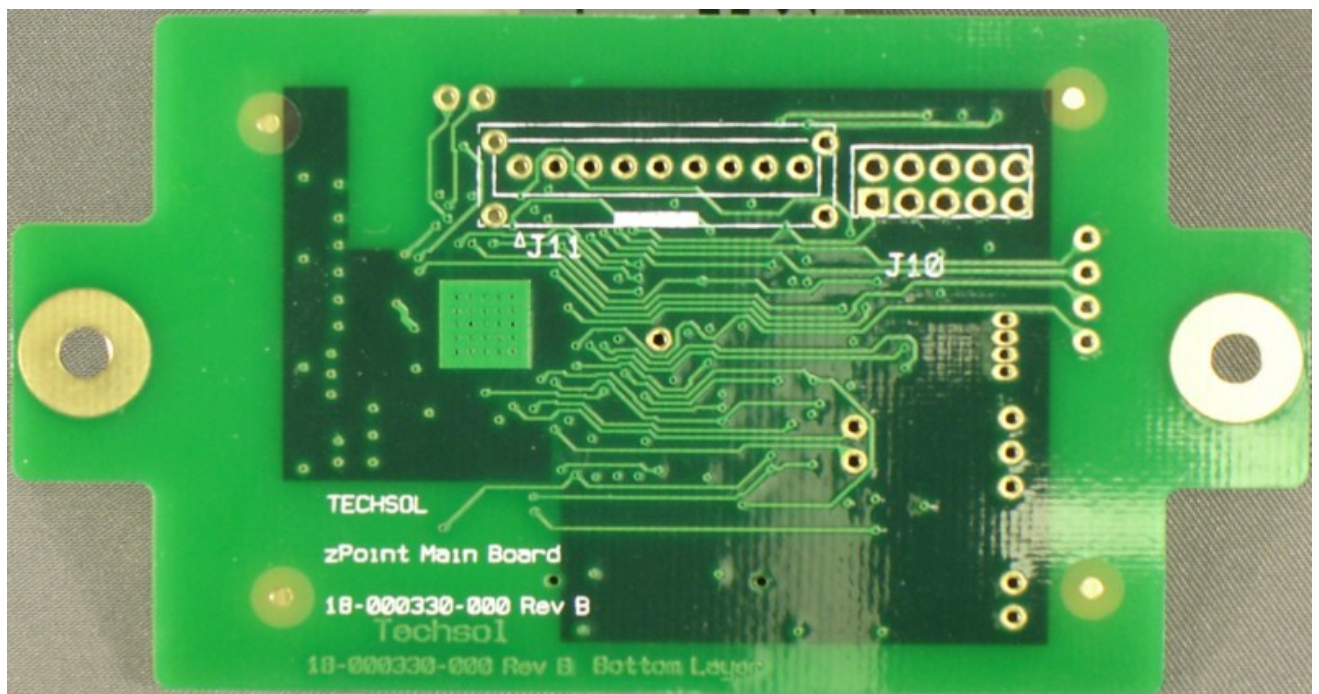
Photo 4 Main pcb, Bottom view
