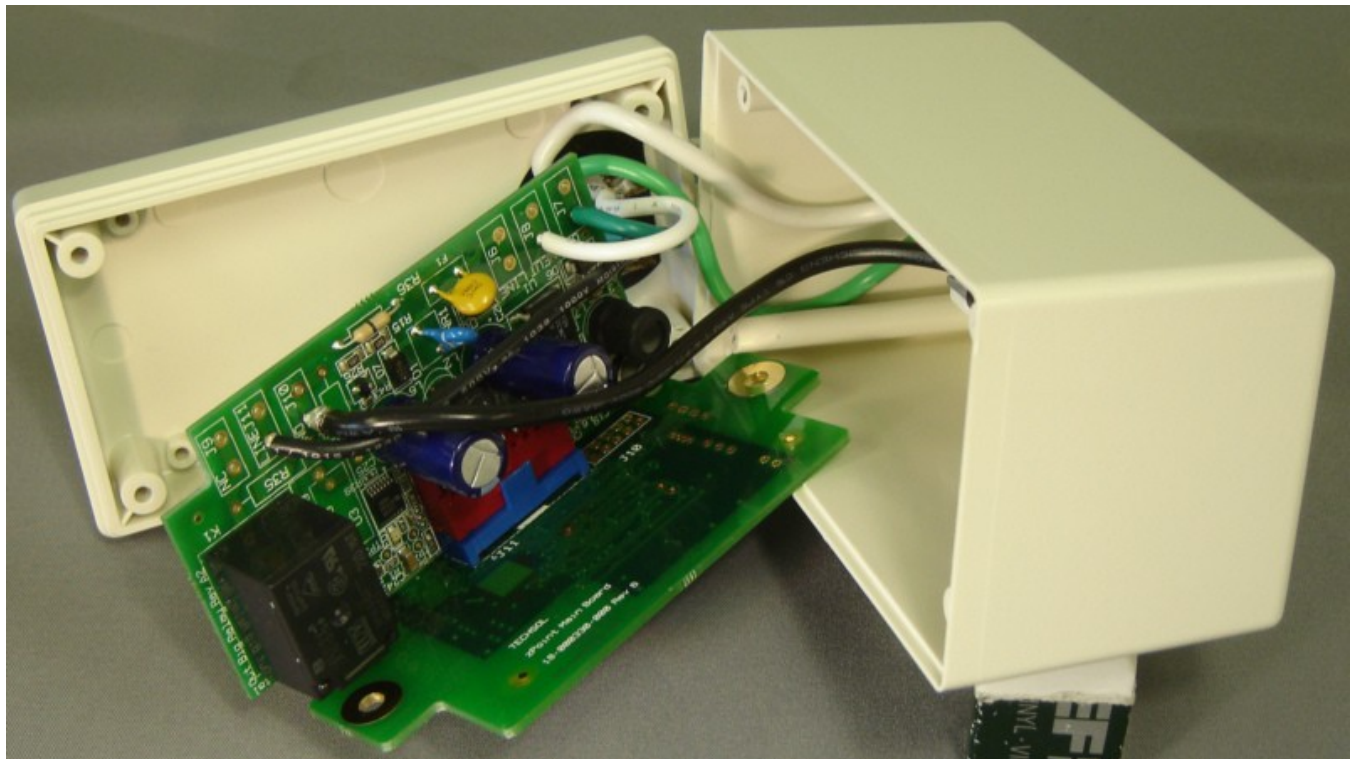
Photo 2 zRY01 internal view 2
