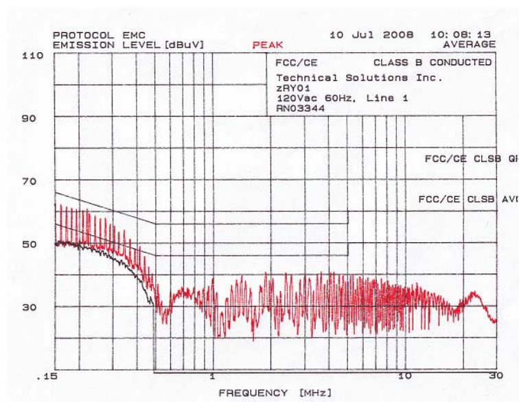
Figure 3: Conducted Emissions Line 1 – 120Vac, 60Hz
