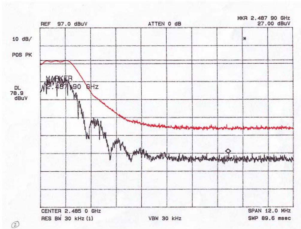
Figure2: Occupied Bandwidth.
