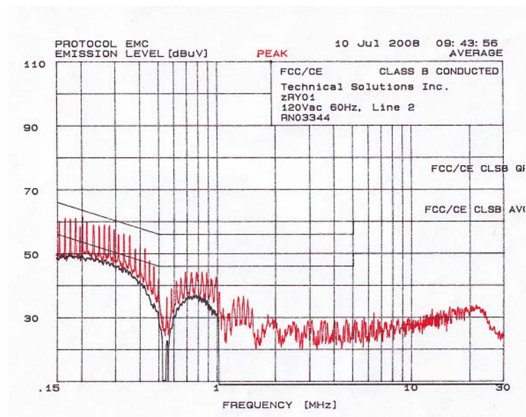
Figure 4: Conducted Emissions Line 2 – 120Vac, 60Hz
