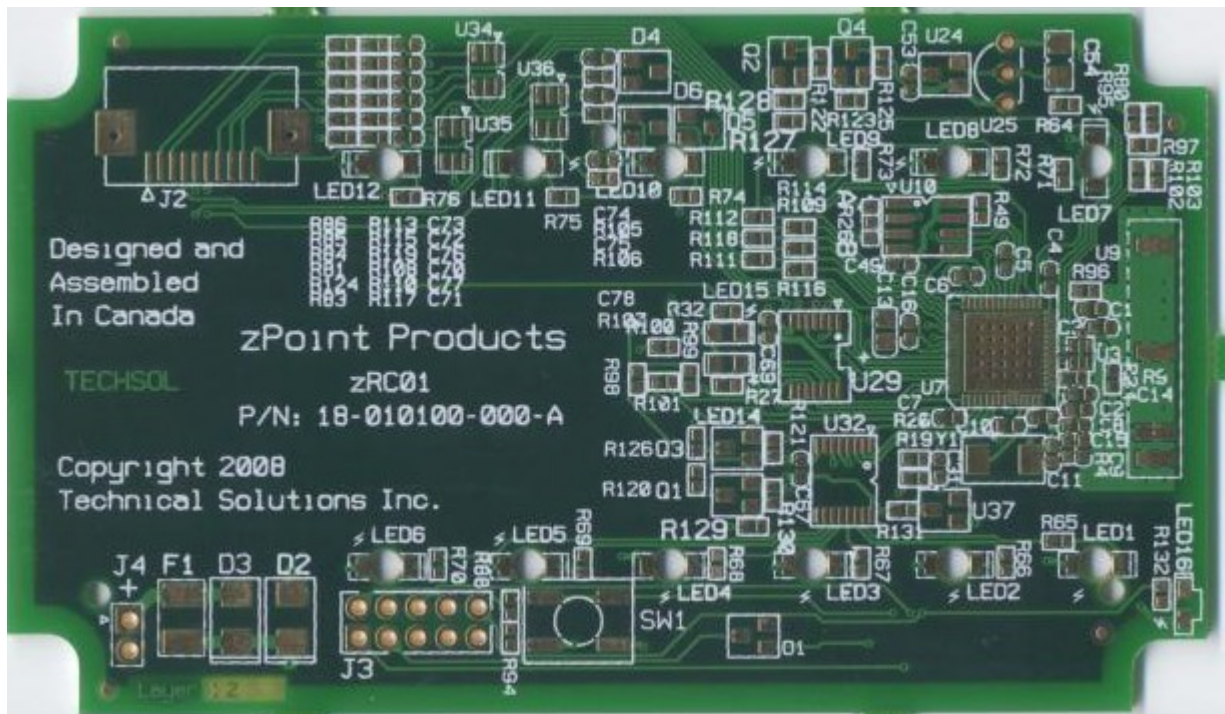
Photo 3 zRC01 Bare PCB Top side
