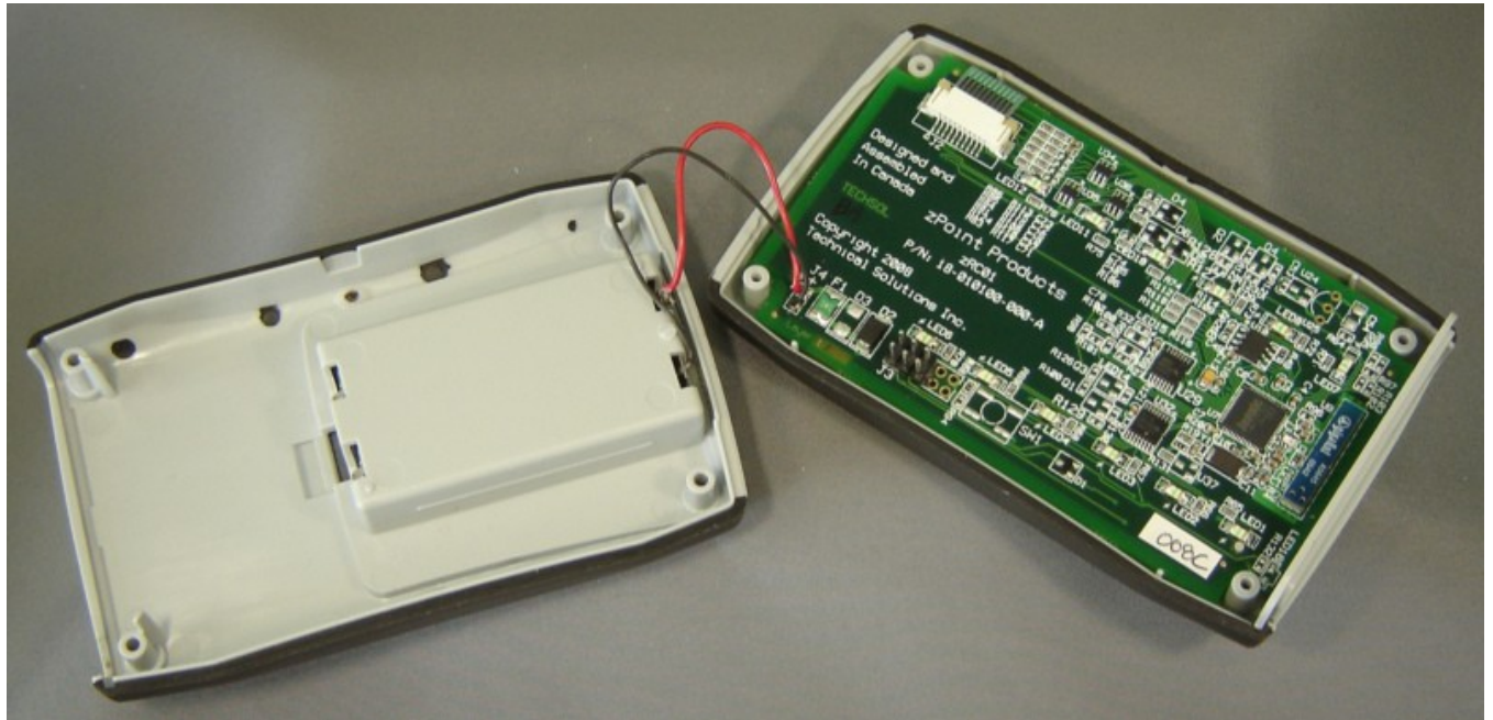
Photo 1 zRC01 Internal view 1
