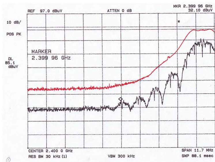
Figure 1.Lower Frequency Band Edge.
