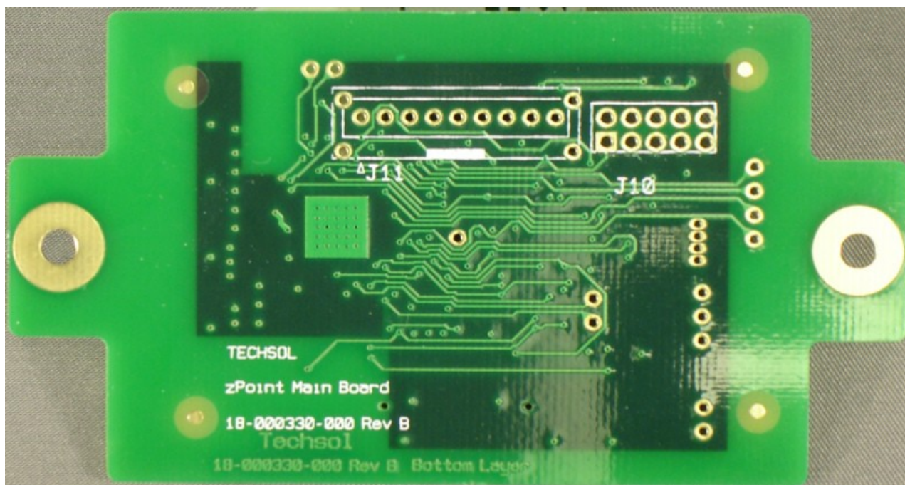
Photo 4 Main pcb, Bottom view
