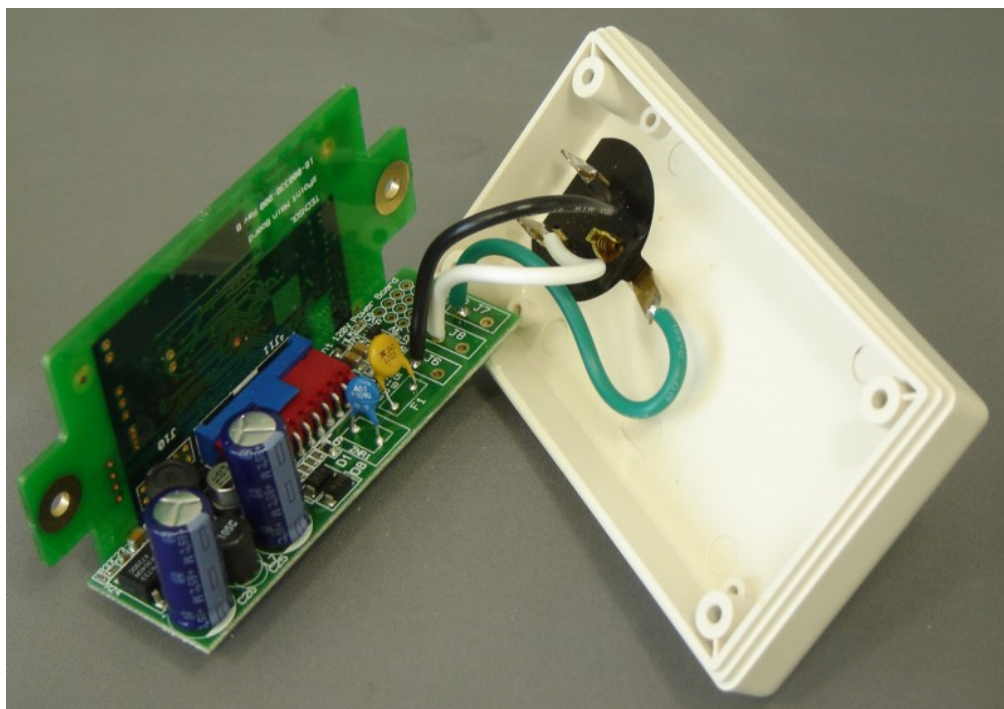
Photo 2 Internal view, with top cover removed
