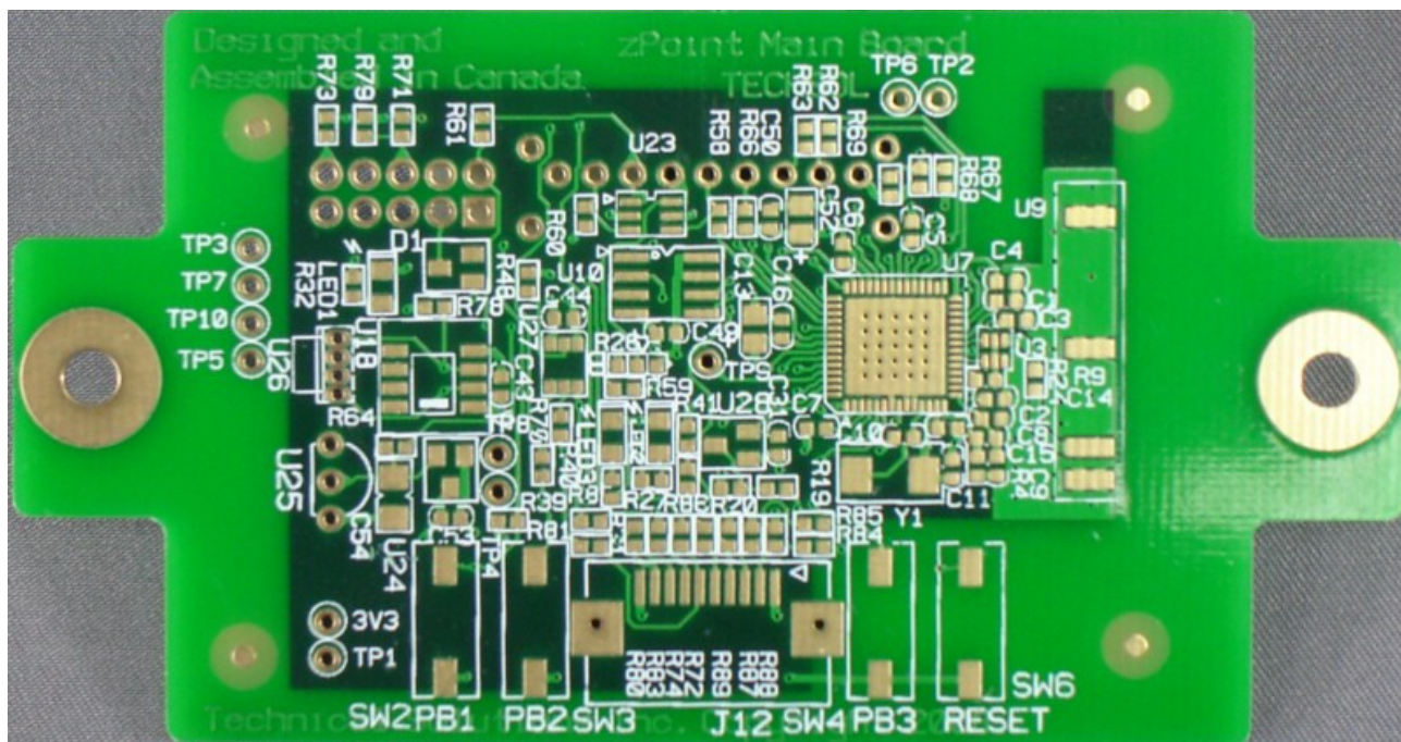
Photo 3 Main pcb, Top view
