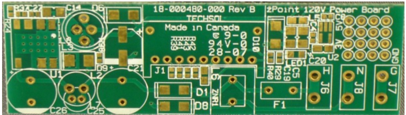
Photo 5 Power Supply pcb, Top view
