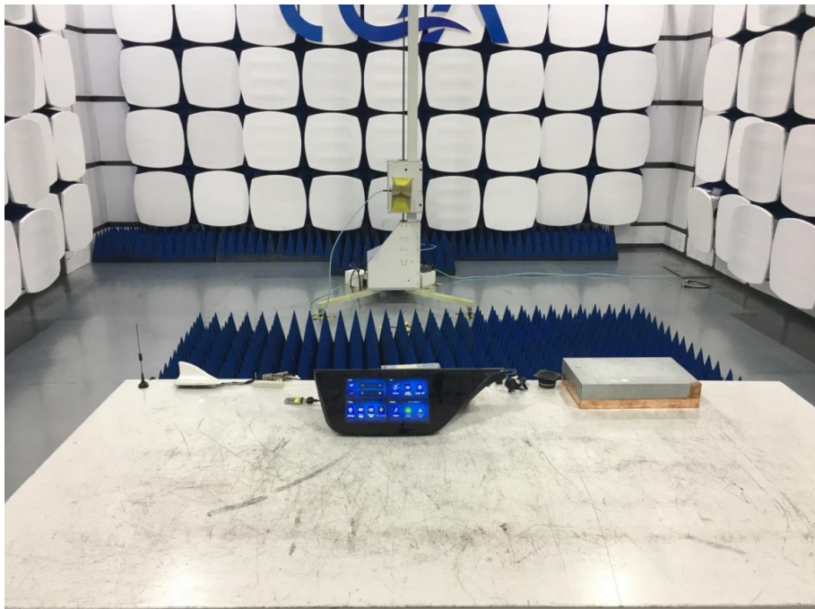
Photograph 2: Set-up for Radiated Emission, above 1GHz
