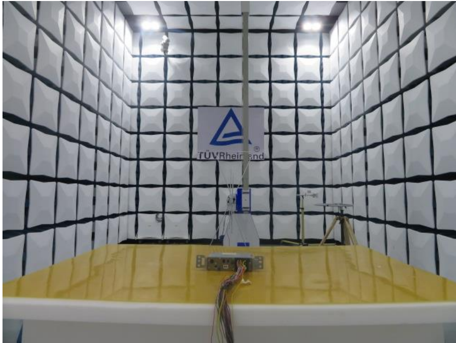
Photograph 3: Set-up for Radiated Spurious Emission, below 1GHz
