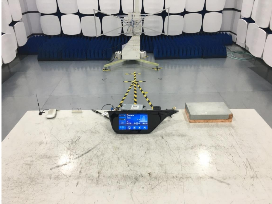
Photograph 1: Set-up for Radiated Emission, below 1GHz
