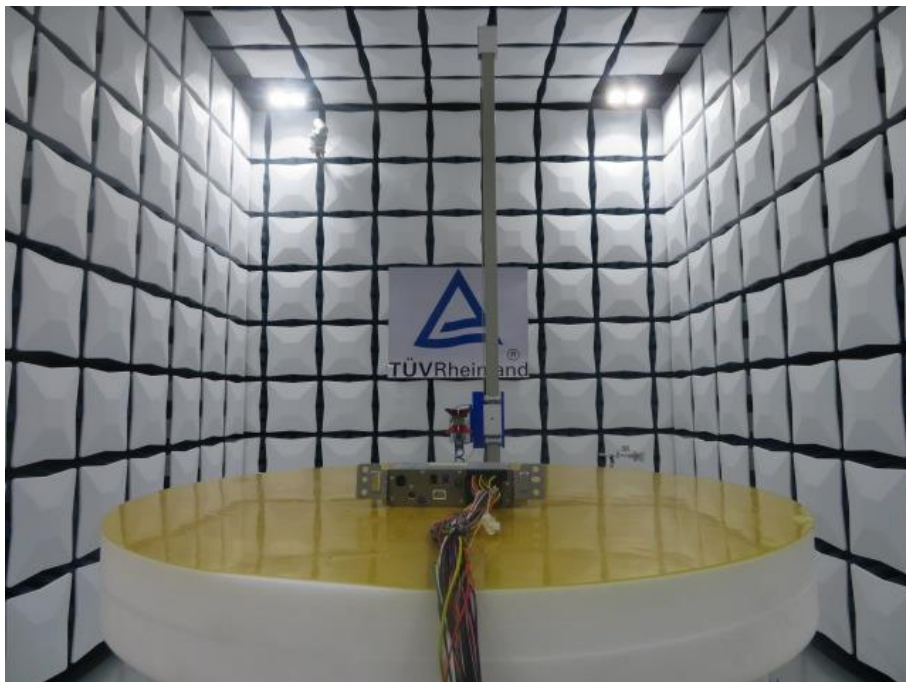
Photograph 4: Set-up for Radiated Spurious Emission, above 1GHz
