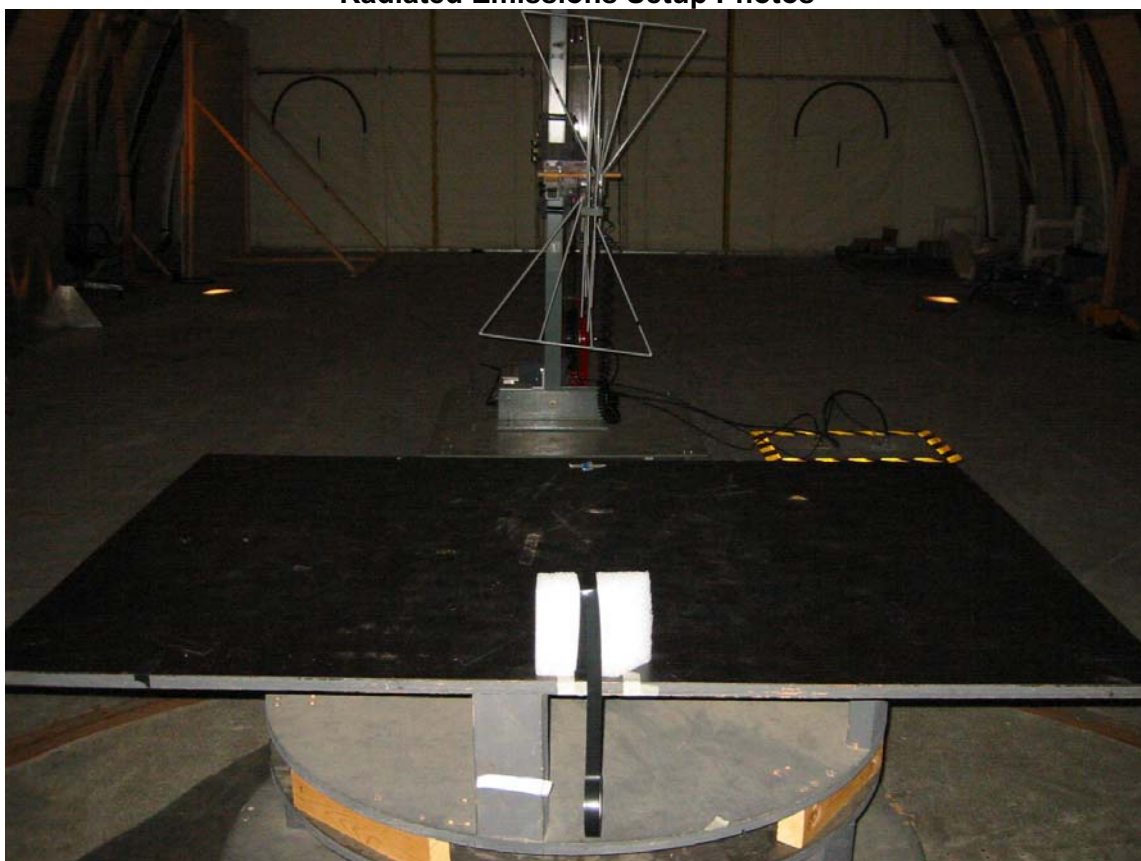
Radiated Emissions Setup Photos
