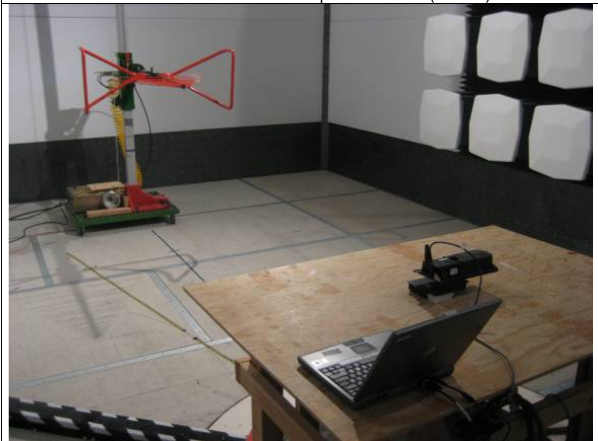
Radiated Emission Test Setup – Rear View (<1GHz)
