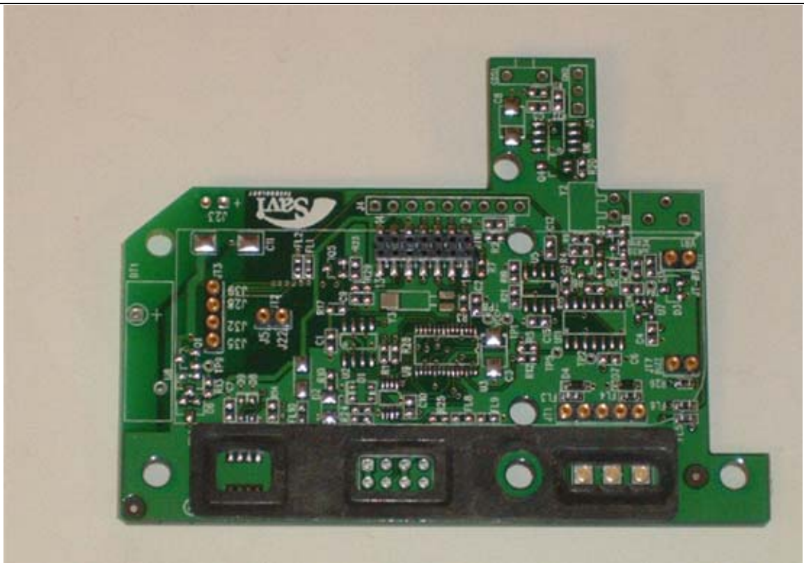
EUT: Sub-PCBA 3 Component View
