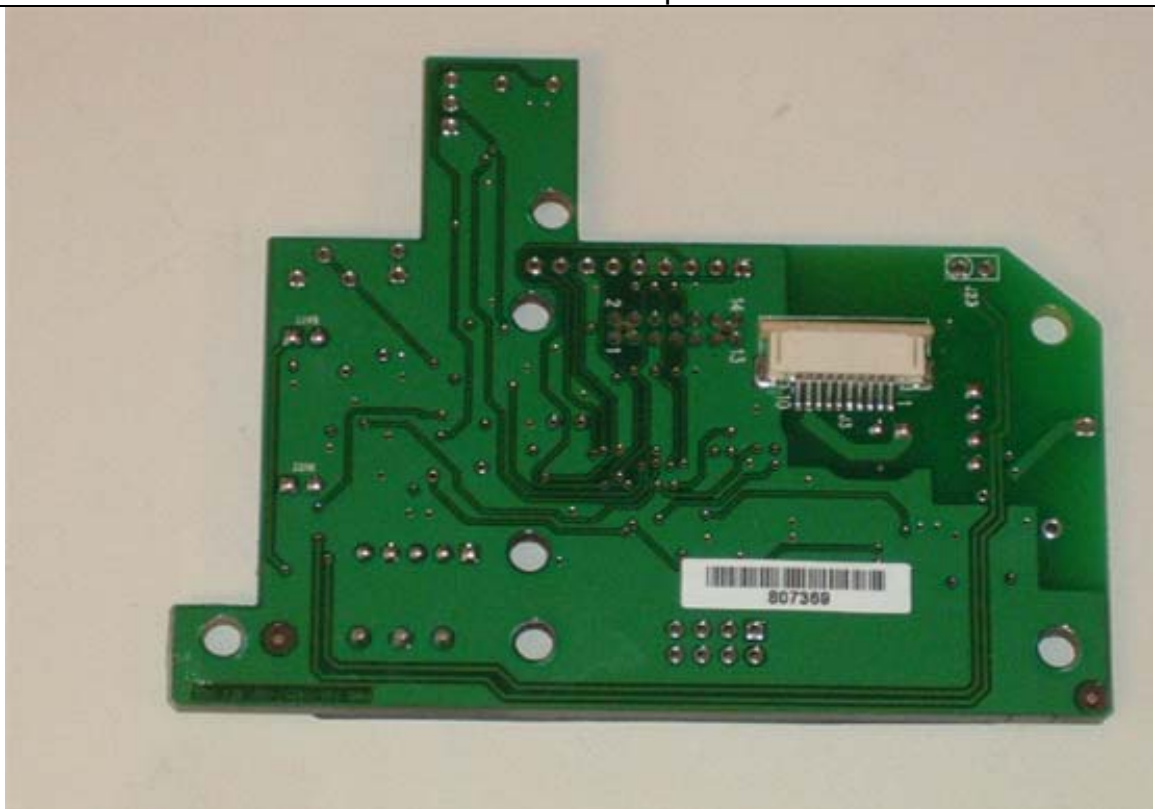
EUT: Sub-PCBA 3 Solder View
