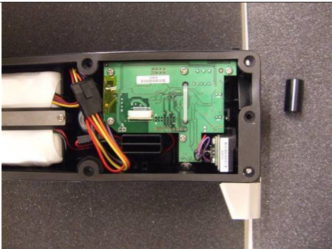
Battery Enclosure and EUT Sub-PCBA 1 View 1
