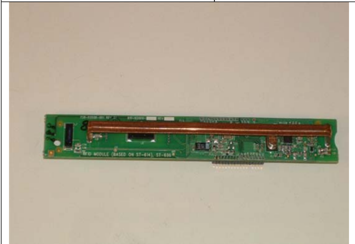
EUT: RFID Main PCBA Antenna View
