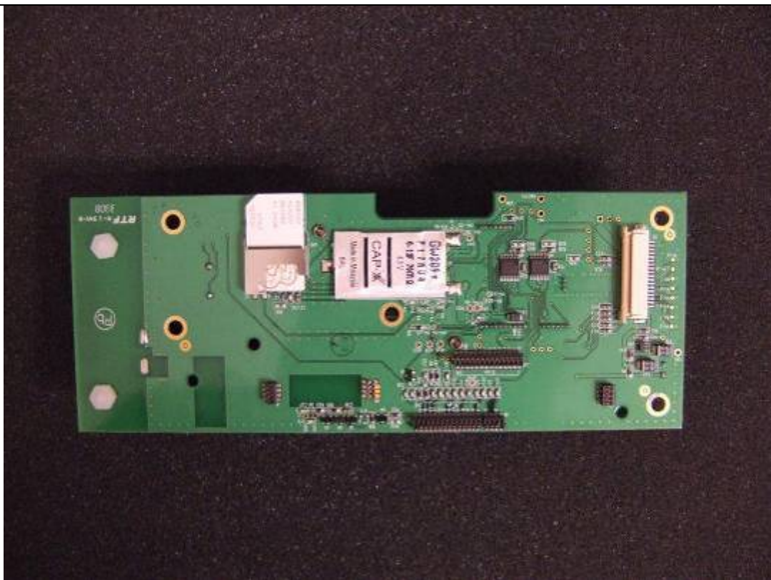
EUT: EUT Main PCBA Solder View
