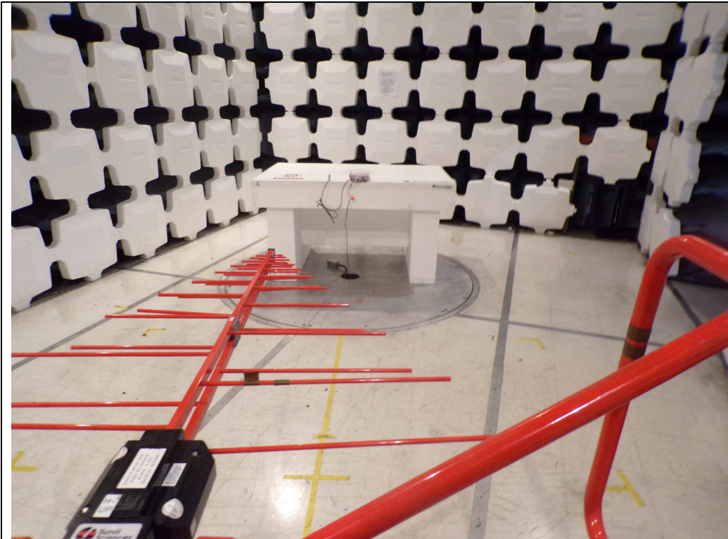
30MHz-1GHz
