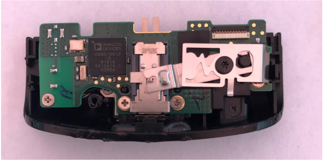
Top Side of Daughter Board PWA
