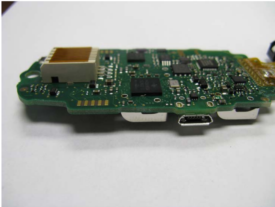
Mother Board Side View - 1
