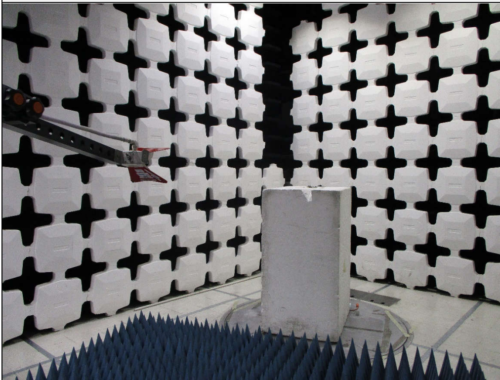
Test Setup for Spurious Radiated Emissions, Above 1-18GHz – Antenna Polarization Vertical
