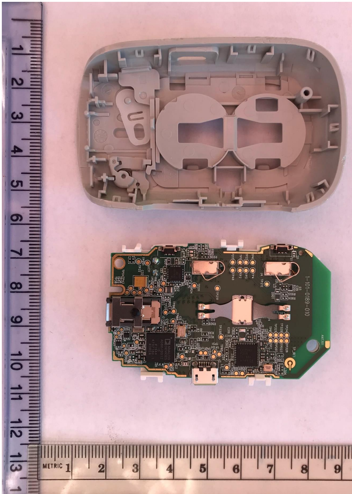
Bottom Housing and PWA
