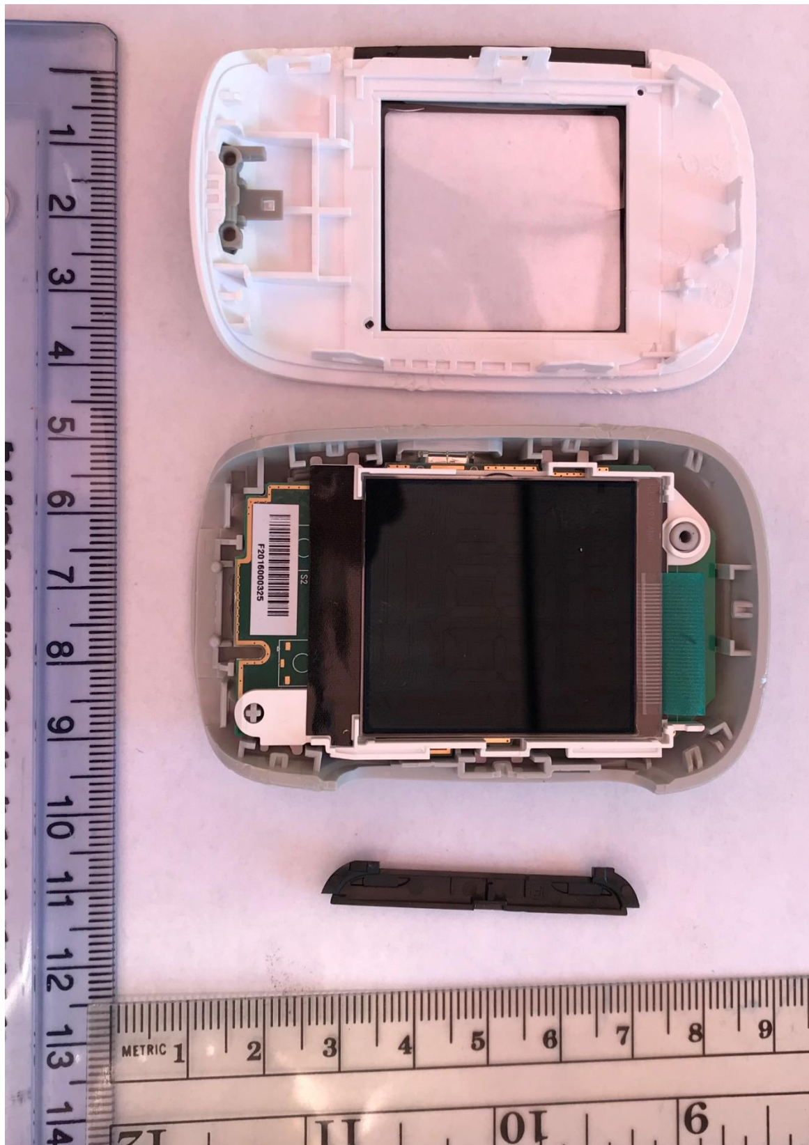
Top Housing, PWA with Display and Plastic Button Plunger
