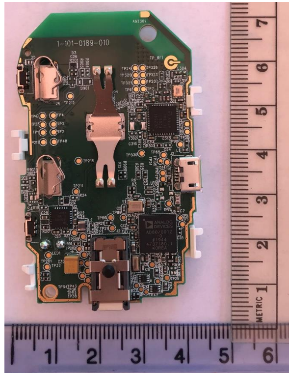
Bottom Side of PWA
