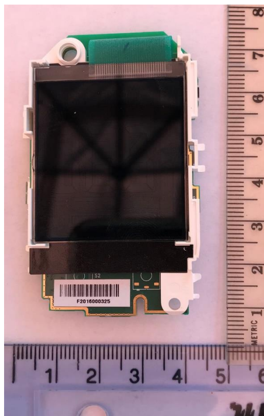
Top Side of PWA with Display
