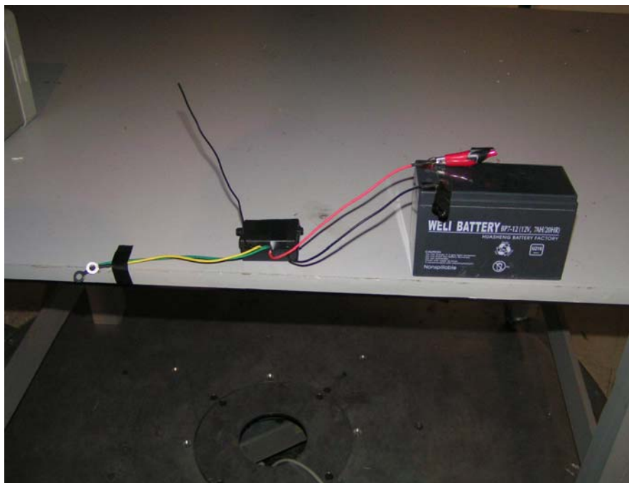
Radiated Emission Test Set-Up View#2
