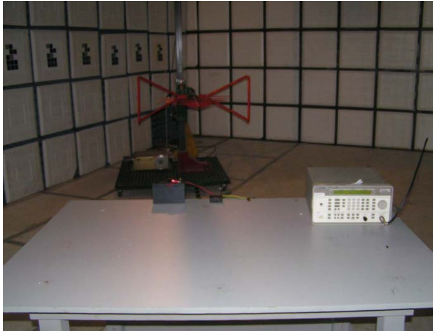
Radiated Emission Test Set-Up View#1
