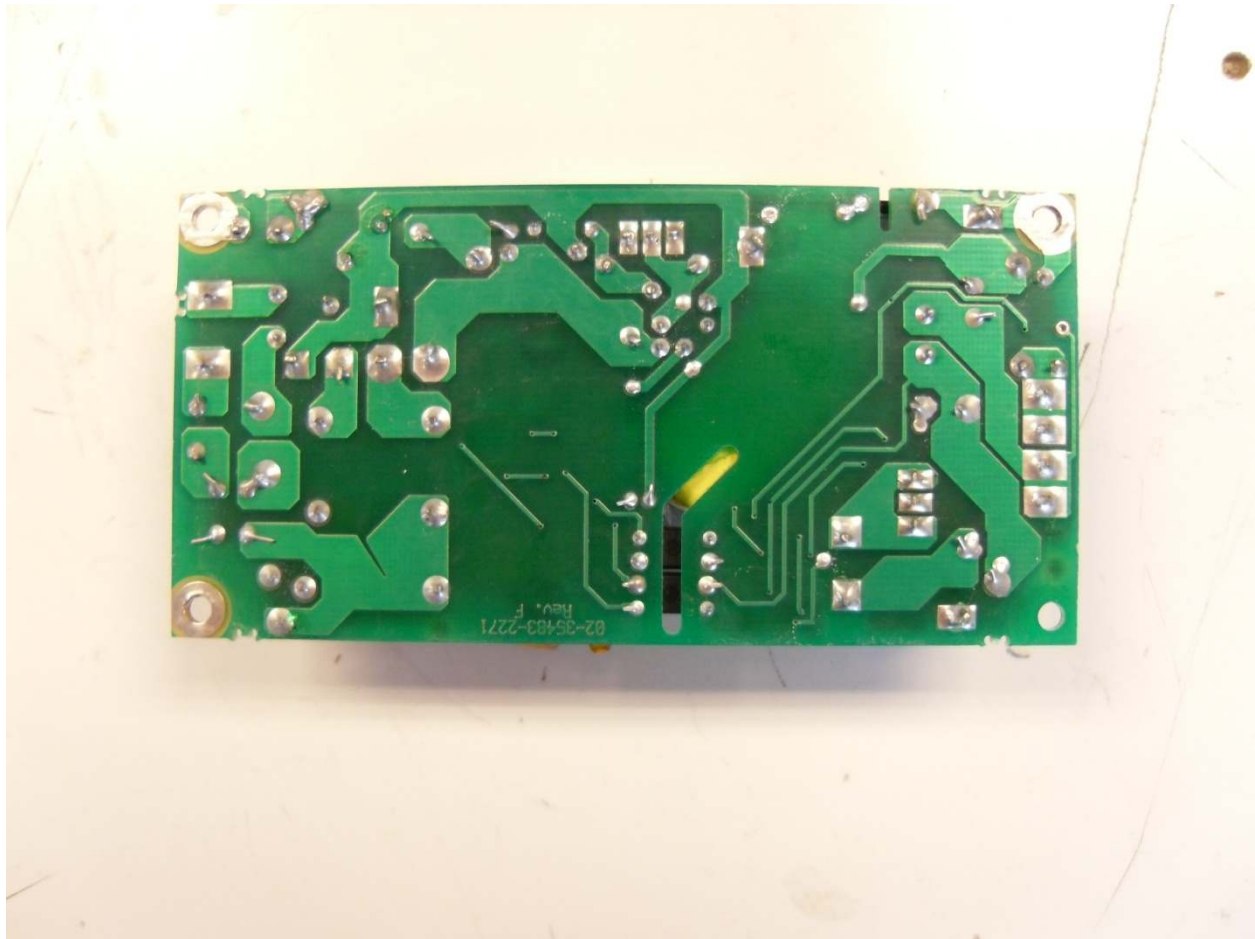
Power Supply (Bottom View)
