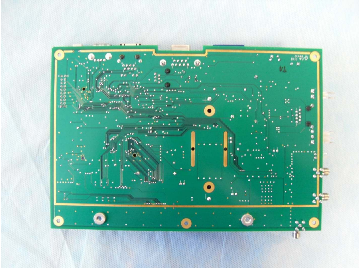
Control Board (Bottom View)
