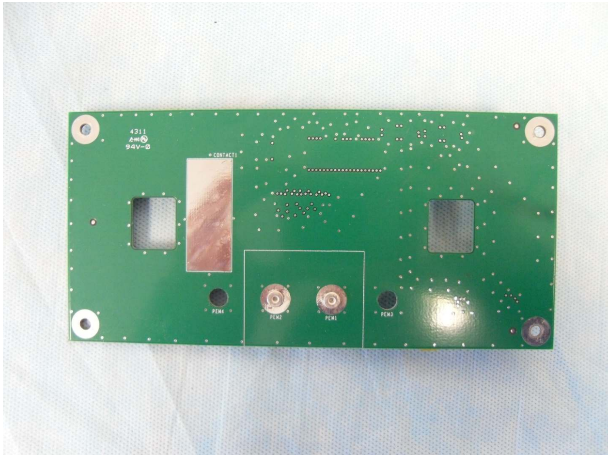
Display Adapter Board (Bottom View)
