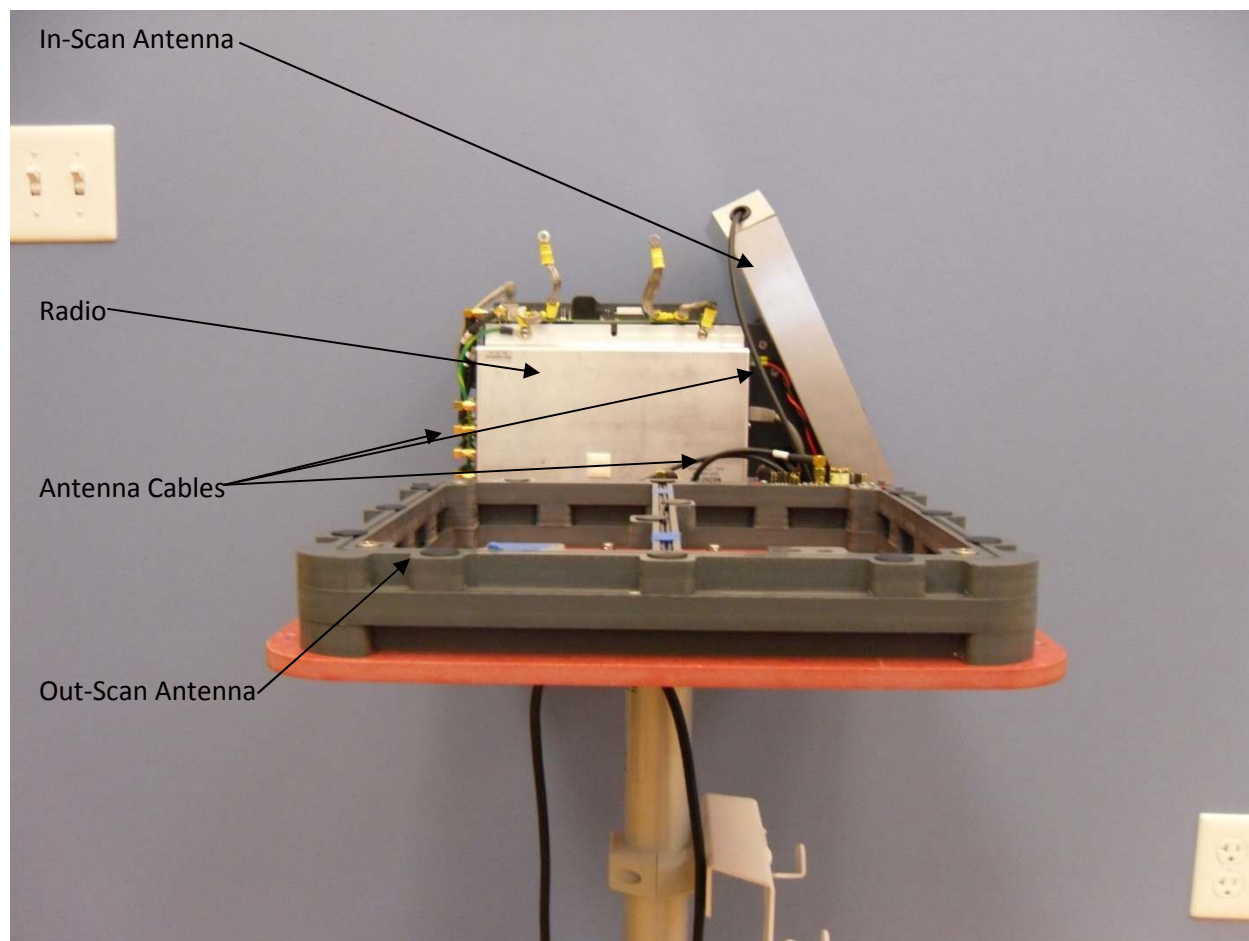
System (Front View Cover Removed)
