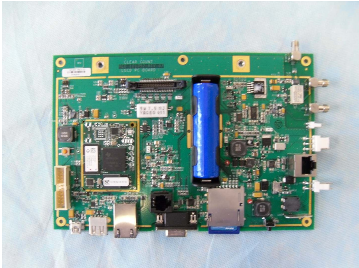
Control Board
