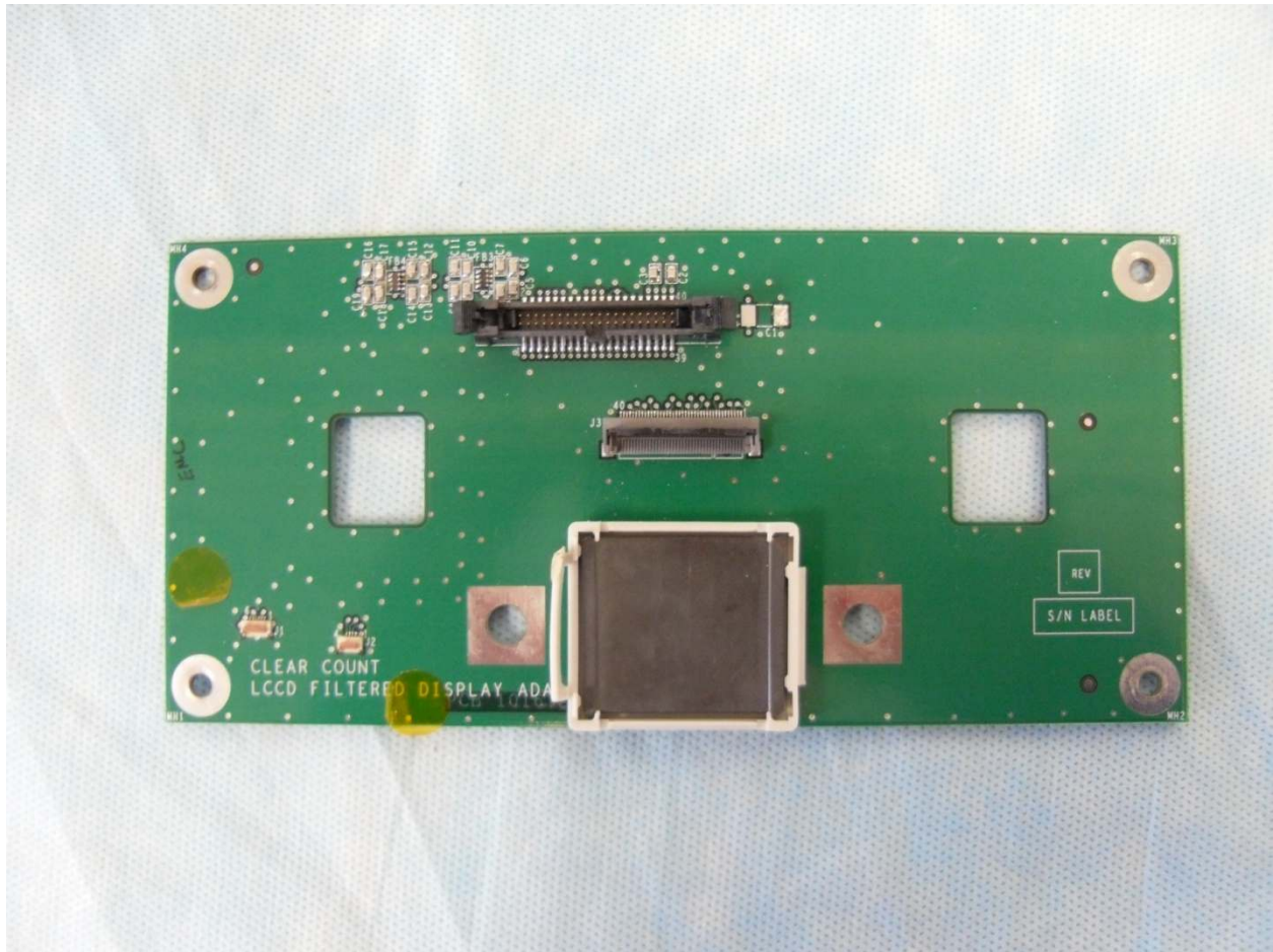
Display Adapter Board
