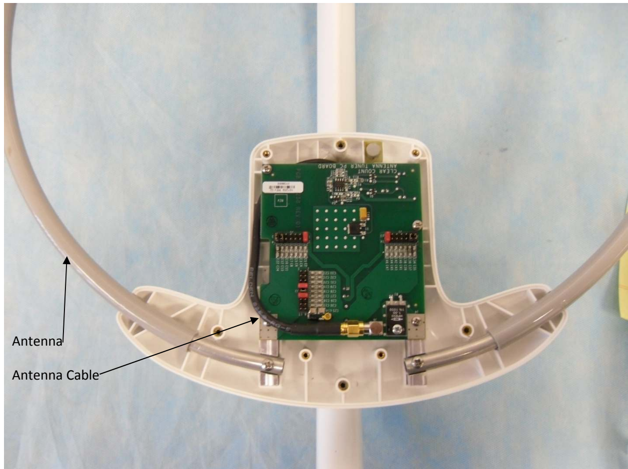
Wand Antenna Board
