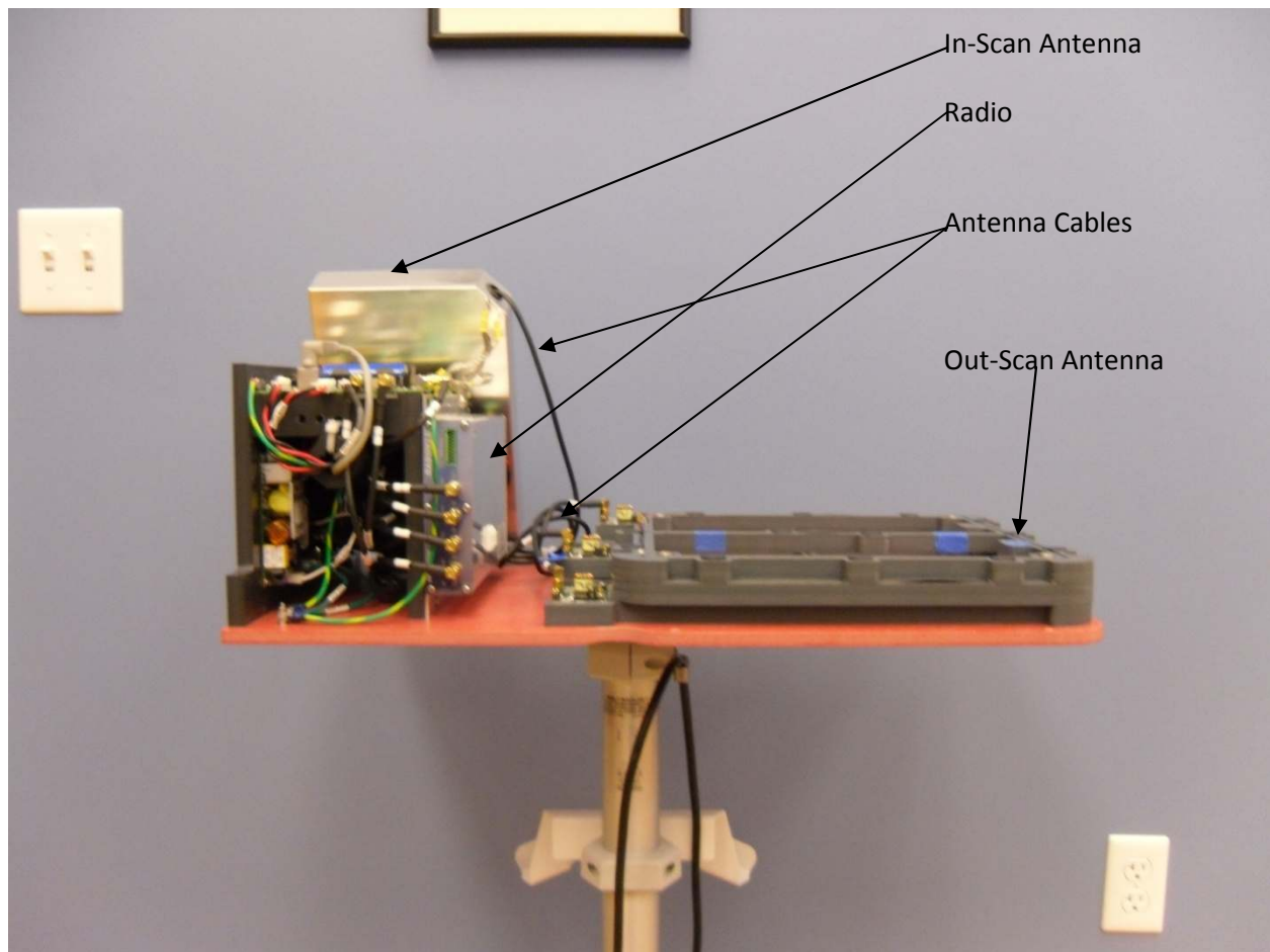
System (Side View Cover Removed)
