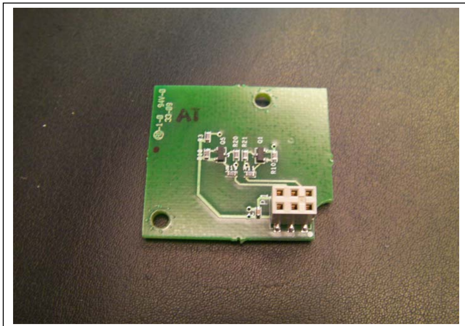
Wand LED PCB Rear
