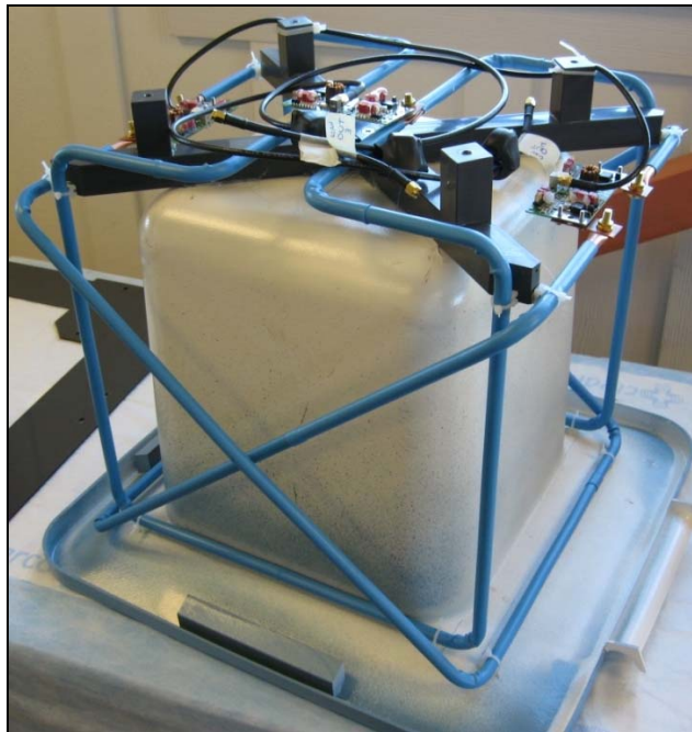
Photograph 6. Outscan Bucket Antennas
