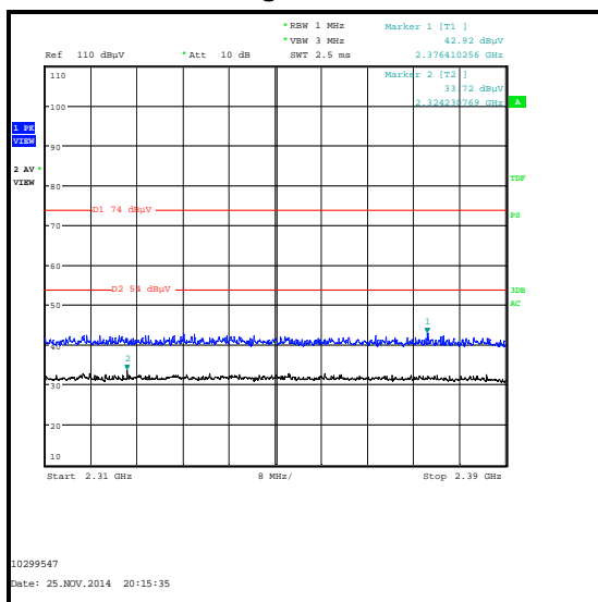
2310 MHz – 2390 MHz Restricted Band Plot
