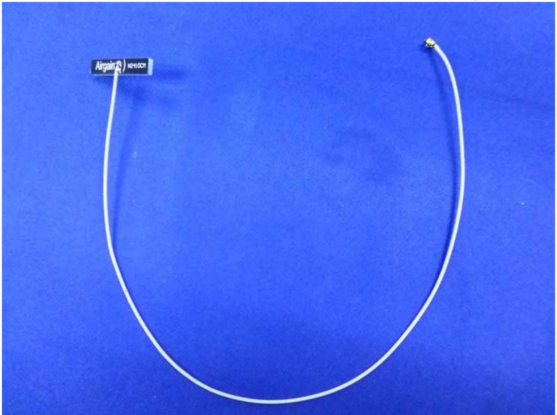
Figure 8 ANT (N2410CM-T-30U)
