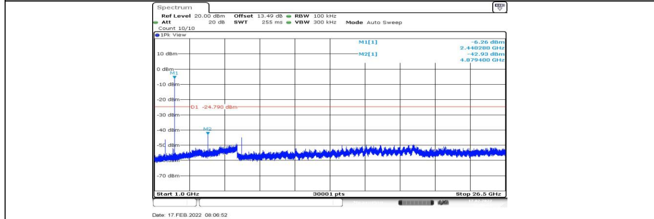
BLE_1M_Ant1_2440_1000~26500
