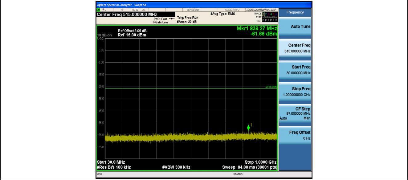
BLE_1M_Ant1_2440_30~1000
