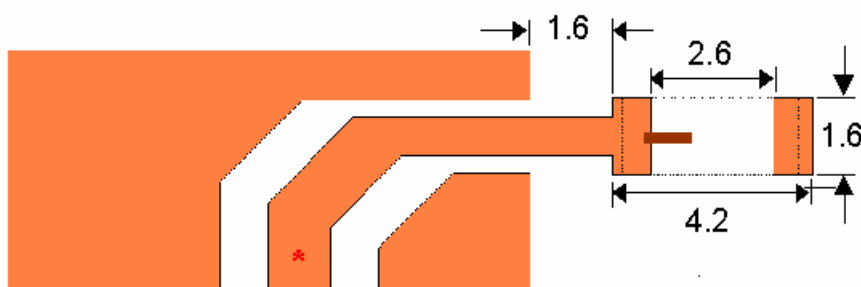
(a) Without Matching Circuits
