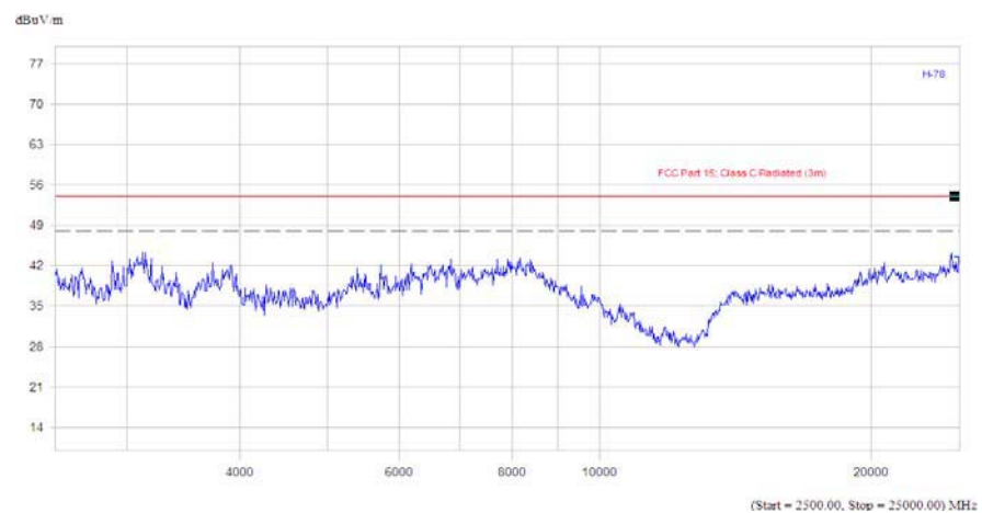
(Plot C.4: Antenna Horizontal, 2.5GHz to 25GHz)
