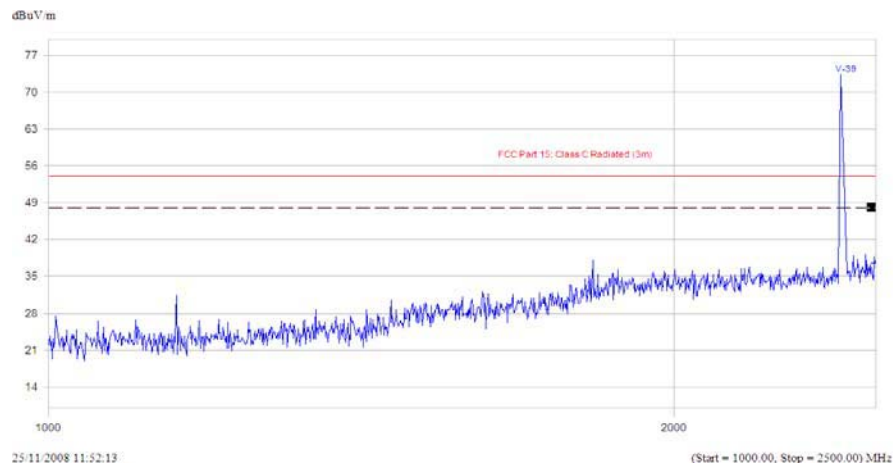
(Plot B.6: Antenna Vertical, 1GHz to 2.5GHz)
