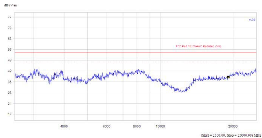
(Plot B.7: Antenna Vertical, 2.5GHz to 25GHz)
