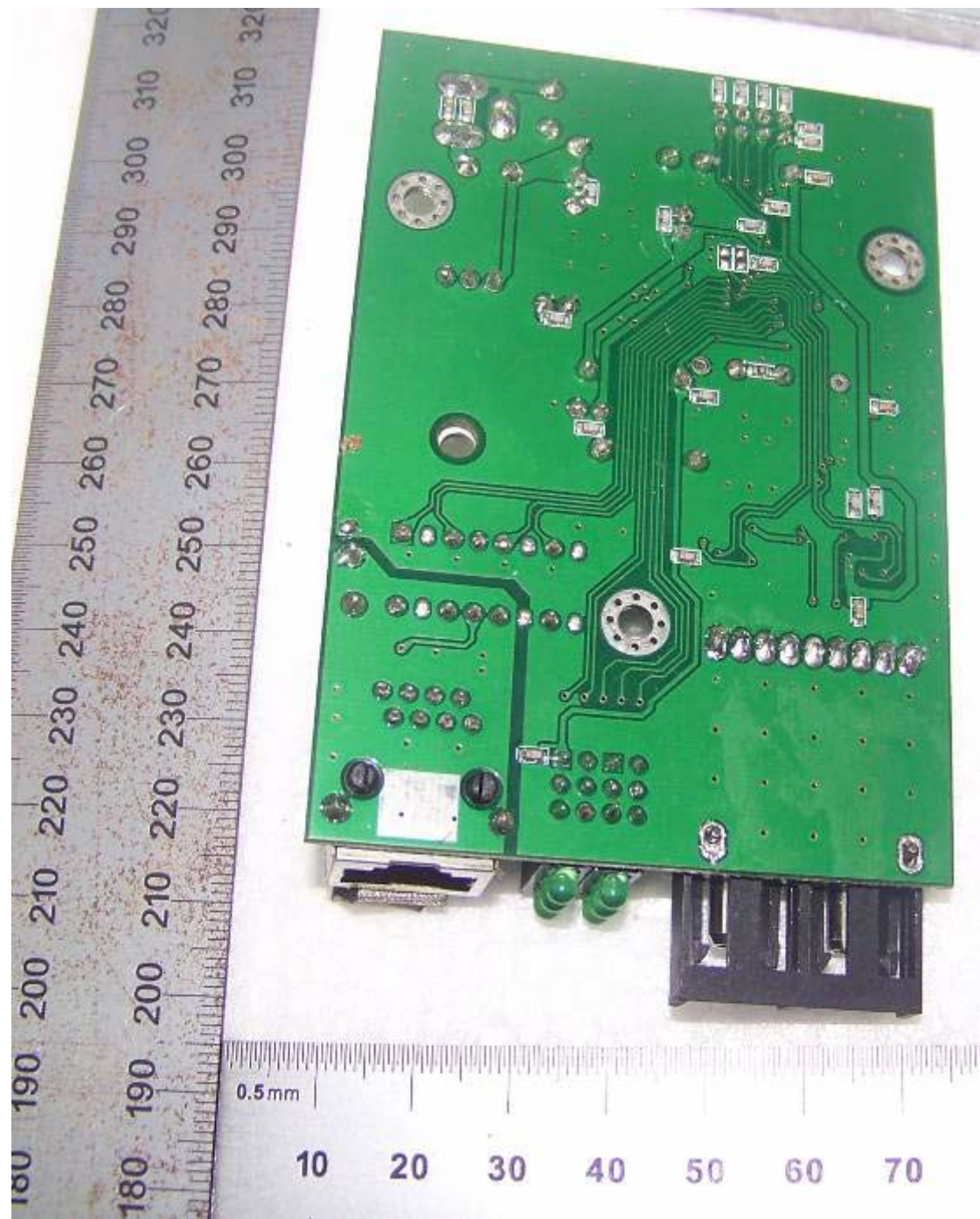
Sample with SFB transceiver module
