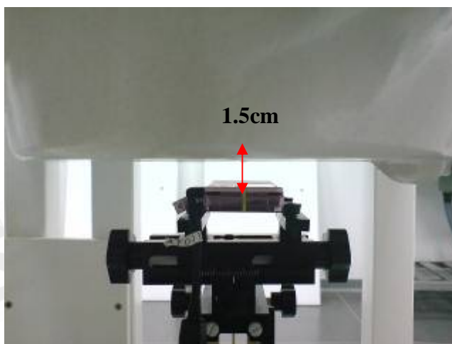
Fig.7 Body worn- EUT back to flat phantom and distance between flat phantom and mobile phone is 1.5 cm with headset
