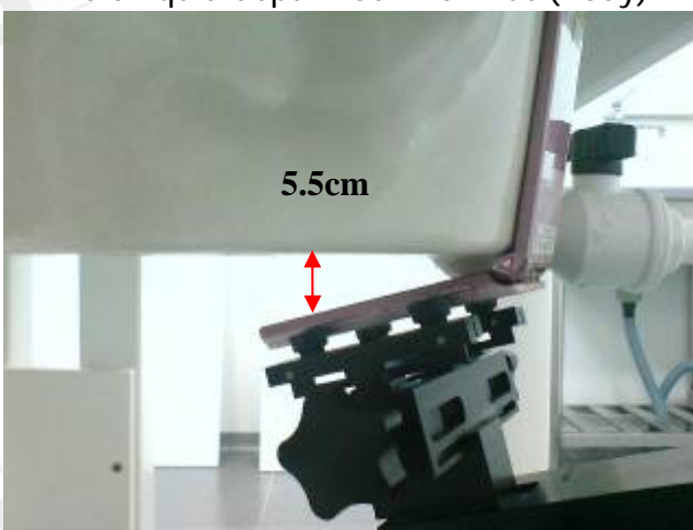
Fig.3.2 Mouth with flat phantom, cheek position
