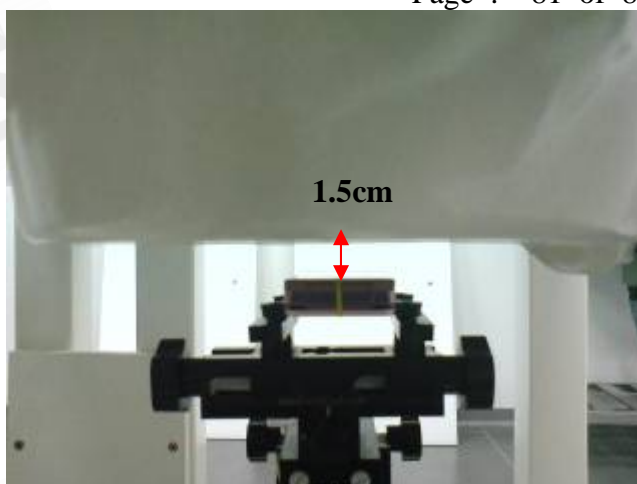
Fig.5 Body worn- EUT front to flat phantom and distance between flat phantom and mobile phone is 1.5 cm
