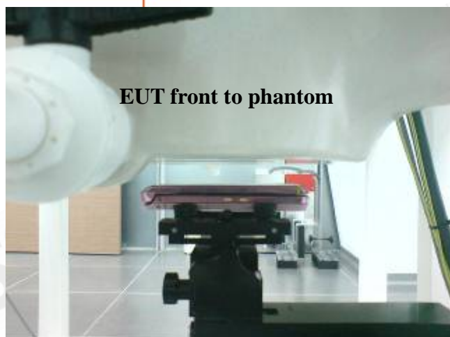
Fig.5 Body worn- EUT front to flat phantom and distance between flat phantom and mobile phone is 1.5 cm
