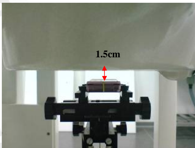
Fig.6 Body worn- EUT back to flat phantom and distance between flat phantom and mobile phone is 1.5 cm
