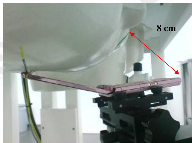
Fig.4.1 Right Head Section/Ear-Tilt(15°) Position
