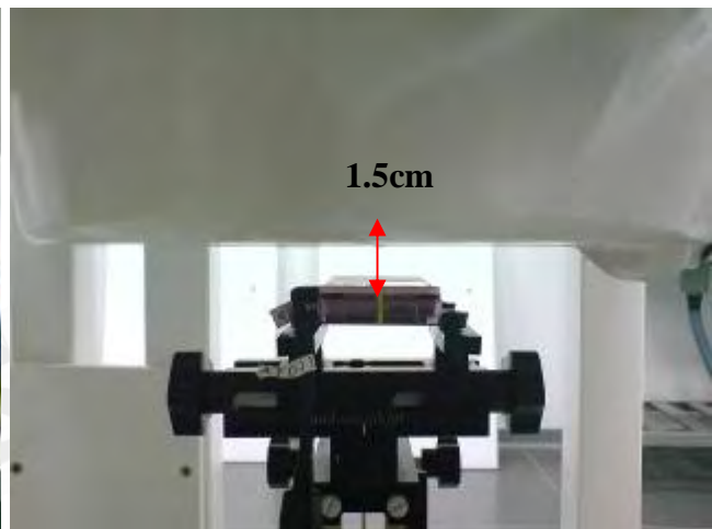
Fig.7 Body worn- EUT back to flat phantom and distance between flat phantom and mobile phone is 1.5 cm with headset
