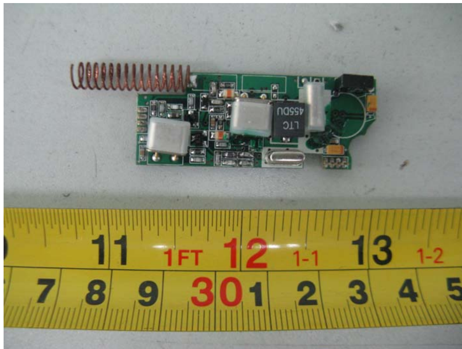
EUT- RF Board Circuit View
