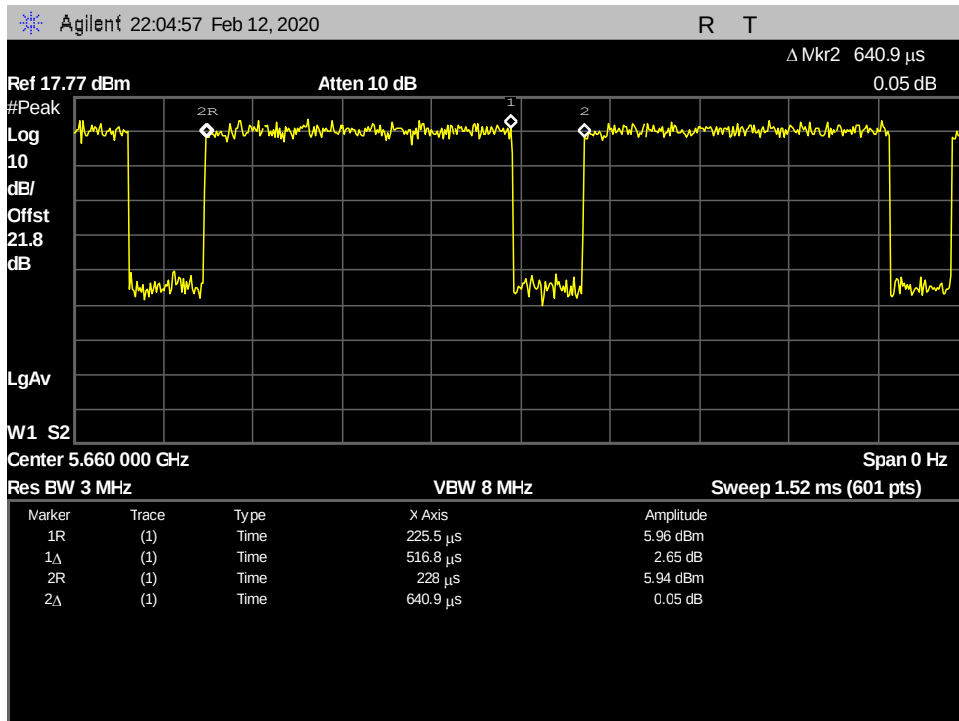
Figure 10: §15.407(b)(1) & (6 – 7) Undesirable Emissions, 802.11ac20 Duty Cycle
