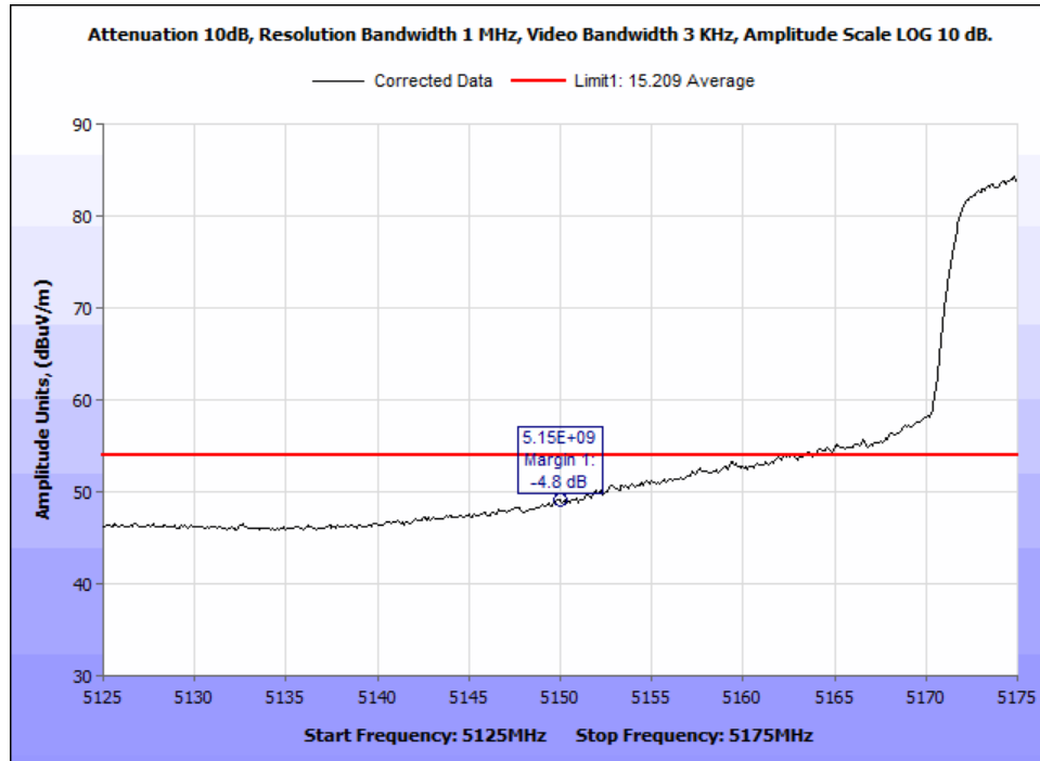
Figure 72: §15.407(b)(1) & (6 – 7) Undesirable Emissions, 802.11ac Average Radiated Bandedge @5150MHz - 40MHz 5190MHz.
