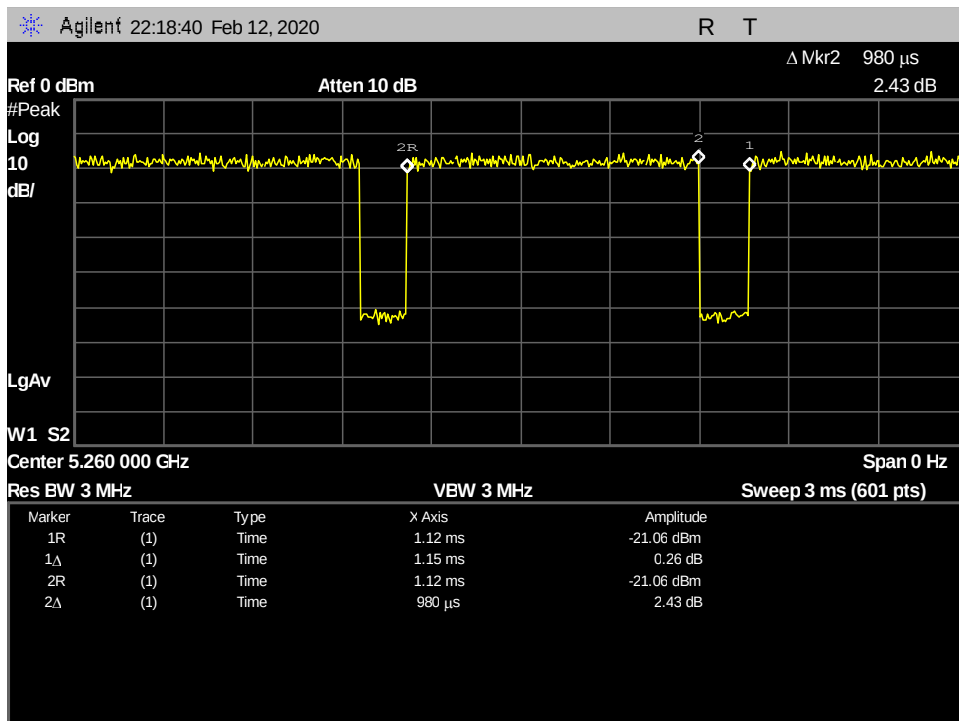
Figure 13: §15.407(b)(1) & (6 – 7) Undesirable Emissions, 802.11n20 Duty Cycle
