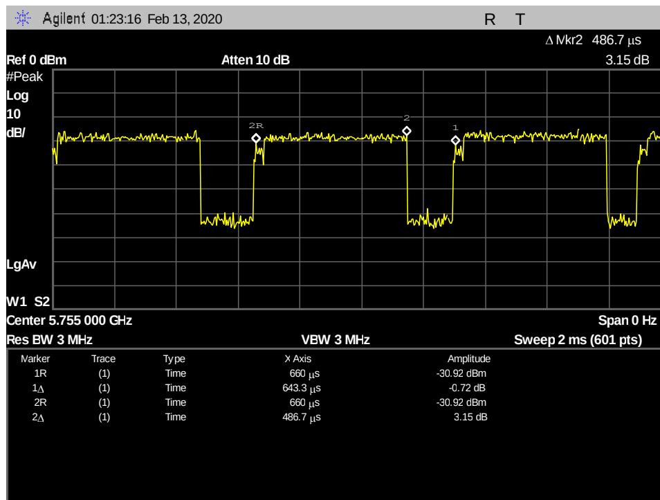
Figure 14: §15.407(b)(1) & (6 – 7) Undesirable Emissions, 802.11n40 Duty Cycle
