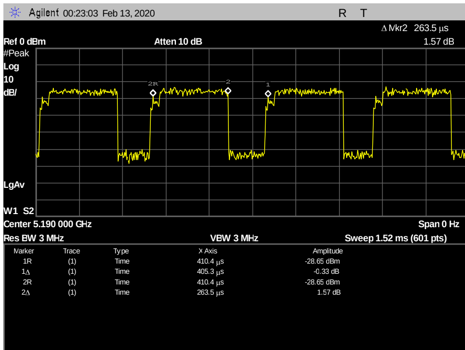
Figure 11: §15.407(b)(1) & (6 – 7) Undesirable Emissions, 802.11ac40 Duty Cycle
