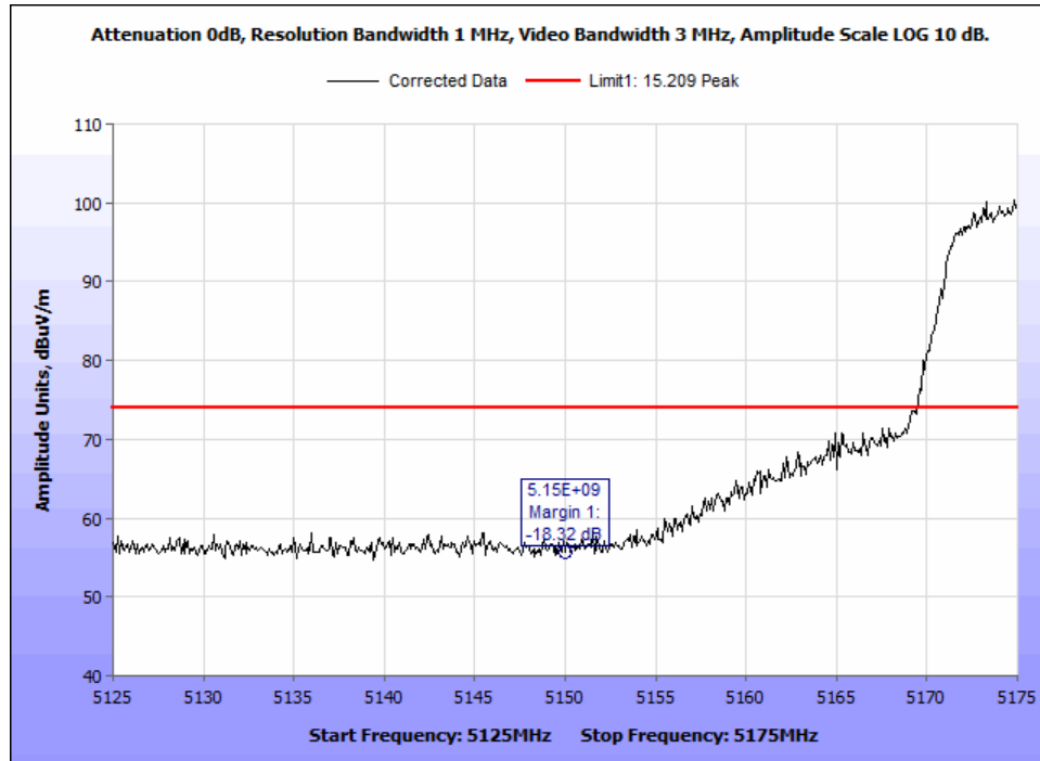
Figure 74: §15.407(b)(1) & (6 – 7) Undesirable Emissions, 802.11ac Peak Radiated Bandedge @5150MHz - 20MHz 5180MHz.
