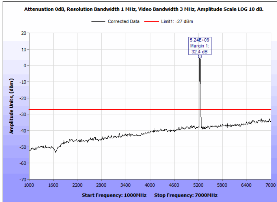
Figure 18: §15.407(b)(1) & (6 – 7) Undesirable Emissions, -27dBm Radiated Emissions - 802.11a 20M 5240M - 1-7GHz.
