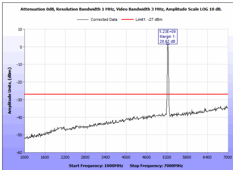
Figure 28: §15.407(b)(1) & (6 – 7) Undesirable Emissions, -27dBm Radiated Emissions - 802.11n 40M 5190M - 1-7GHz.
