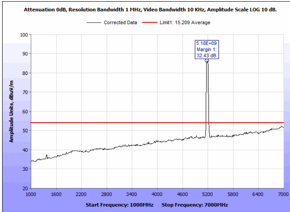
Figure 38: §15.407(b)(1) & (6 – 7) Undesirable Emissions, Average Radiated Emissions - 802.11ac 40M 5190M - 1-7GHz.
