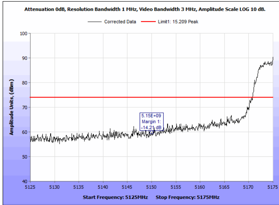
Figure 76: §15.407(b)(1) & (6 – 7) Undesirable Emissions, 802.11ac Peak Radiated Bandedge @5150MHz - 80MHz 5210MHz.
