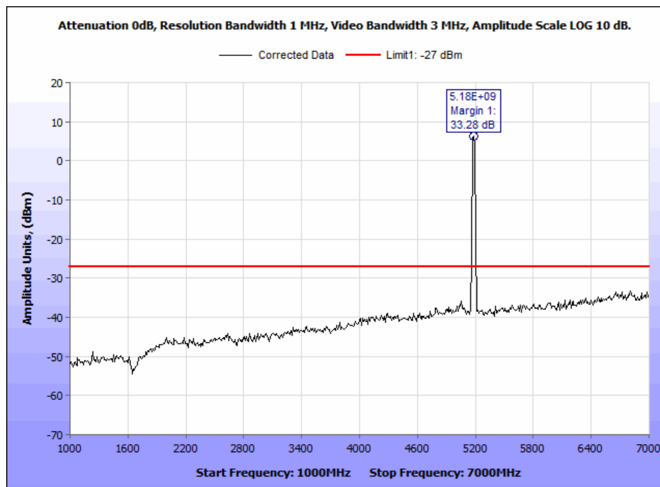
Figure 16: §15.407(b)(1) & (6 – 7) Undesirable Emissions, -27dBm Radiated Emissions - 802.11a 20M 5180M - 1-7GHz.
