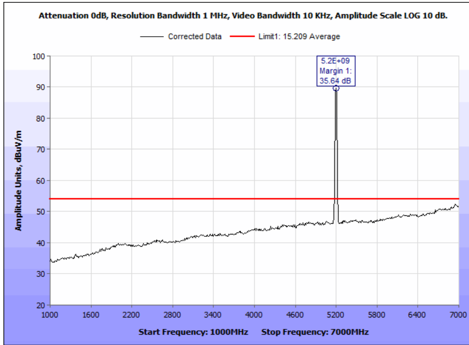
Figure 36: §15.407(b)(1) & (6 – 7) Undesirable Emissions, Average Radiated Emissions - 802.11ac 20M 5200M - 1-7GHz.
