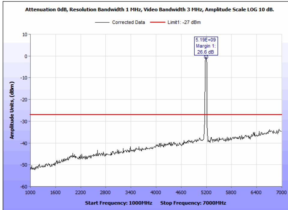
Figure 22: §15.407(b)(1) & (6 – 7) Undesirable Emissions, -27dBm Radiated Emissions - 802.11ac 40M 5190M - 1-7GHz.
