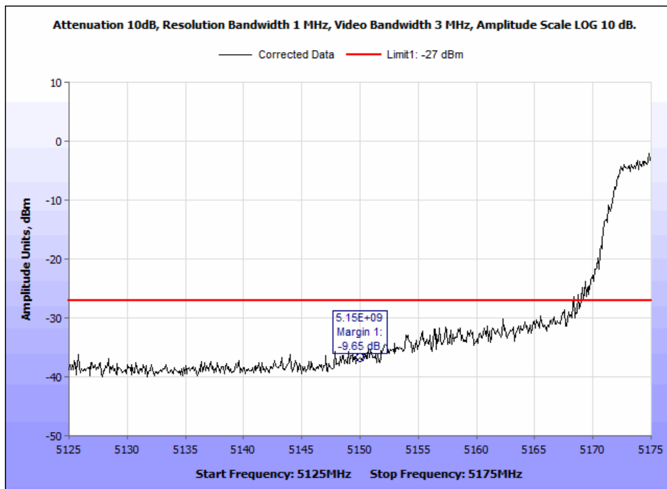
Figure 68: §15.407(b)(1) & (6 – 7) Undesirable Emissions, 802.11ac -27dBm Radiated Bandedge @5150MHz - 20MHz 5180MHz.
