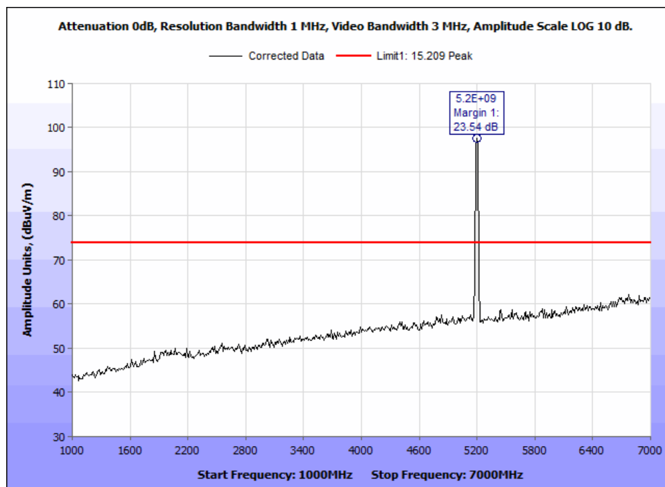
Figure 52: §15.407(b)(1) & (6 – 7) Undesirable Emissions, Peak Radiated Emissions - 802.11ac 20M 5180M - 1-7GHz.
