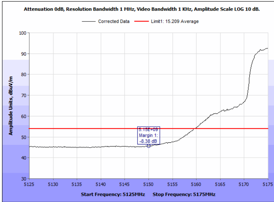
Figure 66: §15.407(b)(1) & (6 – 7) Undesirable Emissions, 802.11a Average Radiated Bandedge @5150MHz - 20MHz 5180MHz.
