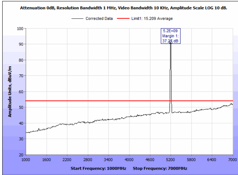
Figure 42: §15.407(b)(1) & (6 – 7) Undesirable Emissions, Average Radiated Emissions - 802.11n 20M 5200M - 1-7GHz.
