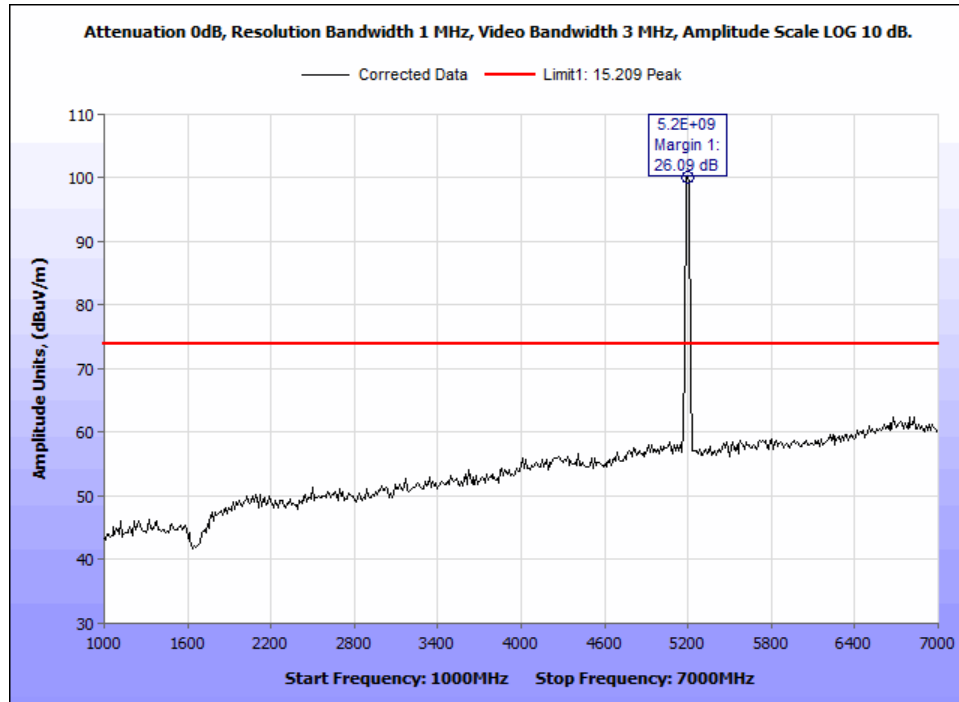
Figure 50: §15.407(b)(1) & (6 – 7) Undesirable Emissions, Peak Radiated Emissions - 802.11a 20M 5200M - 1-7GHz.
