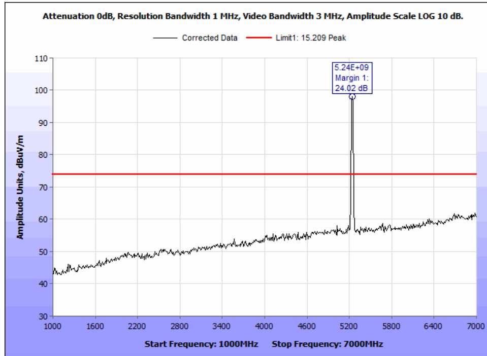
Figure 54: §15.407(b)(1) & (6 – 7) Undesirable Emissions, Peak Radiated Emissions - 802.11ac 20M 5240M - 1-7GHz.
