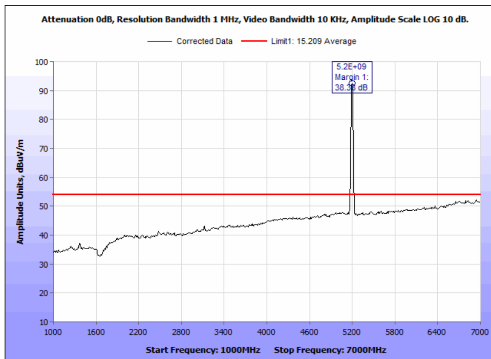
Figure 32: §15.407(b)(1) & (6 – 7) Undesirable Emissions, Average Radiated Emissions - 802.11a 20M 5180M - 1-7GHz.
