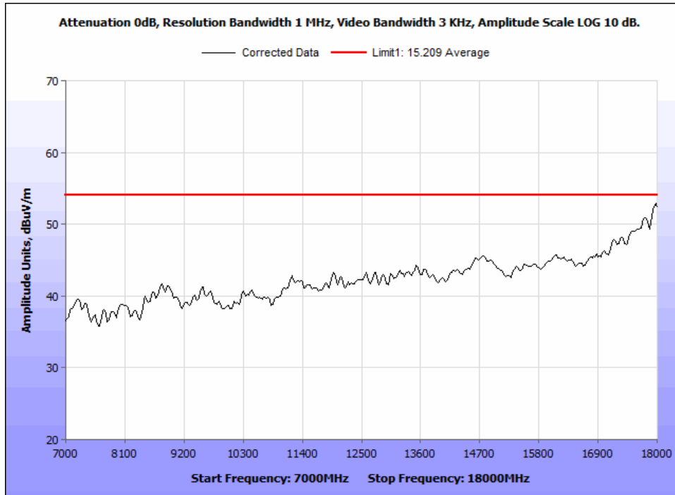
Figure 46: §15.407(b)(1) & (6 – 7) Undesirable Emissions, AVG_15.209_worst case_Radiated Emissions_7-18GHz.
