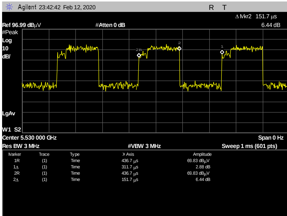
Figure 12: §15.407(b)(1) & (6 – 7) Undesirable Emissions, 802.11ac80 Duty Cycle
