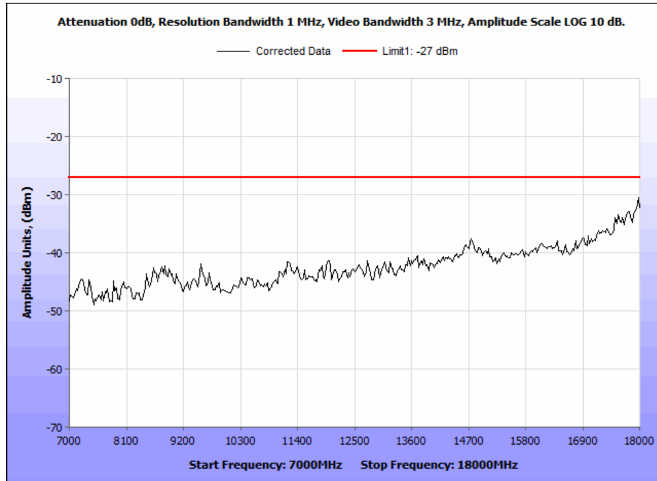
Figure 30: §15.407(b)(1) & (6 – 7) Undesirable Emissions, -27dBm_15.407_worst case_Radiated Emissions_7-18GHz.
