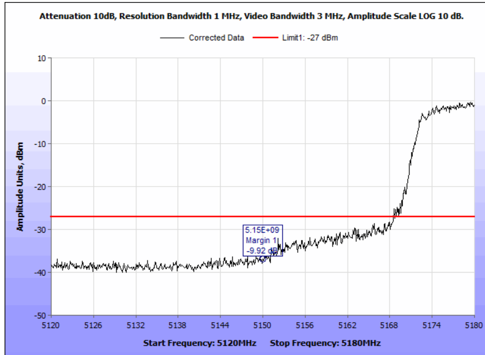
Figure 78: §15.407(b)(1) & (6 – 7) Undesirable Emissions, 802.11n -27dBm Radiated Bandedge @5150MHz - 40MHz 5190MHz.
