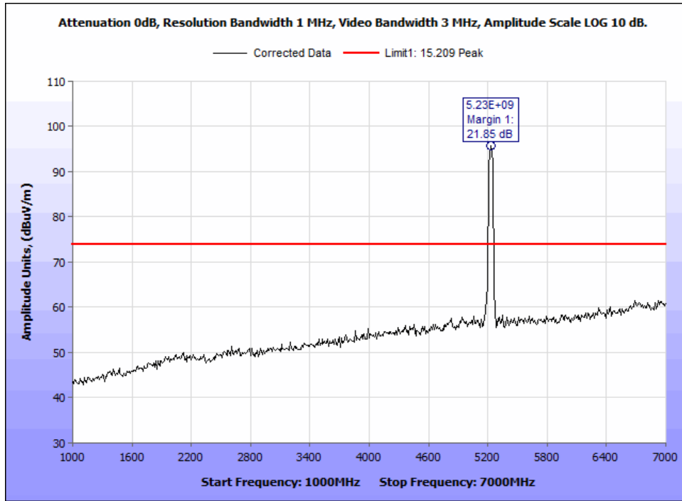
Figure 56: §15.407(b)(1) & (6 – 7) Undesirable Emissions, Peak Radiated Emissions - 802.11ac 40M 5230M - 1-7GHz.
