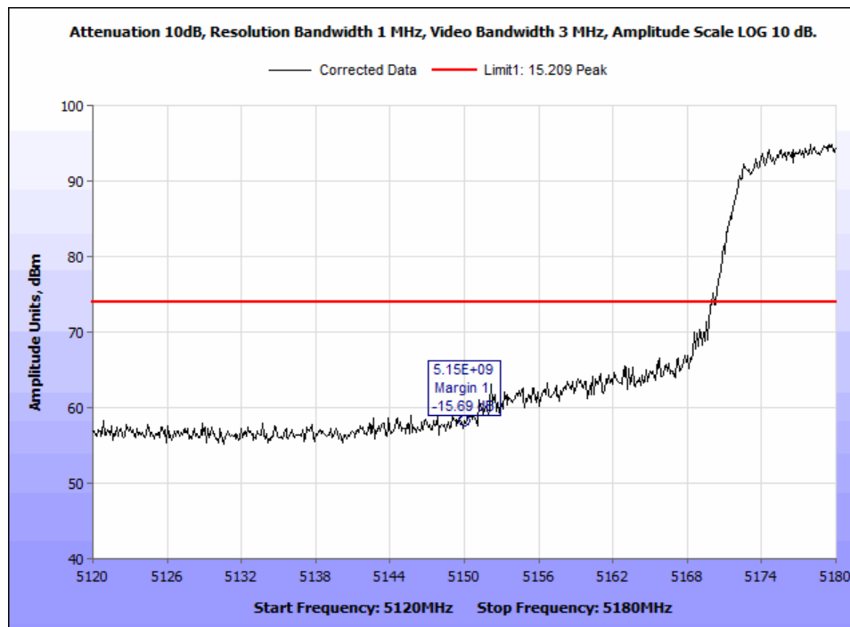
Figure 82: §15.407(b)(1) & (6 – 7) Undesirable Emissions, 802.11n Peak Radiated Bandedge @5150MHz - 40MHz 5190MHz.
