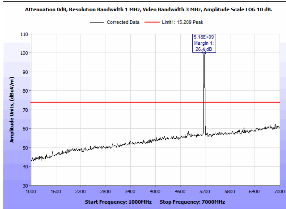
Figure 58: §15.407(b)(1) & (6 – 7) Undesirable Emissions, Peak Radiated Emissions - 802.11n 20M 5180M - 1-7GHz.
