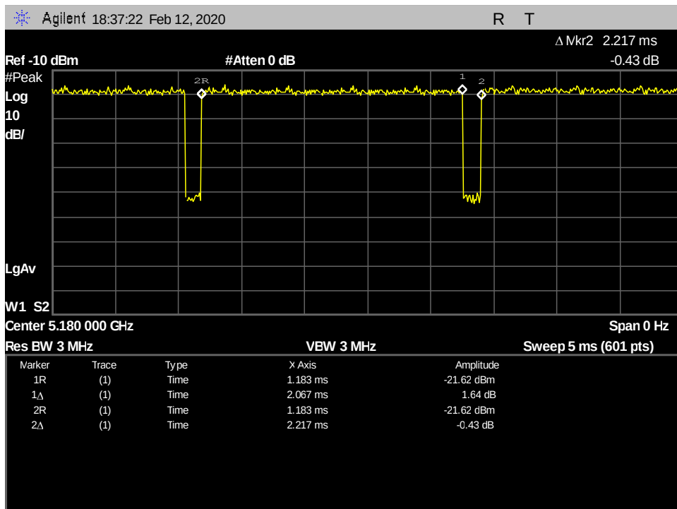
Figure 9: §15.407(b)(1) & (6 – 7) Undesirable Emissions, 802.11a Duty Cycle
