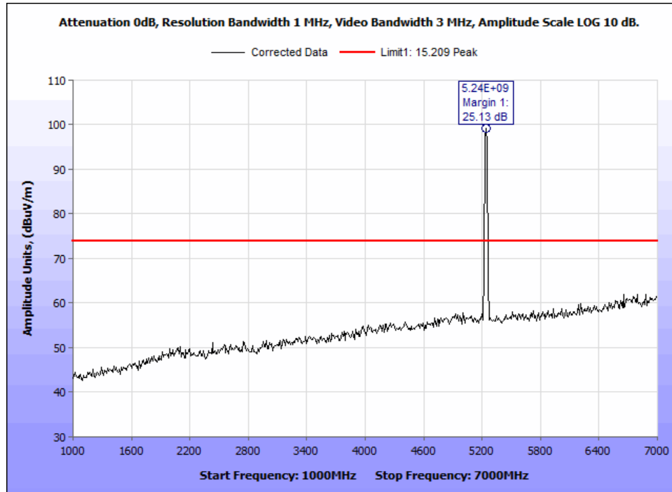
Figure 60: §15.407(b)(1) & (6 – 7) Undesirable Emissions, Peak Radiated Emissions - 802.11n 20M 5240M - 1-7GHz.
