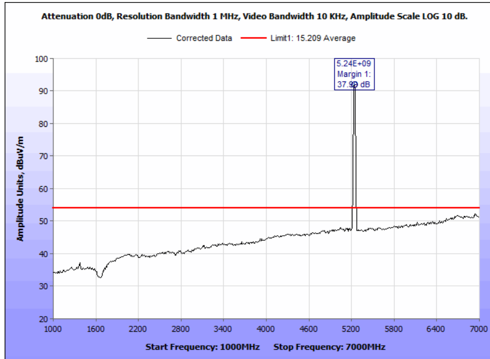
Figure 34: §15.407(b)(1) & (6 – 7) Undesirable Emissions, Average Radiated Emissions - 802.11a 20M 5240M - 1-7GHz.
