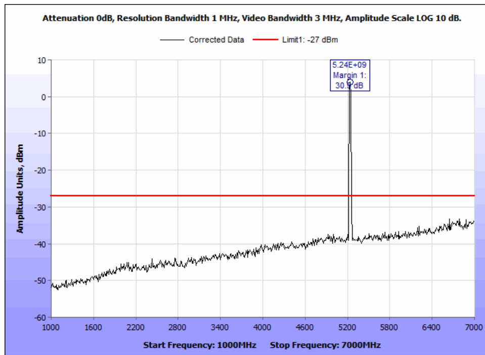
Figure 26: §15.407(b)(1) & (6 – 7) Undesirable Emissions, -27dBm Radiated Emissions - 802.11n 20M 5200M - 1-7GHz.
