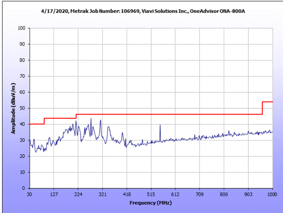
Figure 8: §15.407(b)(1) & (6 – 7) Undesirable Emissions, 15.209 worst case - below 1GHz.
