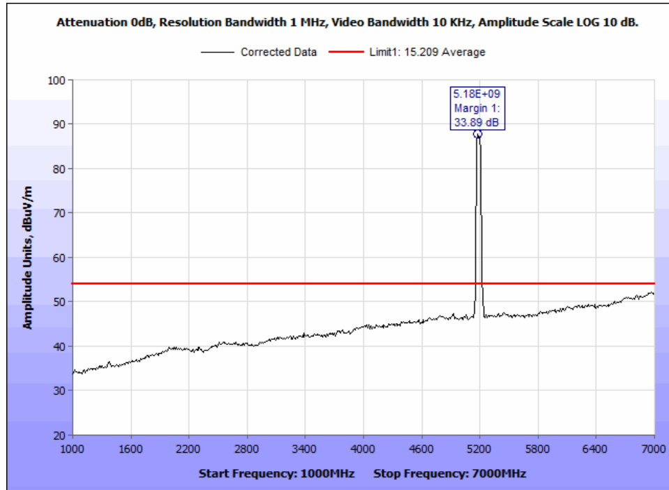
Figure 44: §15.407(b)(1) & (6 – 7) Undesirable Emissions, Average Radiated Emissions - 802.11n 40M 5190M - 1-7GHz.
