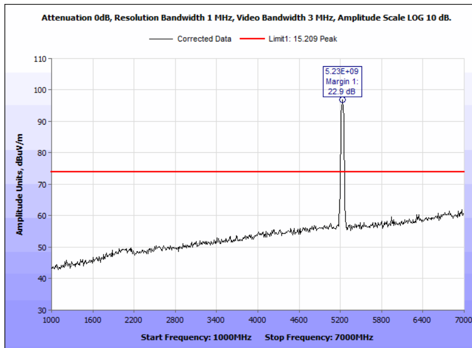
Figure 62: §15.407(b)(1) & (6 – 7) Undesirable Emissions, Peak Radiated Emissions - 802.11n 40M 5230M - 1-7GHz.
