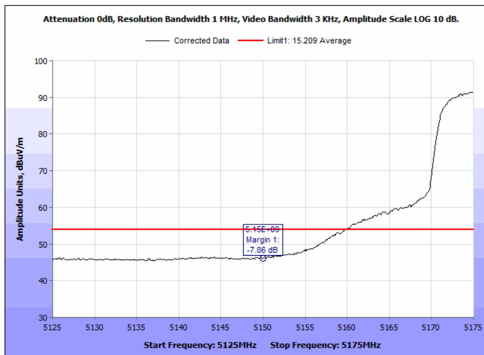
Figure 70: §15.407(b)(1) & (6 – 7) Undesirable Emissions, 802.11ac -27dBm Radiated Bandedge @5150MHz - 80MHz 5210MHz.
