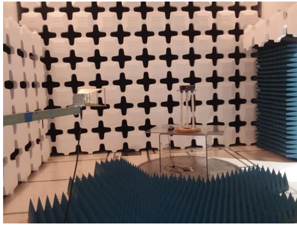
Figure 1: Radiated Emissions Test Setup Above 1GHz
