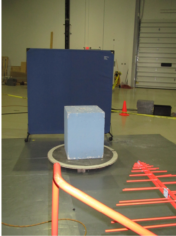
Radiated Emissions – Below 1GHz – OATS
