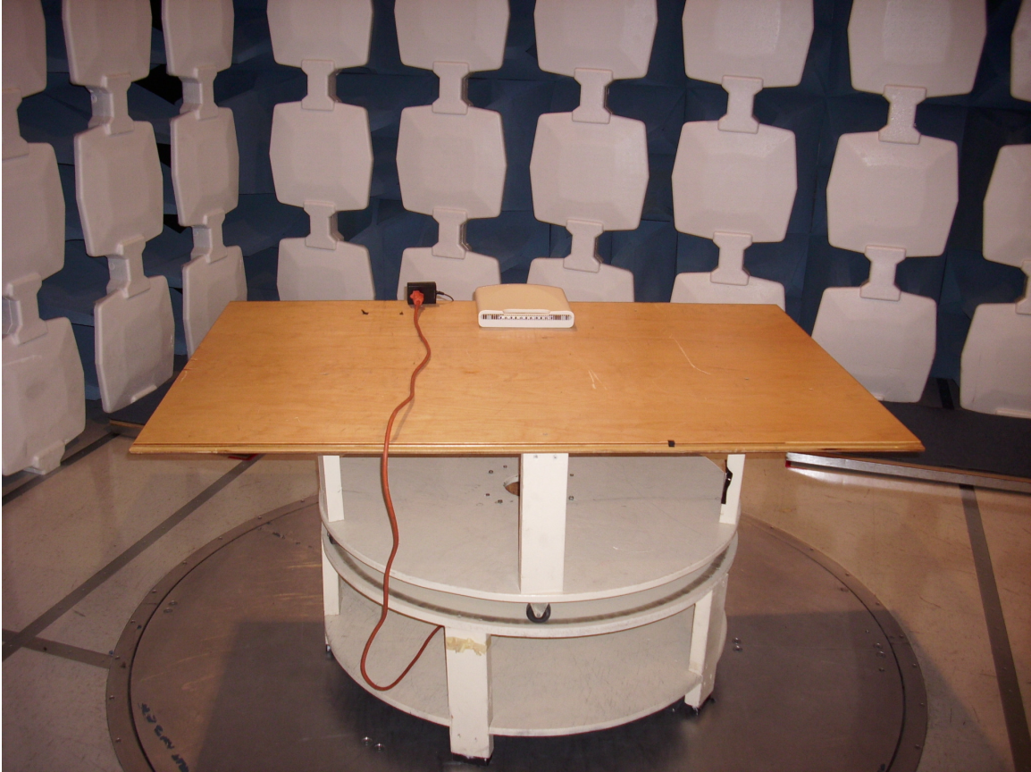
Radiated Emissions, AC Voltage Configuration, Front
