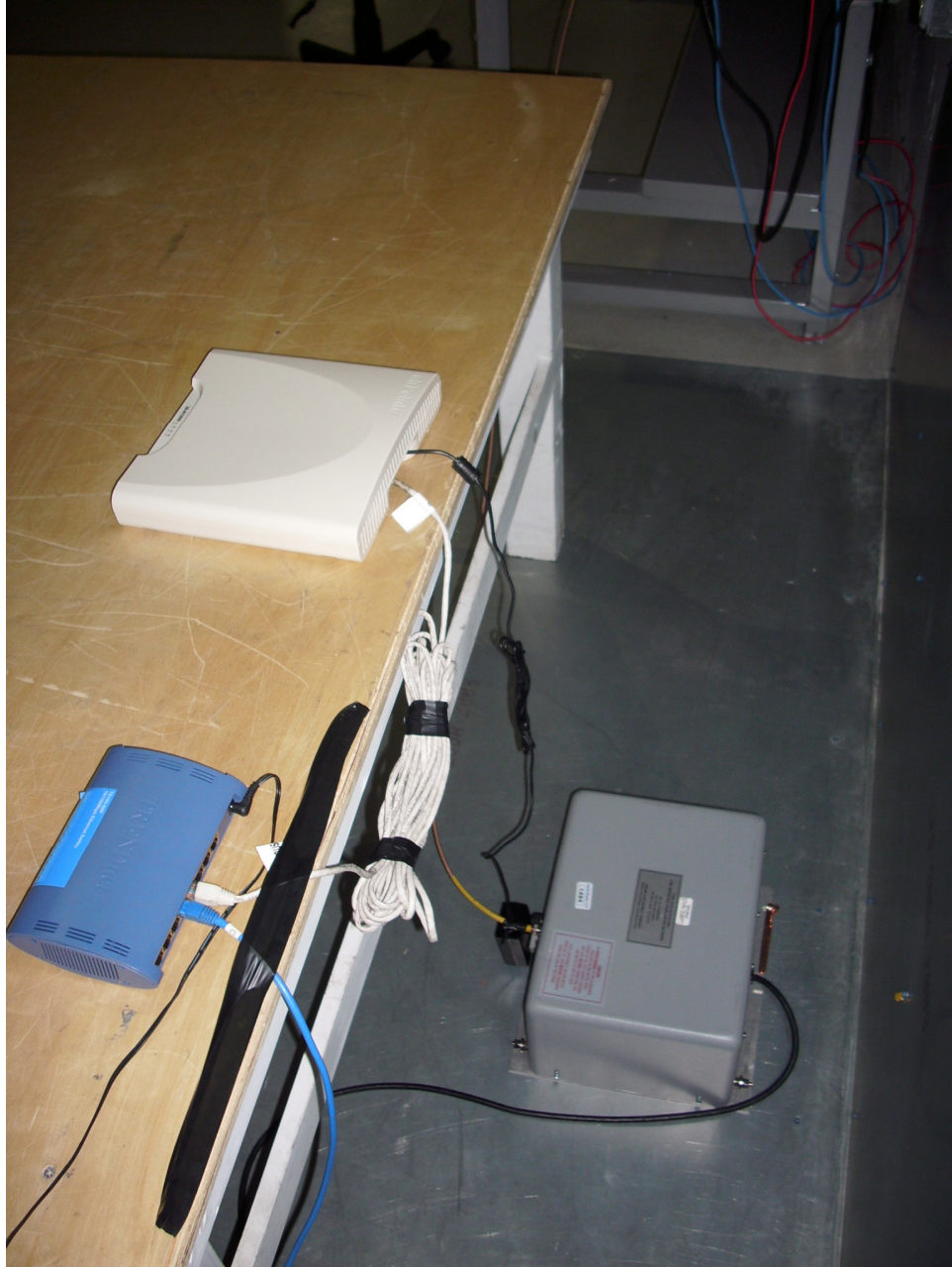
AC Mains Conducted Emissions, AC Voltage Configuration, Back
