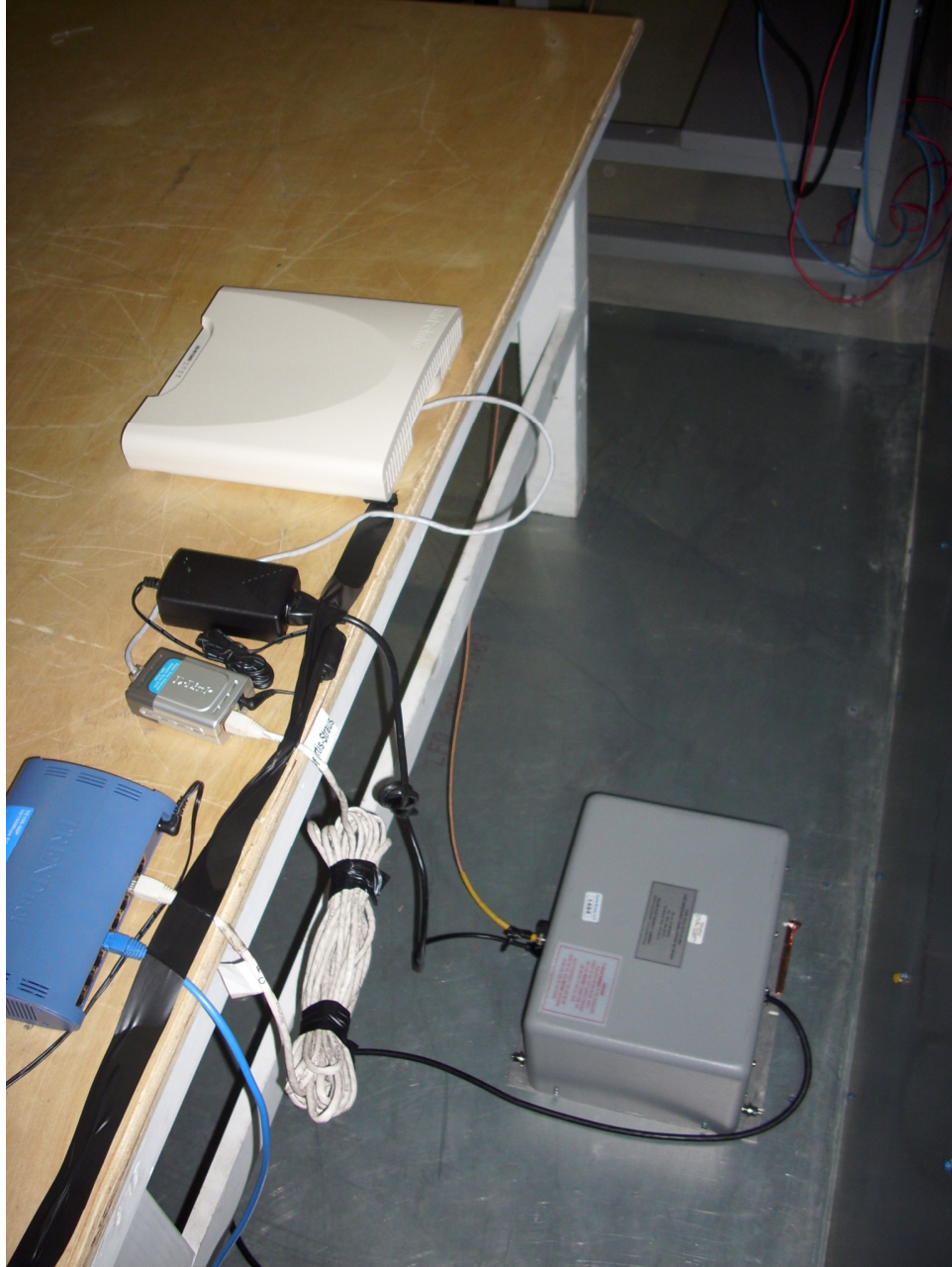
AC Mains Conducted Emissions, Power-Over-Ethernet Configuration, Back
