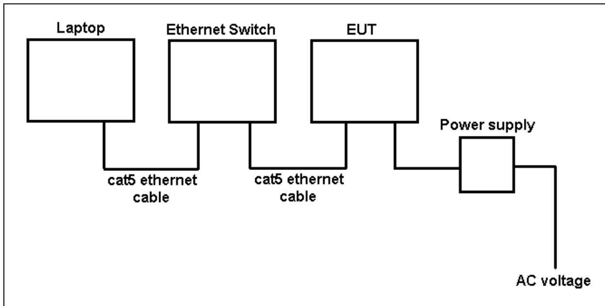
AC voltage configuration
