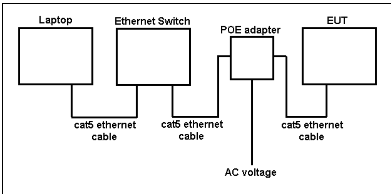
Power Over Ethernet configuration
