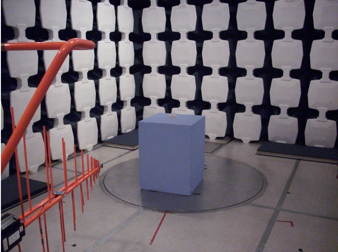
Radiated Measurements below 1GHz in Anechoic Chamber
