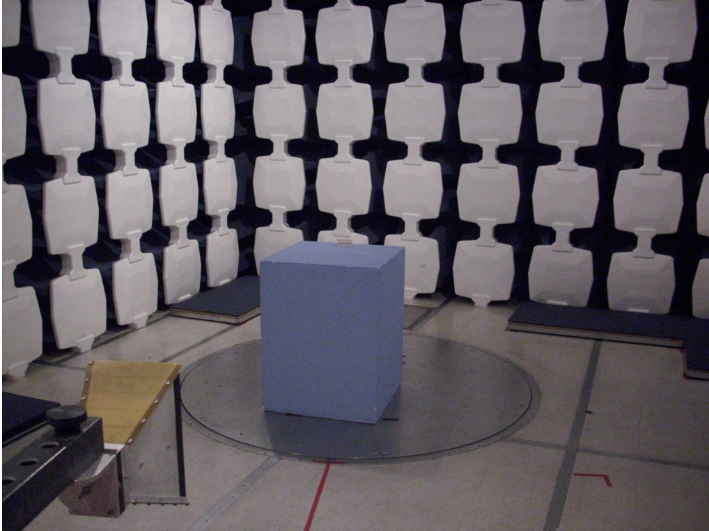
Radiated Measurements above 1GHz in Anechoic Chamber
