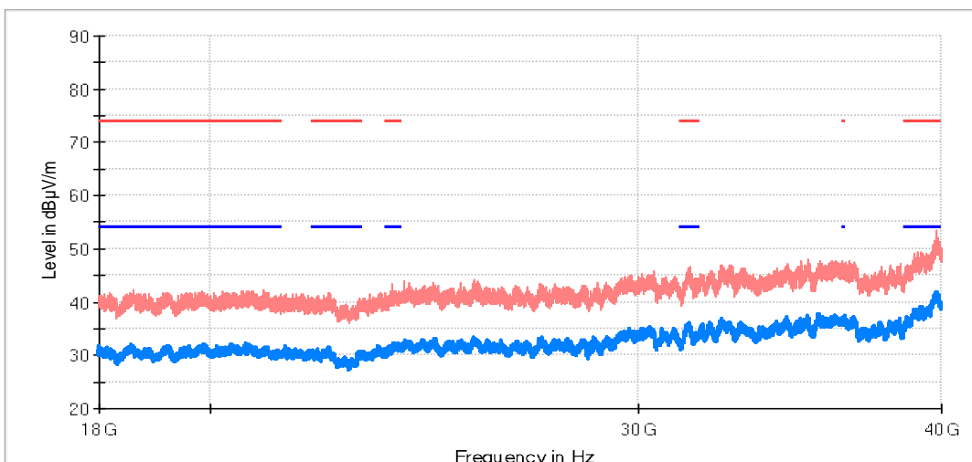
RF_FCC_15.407_E Field_18GHz_40GHz
