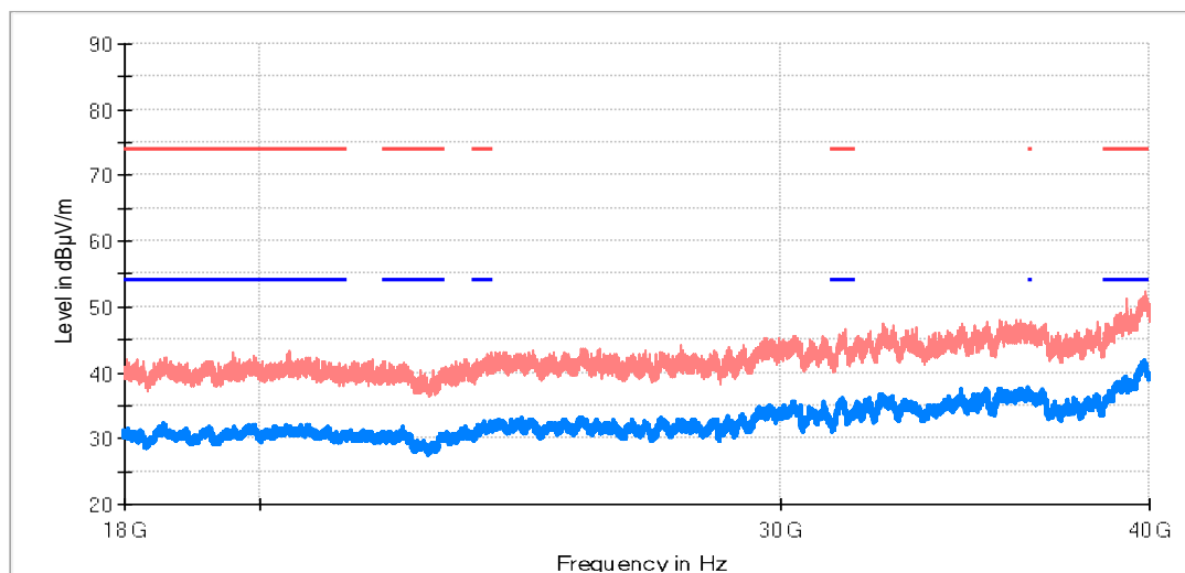
RF_FCC_15.407_E Field_18GHz_40GHz
