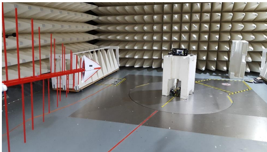
Figure B6. Radiated Emission test setup LR (0.03 – 1GHz)
