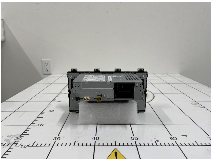
Figure B2. Rear view of the DUT
