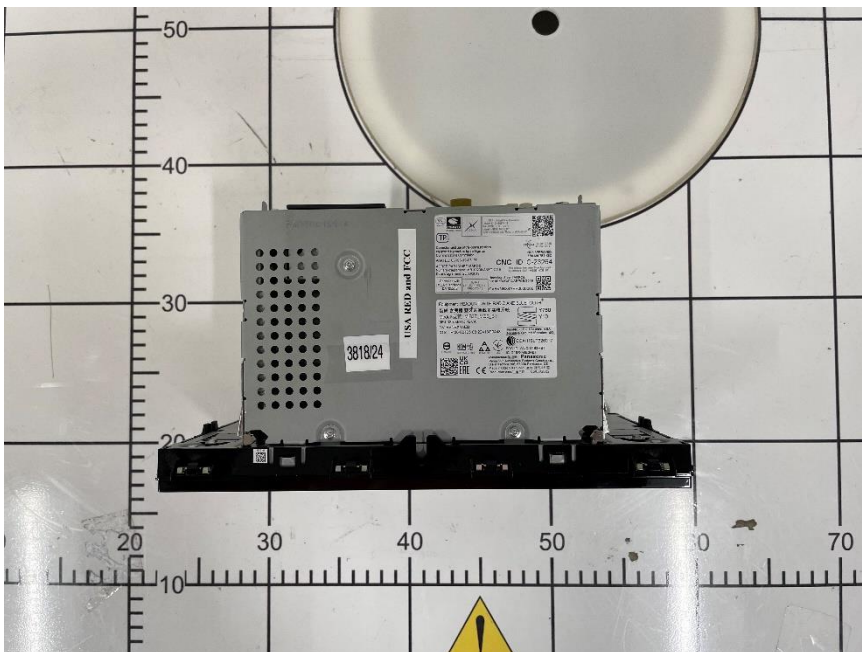
Figure B4. Top view of the DUT
