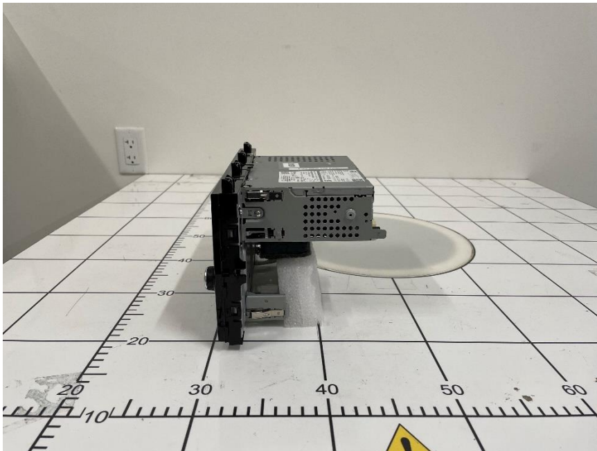
Figure B3. Side view of the DUT
