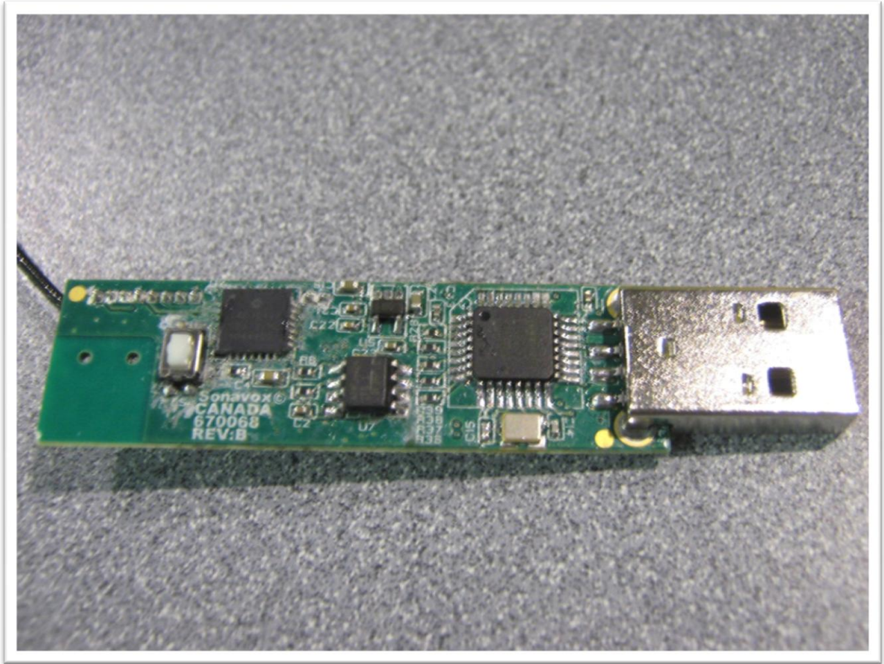
Figure 2 – EUT with chassis open Bottom
