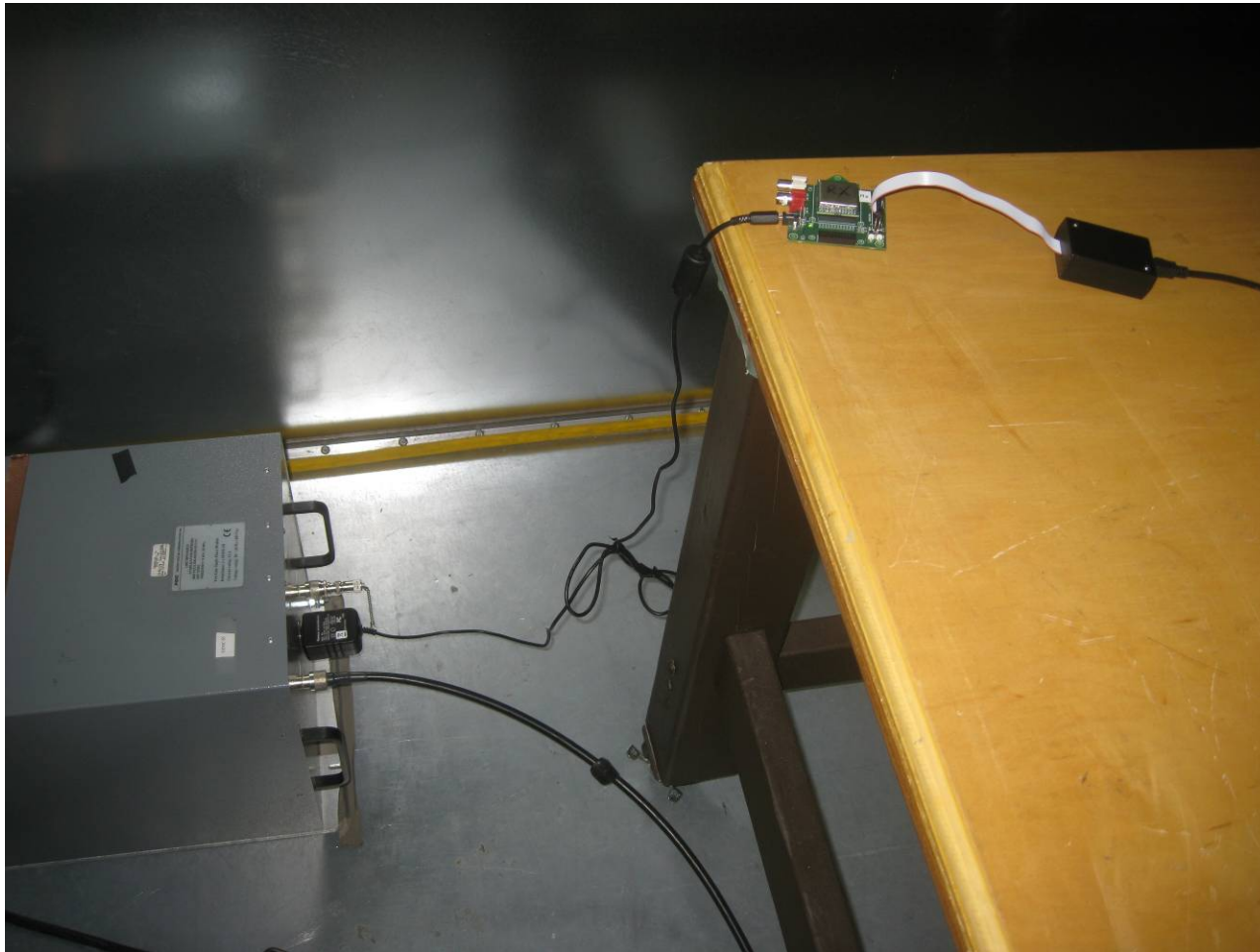
Power Line Conducted Emissions Setup 1
