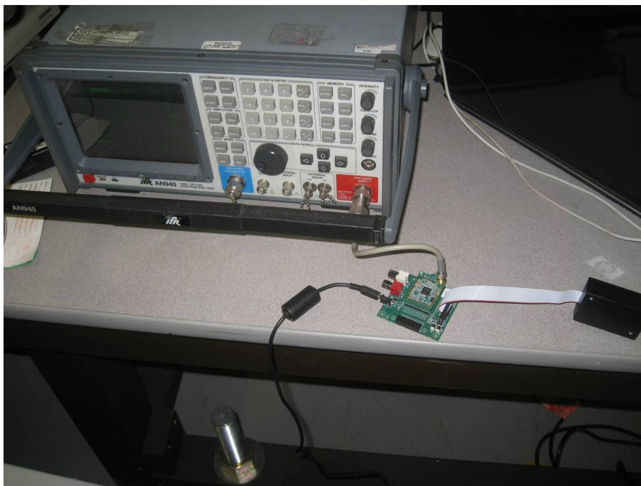
Antenna Conducted – Setup
