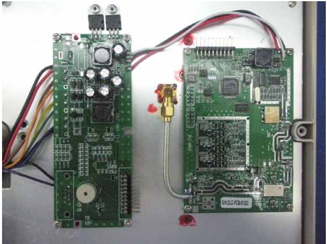
Photo 2 General Appearance of the EUT(Inside)
