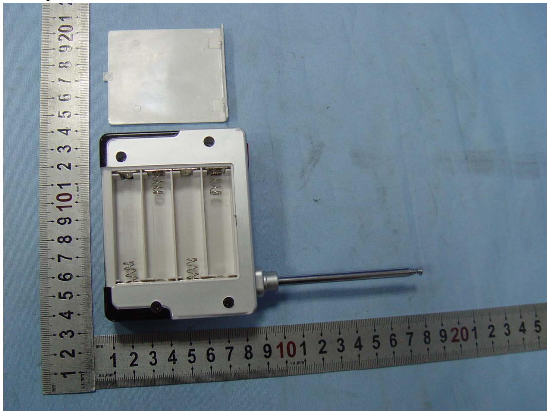
Battery Box
