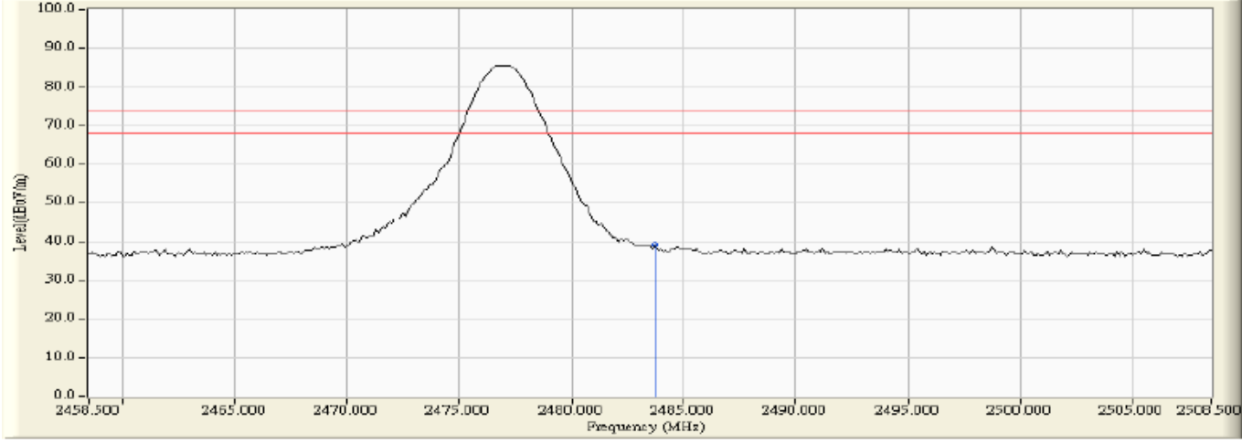
Horizontal (Peak) TX 2477MHz
