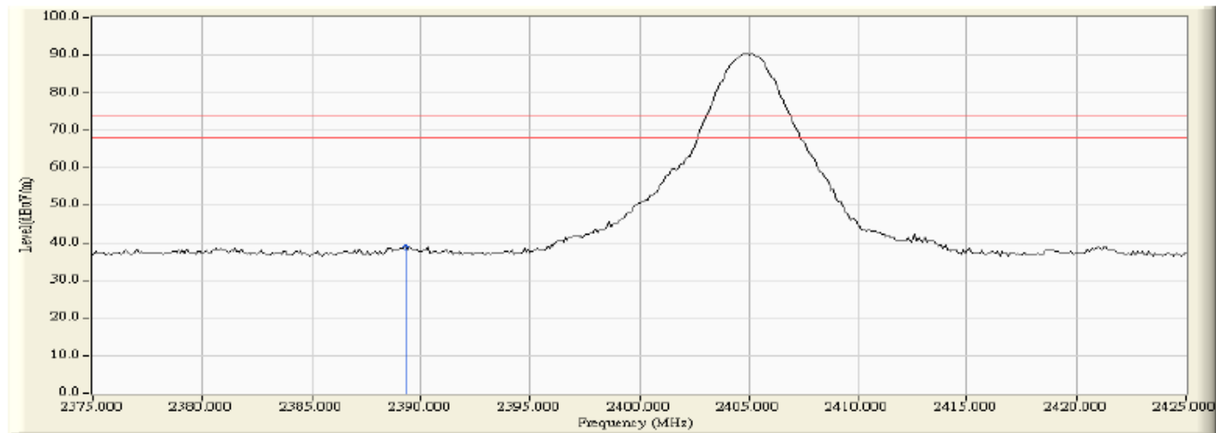
Vertical (Peak) TX 2405MHz
