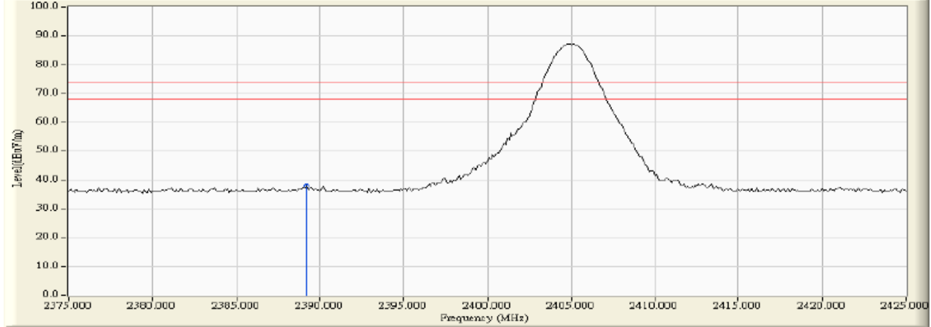
Horizontal (Peak) TX 2405MHz
